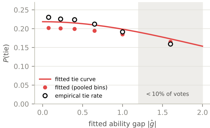
(a) Davidson ( \hat{\nu} = 0.559 , final window)
