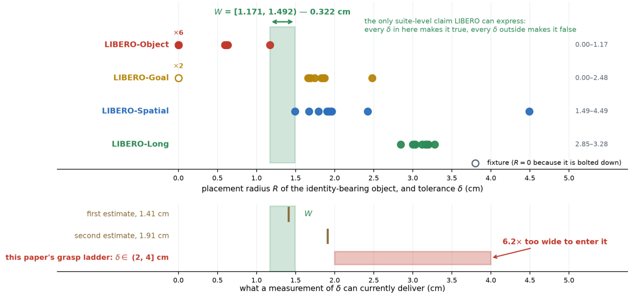
Top: all forty placement radii, computed from released files with no policy, simulator or training. The shaded strip is the decision window — the set of tolerances making “LIBERO-Object is lookup-admissible and no other suite is” true. It is the ONLY such claim of the eight LIBERO can express that any tolerance satisfies at all. Bottom: the same axis with what measurement delivers. Proposition 2 says an estimate wider than the window decides nothing at any sample size, so this gap is not a matter of running more episodes.
