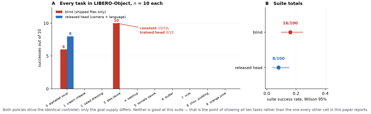
Figure 4: The whole suite, lookup against learning. All ten LIBERO-Object tasks, n=10 each, every trial recorded; both policies drive the identical controller and differ only in where the goal comes from. A The trained head wins task 0 (8 vs 6); the blind constant wins task 3 outright (10 vs 0), the task carrying the suite’s largest placement diameter; on the remaining eight both score zero. B Suite totals with Wilson intervals. Artifacts: results/suite_cells.json , results/blind_cells.json , results/pod_cells.json .
