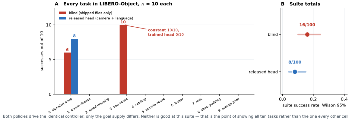
Figure 8: All ten LIBERO-Object tasks , n=10 each, every trial recorded; both policies drive the identical controller. Eight of ten tasks are 0–0. The suite totals in B are shown with i.i.d. Wilson intervals, which are too narrow here by a design effect of 8.4 (§6); they are drawn as reported rather than as believed. Artifacts: results/suite_cells.json , results/suite_inference.json .
