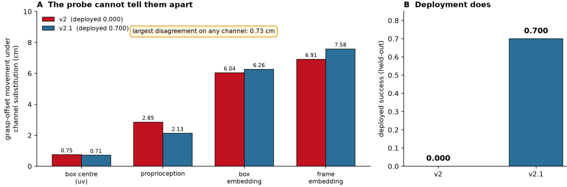
Figure 7: The counterexample to probe-only certification, promoted out of a text box inside Figure 6. A substitution attribution for v2 and v2.1 — same recipe, same 10-episode corpus — which agree to within 0.73 cm on every channel. B the same two heads deployed. A probe run on teacher trajectories is an on-manifold instrument; these two are indistinguishable to it and opposite in the world. Protocol, stated because it matters: the profile substitutes one channel between the two most-separated recorded ticks and reports how far the predicted grasp offset moves — the offset, not the absolute point, because GraspPointHead emits \text{eef}_{xy} + \Delta and substituting proprioception moves the absolute point by the whole arm displacement for any head, which would report \sim 24 cm of “proprioception attribution” even for the repaired one. Regenerated numbers do not reproduce the magnitudes printed in Figure 6, whose generator was never saved; the qualitative claims survive and the earlier magnitudes should not be relied on.
