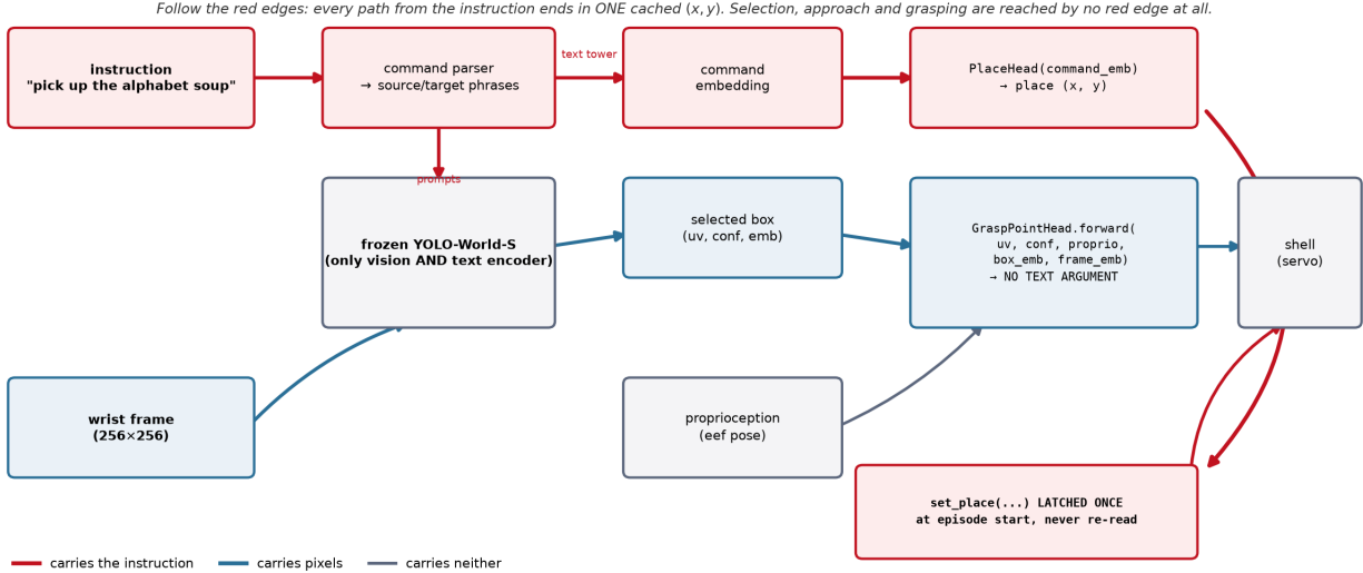
Figure 9: The deployed dataflow, with every edge coloured by what it carries. The architectural half of this section’s argument is a code fact and is drawn here rather than described: GraspPointHead.forward takes (uv, conf, proprio, box\_emb, frame\_emb) and no text argument , so no red edge reaches object selection, approach or grasping. Every red edge terminates in one (x, y) latched once by set_place(place_head(command_emb)) inside MicroVLAPolicy.reset() and never re-read — which also answers whether re-latching mid-episode could change the swap result: there is no re-latch.
