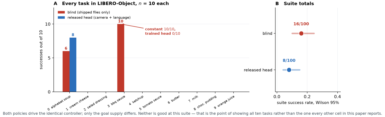
Figure 8: All ten LIBERO-Object tasks , n=10 each, every trial recorded; both policies drive the identical controller. Eight of ten tasks are 0–0. The suite totals in B are shown with i.i.d. Wilson intervals, which are too narrow here by a design effect of 8.4 (§6); they are drawn as reported rather than as believed. Artifacts: results/suite_cells.json , results/suite_inference.json .
