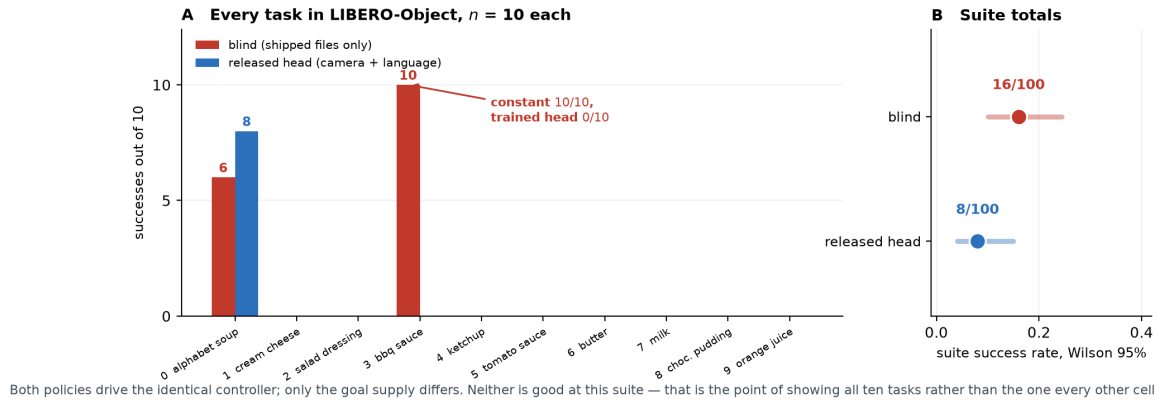
Figure 4: All ten LIBERO-Object tasks , n=10 each, every trial recorded; both policies drive the identical controller. Eight of ten tasks are 0–0. The suite totals in B are shown with i.i.d. Wilson intervals, which are too narrow here by a design effect of 8.4 (§5); they are drawn as reported rather than as believed. Artifacts: results/suite_cells.json , results/suite_inference.json .
