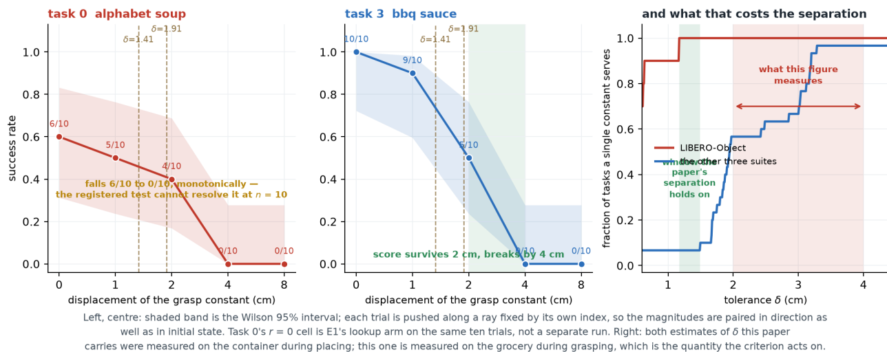
Figure 10: Displace the lookup arm's grasp constant by r and see what the score does. The displacement direction is drawn from default_rng(555000 + trial_seed) , so it is fixed by the trial index: each trial is pushed along its own ray at every magnitude, and the sweep is paired in direction as well as in initial state. Generated by paper/render_fig16-jitter.py from results/e23_analysis.json .
