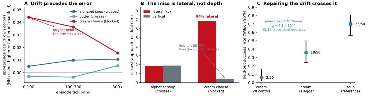
Figure 2: How the third object crossed. (A) Appearance drift by episode tick: the blocked object’s deployment embeddings sit furthest from its own training corpus at the start , before the arm has acted on any prediction, and the gap shrinks 65% — the opposite of the rising trend the two crossing objects show, which is what a consequence of a bad goal looks like. This is the circularity check that retired two earlier instruments. (B) The miss decomposed: 94% lateral, with the blocked object’s height better than the crossing object’s, which rules out a descent failure. (C) The intervention, n=50 per arm on identical seeds, Wilson 95% intervals: fine-tuning the grasp head on the machine’s own viewpoints takes the blocked object from 3/50 to 18/50 (paired exact McNemar p=6.1 \times 10^{-5} , 15/15 discordant one-way), against the crossing object’s 35/50 for reference.
