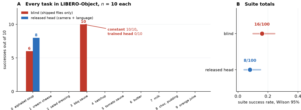
Figure 4: The whole suite, lookup against learning. All ten LIBERO-Object tasks, n=10 each, every trial recorded; both policies drive the identical controller and differ only in where the goal comes from. A The trained head wins task 0 (8 vs 6); the blind constant wins task 3 outright (10 vs 0), the task carrying the suite’s largest placement diameter; on the remaining eight both score zero. B Suite totals with Wilson intervals. Artifacts: results/suite_cells.json , results/blind_cells.json , results/pod_cells.json .
