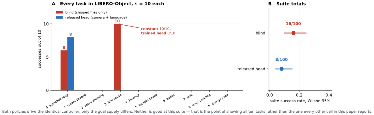
Figure 3: All ten LIBERO-Object tasks , n=10 each, every trial recorded; both policies drive the identical controller. Eight of ten tasks are 0–0. The suite totals in B are shown with i.i.d. Wilson intervals, which are too narrow here by a design effect of 8.4 (§5); they are drawn as reported rather than as believed. Artifacts: results/suite_cells.json , results/suite_inference.json .
