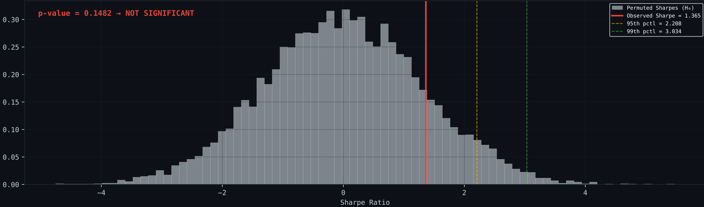
Monte Carlo Permutation Test (10,000 simulations)
