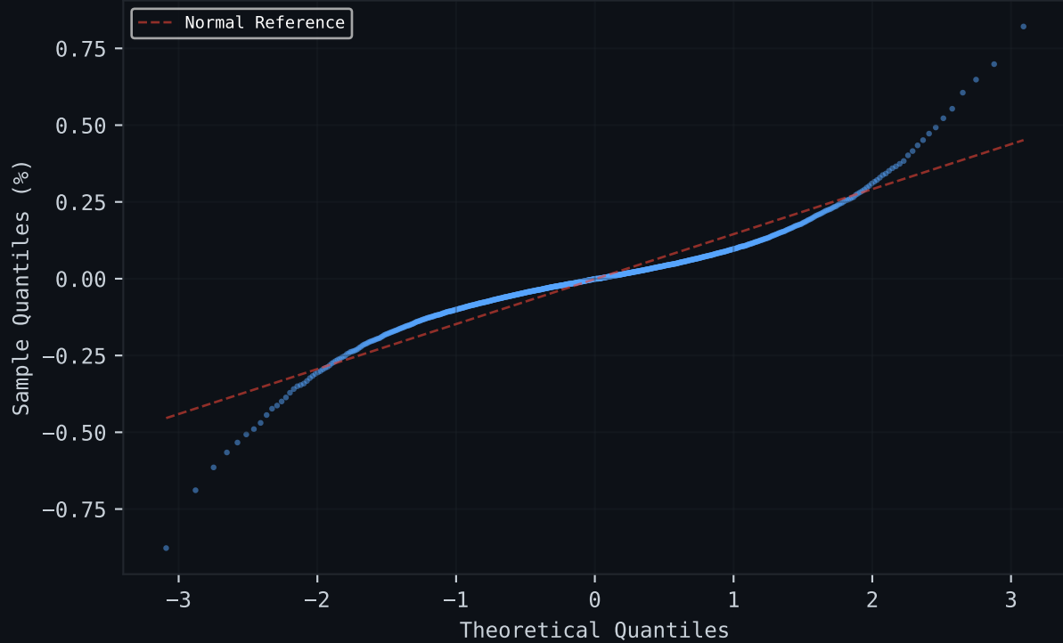
Q-Q Plot (Fat Tail Detection)
