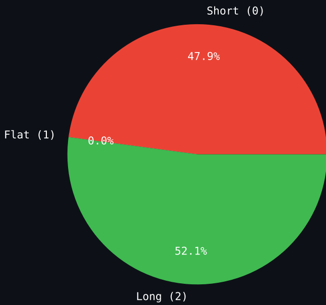
Action Distribution
