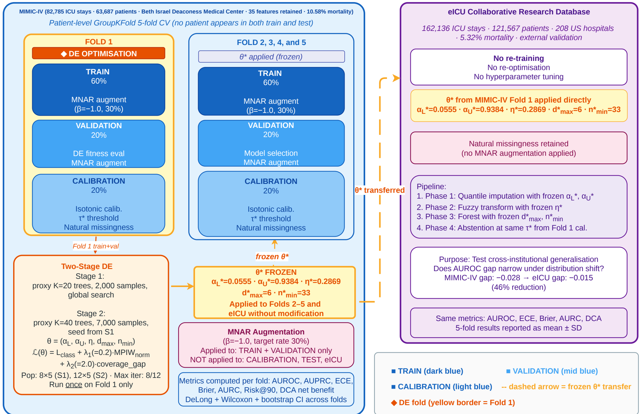
Figure 3 — JUCO Evaluation Protocol
