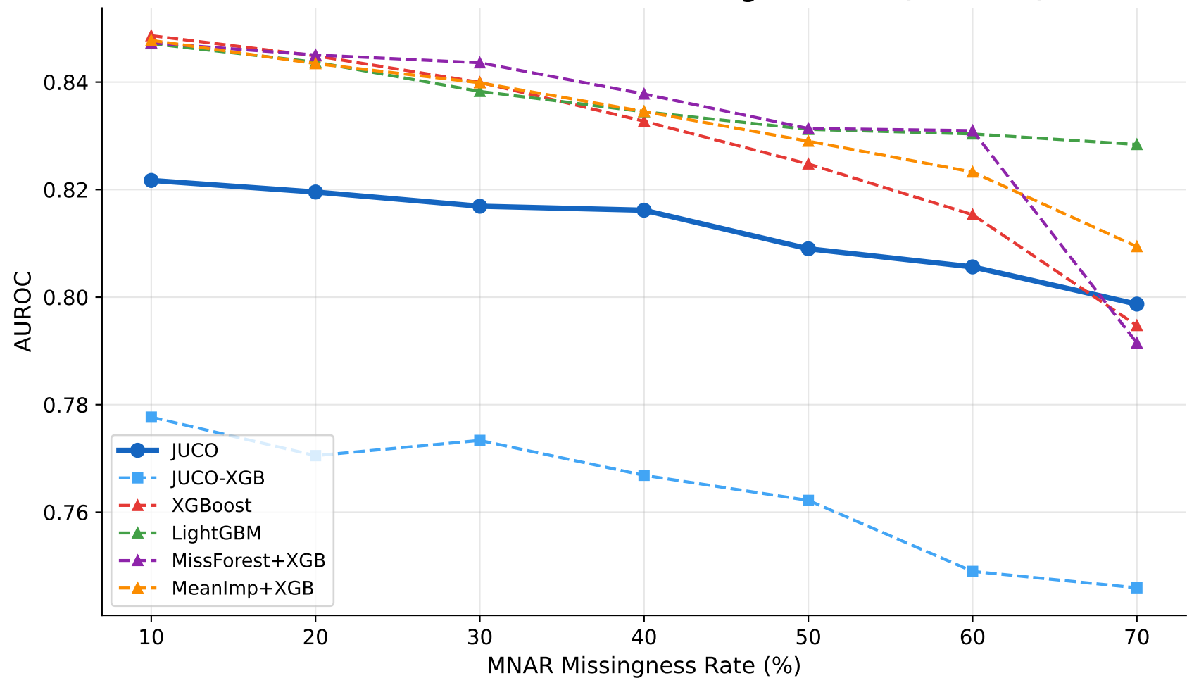
Robustness: AUROC vs MNAR Missingness Rate (MIMIC-IV)
