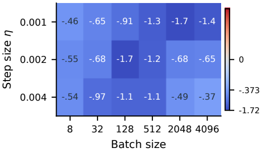
(c) ResNet-32 (no BN) \hat{\Lambda}
