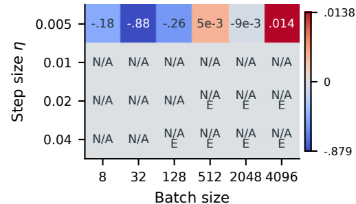
(c) ReLU MLP: 2 \times 512 \hat{\Lambda}
