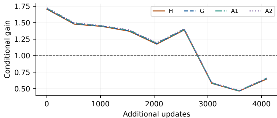
(e) Fixed-axis gain ladder
