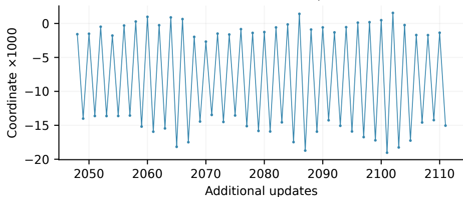
(f) Batch-gradient gain ladder
