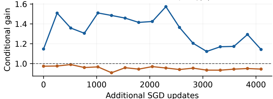
(e2) Geometric G = \exp(|\log|a|)
