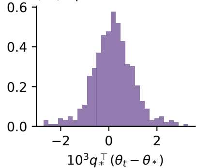
(c4) Updates 3072-3583
