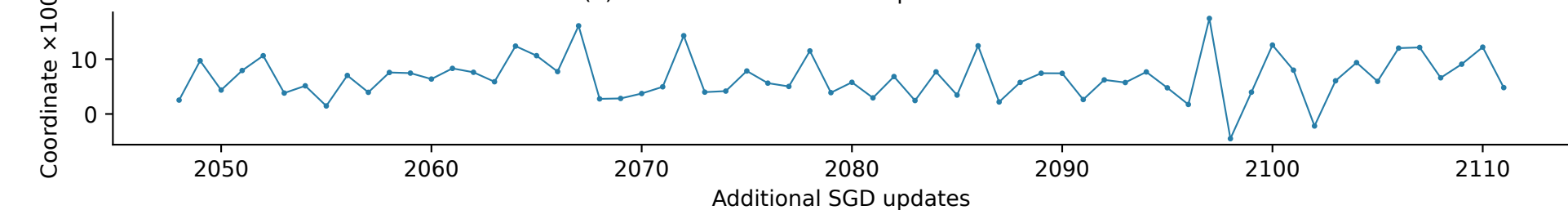
(e1) Harmonic H = 1/(\|a\|^{-1})
