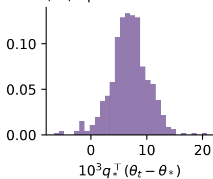
(c4) Updates 3072-3583
