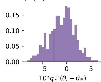
(c4) Updates 3072-3583
