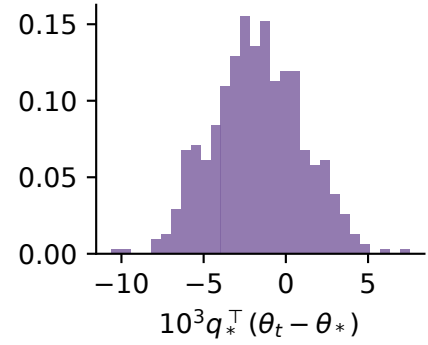
(c4) Updates 3072-3583
