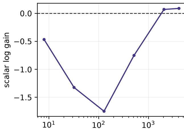
\eta = 0.05
