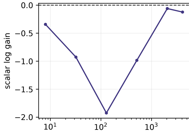
\eta = 0.025
