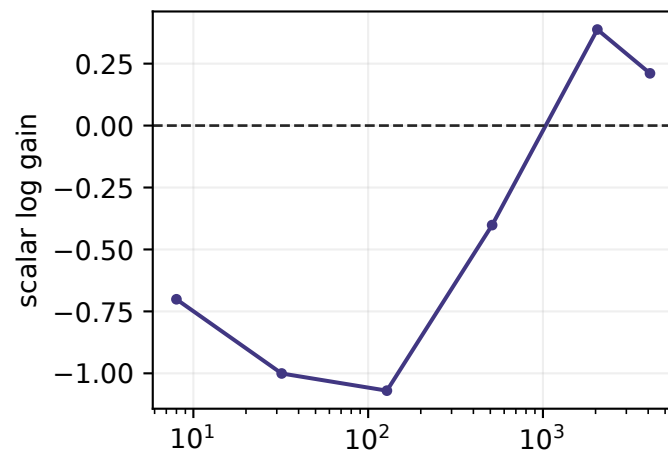
\eta = 0.1
