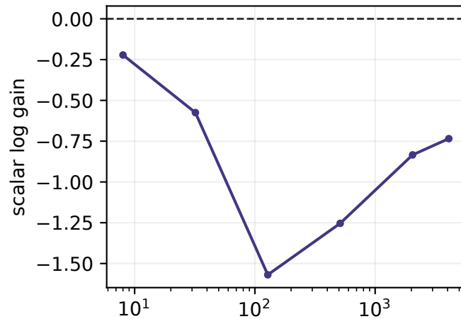
\eta = 0.002
