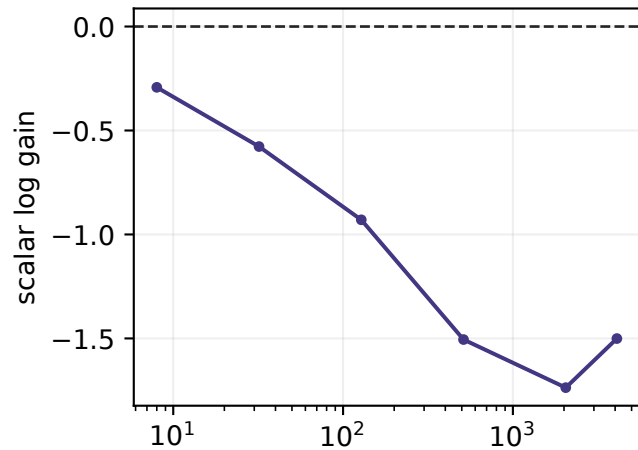
\eta = 0.001
