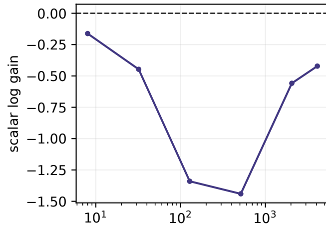
\eta = 0.004
