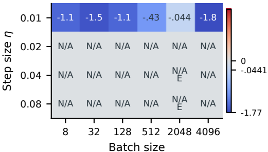
(c) ReLU MLP: 4 \times 512 \hat{\Lambda}
