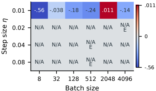
(c) ReLU MLP: 4 \times 512 \hat{\Lambda}
