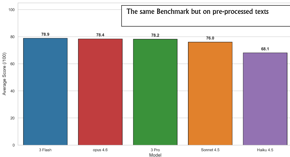
AVERAGE GLOBAL SCORE (Out of 100)
