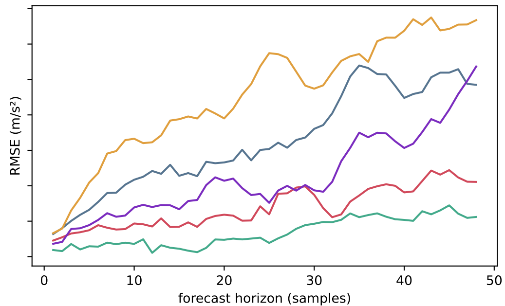
Held-out station 4
