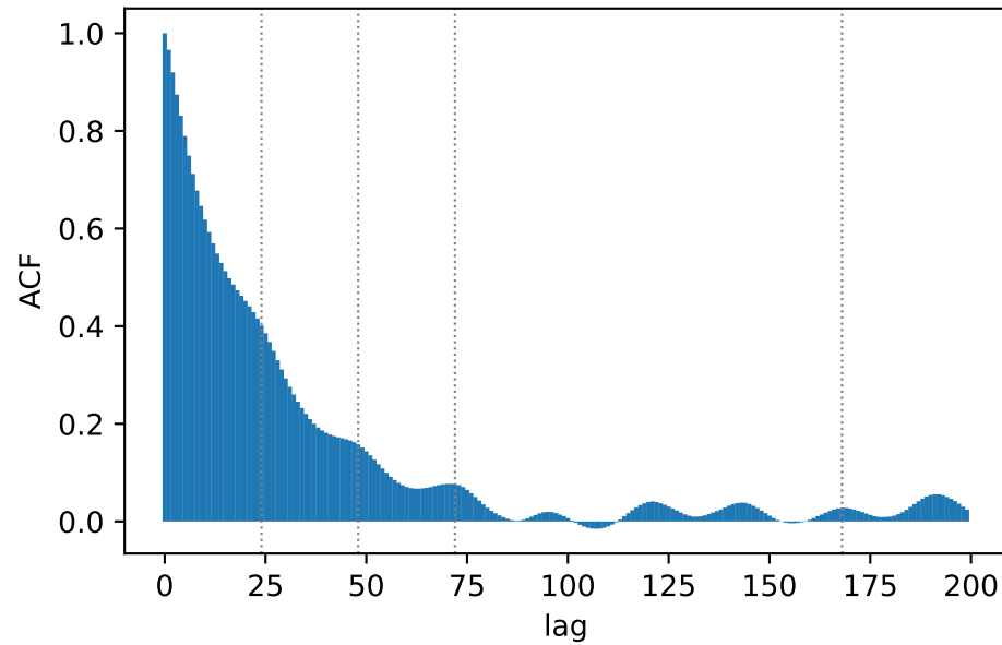
Autocorrelation (lags 0-199)
