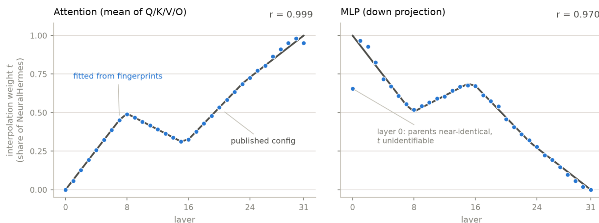
Figure 1 — Reading a merge recipe back out of fingerprints. Each dot is the sum-to-one least-squares weight of one parent (NeuralHermes) fitted on that layer’s fingerprint samples; the line is the interpolation curve the merge’s author published. Regenerate with python paper/make_figures.py .
