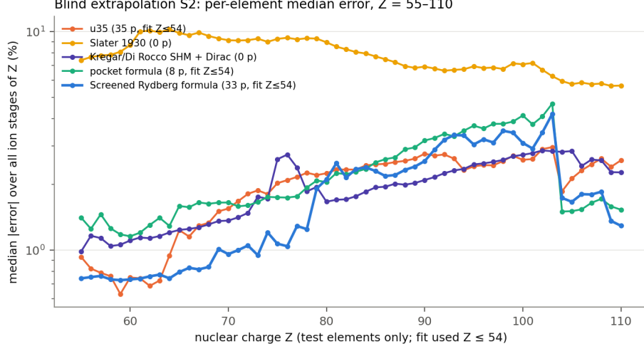
FIG. 1. Blind extrapolation. Each point is the median absolute percentage error over all ion stages of one element Z = 55\text{--}110 . The three fitted models are fitted on Z \leq 54 only; Slater’s rules and the Kregar/Di Rocco SHM have no fitted parameters. The S2 MAPEs, computed from refits with the project’s validation code, reproduce Table I (final 6.603 %, linear-remainder model 57.233 %, pocket 11.334 %, Slater 11.638 %).
