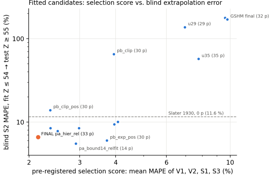
FIG. 2. Selection score (mean of V1, V2, S1, S3; no S2 data, although S1 and S3 contain Z \geq 55 rows) against blind S2 MAPE for every fitted candidate. The pocket formula is omitted because its V1 fit diverged in the frozen run; that divergence depends on the optimizer path (Sec. III D), and with the converged V1 its selection score would be 4.19. The dashed line is Slater’s rules (0 parameters).
