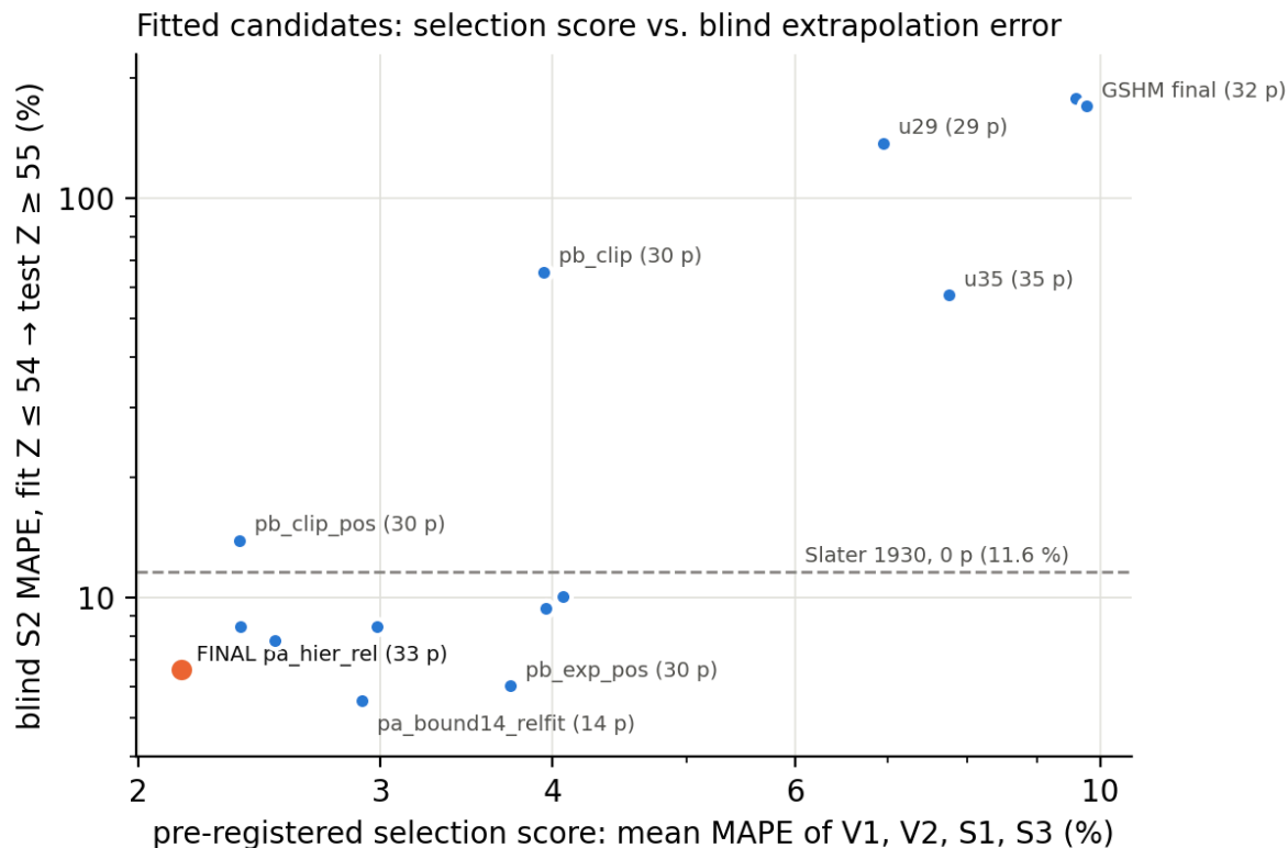
Figure 2. Selection score (mean of V1, V2, S1, S3; no S2 data, although S1 and S3 contain Z \geq 55 rows) against blind S2 MAPE for every fitted candidate. The pocket formula is omitted because its V1 fit diverged in the frozen run; that
