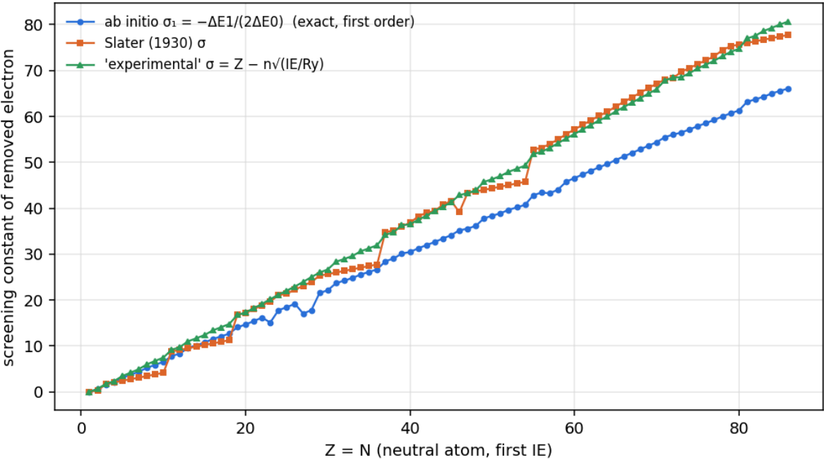
Figure 3. Exact first-order screening \sigma_1 against Slater's \sigma for neutral-atom configurations.
