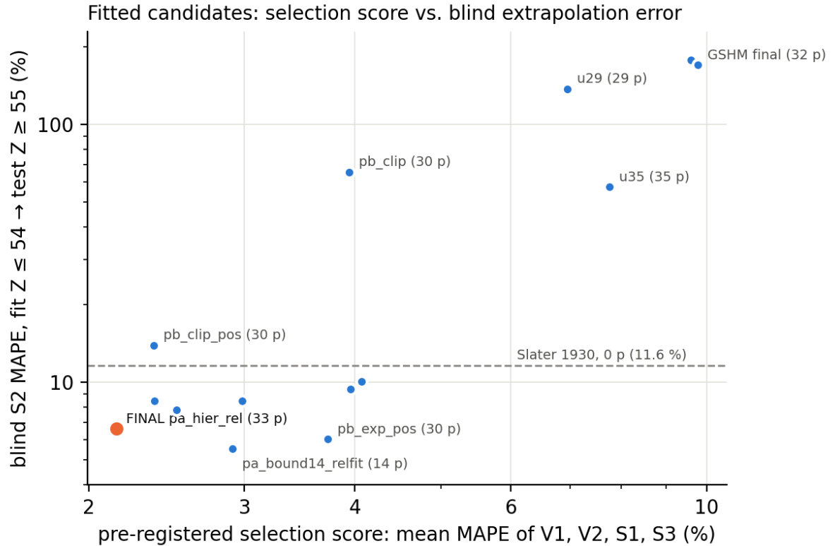
FIG. 2. Selection score (mean of V1, V2, S1, S3; no S2 data, although S1 and S3 contain Z \geq 55 rows) against blind S2 MAPE for every fitted candidate. The pocket formula is omitted because its V1 fit diverged in the frozen run; that divergence depends on the optimizer path (Sec. III D), and with the converged V1 its selection score would be 4.19. The dashed line is Slater's rules (0 parameters).
