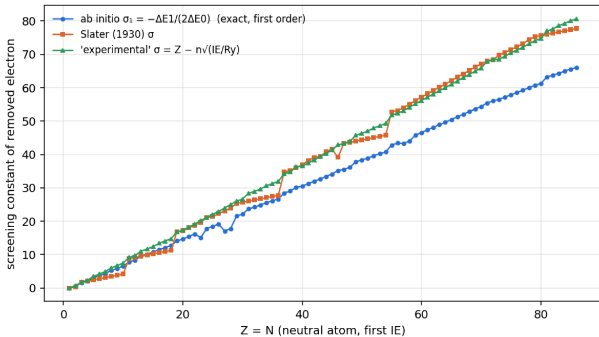
FIG. 3. Exact first-order screening \sigma_1 against Slater's \sigma for neutral-atom configurations.
