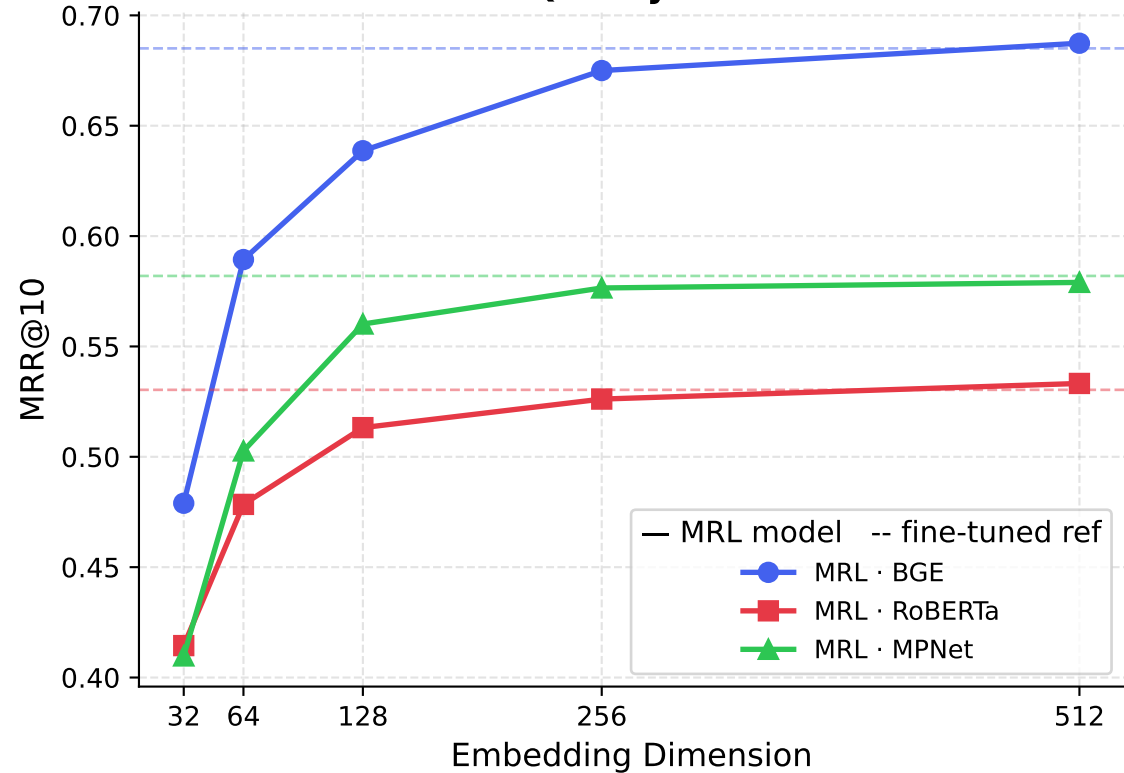
MRL: Retrieval Quality vs Truncation Dim
