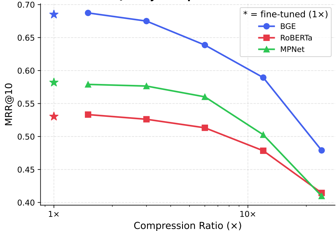
MRL: Quality-Compression Trade-off
