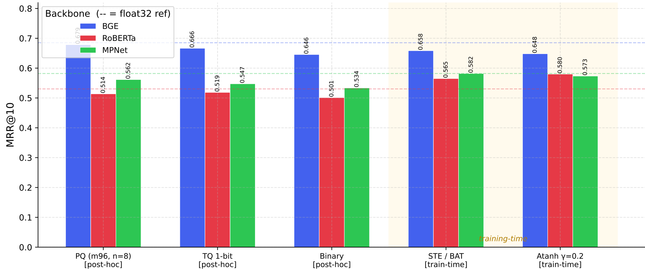
Training-Time vs Post-Hoc Compression at 32× (96 bytes)
