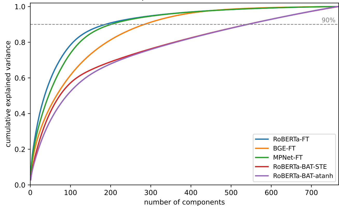
Cumulative explained variance across backbones
