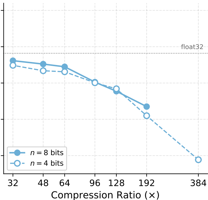
MPNet
