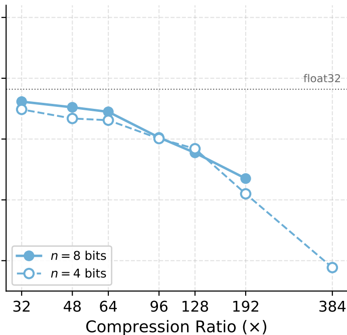
MPNet
