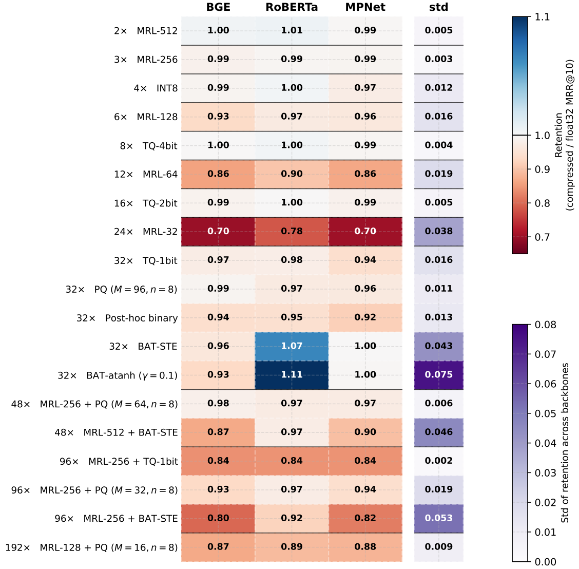
Figure 7: Quality retention (compressed MRR@10 divided by the same backbone’s float32 MRR@10) by configuration. The rightmost column shows the cross-backbone standard deviation.
