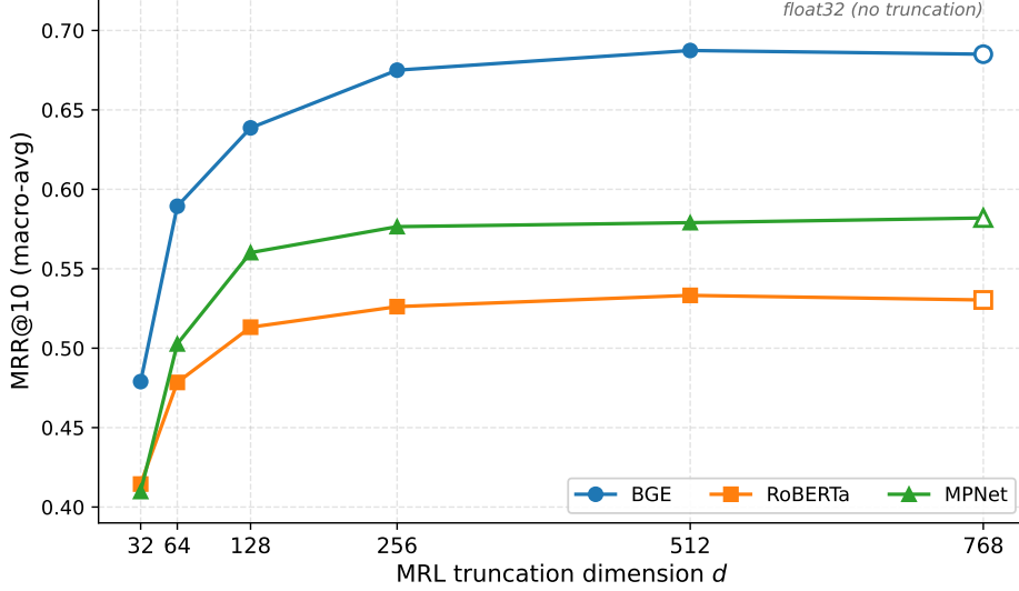
Figure 4: Mean MRR@10 vs MRL truncation dimension d . The point at d = 768 is the float32 baseline.
