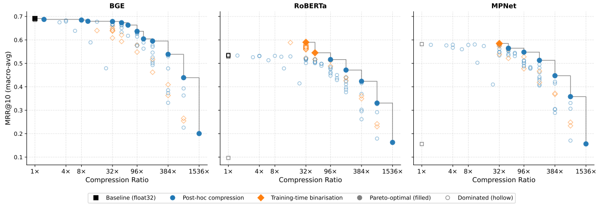
Figure 6: Quality vs compression Pareto frontiers for BGE, RoBERTa, and MPNet ( x -axis log scale). Filled markers are Pareto-optimal; hollow markers are dominated. Colour encodes method family.
