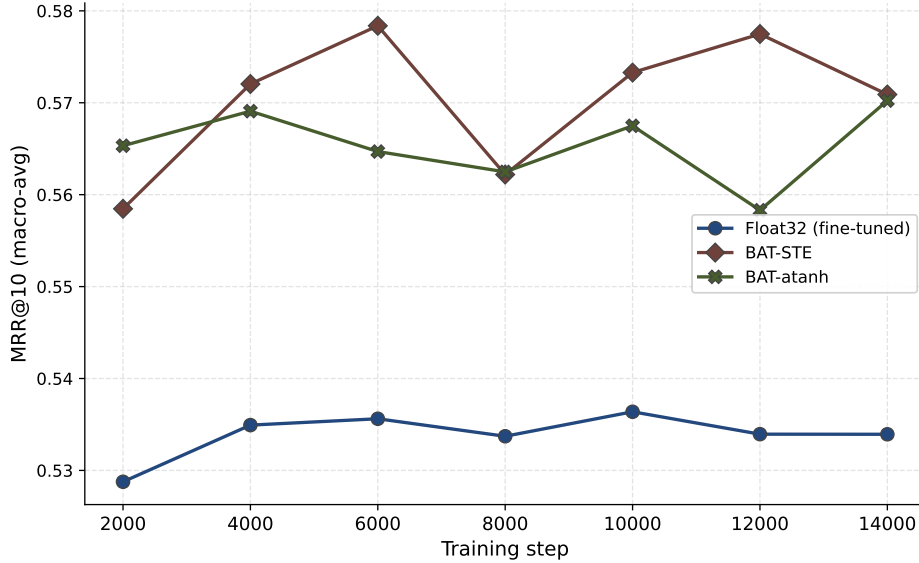
Figure 3: Mean MRR@10 at intermediate RoBERTa checkpoints. The gap from BAT to the float32 fine-tune is present early and does not close with training.
