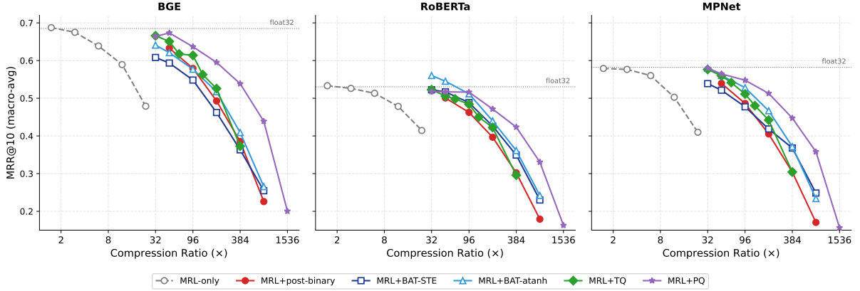
Figure 5: Mean MRR@10 vs compression ratio for the five stacked combinations and MRL-only (grey dashed). Hollow markers are pure training-time stacks; filled markers are hybrid stacks. The dotted line is the float32 baseline.
