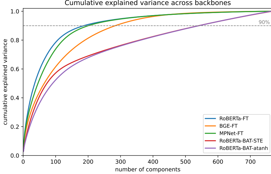
Figure 2: Cumulative explained variance vs number of principal components. A curve that rises quickly indicates a low effective dimension. RoBERTa-FT rises fastest; RoBERTa-BAT-atanh rises slowest.
