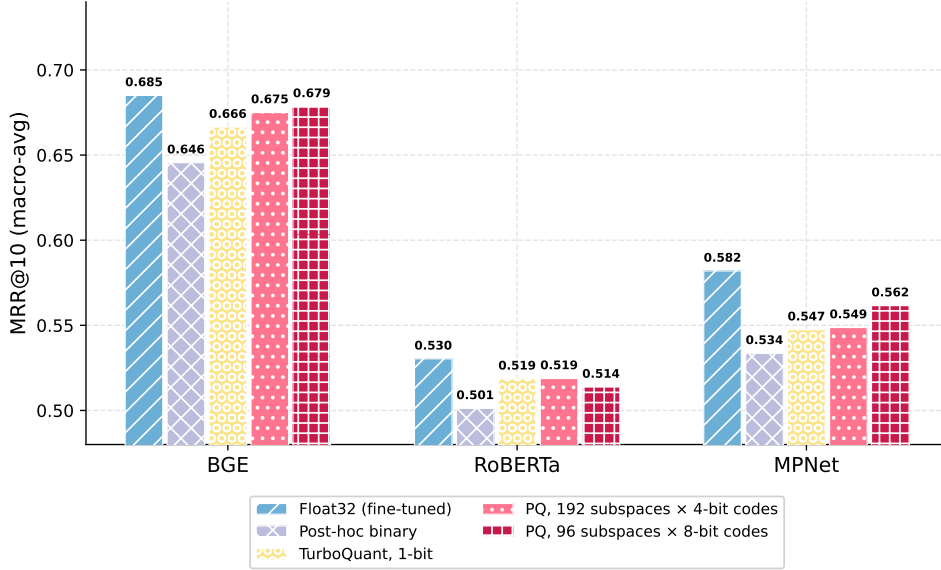
Figure 1: Post-hoc methods at 32\times , mean MRR@10 by backbone. The y -axis starts at 0.48 to highlight inter-method differences.
