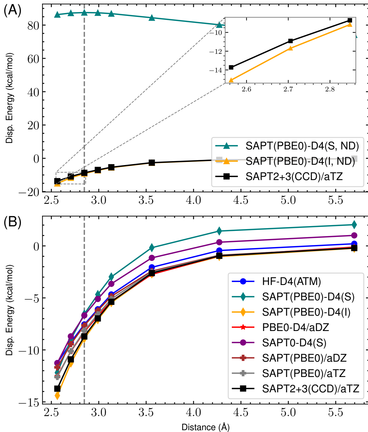
Figure 3: s66x8 41_Uracil-Pentane : Dispersion potential Energy curve for SAPT(PBE0) with aDZ/aTZ and -D4 variants versus the reference SAPT2+3(CCD)/aug-cc-pVTZ dispersion energy. (A) highlights the completely non-damped (ND) D4 curves compared to the reference for both supermolecular (S) and intermolecular (I). The remaining s_8 = 0.89529649 . (B) shows the damped -D4(S), -D4(I), HF-D4, SAPT(PBE0)/aDZ, SAPT(PBE0)/aTZ, and reference dispersion energies. Here, (S) and (I) refer to the supermolecular and intermolecular dispersion energy approaches, respectively. The “ND” states that no damping function is used. For the damped SAPT(PBE0)-D4(S) and SAPT(PBE0)-D4(I) terms, a_1 , a_2 , and s_8 are fit to the residual CCSD(T)/CBS energies on the 4470 dimer dataset.
