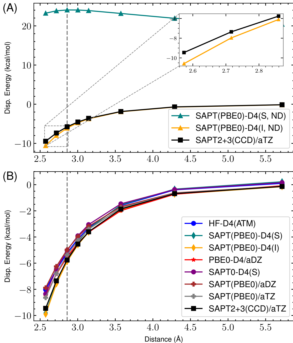
Figure 39: s66x8 63_Benzene-AcOH : Dispersion potential Energy curve for SAPT(PBE0) with aDZ/aTZ and -D4 variants versus the reference SAPT2+3(CCD)/aug-cc-pVTZ dispersion energy. (A) highlights the completely non-damped (ND) D4 curves compared to the reference for both supermolecular (S) and intermolecular (I). The remaining s_8 = 0.89529649 . (B) shows the damped -D4(S), -D4(I), HF-D4, SAPT(PBE0)/aDZ, SAPT(PBE0)/aTZ, and reference dispersion energies. Here, (S) and (I) refer to the supermolecular and intermolecular dispersion energy approaches, respectively. The “ND” states that no damping function is used. For the damped SAPT(PBE0)-D4(S) and SAPT(PBE0)-D4(I) terms, a_1 , a_2 , and s_8 are fit to the residual CCSD(T)/CBS energies on the 4470 dimer dataset.
