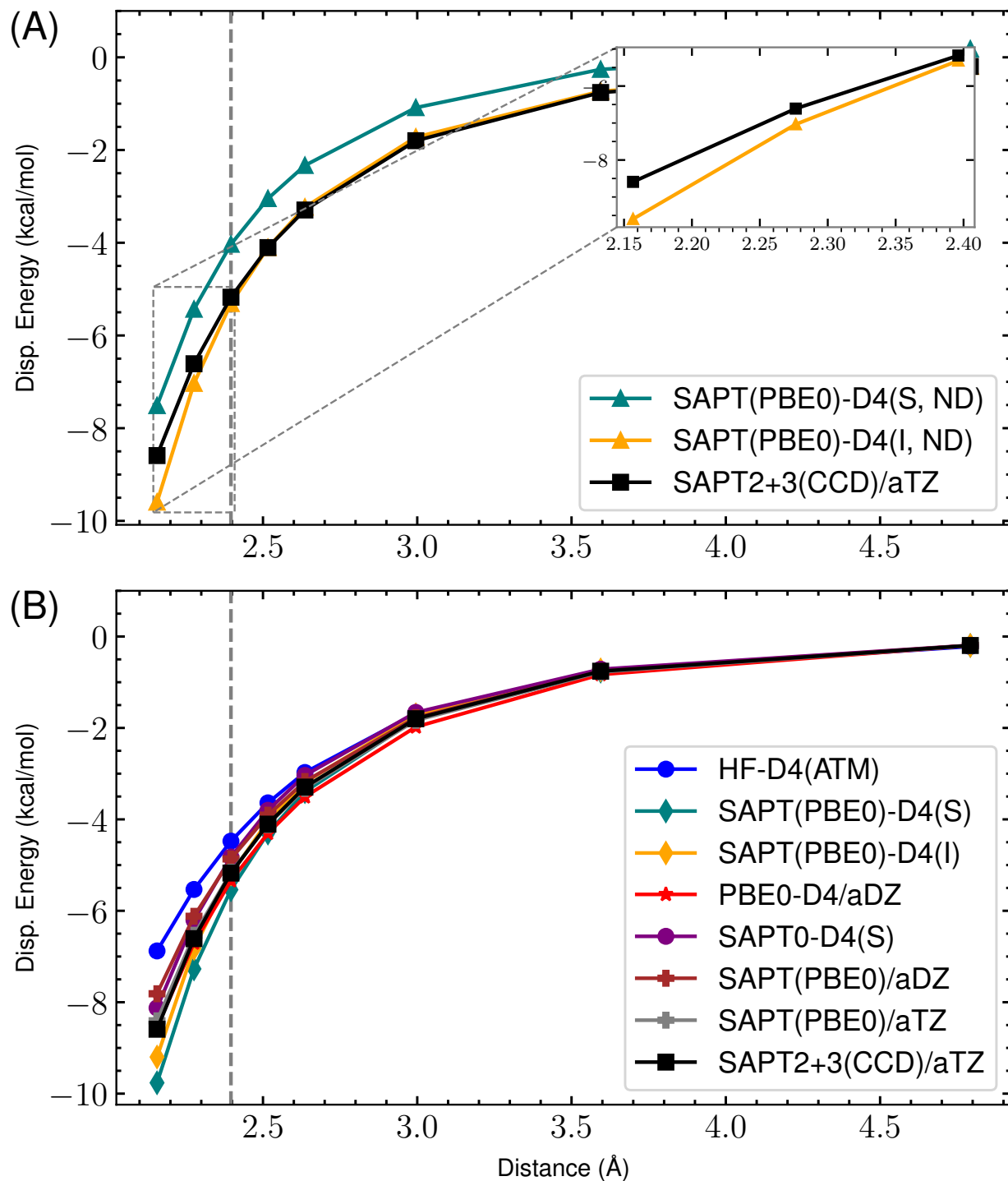
Figure 63: s66x8 37_Cyclopentane-Neopentane : Dispersion potential Energy curve for SAPT(PBE0) with aDZ/aTZ and -D4 variants versus the reference SAPT2+3(CCD)/aug-cc-pVTZ dispersion energy. (A) highlights the completely non-damped (ND) D4 curves compared to the reference for both supermolecular (S) and intermolecular (I). The remaining s_8 = 0.89529649 . (B) shows the damped -D4(S), -D4(I), HF-D4, SAPT(PBE0)/aDZ, SAPT(PBE0)/aTZ, and reference dispersion energies. Here, (S) and (I) refer to the supermolecular and intermolecular dispersion energy approaches, respectively. The “ND” states that no damping function is used. For the damped SAPT(PBE0)-D4(S) and SAPT(PBE0)-D4(I) terms, a_1 , a_2 , and s_8 are fit to the residual CCSD(T)/CBS energies on the 4470 dimer dataset.
