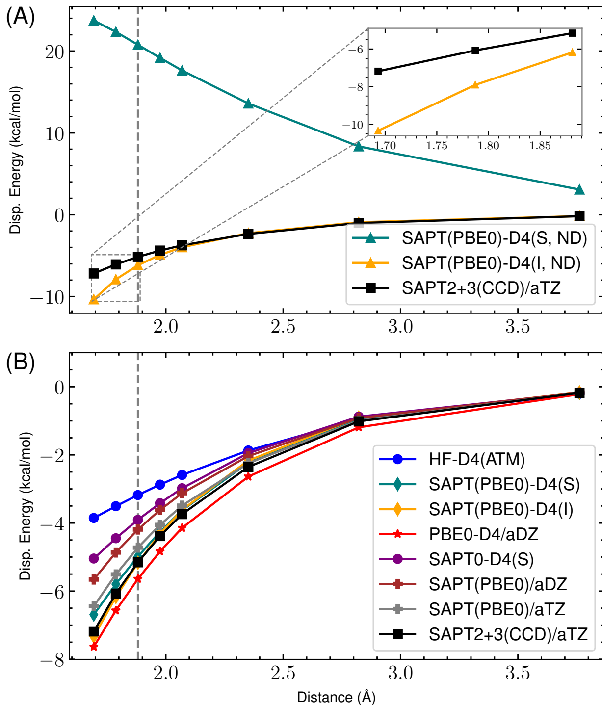
Figure 32: s66x8 07_MeOH-Peptide : Dispersion potential Energy curve for SAPT(PBE0) with aDZ/aTZ and -D4 variants versus the reference SAPT2+3(CCD)/aug-cc-pVTZ dispersion energy. (A) highlights the completely non-damped (ND) D4 curves compared to the reference for both supermolecular (S) and intermolecular (I). The remaining s_8 = 0.89529649 . (B) shows the damped -D4(S), -D4(I), HF-D4, SAPT(PBE0)/aDZ, SAPT(PBE0)/aTZ, and reference dispersion energies. Here, (S) and (I) refer to the supermolecular and intermolecular dispersion energy approaches, respectively. The “ND” states that no damping function is used. For the damped SAPT(PBE0)-D4(S) and SAPT(PBE0)-D4(I) terms, a_1 , a_2 , and s_8 are fit to the residual CCSD(T)/CBS energies on the 4470 dimer dataset.
