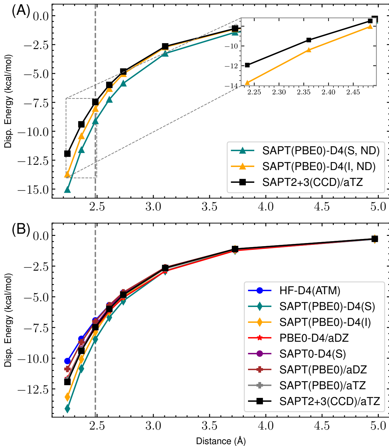
Figure 40: s66x8 34. Pentane-Pentane : Dispersion potential Energy curve for SAPT(PBE0) with aDZ/aTZ and -D4 variants versus the reference SAPT2+3(CCD)/aug-cc-pVTZ dispersion energy. (A) highlights the completely non-damped (ND) D4 curves compared to the reference for both supermolecular (S) and intermolecular (I). The remaining s_8 = 0.89529649 . (B) shows the damped -D4(S), -D4(I), HF-D4, SAPT(PBE0)/aDZ, SAPT(PBE0)/aTZ, and reference dispersion energies. Here, (S) and (I) refer to the supermolecular and intermolecular dispersion energy approaches, respectively. The “ND” states that no damping function is used. For the damped SAPT(PBE0)-D4(S) and SAPT(PBE0)-D4(I) terms, a_1 , a_2 , and s_8 are fit to the residual CCSD(T)/CBS energies on the 4470 dimer dataset.
