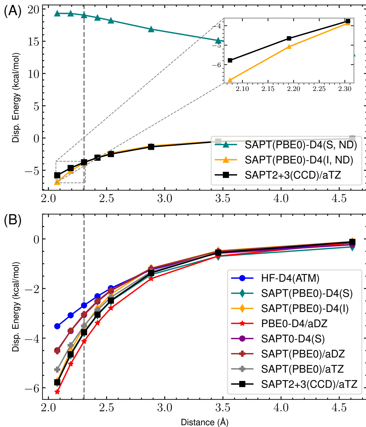
Figure 58: s66x8 60_Ethyne-AcOH : Dispersion potential Energy curve for SAPT(PBE0) with aDZ/aTZ and -D4 variants versus the reference SAPT2+3(CCD)/aug-cc-pVTZ dispersion energy. (A) highlights the completely non-damped (ND) D4 curves compared to the reference for both supermolecular (S) and intermolecular (I). The remaining s_8 = 0.89529649 . (B) shows the damped -D4(S), -D4(I), HF-D4, SAPT(PBE0)/aDZ, SAPT(PBE0)/aTZ, and reference dispersion energies. Here, (S) and (I) refer to the supermolecular and intermolecular dispersion energy approaches, respectively. The “ND” states that no damping function is used. For the damped SAPT(PBE0)-D4(S) and SAPT(PBE0)-D4(I) terms, a_1 , a_2 , and s_8 are fit to the residual CCSD(T)/CBS energies on the 4470 dimer dataset.
