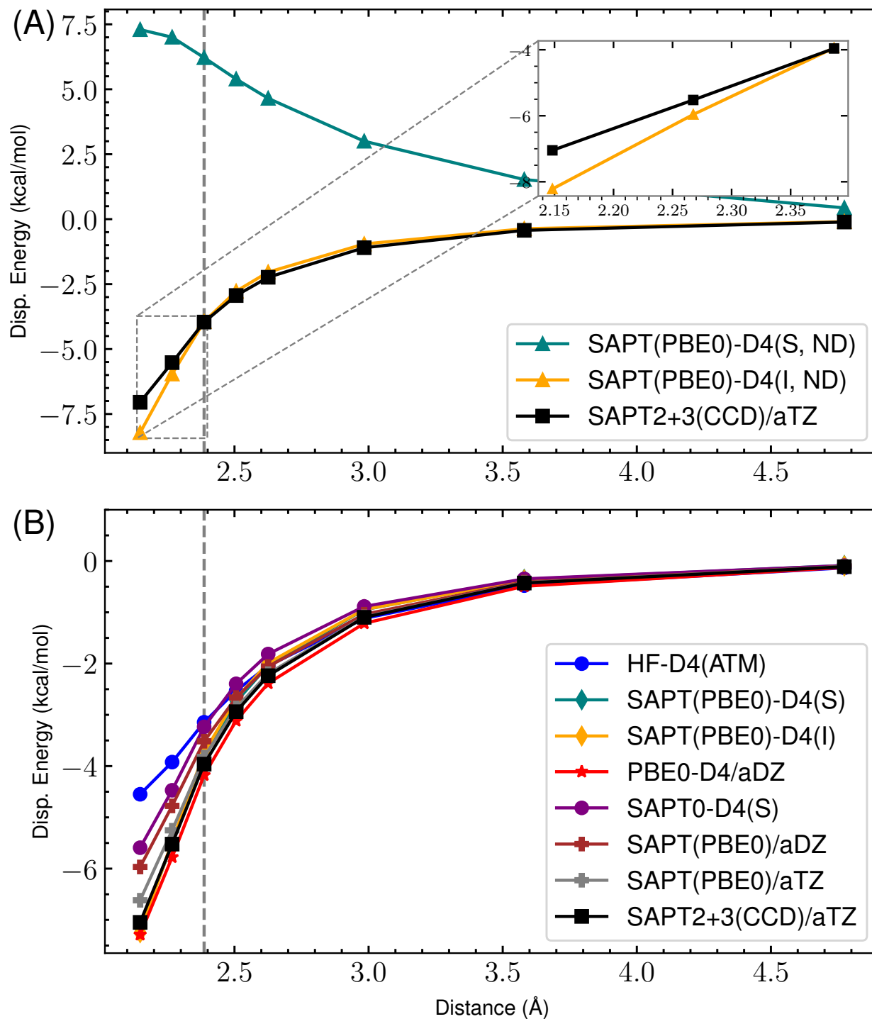
Figure 20: s66x8 58_Pyridine-Pyridine : Dispersion potential Energy curve for SAPT(PBE0) with aDZ/aTZ and -D4 variants versus the reference SAPT2+3(CCD)/aug-cc-pVTZ dispersion energy. (A) highlights the completely non-damped (ND) D4 curves compared to the reference for both supermolecular (S) and intermolecular (I). The remaining s_8 = 0.89529649 . (B) shows the damped -D4(S), -D4(I), HF-D4, SAPT(PBE0)/aDZ, SAPT(PBE0)/aTZ, and reference dispersion energies. Here, (S) and (I) refer to the supermolecular and intermolecular dispersion energy approaches, respectively. The “ND” states that no damping function is used. For the damped SAPT(PBE0)-D4(S) and SAPT(PBE0)-D4(I) terms, a_1 , a_2 , and s_8 are fit to the residual CCSD(T)/CBS energies on the 4470 dimer dataset.
