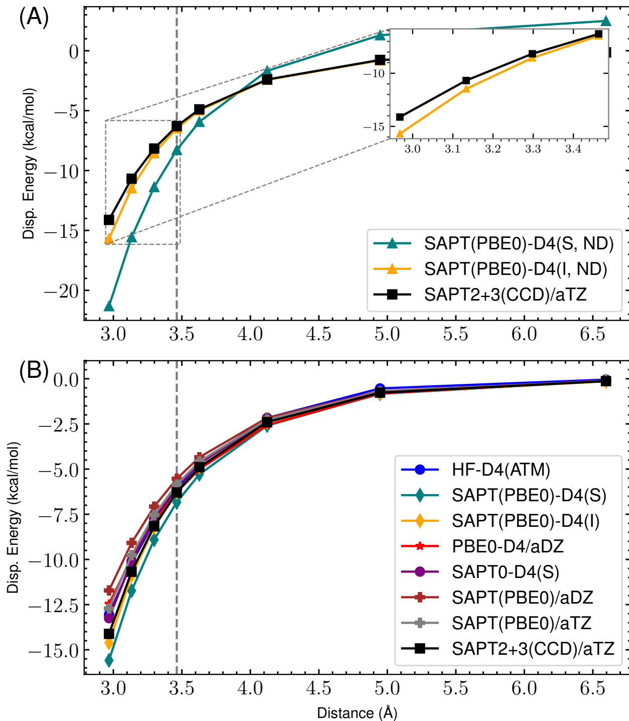
Figure 11: s66x8 27_Benzene-Pyridine : Dispersion potential Energy curve for SAPT(PBE0) with aDZ/aTZ and -D4 variants versus the reference SAPT2+3(CCD)/aug-cc-pVTZ dispersion energy. (A) highlights the completely non-damped (ND) D4 curves compared to the reference for both supermolecular (S) and intermolecular (I). The remaining s_8 = 0.89529649 . (B) shows the damped -D4(S), -D4(I), HF-D4, SAPT(PBE0)/aDZ, SAPT(PBE0)/aTZ, and reference dispersion energies. Here, (S) and (I) refer to the supermolecular and intermolecular dispersion energy approaches, respectively. The “ND” states that no damping function is used. For the damped SAPT(PBE0)-D4(S) and SAPT(PBE0)-D4(I) terms, a_1 , a_2 , and s_8 are fit to the residual CCSD(T)/CBS energies on the 4470 dimer dataset.
