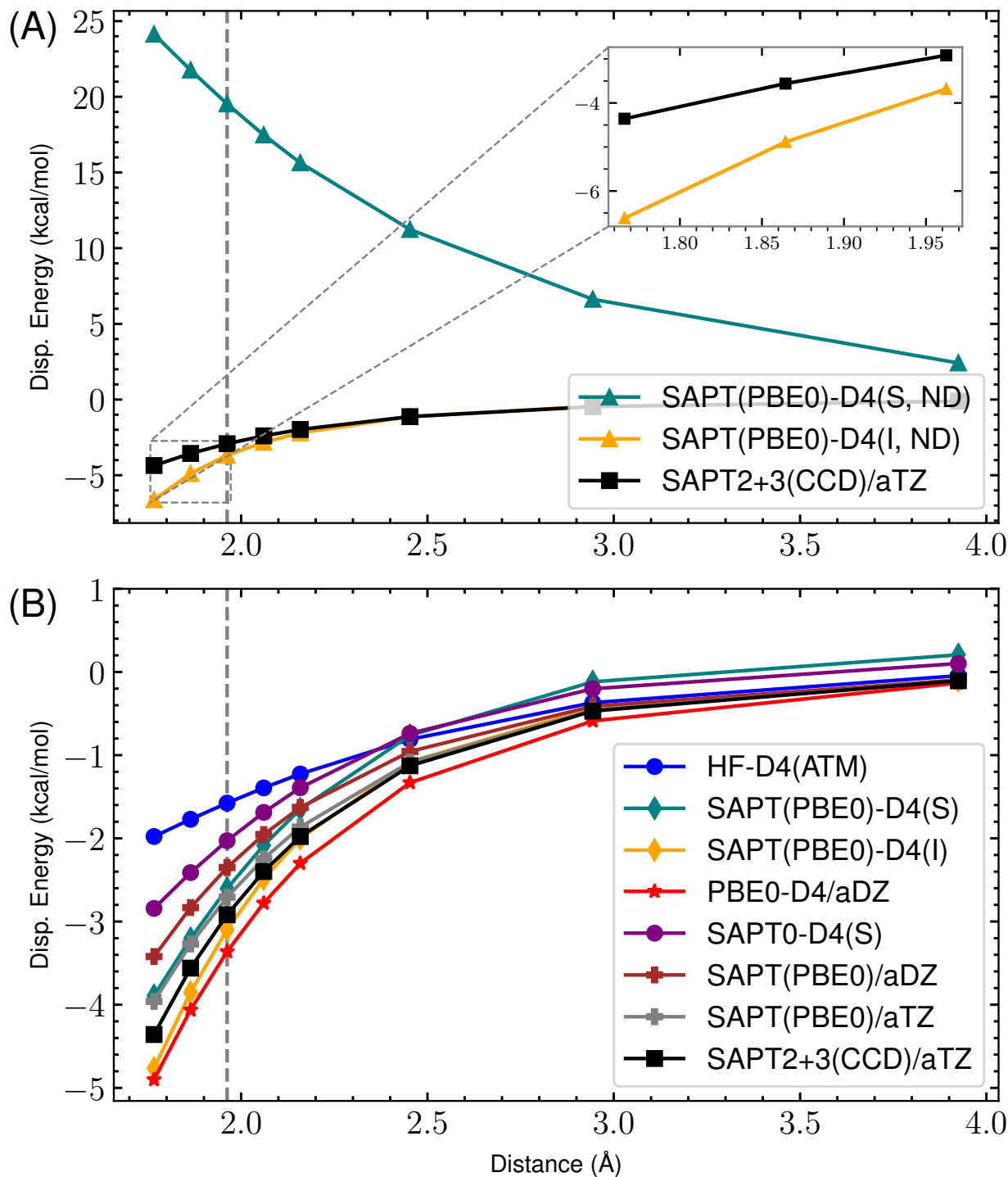
Figure 8: s66x8 02_Water-MeOH : Dispersion potential Energy curve for SAPT(PBE0) with aDZ/aTZ and -D4 variants versus the reference SAPT2+3(CCD)/aug-cc-pVTZ dispersion energy. (A) highlights the completely non-damped (ND) D4 curves compared to the reference for both supermolecular (S) and intermolecular (I). The remaining s_8 = 0.89529649 . (B) shows the damped -D4(S), -D4(I), HF-D4, SAPT(PBE0)/aDZ, SAPT(PBE0)/aTZ, and reference dispersion energies. Here, (S) and (I) refer to the supermolecular and intermolecular dispersion energy approaches, respectively. The “ND” states that no damping function is used. For the damped SAPT(PBE0)-D4(S) and SAPT(PBE0)-D4(I) terms, a_1 , a_2 , and s_8 are fit to the residual CCSD(T)/CBS energies on the 4470 dimer dataset.
