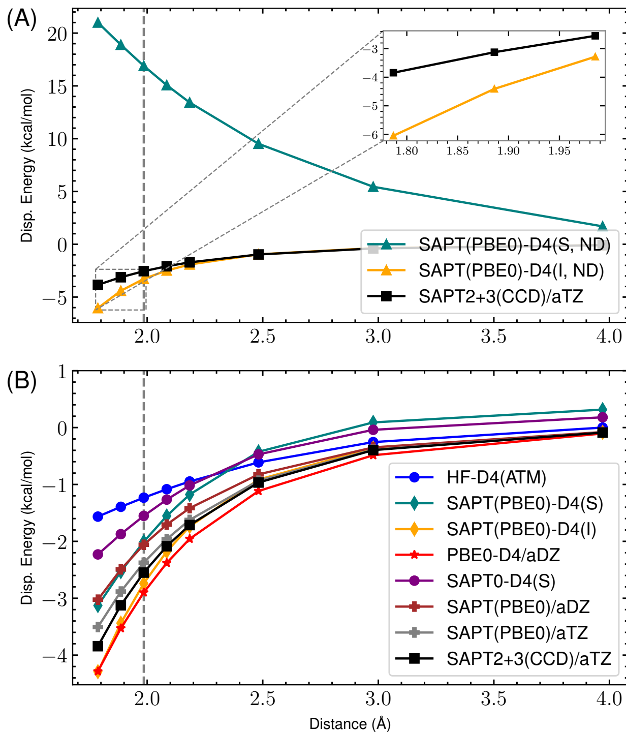
Figure 55: s66x8 08_MeOH-Water : Dispersion potential Energy curve for SAPT(PBE0) with aDZ/aTZ and -D4 variants versus the reference SAPT2+3(CCD)/aug-cc-pVTZ dispersion energy. (A) highlights the completely non-damped (ND) D4 curves compared to the reference for both supermolecular (S) and intermolecular (I). The remaining s_8 = 0.89529649 . (B) shows the damped -D4(S), -D4(I), HF-D4, SAPT(PBE0)/aDZ, SAPT(PBE0)/aTZ, and reference dispersion energies. Here, (S) and (I) refer to the supermolecular and intermolecular dispersion energy approaches, respectively. The “ND” states that no damping function is used. For the damped SAPT(PBE0)-D4(S) and SAPT(PBE0)-D4(I) terms, a_1 , a_2 , and s_8 are fit to the residual CCSD(T)/CBS energies on the 4470 dimer dataset.
