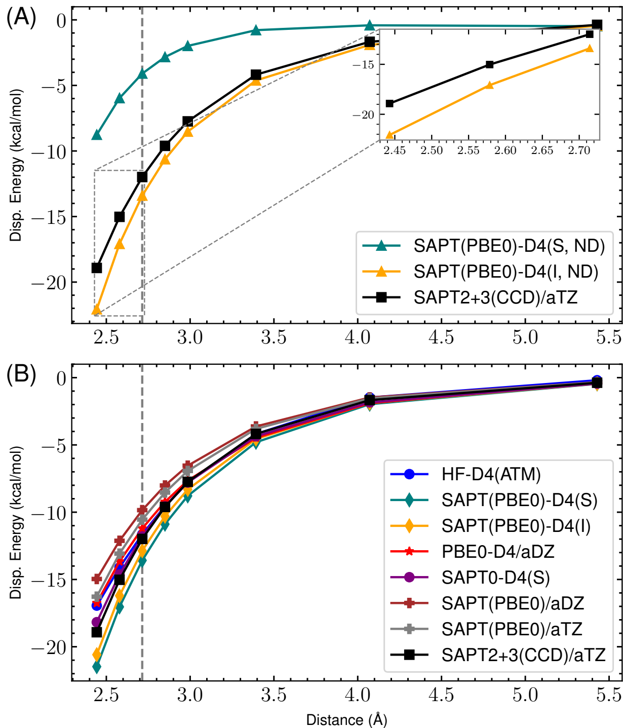
Figure 10: s66x8 26_Uracil-Uracil : Dispersion potential Energy curve for SAPT(PBE0) with aDZ/aTZ and -D4 variants versus the reference SAPT2+3(CCD)/aug-cc-pVTZ dispersion energy. (A) highlights the completely non-damped (ND) D4 curves compared to the reference for both supermolecular (S) and intermolecular (I). The remaining s_8 = 0.89529649 . (B) shows the damped -D4(S), -D4(I), HF-D4, SAPT(PBE0)/aDZ, SAPT(PBE0)/aTZ, and reference dispersion energies. Here, (S) and (I) refer to the supermolecular and intermolecular dispersion energy approaches, respectively. The “ND” states that no damping function is used. For the damped SAPT(PBE0)-D4(S) and SAPT(PBE0)-D4(I) terms, a_1 , a_2 , and s_8 are fit to the residual CCSD(T)/CBS energies on the 4470 dimer dataset.
