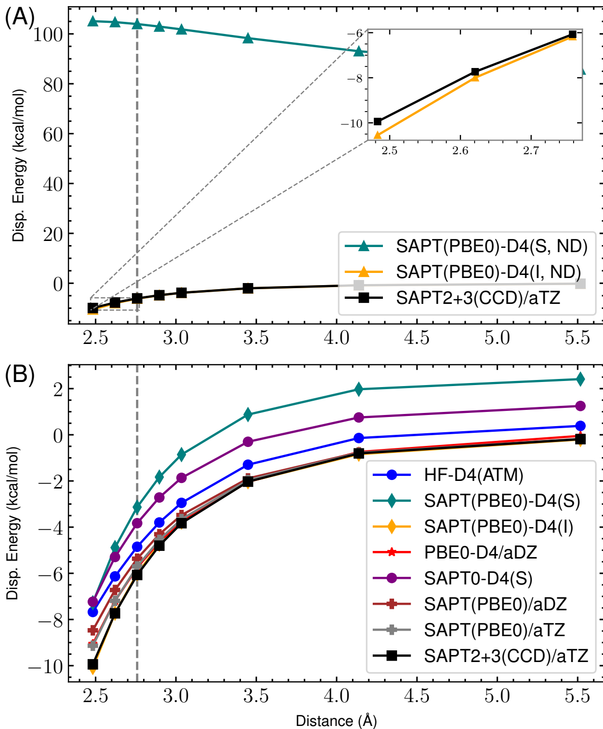
Figure 53: s66x8 43_Uracil-Neopentane : Dispersion potential Energy curve for SAPT(PBE0) with aDZ/aTZ and -D4 variants versus the reference SAPT2+3(CCD)/aug-cc-pVTZ dispersion energy. (A) highlights the completely non-damped (ND) D4 curves compared to the reference for both supermolecular (S) and intermolecular (I). The remaining s_8 = 0.89529649 . (B) shows the damped -D4(S), -D4(I), HF-D4, SAPT(PBE0)/aDZ, SAPT(PBE0)/aTZ, and reference dispersion energies. Here, (S) and (I) refer to the supermolecular and intermolecular dispersion energy approaches, respectively. The “ND” states that no damping function is used. For the damped SAPT(PBE0)-D4(S) and SAPT(PBE0)-D4(I) terms, a_1 , a_2 , and s_8 are fit to the residual CCSD(T)/CBS energies on the 4470 dimer dataset.
