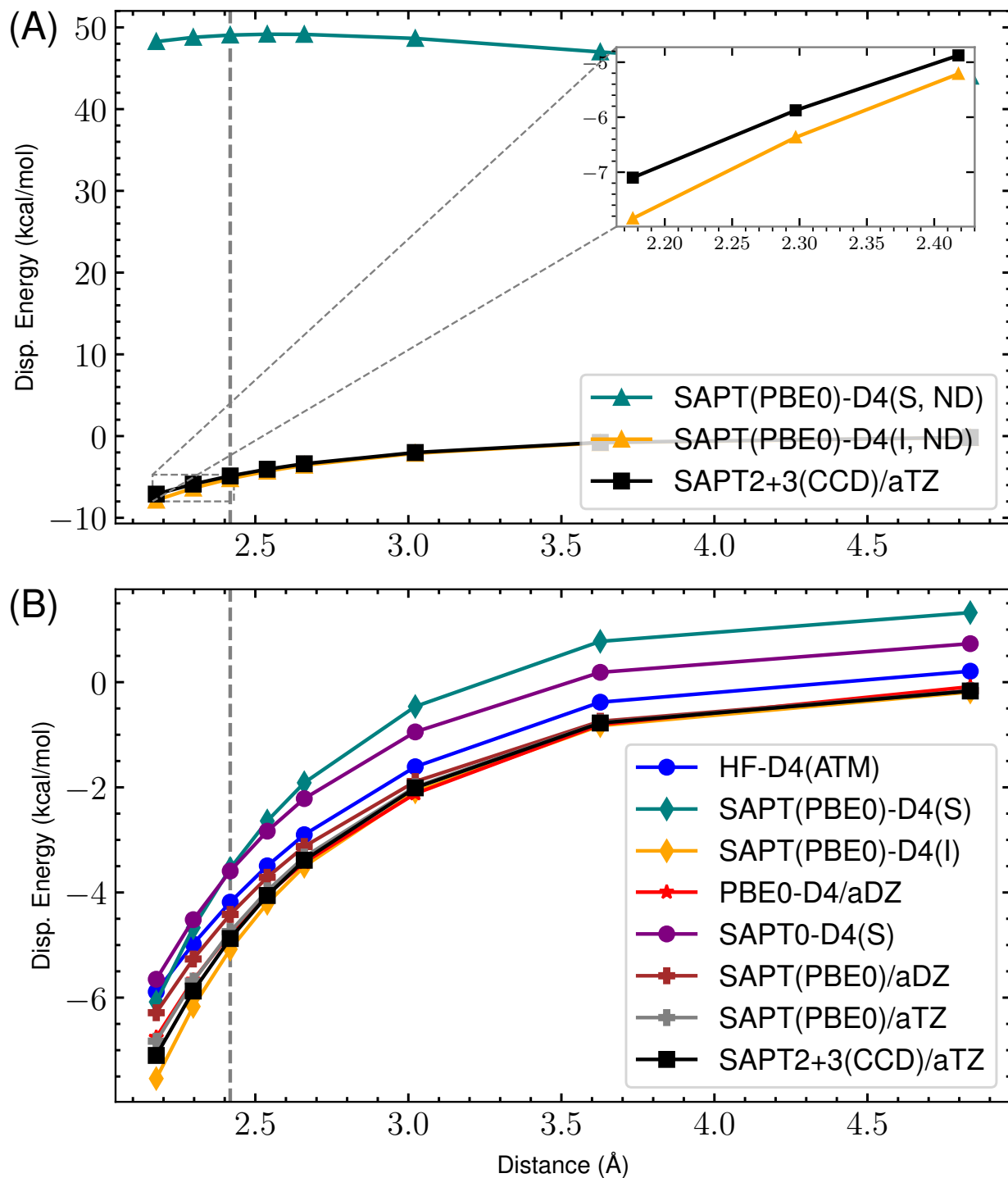
Figure 61: s66x8 61_Pentane-AcOH : Dispersion potential Energy curve for SAPT(PBE0) with aDZ/aTZ and -D4 variants versus the reference SAPT2+3(CCD)/aug-cc-pVTZ dispersion energy. (A) highlights the completely non-damped (ND) D4 curves compared to the reference for both supermolecular (S) and intermolecular (I). The remaining s_8 = 0.89529649 . (B) shows the damped -D4(S), -D4(I), HF-D4, SAPT(PBE0)/aDZ, SAPT(PBE0)/aTZ, and reference dispersion energies. Here, (S) and (I) refer to the supermolecular and intermolecular dispersion energy approaches, respectively. The “ND” states that no damping function is used. For the damped SAPT(PBE0)-D4(S) and SAPT(PBE0)-D4(I) terms, a_1 , a_2 , and s_8 are fit to the residual CCSD(T)/CBS energies on the 4470 dimer dataset.
