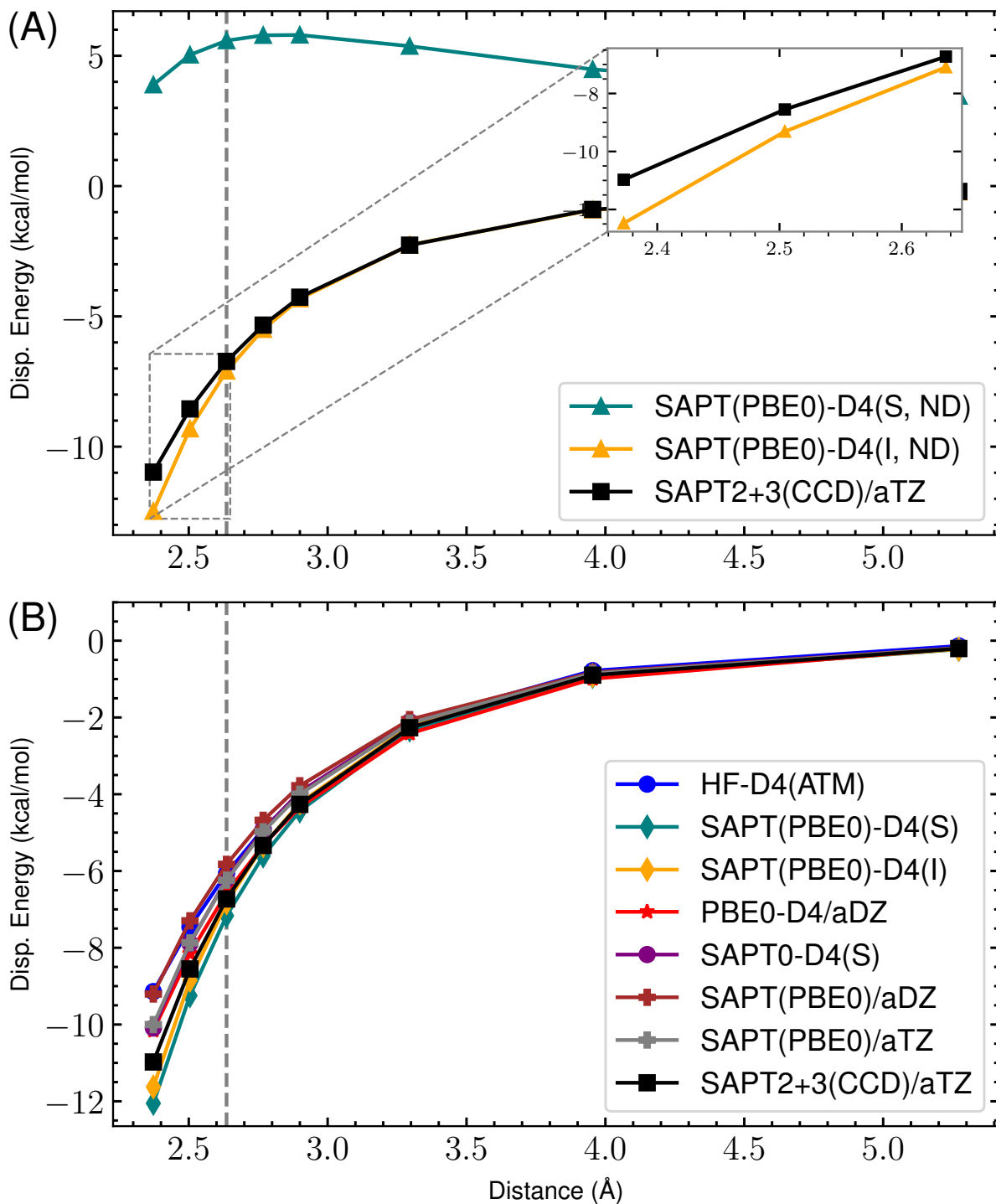
Figure 24: s66x8 57_Benzene-Peptide : Dispersion potential Energy curve for SAPT(PBE0) with aDZ/aTZ and -D4 variants versus the reference SAPT2+3(CCD)/aug-cc-pVTZ dispersion energy. (A) highlights the completely non-damped (ND) D4 curves compared to the reference for both supermolecular (S) and intermolecular (I). The remaining s_8 = 0.89529649 . (B) shows the damped -D4(S), -D4(I), HF-D4, SAPT(PBE0)/aDZ, SAPT(PBE0)/aTZ, and reference dispersion energies. Here, (S) and (I) refer to the supermolecular and intermolecular dispersion energy approaches, respectively. The “ND” states that no damping function is used. For the damped SAPT(PBE0)-D4(S) and SAPT(PBE0)-D4(I) terms, a_1 , a_2 , and s_8 are fit to the residual CCSD(T)/CBS energies on the 4470 dimer dataset.
