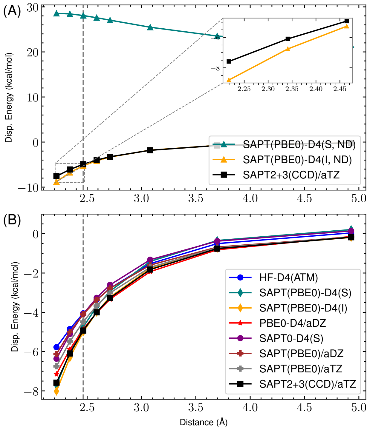
Figure 9: s66x8 52_Benzene-AcOH : Dispersion potential Energy curve for SAPT(PBE0) with aDZ/aTZ and -D4 variants versus the reference SAPT2+3(CCD)/aug-cc-pVTZ dispersion energy. (A) highlights the completely non-damped (ND) D4 curves compared to the reference for both supermolecular (S) and intermolecular (I). The remaining s_8 = 0.89529649 . (B) shows the damped -D4(S), -D4(I), HF-D4, SAPT(PBE0)/aDZ, SAPT(PBE0)/aTZ, and reference dispersion energies. Here, (S) and (I) refer to the supermolecular and intermolecular dispersion energy approaches, respectively. The “ND” states that no damping function is used. For the damped SAPT(PBE0)-D4(S) and SAPT(PBE0)-D4(I) terms, a_1 , a_2 , and s_8 are fit to the residual CCSD(T)/CBS energies on the 4470 dimer dataset.
