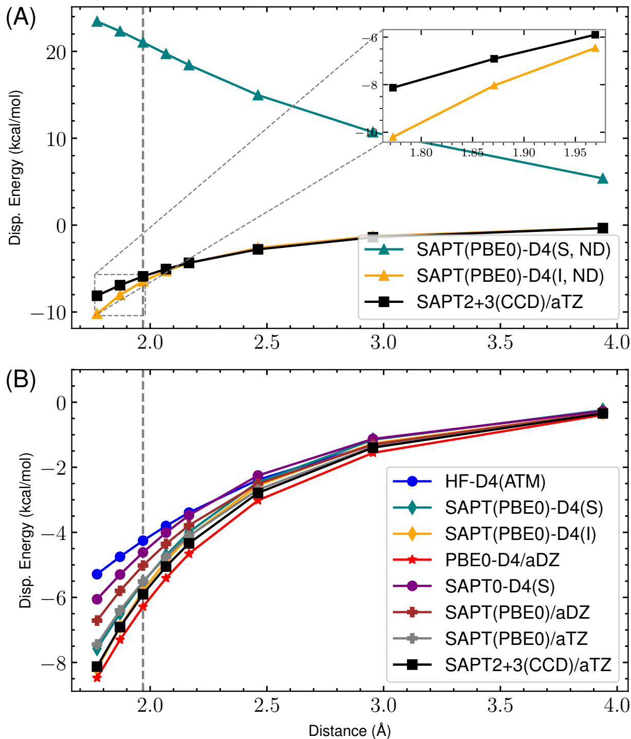
Figure 27: s66x8 15_Peptide-Peptide : Dispersion potential Energy curve for SAPT(PBE0) with aDZ/aTZ and -D4 variants versus the reference SAPT2+3(CCD)/aug-cc-pVTZ dispersion energy. (A) highlights the completely non-damped (ND) D4 curves compared to the reference for both supermolecular (S) and intermolecular (I). The remaining s_8 = 0.89529649 . (B) shows the damped -D4(S), -D4(I), HF-D4, SAPT(PBE0)/aDZ, SAPT(PBE0)/aTZ, and reference dispersion energies. Here, (S) and (I) refer to the supermolecular and intermolecular dispersion energy approaches, respectively. The “ND” states that no damping function is used. For the damped SAPT(PBE0)-D4(S) and SAPT(PBE0)-D4(I) terms, a_1 , a_2 , and s_8 are fit to the residual CCSD(T)/CBS energies on the 4470 dimer dataset.
