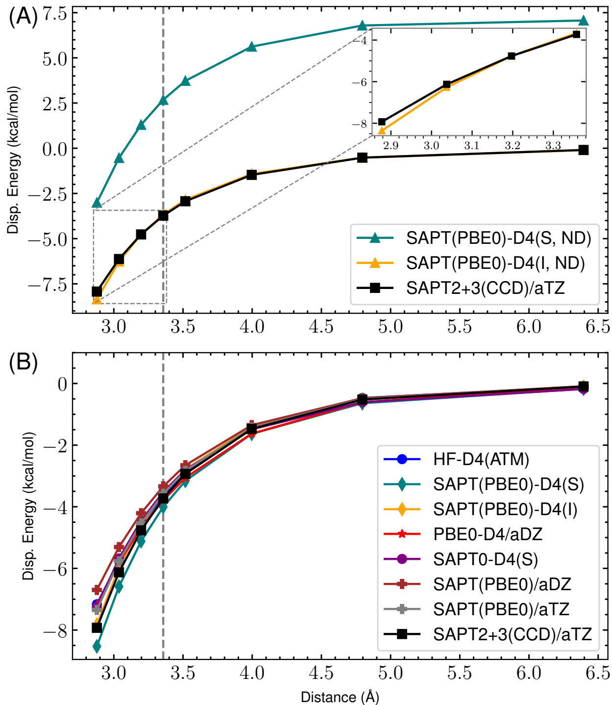
Figure 14: s66x8 33_Pyridine-Ethene : Dispersion potential Energy curve for SAPT(PBE0) with aDZ/aTZ and -D4 variants versus the reference SAPT2+3(CCD)/aug-cc-pVTZ dispersion energy. (A) highlights the completely non-damped (ND) D4 curves compared to the reference for both supermolecular (S) and intermolecular (I). The remaining s_8 = 0.89529649 . (B) shows the damped -D4(S), -D4(I), HF-D4, SAPT(PBE0)/aDZ, SAPT(PBE0)/aTZ, and reference dispersion energies. Here, (S) and (I) refer to the supermolecular and intermolecular dispersion energy approaches, respectively. The “ND” states that no damping function is used. For the damped SAPT(PBE0)-D4(S) and SAPT(PBE0)-D4(I) terms, a_1 , a_2 , and s_8 are fit to the residual CCSD(T)/CBS energies on the 4470 dimer dataset.
