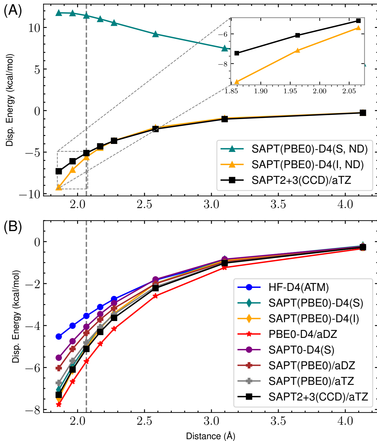
Figure 1: s66x8 14_Peptide-MeNH2 : Dispersion potential Energy curve for SAPT(PBE0) with aDZ/aTZ and -D4 variants versus the reference SAPT2+3(CCD)/aug-cc-pVTZ dispersion energy. (A) highlights the completely non-damped (ND) D4 curves compared to the reference for both supermolecular (S) and intermolecular (I). The remaining s_8 = 0.89529649 . (B) shows the damped -D4(S), -D4(I), HF-D4, SAPT(PBE0)/aDZ, SAPT(PBE0)/aTZ, and reference dispersion energies. Here, (S) and (I) refer to the supermolecular and intermolecular dispersion energy approaches, respectively. The “ND” states that no damping function is used. For the damped SAPT(PBE0)-D4(S) and SAPT(PBE0)-D4(I) terms, a_1 , a_2 , and s_8 are fit to the residual CCSD(T)/CBS energies on the 4470 dimer dataset.
