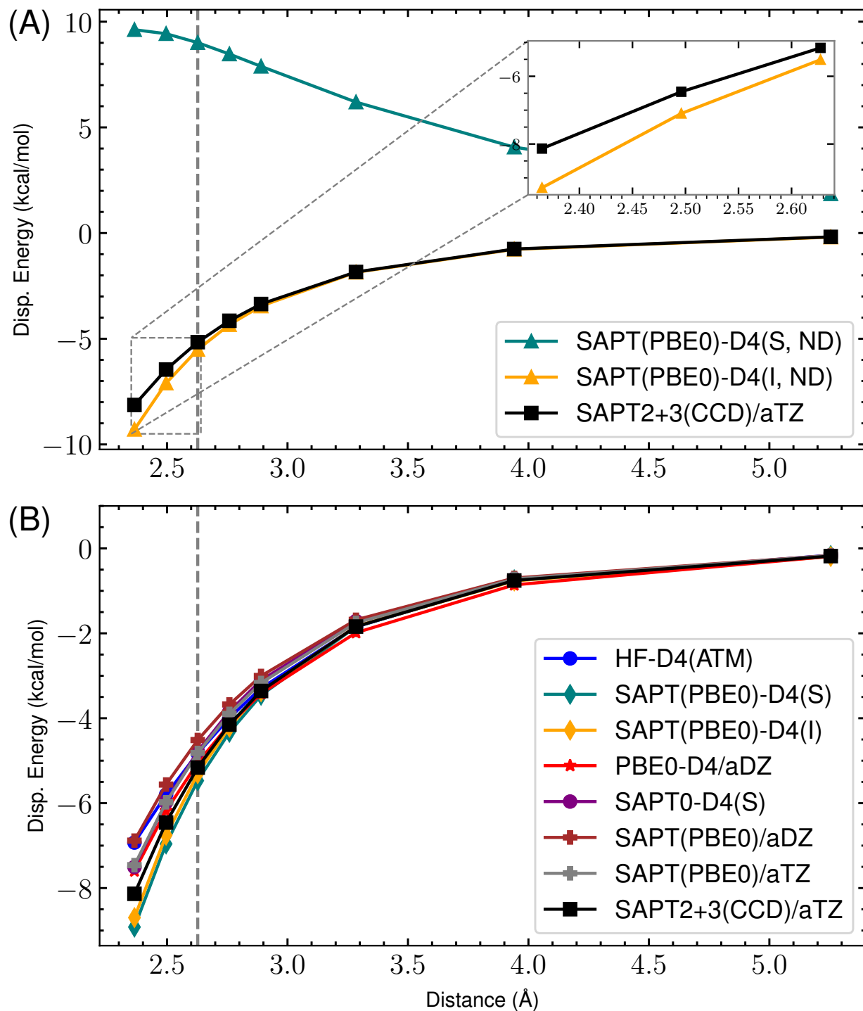
Figure 28: s66x8 48_Pyridine-Pyridine : Dispersion potential Energy curve for SAPT(PBE0) with aDZ/aTZ and -D4 variants versus the reference SAPT2+3(CCD)/aug-cc-pVTZ dispersion energy. (A) highlights the completely non-damped (ND) D4 curves compared to the reference for both supermolecular (S) and intermolecular (I). The remaining s_8 = 0.89529649 . (B) shows the damped -D4(S), -D4(I), HF-D4, SAPT(PBE0)/aDZ, SAPT(PBE0)/aTZ, and reference dispersion energies. Here, (S) and (I) refer to the supermolecular and intermolecular dispersion energy approaches, respectively. The “ND” states that no damping function is used. For the damped SAPT(PBE0)-D4(S) and SAPT(PBE0)-D4(I) terms, a_1 , a_2 , and s_8 are fit to the residual CCSD(T)/CBS energies on the 4470 dimer dataset.
