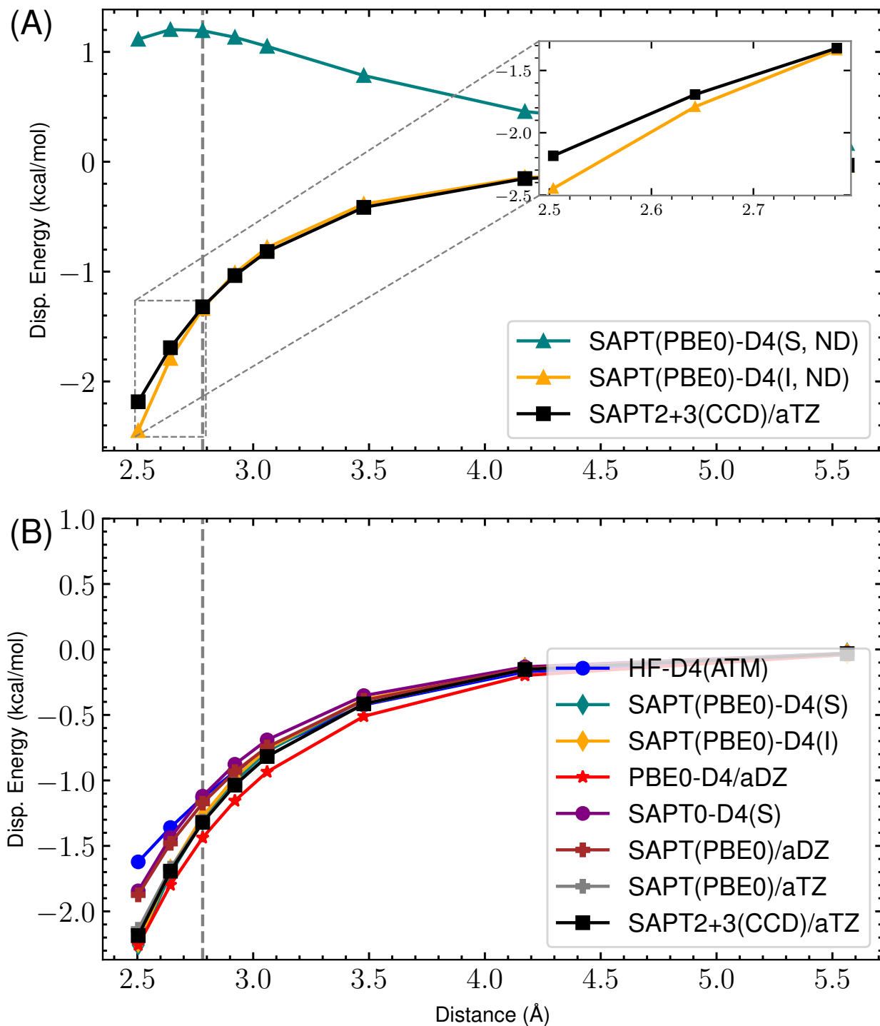
Figure 35: s66x8 51_Ethyne-Ethyne : Dispersion potential Energy curve for SAPT(PBE0) with aDZ/aTZ and -D4 variants versus the reference SAPT2+3(CCD)/aug-cc-pVTZ dispersion energy. (A) highlights the completely non-damped (ND) D4 curves compared to the reference for both supermolecular (S) and intermolecular (I). The remaining s_8 = 0.89529649 . (B) shows the damped -D4(S), -D4(I), HF-D4, SAPT(PBE0)/aDZ, SAPT(PBE0)/aTZ, and reference dispersion energies. Here, (S) and (I) refer to the supermolecular and intermolecular dispersion energy approaches, respectively. The “ND” states that no damping function is used. For the damped SAPT(PBE0)-D4(S) and SAPT(PBE0)-D4(I) terms, a_1 , a_2 , and s_8 are fit to the residual CCSD(T)/CBS energies on the 4470 dimer dataset.
