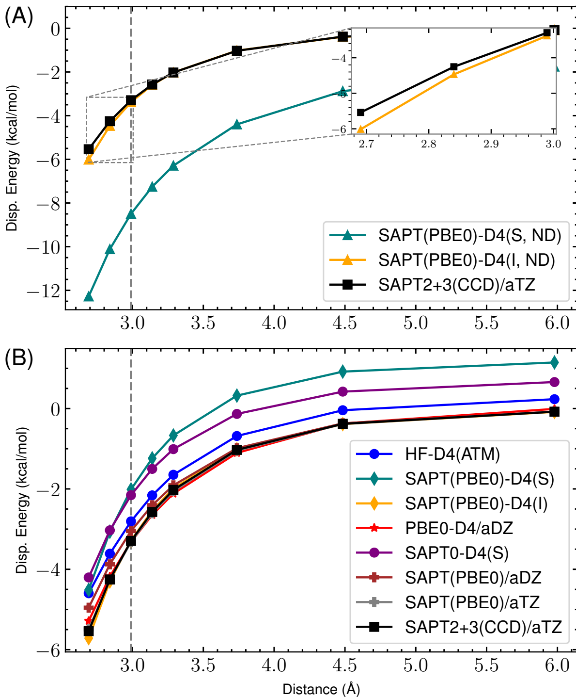
Figure 2: s66x8 45_Ethyne-Pentane : Dispersion potential Energy curve for SAPT(PBE0) with aDZ/aTZ and -D4 variants versus the reference SAPT2+3(CCD)/aug-cc-pVTZ dispersion energy. (A) highlights the completely non-damped (ND) D4 curves compared to the reference for both supermolecular (S) and intermolecular (I). The remaining s_8 = 0.89529649 . (B) shows the damped -D4(S), -D4(I), HF-D4, SAPT(PBE0)/aDZ, SAPT(PBE0)/aTZ, and reference dispersion energies. Here, (S) and (I) refer to the supermolecular and intermolecular dispersion energy approaches, respectively. The “ND” states that no damping function is used. For the damped SAPT(PBE0)-D4(S) and SAPT(PBE0)-D4(I) terms, a_1 , a_2 , and s_8 are fit to the residual CCSD(T)/CBS energies on the 4470 dimer dataset.
