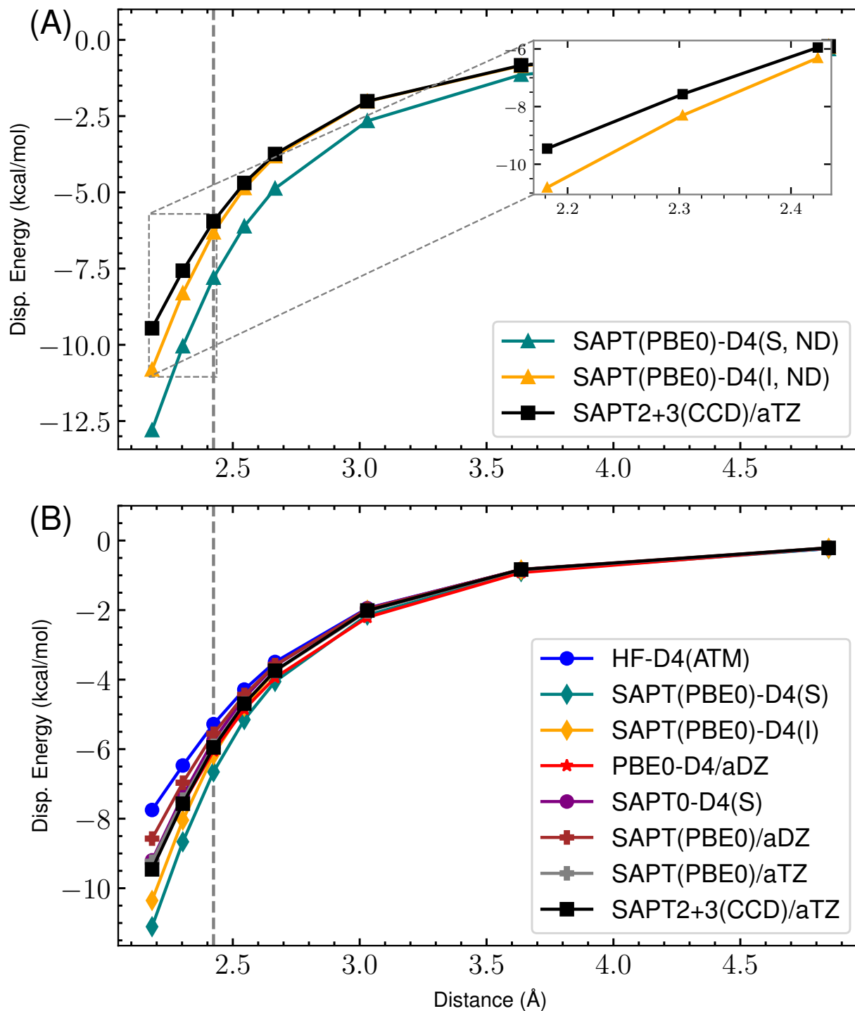
Figure 57: s66x8 38_Cyclopentane-Cyclopentane : Dispersion potential Energy curve for SAPT(PBE0) with aDZ/aTZ and -D4 variants versus the reference SAPT2+3(CCD)/aug-cc-pVTZ dispersion energy. (A) highlights the completely non-damped (ND) D4 curves compared to the reference for both supermolecular (S) and intermolecular (I). The remaining s_8 = 0.89529649 . (B) shows the damped -D4(S), -D4(I), HF-D4, SAPT(PBE0)/aDZ, SAPT(PBE0)/aTZ, and reference dispersion energies. Here, (S) and (I) refer to the supermolecular and intermolecular dispersion energy approaches, respectively. The “ND” states that no damping function is used. For the damped SAPT(PBE0)-D4(S) and SAPT(PBE0)-D4(I) terms, a_1 , a_2 , and s_8 are fit to the residual CCSD(T)/CBS energies on the 4470 dimer dataset.
