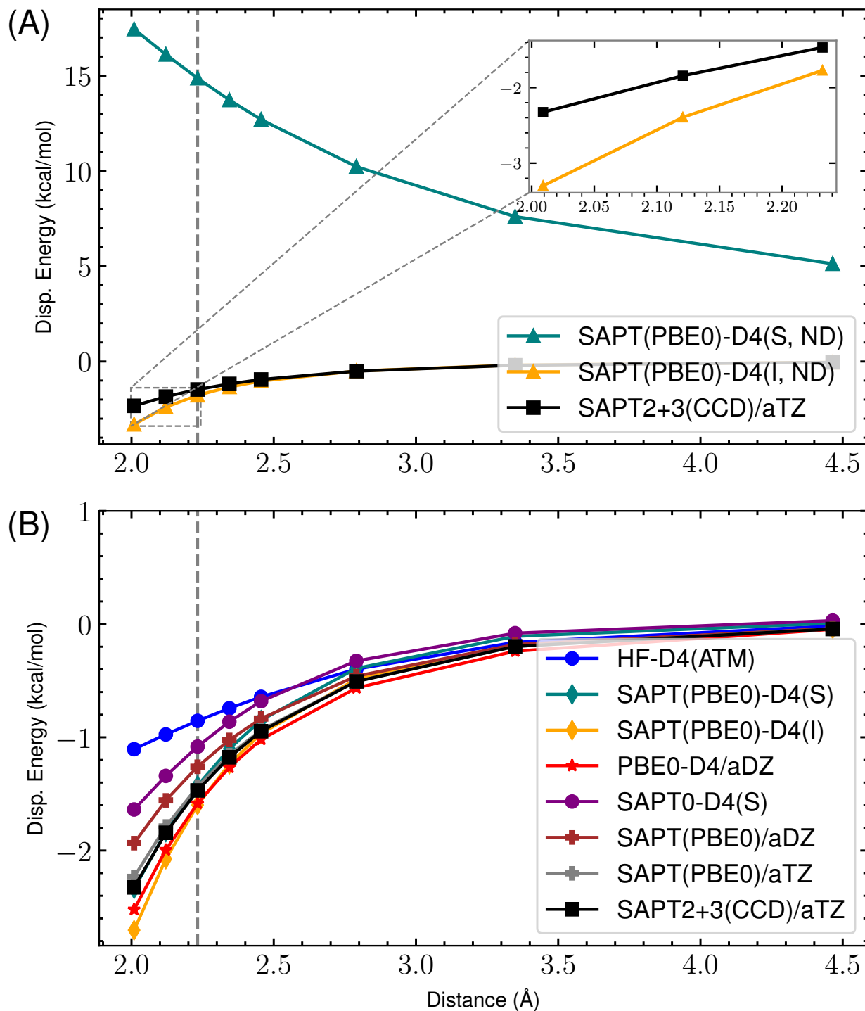
Figure 30: s66x8 59_Ethyne-Water : Dispersion potential Energy curve for SAPT(PBE0) with aDZ/aTZ and -D4 variants versus the reference SAPT2+3(CCD)/aug-cc-pVTZ dispersion energy. (A) highlights the completely non-damped (ND) D4 curves compared to the reference for both supermolecular (S) and intermolecular (I). The remaining s_8 = 0.89529649 . (B) shows the damped -D4(S), -D4(I), HF-D4, SAPT(PBE0)/aDZ, SAPT(PBE0)/aTZ, and reference dispersion energies. Here, (S) and (I) refer to the supermolecular and intermolecular dispersion energy approaches, respectively. The “ND” states that no damping function is used. For the damped SAPT(PBE0)-D4(S) and SAPT(PBE0)-D4(I) terms, a_1 , a_2 , and s_8 are fit to the residual CCSD(T)/CBS energies on the 4470 dimer dataset.
