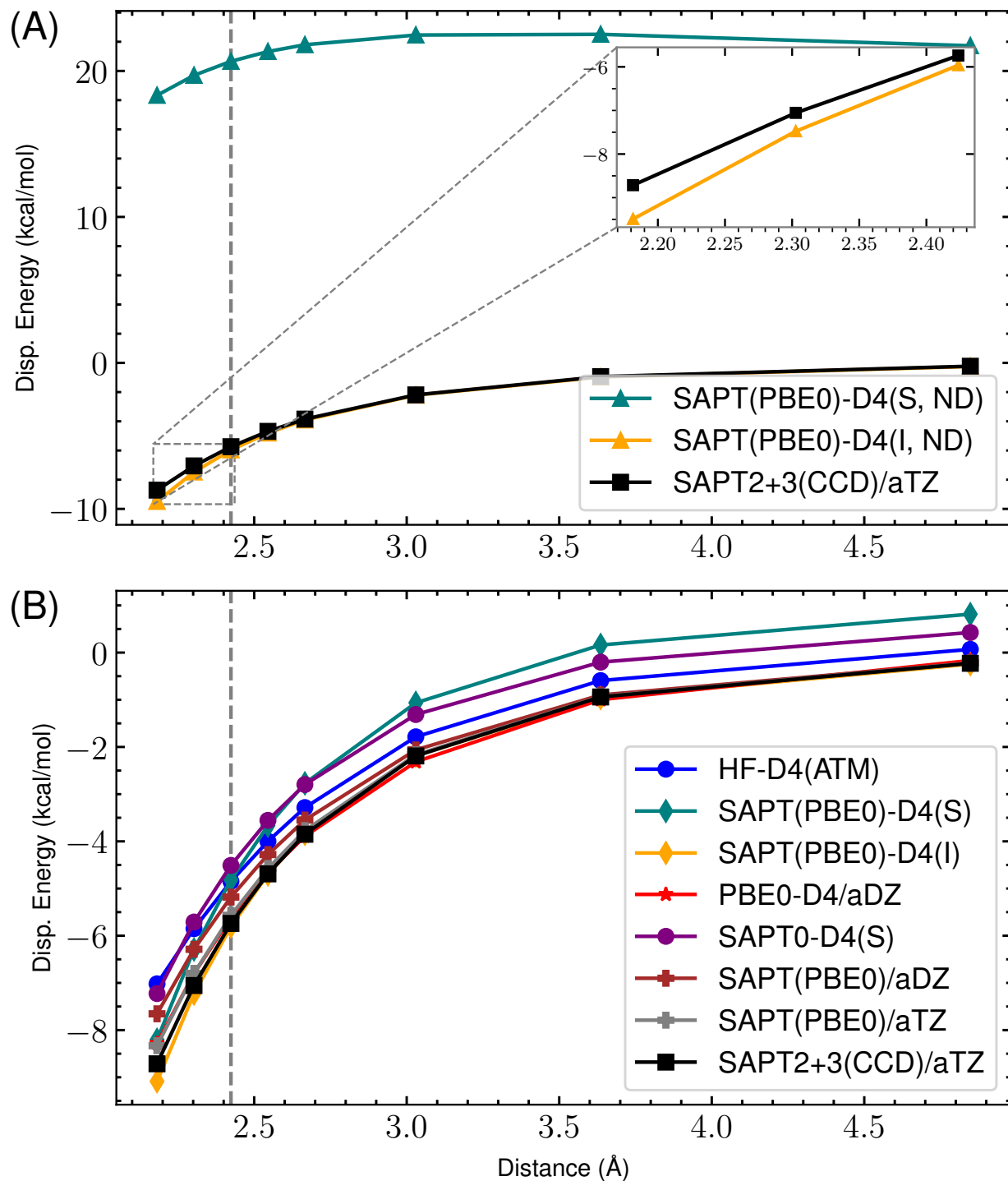
Figure 51: s66x8 62_Pentane-AcNH2 : Dispersion potential Energy curve for SAPT(PBE0) with aDZ/aTZ and -D4 variants versus the reference SAPT2+3(CCD)/aug-cc-pVTZ dispersion energy. (A) highlights the completely non-damped (ND) D4 curves compared to the reference for both supermolecular (S) and intermolecular (I). The remaining s_8 = 0.89529649 . (B) shows the damped -D4(S), -D4(I), HF-D4, SAPT(PBE0)/aDZ, SAPT(PBE0)/aTZ, and reference dispersion energies. Here, (S) and (I) refer to the supermolecular and intermolecular dispersion energy approaches, respectively. The “ND” states that no damping function is used. For the damped SAPT(PBE0)-D4(S) and SAPT(PBE0)-D4(I) terms, a_1 , a_2 , and s_8 are fit to the residual CCSD(T)/CBS energies on the 4470 dimer dataset.
