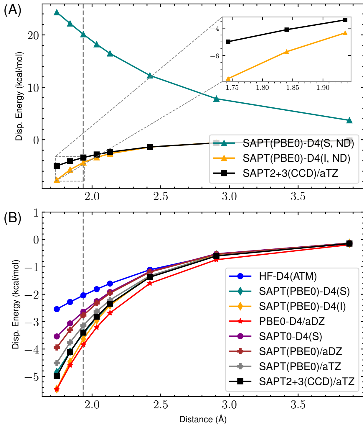
Figure 33: s66x8 05_MeOH-MeOH : Dispersion potential Energy curve for SAPT(PBE0) with aDZ/aTZ and -D4 variants versus the reference SAPT2+3(CCD)/aug-cc-pVTZ dispersion energy. (A) highlights the completely non-damped (ND) D4 curves compared to the reference for both supermolecular (S) and intermolecular (I). The remaining s_8 = 0.89529649 . (B) shows the damped -D4(S), -D4(I), HF-D4, SAPT(PBE0)/aDZ, SAPT(PBE0)/aTZ, and reference dispersion energies. Here, (S) and (I) refer to the supermolecular and intermolecular dispersion energy approaches, respectively. The “ND” states that no damping function is used. For the damped SAPT(PBE0)-D4(S) and SAPT(PBE0)-D4(I) terms, a_1 , a_2 , and s_8 are fit to the residual CCSD(T)/CBS energies on the 4470 dimer dataset.
