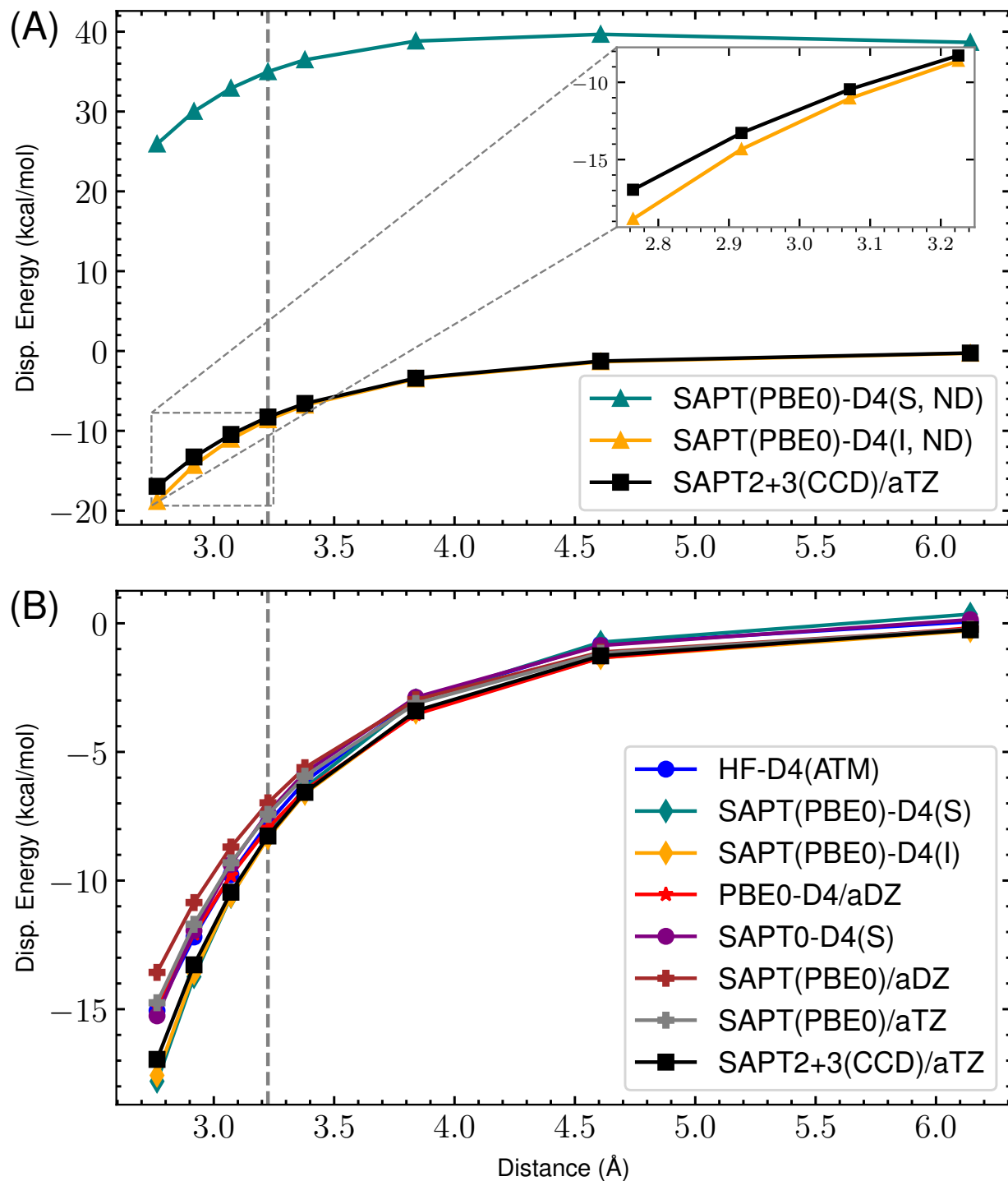
Figure 4: s66x8 28_Benzene-Uracil : Dispersion potential Energy curve for SAPT(PBE0) with aDZ/aTZ and -D4 variants versus the reference SAPT2+3(CCD)/aug-cc-pVTZ dispersion energy. (A) highlights the completely non-damped (ND) D4 curves compared to the reference for both supermolecular (S) and intermolecular (I). The remaining s_8 = 0.89529649 . (B) shows the damped -D4(S), -D4(I), HF-D4, SAPT(PBE0)/aDZ, SAPT(PBE0)/aTZ, and reference dispersion energies. Here, (S) and (I) refer to the supermolecular and intermolecular dispersion energy approaches, respectively. The “ND” states that no damping function is used. For the damped SAPT(PBE0)-D4(S) and SAPT(PBE0)-D4(I) terms, a_1 , a_2 , and s_8 are fit to the residual CCSD(T)/CBS energies on the 4470 dimer dataset.
