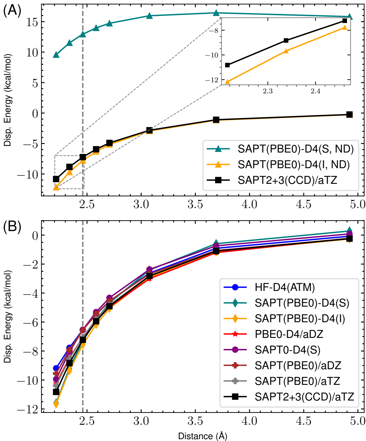
Figure 45: s66x8 46_Peptide-Pentane : Dispersion potential Energy curve for SAPT(PBE0) with aDZ/aTZ and -D4 variants versus the reference SAPT2+3(CCD)/aug-cc-pVTZ dispersion energy. (A) highlights the completely non-damped (ND) D4 curves compared to the reference for both supermolecular (S) and intermolecular (I). The remaining s_8 = 0.89529649 . (B) shows the damped -D4(S), -D4(I), HF-D4, SAPT(PBE0)/aDZ, SAPT(PBE0)/aTZ, and reference dispersion energies. Here, (S) and (I) refer to the supermolecular and intermolecular dispersion energy approaches, respectively. The “ND” states that no damping function is used. For the damped SAPT(PBE0)-D4(S) and SAPT(PBE0)-D4(I) terms, a_1 , a_2 , and s_8 are fit to the residual CCSD(T)/CBS energies on the 4470 dimer dataset.
