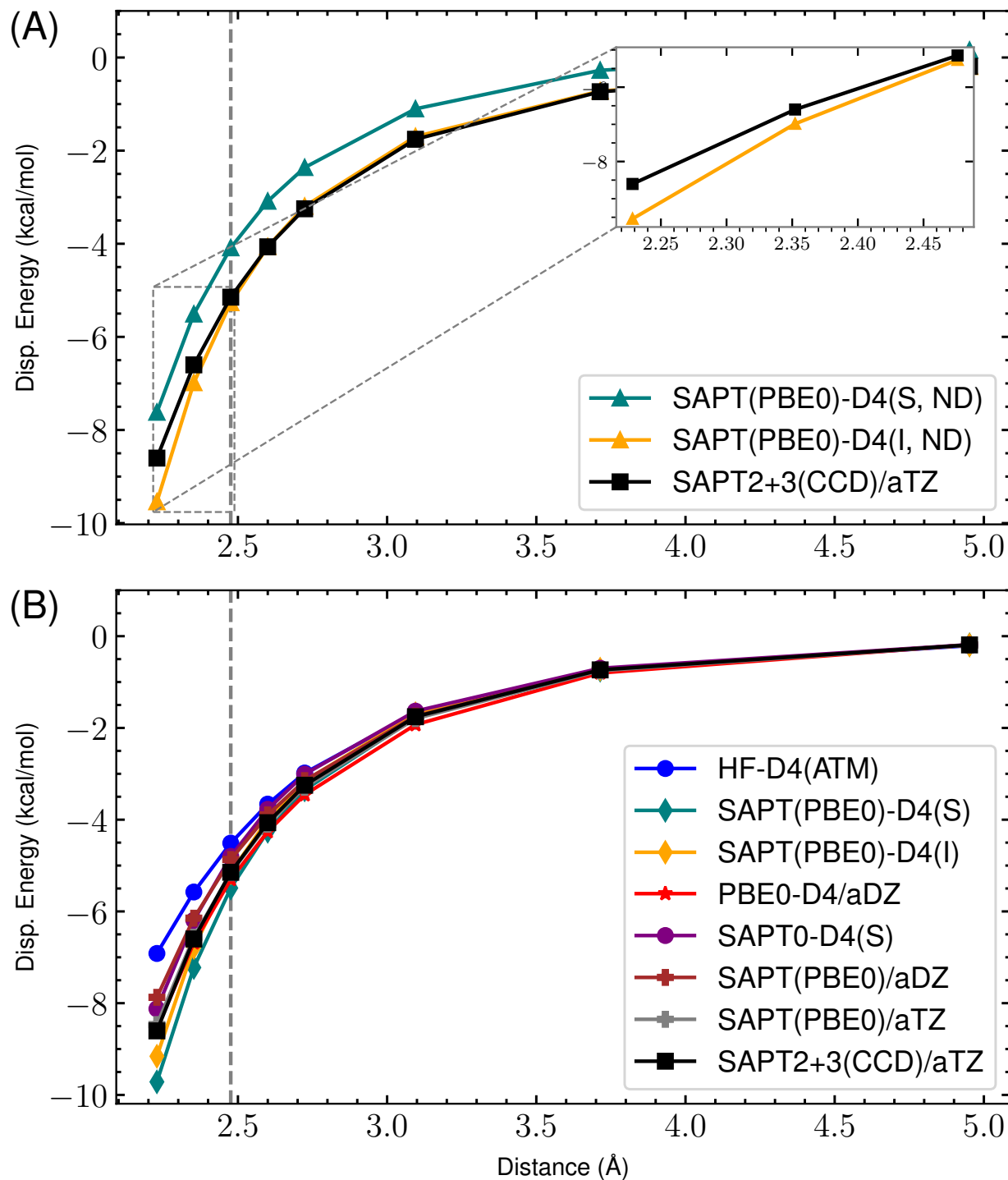
Figure 47: s66x8 35_Neopentane-Pentane : Dispersion potential Energy curve for SAPT(PBE0) with aDZ/aTZ and -D4 variants versus the reference SAPT2+3(CCD)/aug-cc-pVTZ dispersion energy. (A) highlights the completely non-damped (ND) D4 curves compared to the reference for both supermolecular (S) and intermolecular (I). The remaining s_8 = 0.89529649 . (B) shows the damped -D4(S), -D4(I), HF-D4, SAPT(PBE0)/aDZ, SAPT(PBE0)/aTZ, and reference dispersion energies. Here, (S) and (I) refer to the supermolecular and intermolecular dispersion energy approaches, respectively. The “ND” states that no damping function is used. For the damped SAPT(PBE0)-D4(S) and SAPT(PBE0)-D4(I) terms, a_1 , a_2 , and s_8 are fit to the residual CCSD(T)/CBS energies on the 4470 dimer dataset.
