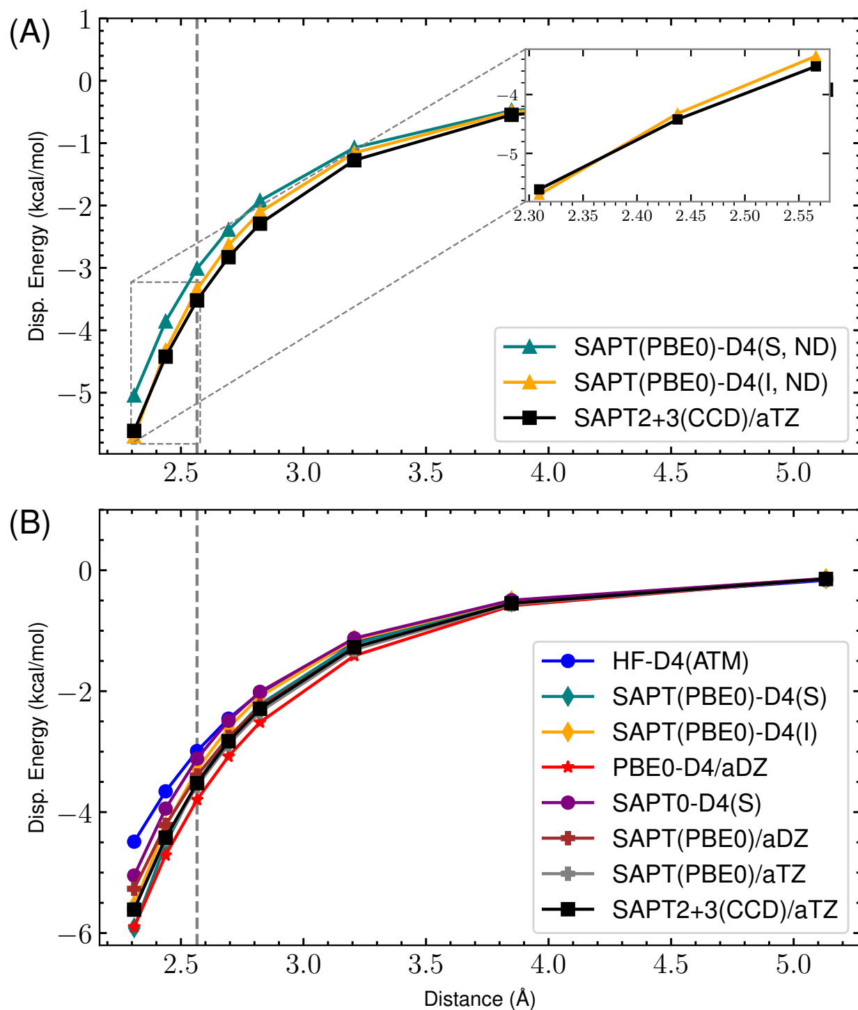
Figure 62: s66x8 36_Neopentane-Neopentane : Dispersion potential Energy curve for SAPT(PBE0) with aDZ/aTZ and -D4 variants versus the reference SAPT2+3(CCD)/aug-cc-pVTZ dispersion energy. (A) highlights the completely non-damped (ND) D4 curves compared to the reference for both supermolecular (S) and intermolecular (I). The remaining s_8 = 0.89529649 . (B) shows the damped -D4(S), -D4(I), HF-D4, SAPT(PBE0)/aDZ, SAPT(PBE0)/aTZ, and reference dispersion energies. Here, (S) and (I) refer to the supermolecular and intermolecular dispersion energy approaches, respectively. The “ND” states that no damping function is used. For the damped SAPT(PBE0)-D4(S) and SAPT(PBE0)-D4(I) terms, a_1 , a_2 , and s_8 are fit to the residual CCSD(T)/CBS energies on the 4470 dimer dataset.
