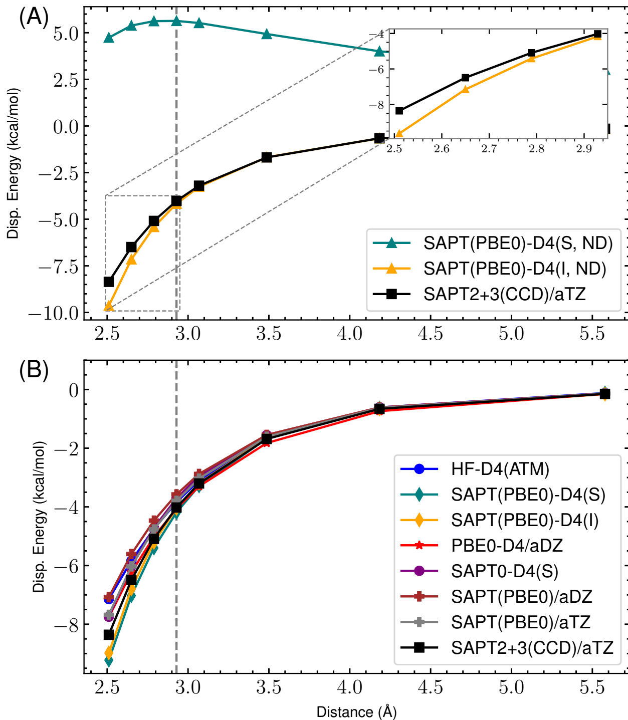
Figure 64: s66x8 49_Benzene-Pyridine : Dispersion potential Energy curve for SAPT(PBE0) with aDZ/aTZ and -D4 variants versus the reference SAPT2+3(CCD)/aug-cc-pVTZ dispersion energy. (A) highlights the completely non-damped (ND) D4 curves compared to the reference for both supermolecular (S) and intermolecular (I). The remaining s_8 = 0.89529649 . (B) shows the damped -D4(S), -D4(I), HF-D4, SAPT(PBE0)/aDZ, SAPT(PBE0)/aTZ, and reference dispersion energies. Here, (S) and (I) refer to the supermolecular and intermolecular dispersion energy approaches, respectively. The “ND” states that no damping function is used. For the damped SAPT(PBE0)-D4(S) and SAPT(PBE0)-D4(I) terms, a_1 , a_2 , and s_8 are fit to the residual CCSD(T)/CBS energies on the 4470 dimer dataset.
