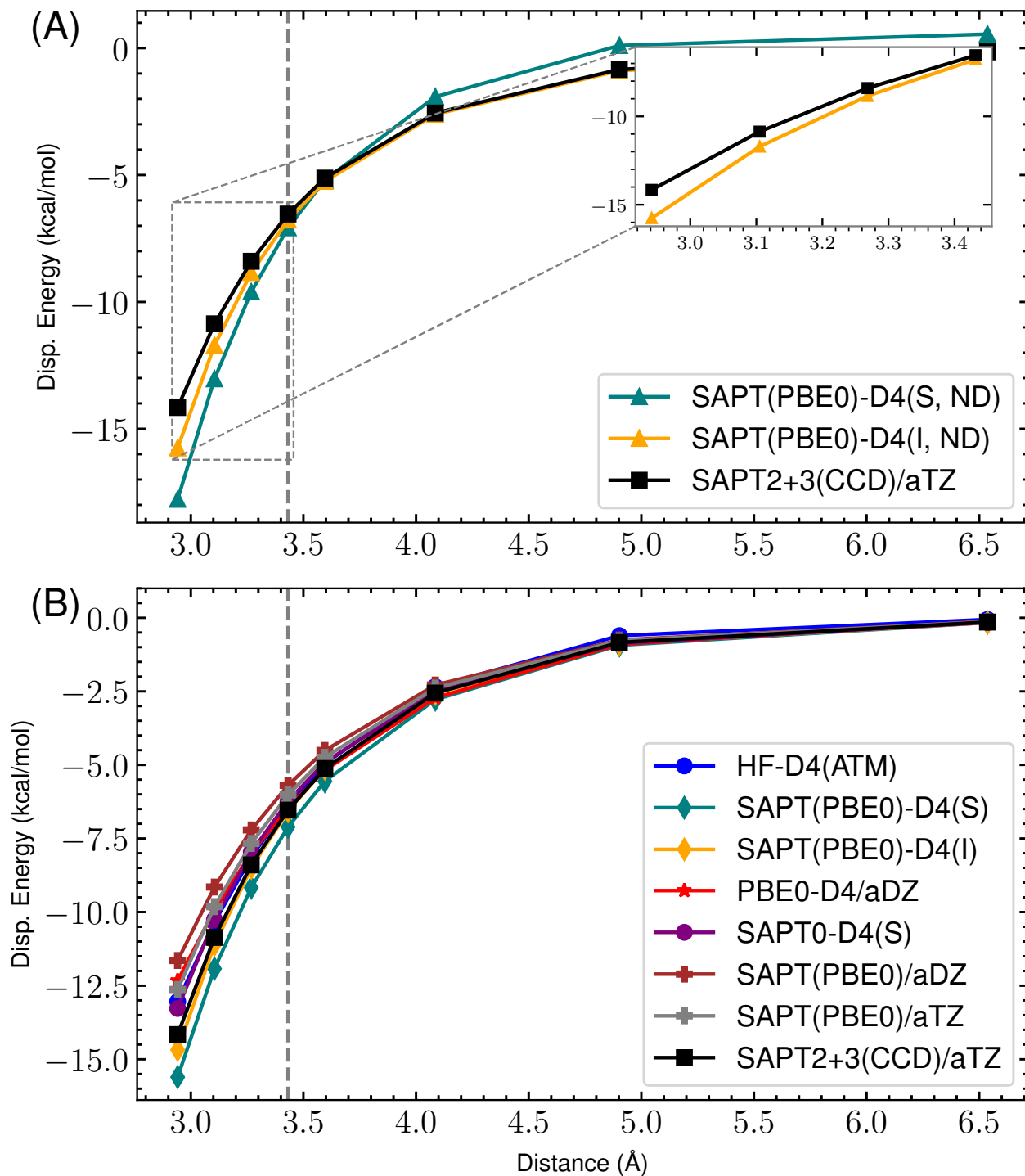
Figure 12: s66x8 25.Pyridine-Pyridine : Dispersion potential Energy curve for SAPT(PBE0) with aDZ/aTZ and -D4 variants versus the reference SAPT2+3(CCD)/aug-cc-pVTZ dispersion energy. (A) highlights the completely non-damped (ND) D4 curves compared to the reference for both supermolecular (S) and intermolecular (I). The remaining s_8 = 0.89529649 . (B) shows the damped -D4(S), -D4(I), HF-D4, SAPT(PBE0)/aDZ, SAPT(PBE0)/aTZ, and reference dispersion energies. Here, (S) and (I) refer to the supermolecular and intermolecular dispersion energy approaches, respectively. The “ND” states that no damping function is used. For the damped SAPT(PBE0)-D4(S) and SAPT(PBE0)-D4(I) terms, a_1 , a_2 , and s_8 are fit to the residual CCSD(T)/CBS energies on the 4470 dimer dataset.
