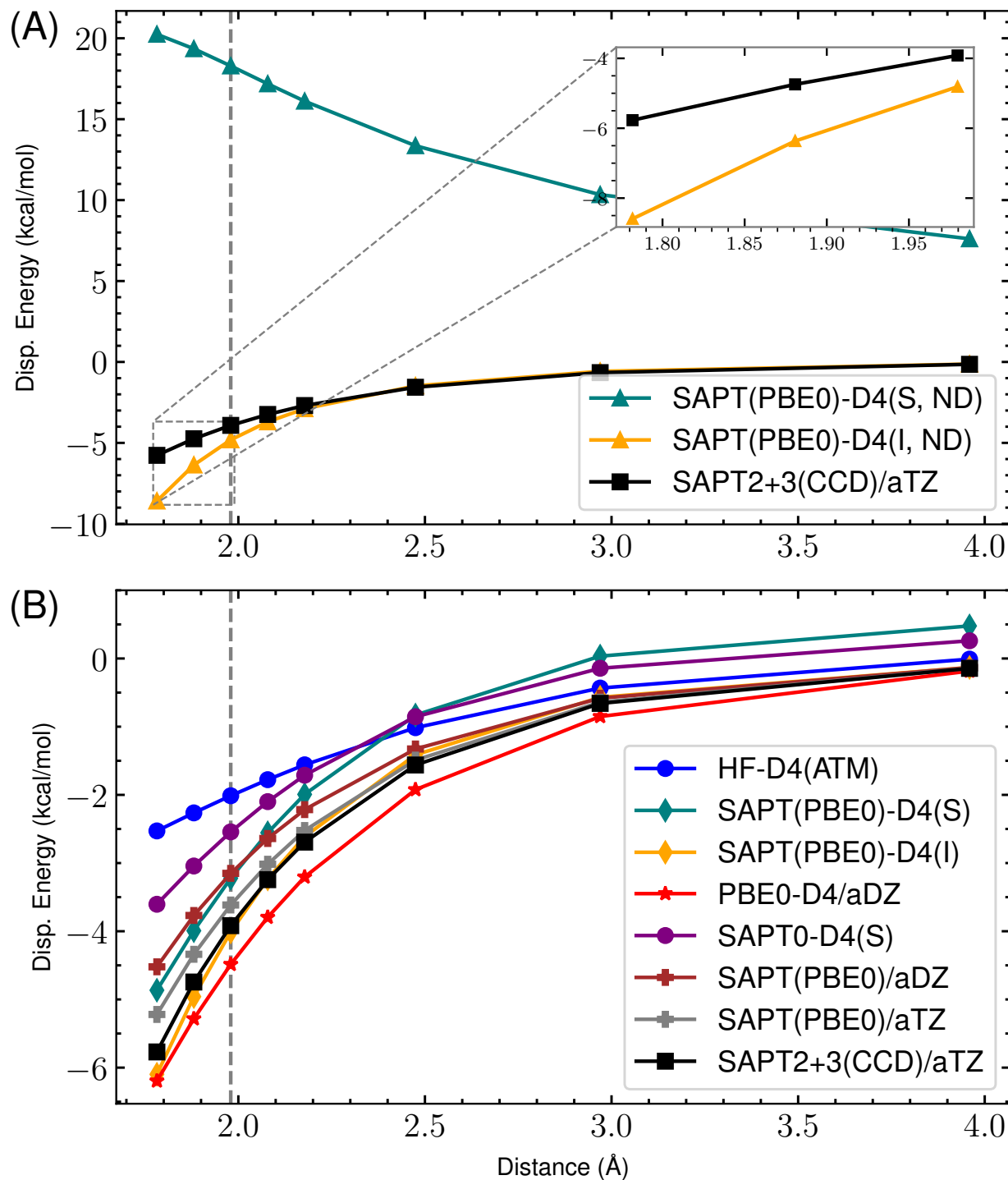
Figure 60: s66x8 12_MeNH2-Water : Dispersion potential Energy curve for SAPT(PBE0) with aDZ/aTZ and -D4 variants versus the reference SAPT2+3(CCD)/aug-cc-pVTZ dispersion energy. (A) highlights the completely non-damped (ND) D4 curves compared to the reference for both supermolecular (S) and intermolecular (I). The remaining s_8 = 0.89529649 . (B) shows the damped -D4(S), -D4(I), HF-D4, SAPT(PBE0)/aDZ, SAPT(PBE0)/aTZ, and reference dispersion energies. Here, (S) and (I) refer to the supermolecular and intermolecular dispersion energy approaches, respectively. The “ND” states that no damping function is used. For the damped SAPT(PBE0)-D4(S) and SAPT(PBE0)-D4(I) terms, a_1 , a_2 , and s_8 are fit to the residual CCSD(T)/CBS energies on the 4470 dimer dataset.
