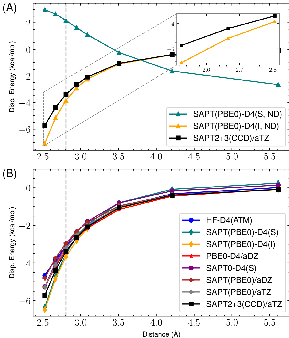
Figure 21: s66x8 50_Benzene-Ethyne : Dispersion potential Energy curve for SAPT(PBE0) with aDZ/aTZ and -D4 variants versus the reference SAPT2+3(CCD)/aug-cc-pVTZ dispersion energy. (A) highlights the completely non-damped (ND) D4 curves compared to the reference for both supermolecular (S) and intermolecular (I). The remaining s_8 = 0.89529649 . (B) shows the damped -D4(S), -D4(I), HF-D4, SAPT(PBE0)/aDZ, SAPT(PBE0)/aTZ, and reference dispersion energies. Here, (S) and (I) refer to the supermolecular and intermolecular dispersion energy approaches, respectively. The “ND” states that no damping function is used. For the damped SAPT(PBE0)-D4(S) and SAPT(PBE0)-D4(I) terms, a_1 , a_2 , and s_8 are fit to the residual CCSD(T)/CBS energies on the 4470 dimer dataset.
