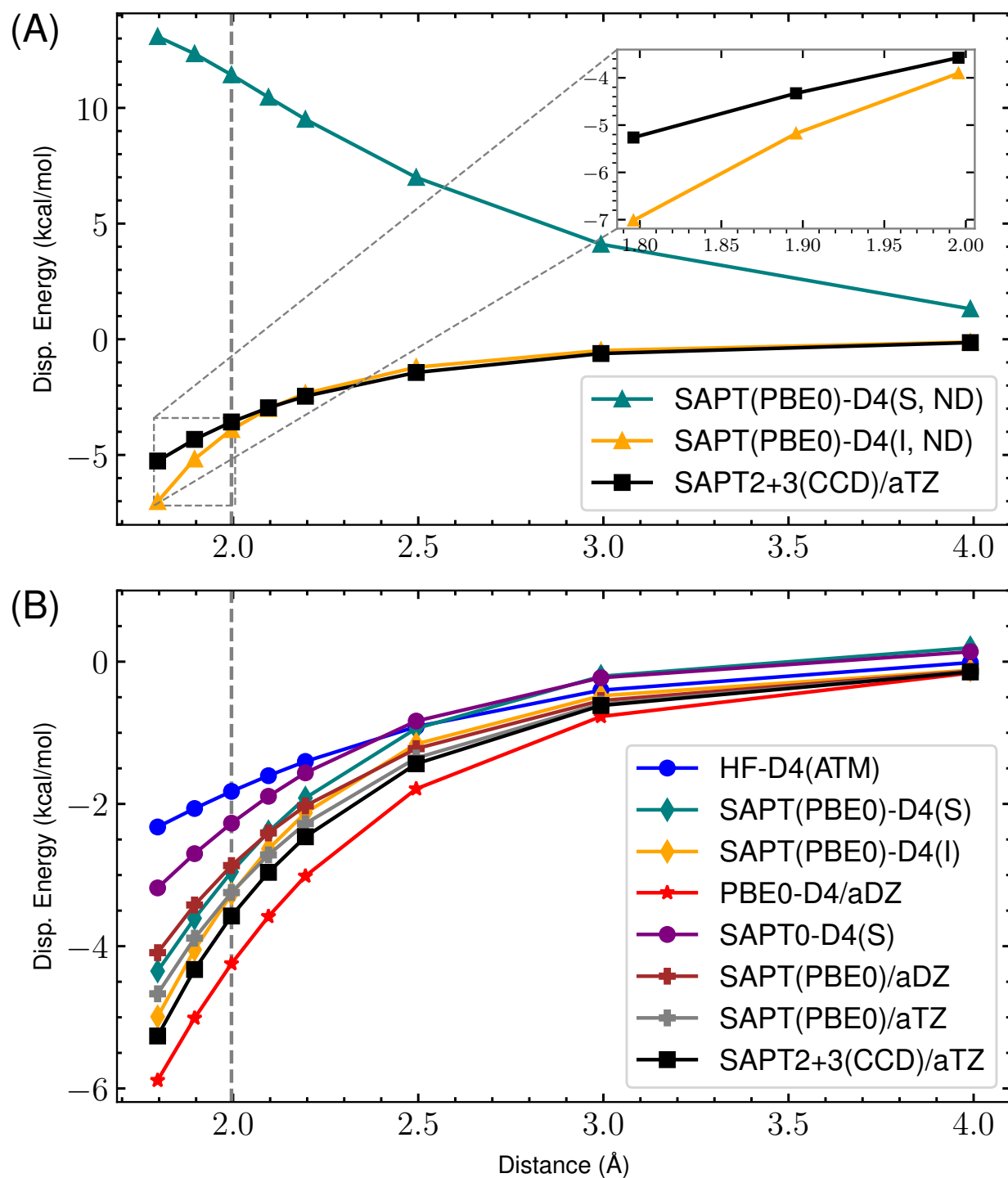
Figure 49: s66x8 18_Water-Pyridine : Dispersion potential Energy curve for SAPT(PBE0) with aDZ/aTZ and -D4 variants versus the reference SAPT2+3(CCD)/aug-cc-pVTZ dispersion energy. (A) highlights the completely non-damped (ND) D4 curves compared to the reference for both supermolecular (S) and intermolecular (I). The remaining s_8 = 0.89529649 . (B) shows the damped -D4(S), -D4(I), HF-D4, SAPT(PBE0)/aDZ, SAPT(PBE0)/aTZ, and reference dispersion energies. Here, (S) and (I) refer to the supermolecular and intermolecular dispersion energy approaches, respectively. The “ND” states that no damping function is used. For the damped SAPT(PBE0)-D4(S) and SAPT(PBE0)-D4(I) terms, a_1 , a_2 , and s_8 are fit to the residual CCSD(T)/CBS energies on the 4470 dimer dataset.
