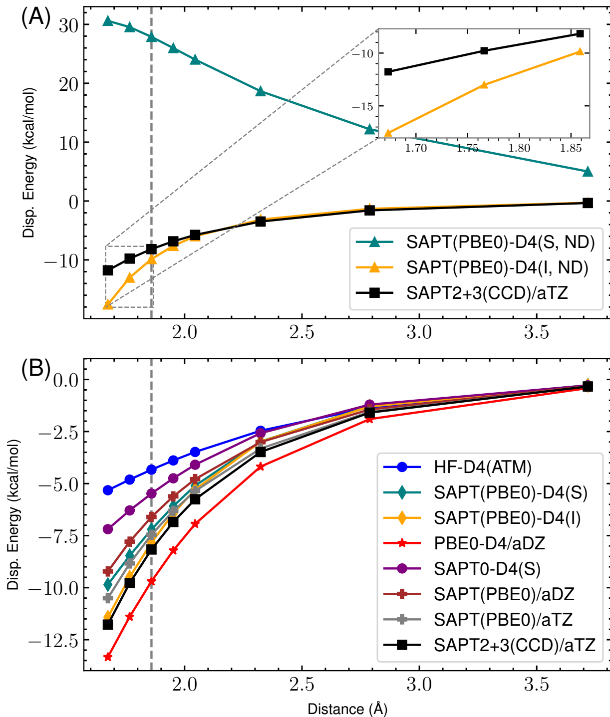
Figure 50: s66x8 21_AcNH 2 -AcNH 2 : Dispersion potential Energy curve for SAPT(PBE0) with aDZ/aTZ and -D4 variants versus the reference SAPT2+3(CCD)/aug-cc-pVTZ dispersion energy. (A) highlights the completely non-damped (ND) D4 curves compared to the reference for both supermolecular (S) and intermolecular (I). The remaining s_8 = 0.89529649 . (B) shows the damped -D4(S), -D4(I), HF-D4, SAPT(PBE0)/aDZ, SAPT(PBE0)/aTZ, and reference dispersion energies. Here, (S) and (I) refer to the supermolecular and intermolecular dispersion energy approaches, respectively. The “ND” states that no damping function is used. For the damped SAPT(PBE0)-D4(S) and SAPT(PBE0)-D4(I) terms, a_1 , a_2 , and s_8 are fit to the residual CCSD(T)/CBS energies on the 4470 dimer dataset.
