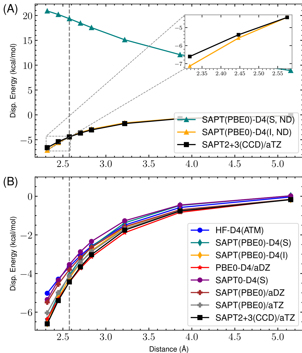
Figure 36: s66x8 53_Benzene-AcNH2 : Dispersion potential Energy curve for SAPT(PBE0) with aDZ/aTZ and -D4 variants versus the reference SAPT2+3(CCD)/aug-cc-pVTZ dispersion energy. (A) highlights the completely non-damped (ND) D4 curves compared to the reference for both supermolecular (S) and intermolecular (I). The remaining s_8 = 0.89529649 . (B) shows the damped -D4(S), -D4(I), HF-D4, SAPT(PBE0)/aDZ, SAPT(PBE0)/aTZ, and reference dispersion energies. Here, (S) and (I) refer to the supermolecular and intermolecular dispersion energy approaches, respectively. The “ND” states that no damping function is used. For the damped SAPT(PBE0)-D4(S) and SAPT(PBE0)-D4(I) terms, a_1 , a_2 , and s_8 are fit to the residual CCSD(T)/CBS energies on the 4470 dimer dataset.
