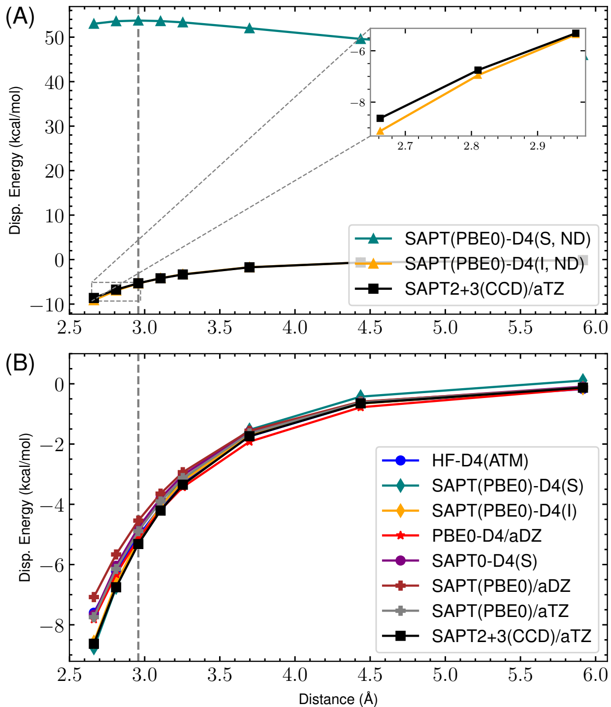
Figure 23: s66x8 31_Uracil-Ethene : Dispersion potential Energy curve for SAPT(PBE0) with aDZ/aTZ and -D4 variants versus the reference SAPT2+3(CCD)/aug-cc-pVTZ dispersion energy. (A) highlights the completely non-damped (ND) D4 curves compared to the reference for both supermolecular (S) and intermolecular (I). The remaining s_8 = 0.89529649 . (B) shows the damped -D4(S), -D4(I), HF-D4, SAPT(PBE0)/aDZ, SAPT(PBE0)/aTZ, and reference dispersion energies. Here, (S) and (I) refer to the supermolecular and intermolecular dispersion energy approaches, respectively. The “ND” states that no damping function is used. For the damped SAPT(PBE0)-D4(S) and SAPT(PBE0)-D4(I) terms, a_1 , a_2 , and s_8 are fit to the residual CCSD(T)/CBS energies on the 4470 dimer dataset.
