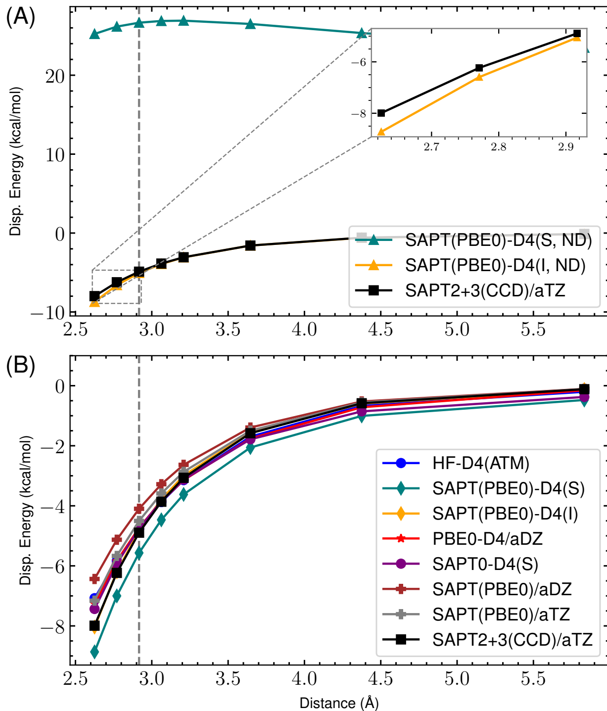
Figure 65: s66x8 32_Uracil-Ethyne : Dispersion potential Energy curve for SAPT(PBE0) with aDZ/aTZ and -D4 variants versus the reference SAPT2+3(CCD)/aug-cc-pVTZ dispersion energy. (A) highlights the completely non-damped (ND) D4 curves compared to the reference for both supermolecular (S) and intermolecular (I). The remaining s_8 = 0.89529649 . (B) shows the damped -D4(S), -D4(I), HF-D4, SAPT(PBE0)/aDZ, SAPT(PBE0)/aTZ, and reference dispersion energies. Here, (S) and (I) refer to the supermolecular and intermolecular dispersion energy approaches, respectively. The “ND” states that no damping function is used. For the damped SAPT(PBE0)-D4(S) and SAPT(PBE0)-D4(I) terms, a_1 , a_2 , and s_8 are fit to the residual CCSD(T)/CBS energies on the 4470 dimer dataset.
