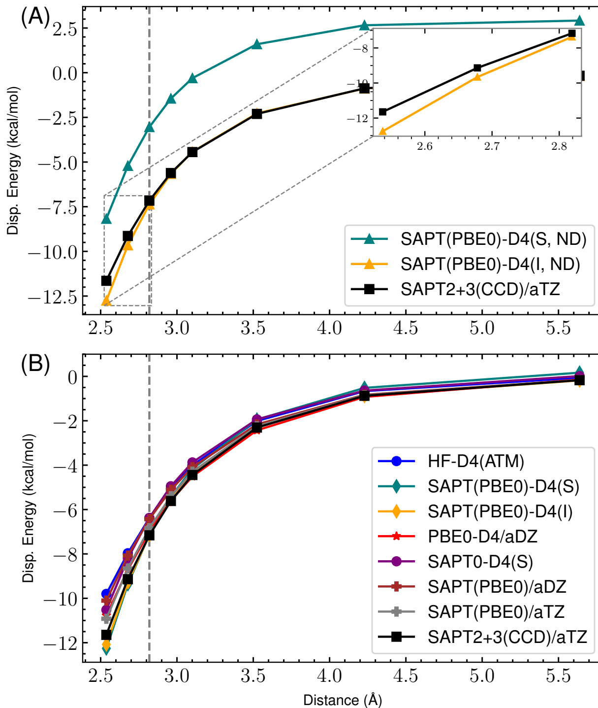
Figure 54: s66x8 39_Benzene-Cyclopentane : Dispersion potential Energy curve for SAPT(PBE0) with aDZ/aTZ and -D4 variants versus the reference SAPT2+3(CCD)/aug-cc-pVTZ dispersion energy. (A) highlights the completely non-damped (ND) D4 curves compared to the reference for both supermolecular (S) and intermolecular (I). The remaining s_8 = 0.89529649 . (B) shows the damped -D4(S), -D4(I), HF-D4, SAPT(PBE0)/aDZ, SAPT(PBE0)/aTZ, and reference dispersion energies. Here, (S) and (I) refer to the supermolecular and intermolecular dispersion energy approaches, respectively. The “ND” states that no damping function is used. For the damped SAPT(PBE0)-D4(S) and SAPT(PBE0)-D4(I) terms, a_1 , a_2 , and s_8 are fit to the residual CCSD(T)/CBS energies on the 4470 dimer dataset.
