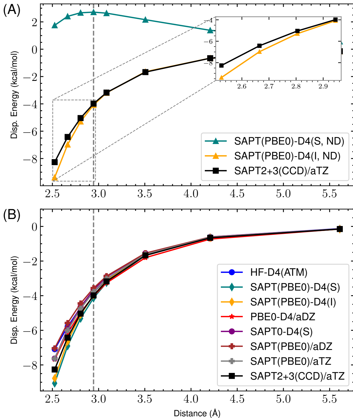
Figure 17: s66x8 47_Benzene-Benzene : Dispersion potential Energy curve for SAPT(PBE0) with aDZ/aTZ and -D4 variants versus the reference SAPT2+3(CCD)/aug-cc-pVTZ dispersion energy. (A) highlights the completely non-damped (ND) D4 curves compared to the reference for both supermolecular (S) and intermolecular (I). The remaining s_8 = 0.89529649 . (B) shows the damped -D4(S), -D4(I), HF-D4, SAPT(PBE0)/aDZ, SAPT(PBE0)/aTZ, and reference dispersion energies. Here, (S) and (I) refer to the supermolecular and intermolecular dispersion energy approaches, respectively. The “ND” states that no damping function is used. For the damped SAPT(PBE0)-D4(S) and SAPT(PBE0)-D4(I) terms, a_1 , a_2 , and s_8 are fit to the residual CCSD(T)/CBS energies on the 4470 dimer dataset.
