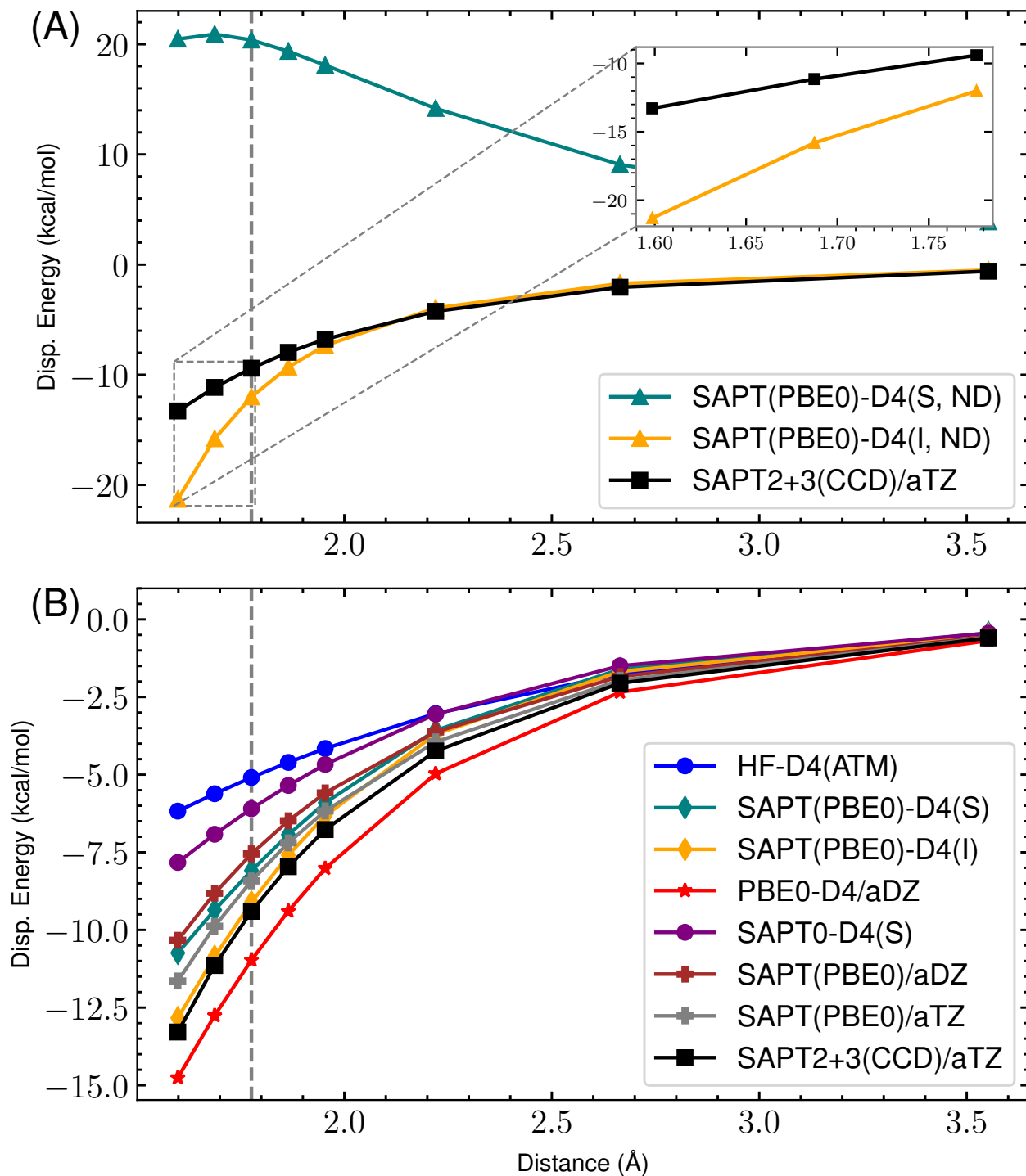
Figure 46: s66x8 17_Uracil-Uracil : Dispersion potential Energy curve for SAPT(PBE0) with aDZ/aTZ and -D4 variants versus the reference SAPT2+3(CCD)/aug-cc-pVTZ dispersion energy. (A) highlights the completely non-damped (ND) D4 curves compared to the reference for both supermolecular (S) and intermolecular (I). The remaining s_8 = 0.89529649 . (B) shows the damped -D4(S), -D4(I), HF-D4, SAPT(PBE0)/aDZ, SAPT(PBE0)/aTZ, and reference dispersion energies. Here, (S) and (I) refer to the supermolecular and intermolecular dispersion energy approaches, respectively. The “ND” states that no damping function is used. For the damped SAPT(PBE0)-D4(S) and SAPT(PBE0)-D4(I) terms, a_1 , a_2 , and s_8 are fit to the residual CCSD(T)/CBS energies on the 4470 dimer dataset.
