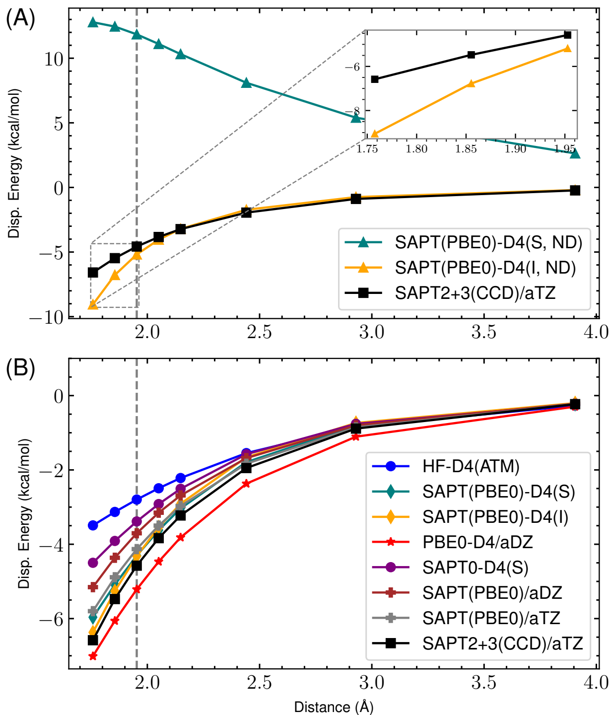
Figure 66: s66x8 19_MeOH-Pyridine : Dispersion potential Energy curve for SAPT(PBE0) with aDZ/aTZ and -D4 variants versus the reference SAPT2+3(CCD)/aug-cc-pVTZ dispersion energy. (A) highlights the completely non-damped (ND) D4 curves compared to the reference for both supermolecular (S) and intermolecular (I). The remaining s_8 = 0.89529649 . (B) shows the damped -D4(S), -D4(I), HF-D4, SAPT(PBE0)/aDZ, SAPT(PBE0)/aTZ, and reference dispersion energies. Here, (S) and (I) refer to the supermolecular and intermolecular dispersion energy approaches, respectively. The “ND” states that no damping function is used. For the damped SAPT(PBE0)-D4(S) and SAPT(PBE0)-D4(I) terms, a_1 , a_2 , and s_8 are fit to the residual CCSD(T)/CBS energies on the 4470 dimer dataset.
