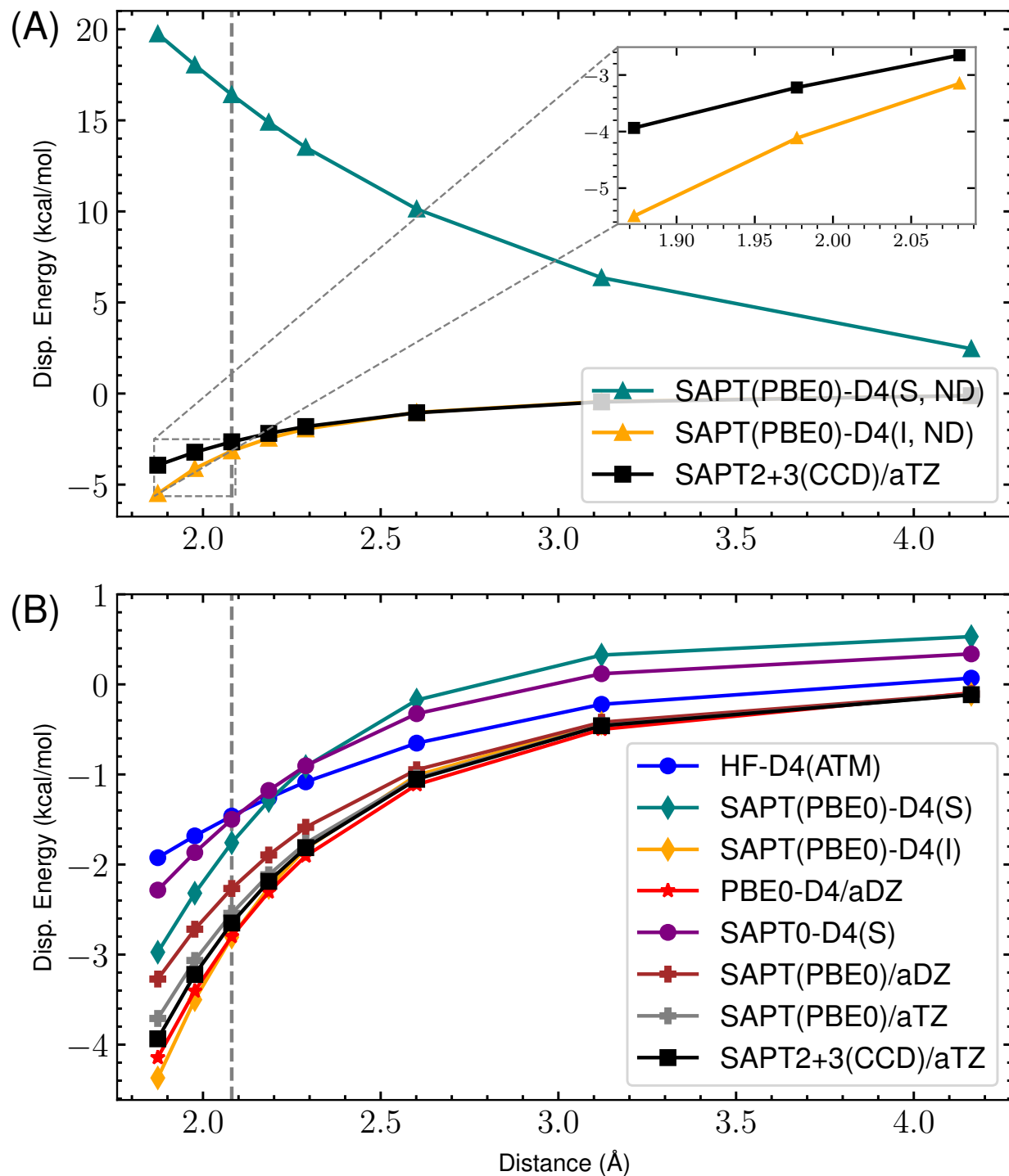
Figure 6: s66x8 16_Peptide-Water : Dispersion potential Energy curve for SAPT(PBE0) with aDZ/aTZ and -D4 variants versus the reference SAPT2+3(CCD)/aug-cc-pVTZ dispersion energy. (A) highlights the completely non-damped (ND) D4 curves compared to the reference for both supermolecular (S) and intermolecular (I). The remaining s_8 = 0.89529649 . (B) shows the damped -D4(S), -D4(I), HF-D4, SAPT(PBE0)/aDZ, SAPT(PBE0)/aTZ, and reference dispersion energies. Here, (S) and (I) refer to the supermolecular and intermolecular dispersion energy approaches, respectively. The “ND” states that no damping function is used. For the damped SAPT(PBE0)-D4(S) and SAPT(PBE0)-D4(I) terms, a_1 , a_2 , and s_8 are fit to the residual CCSD(T)/CBS energies on the 4470 dimer dataset.
