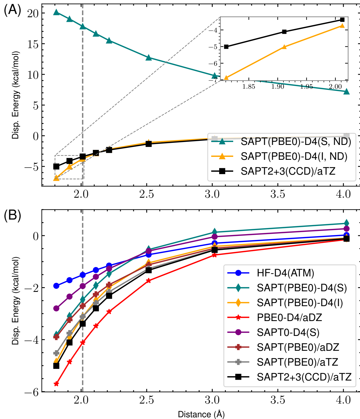
Figure 41: s66x8 03_Water-MeNH 2 : Dispersion potential Energy curve for SAPT(PBE0) with aDZ/aTZ and -D4 variants versus the reference SAPT2+3(CCD)/aug-cc-pVTZ dispersion energy. (A) highlights the completely non-damped (ND) D4 curves compared to the reference for both supermolecular (S) and intermolecular (I). The remaining s_8 = 0.89529649 . (B) shows the damped -D4(S), -D4(I), HF-D4, SAPT(PBE0)/aDZ, SAPT(PBE0)/aTZ, and reference dispersion energies. Here, (S) and (I) refer to the supermolecular and intermolecular dispersion energy approaches, respectively. The “ND” states that no damping function is used. For the damped SAPT(PBE0)-D4(S) and SAPT(PBE0)-D4(I) terms, a_1 , a_2 , and s_8 are fit to the residual CCSD(T)/CBS energies on the 4470 dimer dataset.
