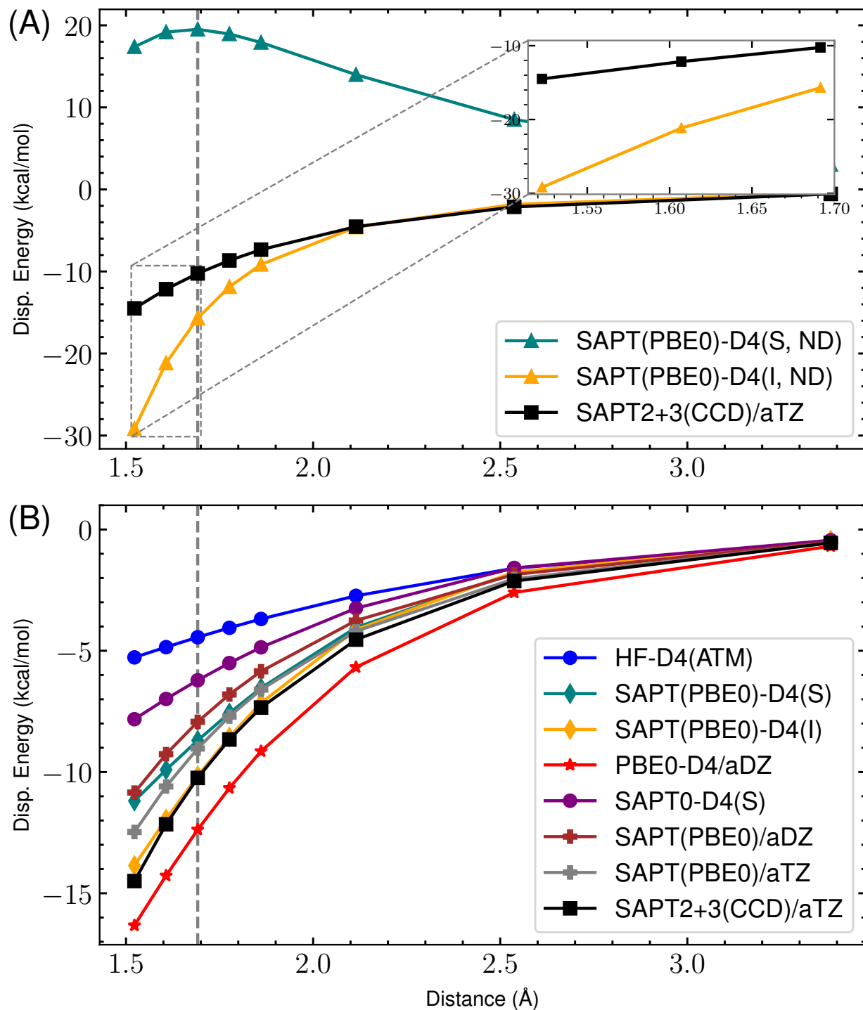
Figure 34: s66x8 20_AcOH-AcOH: Dispersion potential Energy curve for SAPT(PBE0) with aDZ/aTZ and -D4 variants versus the reference SAPT2+3(CCD)/aug-cc-pVTZ dispersion energy. (A) highlights the completely non-damped (ND) D4 curves compared to the reference for both supermolecular (S) and intermolecular (I). The remaining s_8 = 0.89529649 . (B) shows the damped -D4(S), -D4(I), HF-D4, SAPT(PBE0)/aDZ, SAPT(PBE0)/aTZ, and reference dispersion energies. Here, (S) and (I) refer to the supermolecular and intermolecular dispersion energy approaches, respectively. The “ND” states that no damping function is used. For the damped SAPT(PBE0)-D4(S) and SAPT(PBE0)-D4(I) terms, a_1 , a_2 , and s_8 are fit to the residual CCSD(T)/CBS energies on the 4470 dimer dataset.
