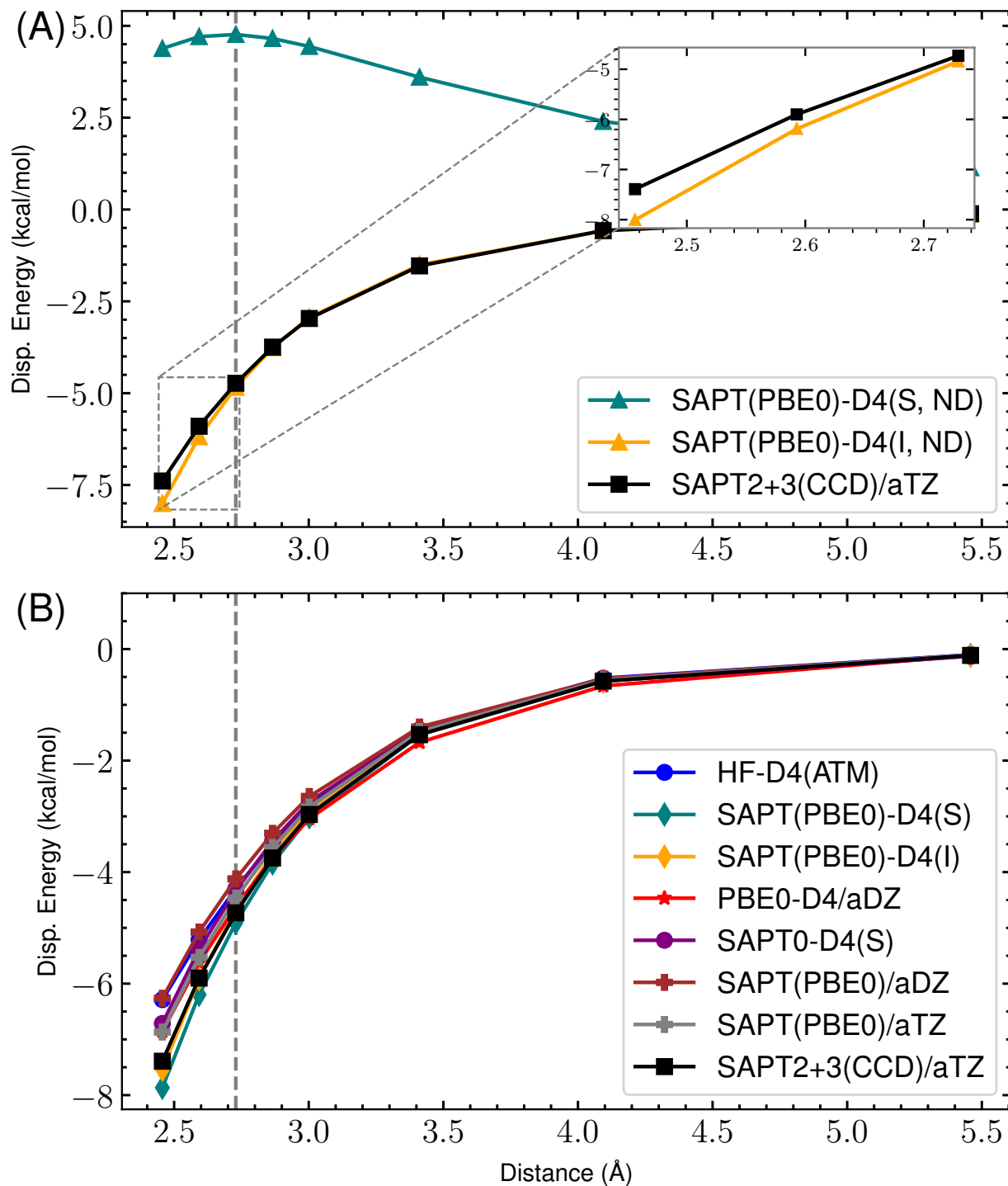
Figure 44: s66x8 56_Benzene-MeNH 2 : Dispersion potential Energy curve for SAPT(PBE0) with aDZ/aTZ and -D4 variants versus the reference SAPT2+3(CCD)/aug-cc-pVTZ dispersion energy. (A) highlights the completely non-damped (ND) D4 curves compared to the reference for both supermolecular (S) and intermolecular (I). The remaining s_8 = 0.89529649 . (B) shows the damped -D4(S), -D4(I), HF-D4, SAPT(PBE0)/aDZ, SAPT(PBE0)/aTZ, and reference dispersion energies. Here, (S) and (I) refer to the supermolecular and intermolecular dispersion energy approaches, respectively. The “ND” states that no damping function is used. For the damped SAPT(PBE0)-D4(S) and SAPT(PBE0)-D4(I) terms, a_1 , a_2 , and s_8 are fit to the residual CCSD(T)/CBS energies on the 4470 dimer dataset.
