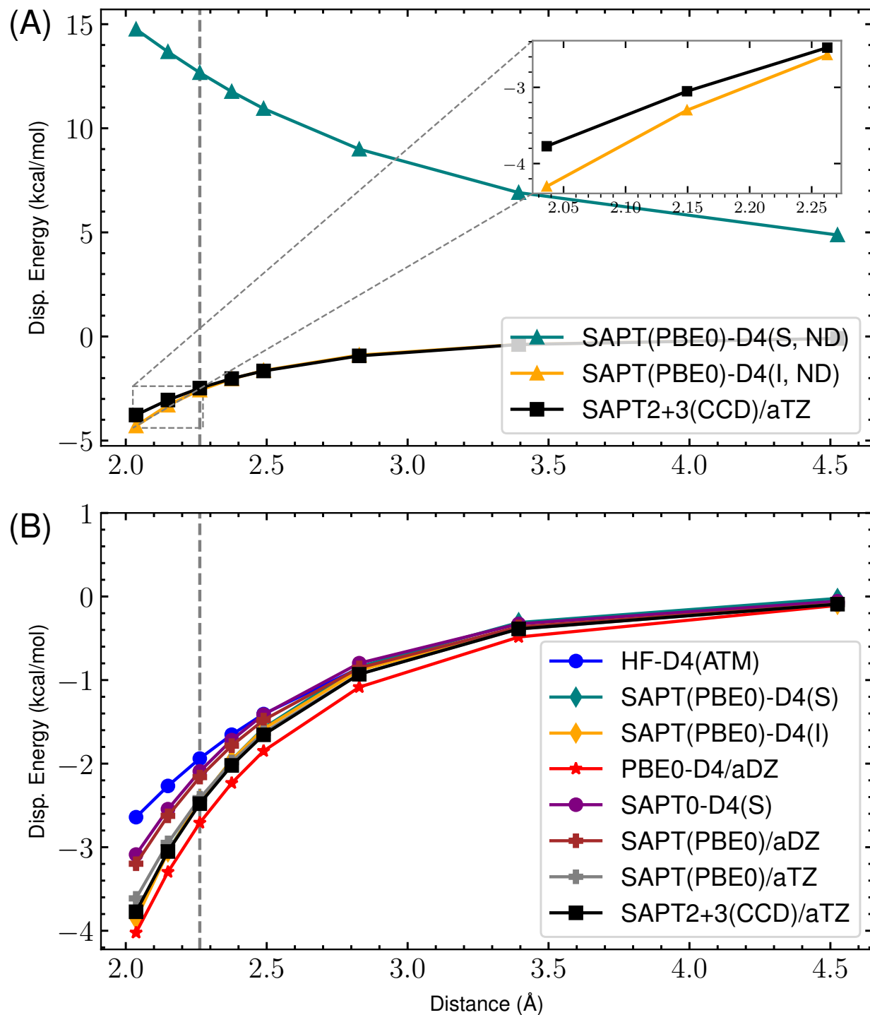
Figure 42: s66x8 09_MeNH 2 -MeOH : Dispersion potential Energy curve for SAPT(PBE0) with aDZ/aTZ and -D4 variants versus the reference SAPT2+3(CCD)/aug-cc-pVTZ dispersion energy. (A) highlights the completely non-damped (ND) D4 curves compared to the reference for both supermolecular (S) and intermolecular (I). The remaining s_8 = 0.89529649 . (B) shows the damped -D4(S), -D4(I), HF-D4, SAPT(PBE0)/aDZ, SAPT(PBE0)/aTZ, and reference dispersion energies. Here, (S) and (I) refer to the supermolecular and intermolecular dispersion energy approaches, respectively. The “ND” states that no damping function is used. For the damped SAPT(PBE0)-D4(S) and SAPT(PBE0)-D4(I) terms, a_1 , a_2 , and s_8 are fit to the residual CCSD(T)/CBS energies on the 4470 dimer dataset.
