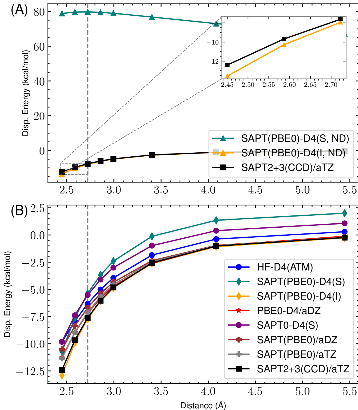
Figure 29: s66x8 42_Uracil-Cyclopentane : Dispersion potential Energy curve for SAPT(PBE0) with aDZ/aTZ and -D4 variants versus the reference SAPT2+3(CCD)/aug-cc-pVTZ dispersion energy. (A) highlights the completely non-damped (ND) D4 curves compared to the reference for both supermolecular (S) and intermolecular (I). The remaining s_8 = 0.89529649 . (B) shows the damped -D4(S), -D4(I), HF-D4, SAPT(PBE0)/aDZ, SAPT(PBE0)/aTZ, and reference dispersion energies. Here, (S) and (I) refer to the supermolecular and intermolecular dispersion energy approaches, respectively. The “ND” states that no damping function is used. For the damped SAPT(PBE0)-D4(S) and SAPT(PBE0)-D4(I) terms, a_1 , a_2 , and s_8 are fit to the residual CCSD(T)/CBS energies on the 4470 dimer dataset.
