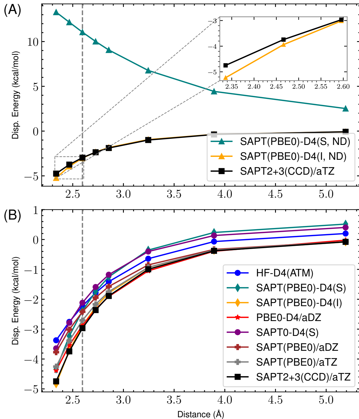
Figure 13: s66x8 54_Benzene-Water : Dispersion potential Energy curve for SAPT(PBE0) with aDZ/aTZ and -D4 variants versus the reference SAPT2+3(CCD)/aug-cc-pVTZ dispersion energy. (A) highlights the completely non-damped (ND) D4 curves compared to the reference for both supermolecular (S) and intermolecular (I). The remaining s_8 = 0.89529649 . (B) shows the damped -D4(S), -D4(I), HF-D4, SAPT(PBE0)/aDZ, SAPT(PBE0)/aTZ, and reference dispersion energies. Here, (S) and (I) refer to the supermolecular and intermolecular dispersion energy approaches, respectively. The “ND” states that no damping function is used. For the damped SAPT(PBE0)-D4(S) and SAPT(PBE0)-D4(I) terms, a_1 , a_2 , and s_8 are fit to the residual CCSD(T)/CBS energies on the 4470 dimer dataset.
