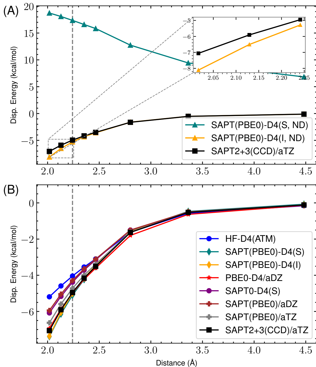
Figure 52: s66x8 11_MeNH2-Peptide : Dispersion potential Energy curve for SAPT(PBE0) with aDZ/aTZ and -D4 variants versus the reference SAPT2+3(CCD)/aug-cc-pVTZ dispersion energy. (A) highlights the completely non-damped (ND) D4 curves compared to the reference for both supermolecular (S) and intermolecular (I). The remaining s_8 = 0.89529649 . (B) shows the damped -D4(S), -D4(I), HF-D4, SAPT(PBE0)/aDZ, SAPT(PBE0)/aTZ, and reference dispersion energies. Here, (S) and (I) refer to the supermolecular and intermolecular dispersion energy approaches, respectively. The “ND” states that no damping function is used. For the damped SAPT(PBE0)-D4(S) and SAPT(PBE0)-D4(I) terms, a_1 , a_2 , and s_8 are fit to the residual CCSD(T)/CBS energies on the 4470 dimer dataset.
