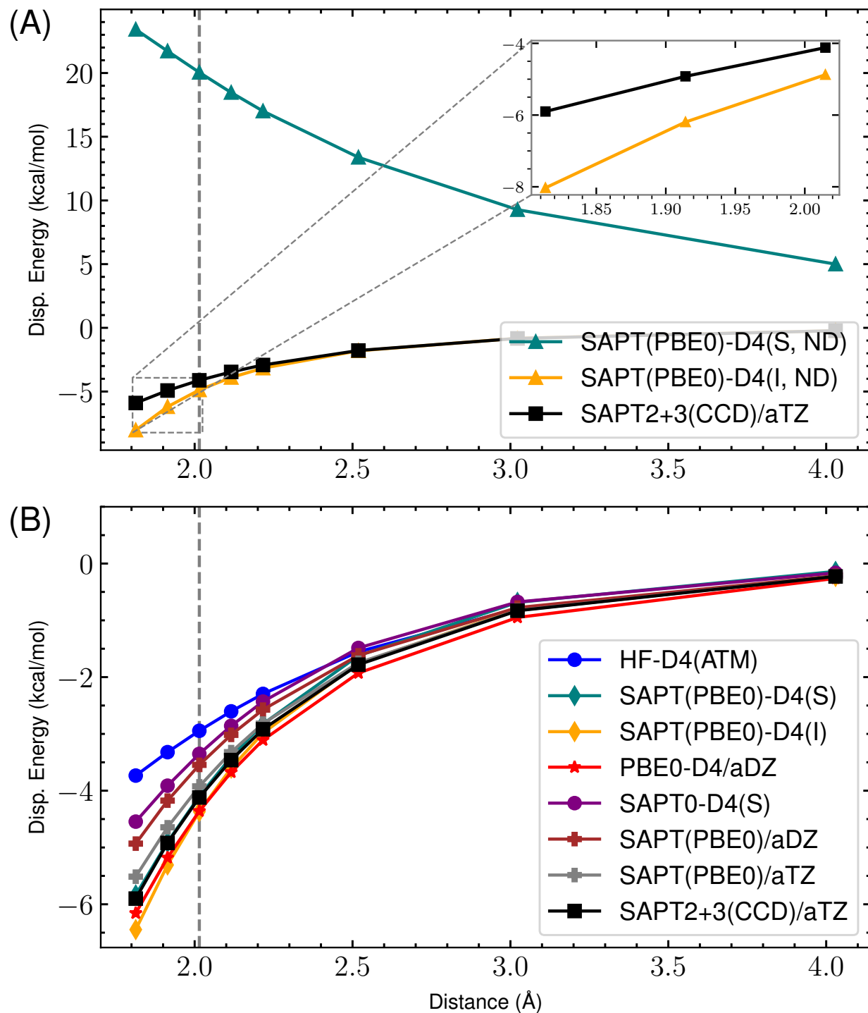
Figure 56: s66x8 13_Peptide-MeOH : Dispersion potential Energy curve for SAPT(PBE0) with aDZ/aTZ and -D4 variants versus the reference SAPT2+3(CCD)/aug-cc-pVTZ dispersion energy. (A) highlights the completely non-damped (ND) D4 curves compared to the reference for both supermolecular (S) and intermolecular (I). The remaining s_8 = 0.89529649 . (B) shows the damped -D4(S), -D4(I), HF-D4, SAPT(PBE0)/aDZ, SAPT(PBE0)/aTZ, and reference dispersion energies. Here, (S) and (I) refer to the supermolecular and intermolecular dispersion energy approaches, respectively. The “ND” states that no damping function is used. For the damped SAPT(PBE0)-D4(S) and SAPT(PBE0)-D4(I) terms, a_1 , a_2 , and s_8 are fit to the residual CCSD(T)/CBS energies on the 4470 dimer dataset.
