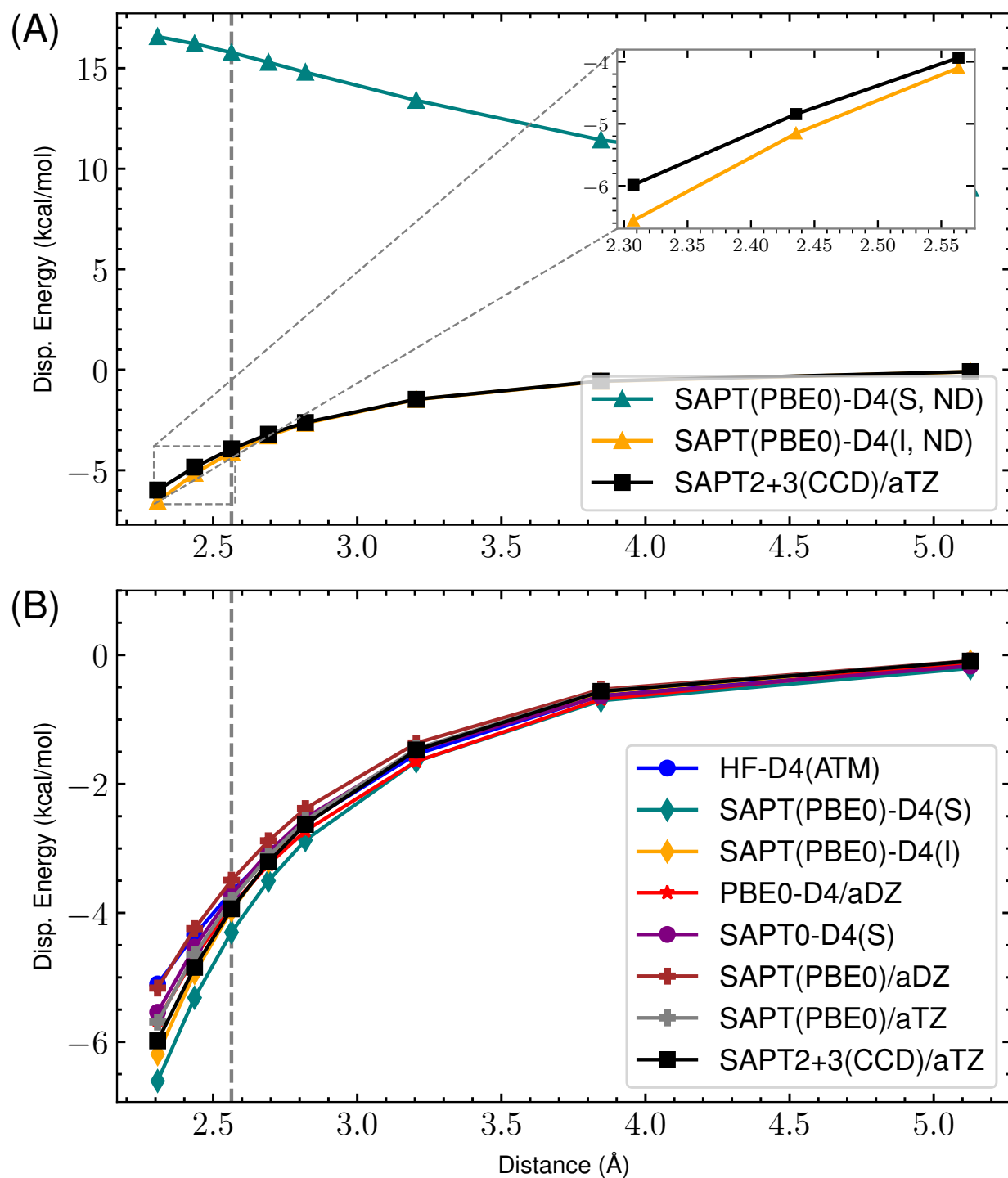
Figure 31: s66x8 64_Peptide-Ethene : Dispersion potential Energy curve for SAPT(PBE0) with aDZ/aTZ and -D4 variants versus the reference SAPT2+3(CCD)/aug-cc-pVTZ dispersion energy. (A) highlights the completely non-damped (ND) D4 curves compared to the reference for both supermolecular (S) and intermolecular (I). The remaining s_8 = 0.89529649 . (B) shows the damped -D4(S), -D4(I), HF-D4, SAPT(PBE0)/aDZ, SAPT(PBE0)/aTZ, and reference dispersion energies. Here, (S) and (I) refer to the supermolecular and intermolecular dispersion energy approaches, respectively. The “ND” states that no damping function is used. For the damped SAPT(PBE0)-D4(S) and SAPT(PBE0)-D4(I) terms, a_1 , a_2 , and s_8 are fit to the residual CCSD(T)/CBS energies on the 4470 dimer dataset.
