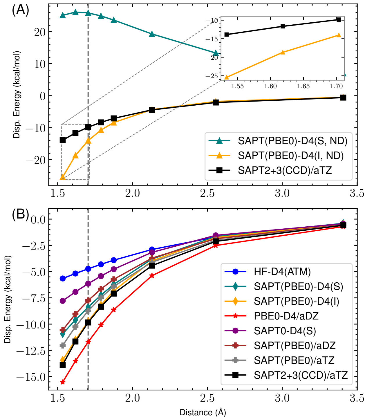
Figure 15: s66x8 22_AcOH-Uracil : Dispersion potential Energy curve for SAPT(PBE0) with aDZ/aTZ and -D4 variants versus the reference SAPT2+3(CCD)/aug-cc-pVTZ dispersion energy. (A) highlights the completely non-damped (ND) D4 curves compared to the reference for both supermolecular (S) and intermolecular (I). The remaining s_8 = 0.89529649 . (B) shows the damped -D4(S), -D4(I), HF-D4, SAPT(PBE0)/aDZ, SAPT(PBE0)/aTZ, and reference dispersion energies. Here, (S) and (I) refer to the supermolecular and intermolecular dispersion energy approaches, respectively. The “ND” states that no damping function is used. For the damped SAPT(PBE0)-D4(S) and SAPT(PBE0)-D4(I) terms, a_1 , a_2 , and s_8 are fit to the residual CCSD(T)/CBS energies on the 4470 dimer dataset.
