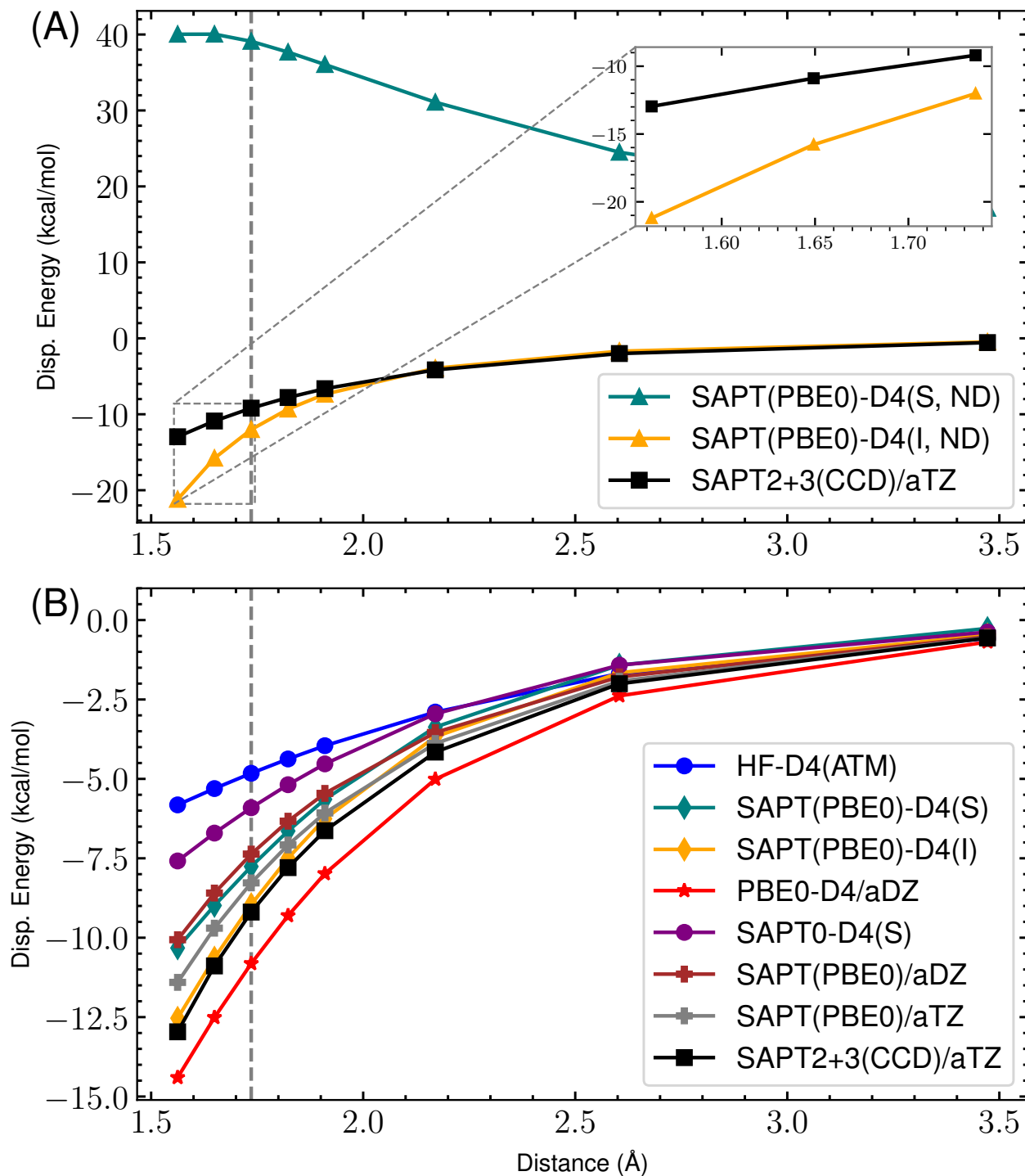
Figure 26: s66x8 23_AcNH2-Uracil : Dispersion potential Energy curve for SAPT(PBE0) with aDZ/aTZ and -D4 variants versus the reference SAPT2+3(CCD)/aug-cc-pVTZ dispersion energy. (A) highlights the completely non-damped (ND) D4 curves compared to the reference for both supermolecular (S) and intermolecular (I). The remaining s_8 = 0.89529649 . (B) shows the damped -D4(S), -D4(I), HF-D4, SAPT(PBE0)/aDZ, SAPT(PBE0)/aTZ, and reference dispersion energies. Here, (S) and (I) refer to the supermolecular and intermolecular dispersion energy approaches, respectively. The “ND” states that no damping function is used. For the damped SAPT(PBE0)-D4(S) and SAPT(PBE0)-D4(I) terms, a_1 , a_2 , and s_8 are fit to the residual CCSD(T)/CBS energies on the 4470 dimer dataset.
