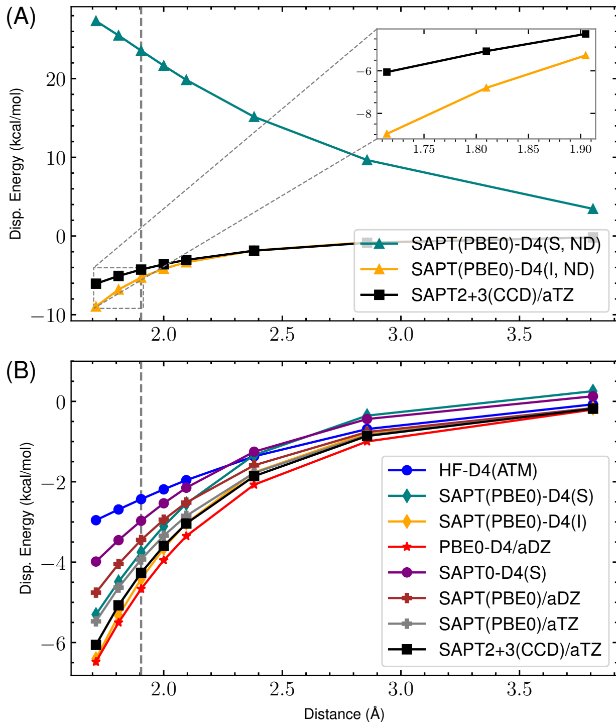
Figure 25: s66x8 04_Water-Peptide : Dispersion potential Energy curve for SAPT(PBE0) with aDZ/aTZ and -D4 variants versus the reference SAPT2+3(CCD)/aug-cc-pVTZ dispersion energy. (A) highlights the completely non-damped (ND) D4 curves compared to the reference for both supermolecular (S) and intermolecular (I). The remaining s_8 = 0.89529649 . (B) shows the damped -D4(S), -D4(I), HF-D4, SAPT(PBE0)/aDZ, SAPT(PBE0)/aTZ, and reference dispersion energies. Here, (S) and (I) refer to the supermolecular and intermolecular dispersion energy approaches, respectively. The “ND” states that no damping function is used. For the damped SAPT(PBE0)-D4(S) and SAPT(PBE0)-D4(I) terms, a_1 , a_2 , and s_8 are fit to the residual CCSD(T)/CBS energies on the 4470 dimer dataset.
