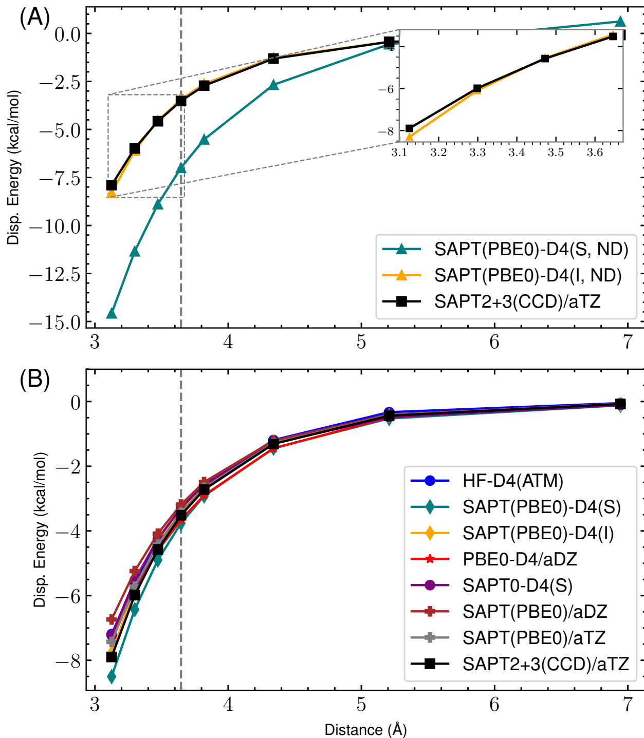
Figure 43: s66x8 30_Benzene-Ethene : Dispersion potential Energy curve for SAPT(PBE0) with aDZ/aTZ and -D4 variants versus the reference SAPT2+3(CCD)/aug-cc-pVTZ dispersion energy. (A) highlights the completely non-damped (ND) D4 curves compared to the reference for both supermolecular (S) and intermolecular (I). The remaining s_8 = 0.89529649 . (B) shows the damped -D4(S), -D4(I), HF-D4, SAPT(PBE0)/aDZ, SAPT(PBE0)/aTZ, and reference dispersion energies. Here, (S) and (I) refer to the supermolecular and intermolecular dispersion energy approaches, respectively. The “ND” states that no damping function is used. For the damped SAPT(PBE0)-D4(S) and SAPT(PBE0)-D4(I) terms, a_1 , a_2 , and s_8 are fit to the residual CCSD(T)/CBS energies on the 4470 dimer dataset.
