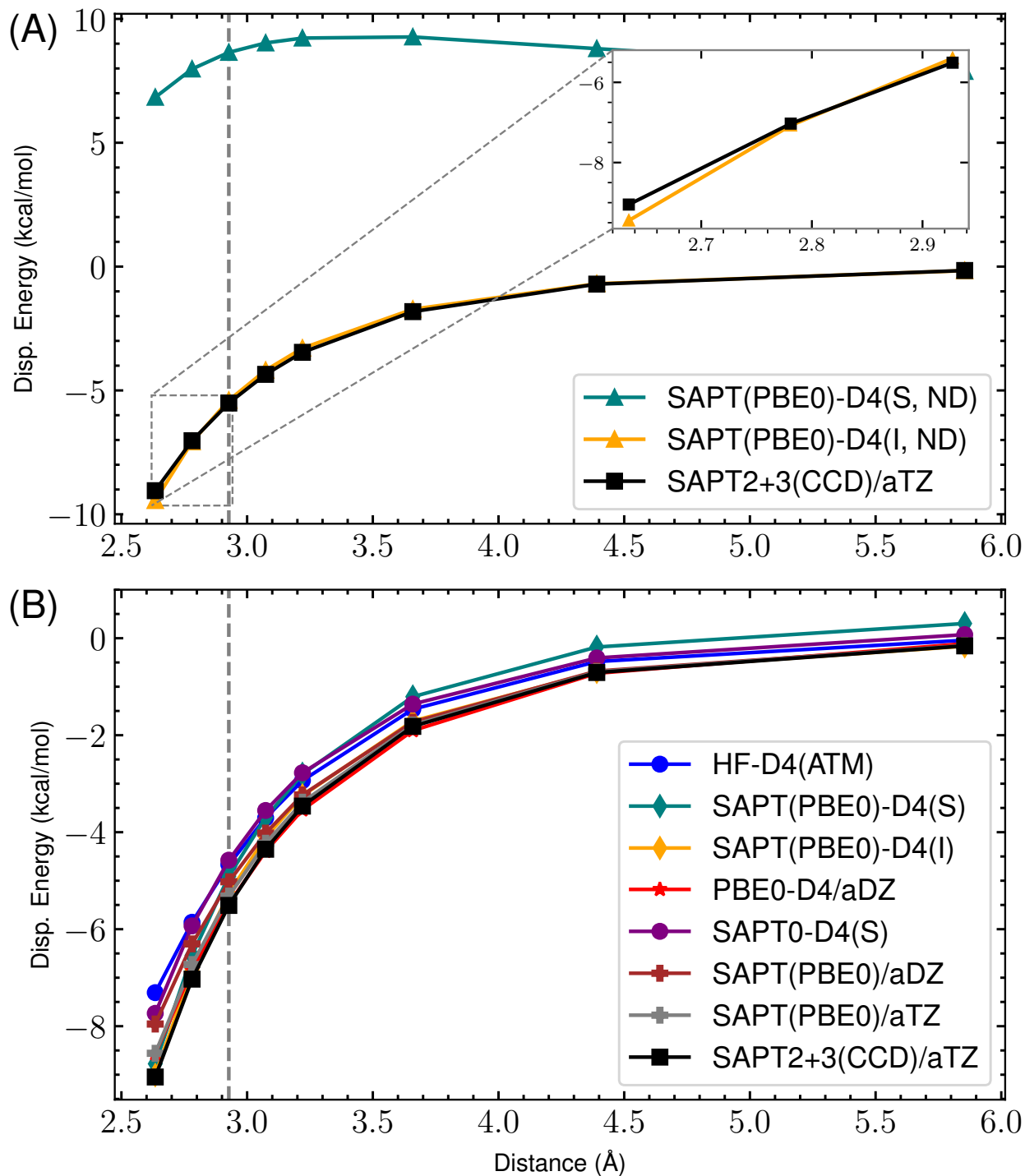
Figure 59: s66x8 40_Benzene-Neopentane : Dispersion potential Energy curve for SAPT(PBE0) with aDZ/aTZ and -D4 variants versus the reference SAPT2+3(CCD)/aug-cc-pVTZ dispersion energy. (A) highlights the completely non-damped (ND) D4 curves compared to the reference for both supermolecular (S) and intermolecular (I). The remaining s_8 = 0.89529649 . (B) shows the damped -D4(S), -D4(I), HF-D4, SAPT(PBE0)/aDZ, SAPT(PBE0)/aTZ, and reference dispersion energies. Here, (S) and (I) refer to the supermolecular and intermolecular dispersion energy approaches, respectively. The “ND” states that no damping function is used. For the damped SAPT(PBE0)-D4(S) and SAPT(PBE0)-D4(I) terms, a_1 , a_2 , and s_8 are fit to the residual CCSD(T)/CBS energies on the 4470 dimer dataset.
