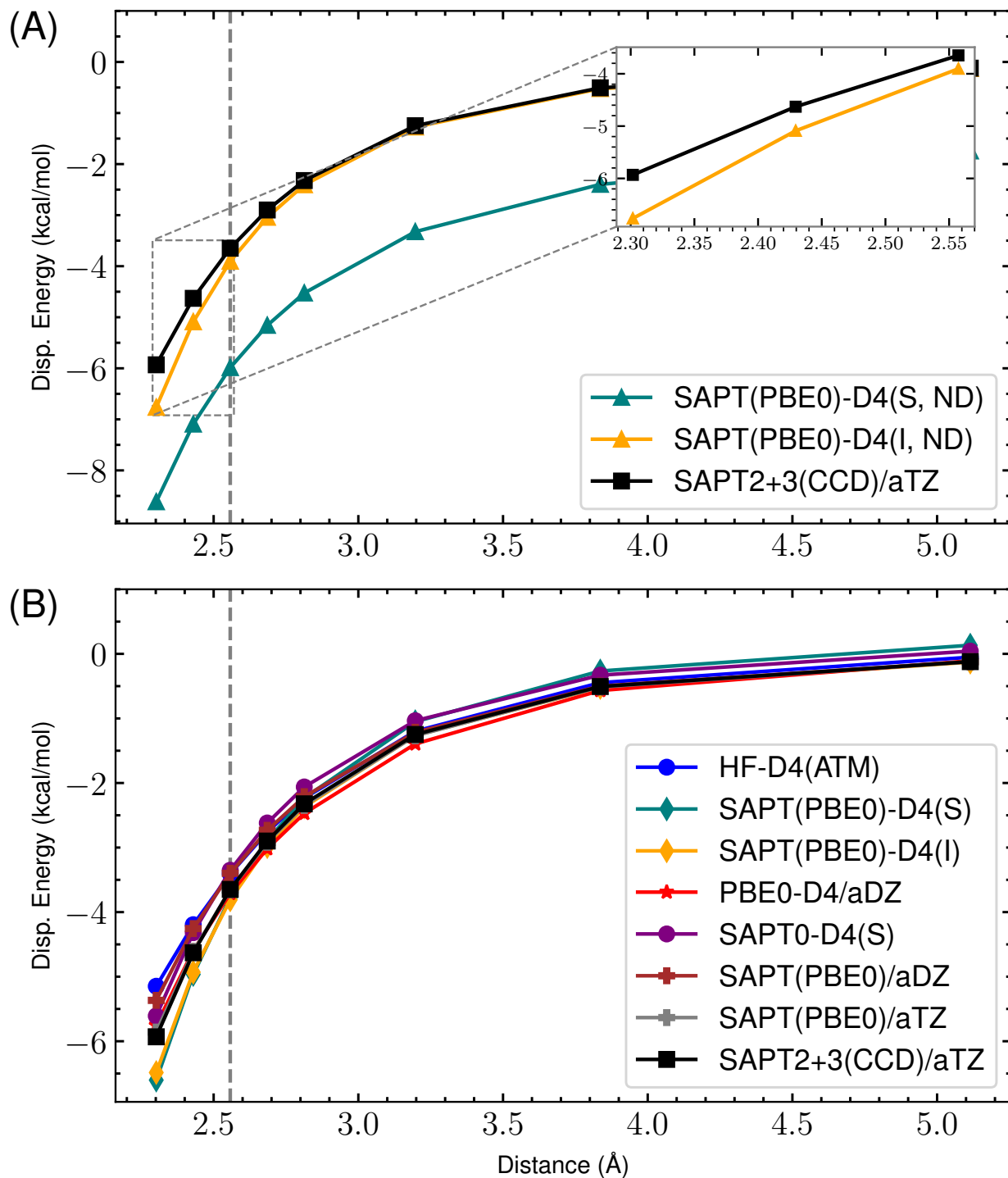
Figure 7: s66x8 44_Ethene-Pentane : Dispersion potential Energy curve for SAPT(PBE0) with aDZ/aTZ and -D4 variants versus the reference SAPT2+3(CCD)/aug-cc-pVTZ dispersion energy. (A) highlights the completely non-damped (ND) D4 curves compared to the reference for both supermolecular (S) and intermolecular (I). The remaining s_8 = 0.89529649 . (B) shows the damped -D4(S), -D4(I), HF-D4, SAPT(PBE0)/aDZ, SAPT(PBE0)/aTZ, and reference dispersion energies. Here, (S) and (I) refer to the supermolecular and intermolecular dispersion energy approaches, respectively. The “ND” states that no damping function is used. For the damped SAPT(PBE0)-D4(S) and SAPT(PBE0)-D4(I) terms, a_1 , a_2 , and s_8 are fit to the residual CCSD(T)/CBS energies on the 4470 dimer dataset.
