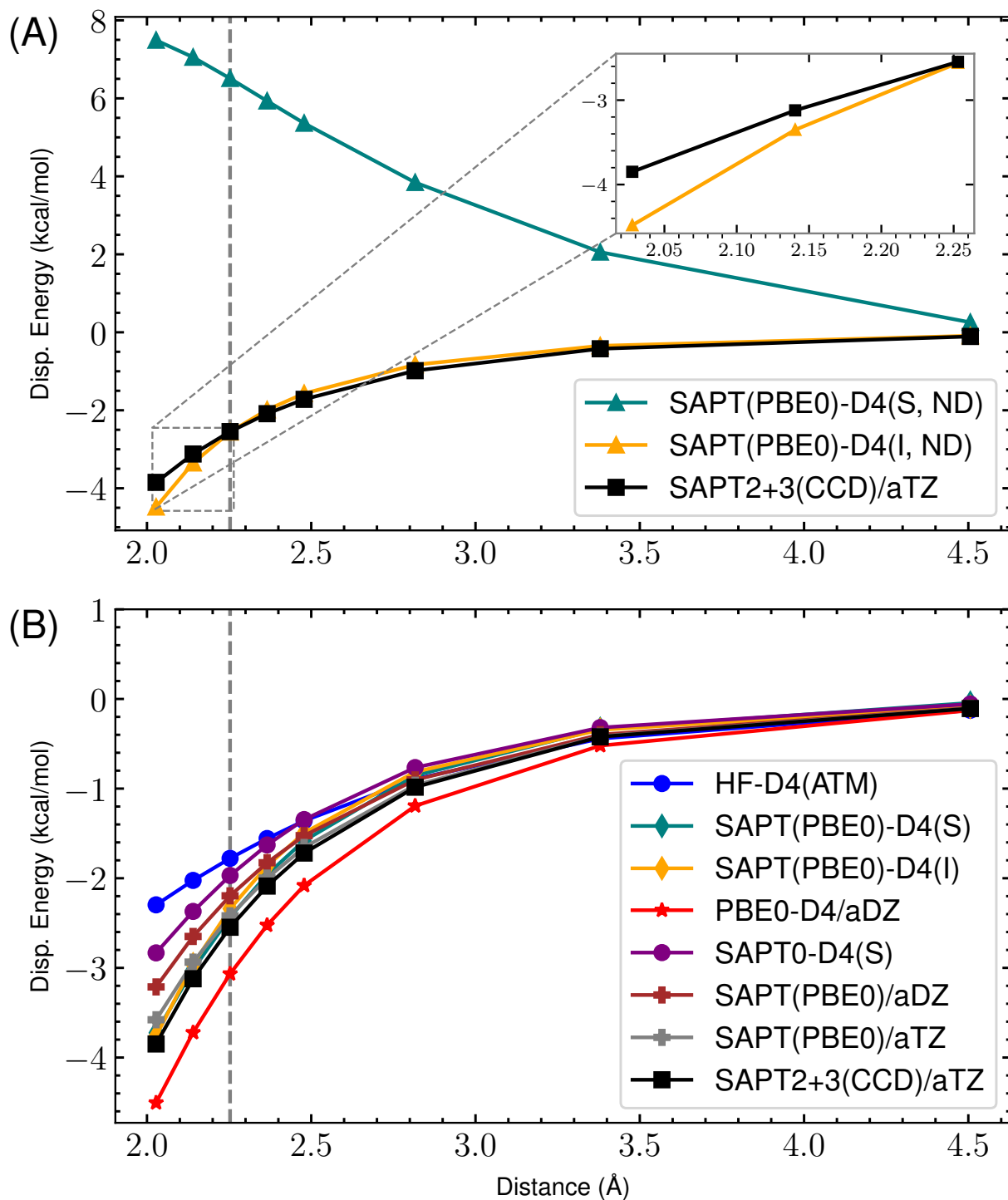
Figure 16: s66x8 65_Pyridine-Ethyne : Dispersion potential Energy curve for SAPT(PBE0) with aDZ/aTZ and -D4 variants versus the reference SAPT2+3(CCD)/aug-cc-pVTZ dispersion energy. (A) highlights the completely non-damped (ND) D4 curves compared to the reference for both supermolecular (S) and intermolecular (I). The remaining s_8 = 0.89529649 . (B) shows the damped -D4(S), -D4(I), HF-D4, SAPT(PBE0)/aDZ, SAPT(PBE0)/aTZ, and reference dispersion energies. Here, (S) and (I) refer to the supermolecular and intermolecular dispersion energy approaches, respectively. The “ND” states that no damping function is used. For the damped SAPT(PBE0)-D4(S) and SAPT(PBE0)-D4(I) terms, a_1 , a_2 , and s_8 are fit to the residual CCSD(T)/CBS energies on the 4470 dimer dataset.
