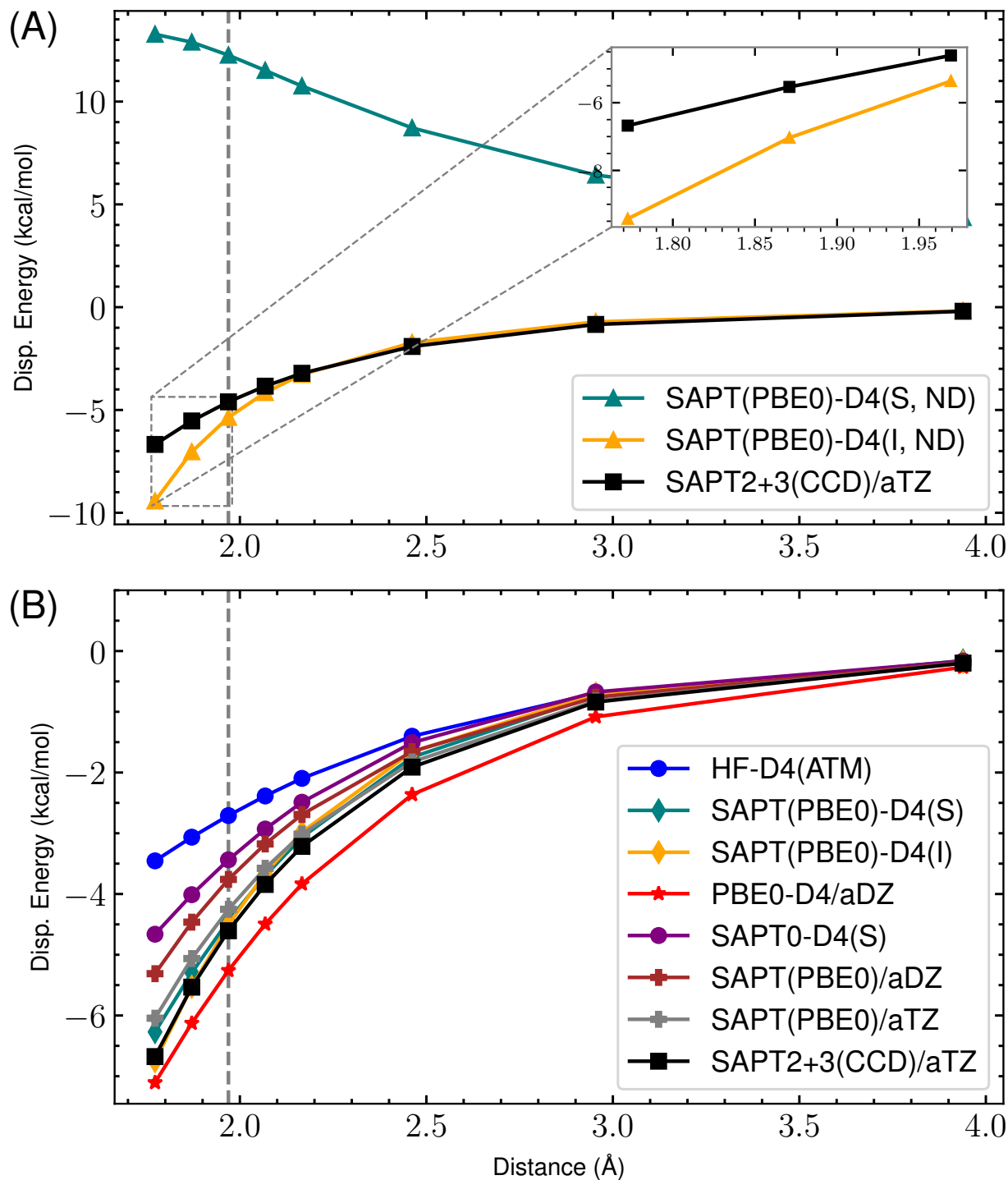
Figure 48: s66x8 06_MeOH-MeNH2 : Dispersion potential Energy curve for SAPT(PBE0) with aDZ/aTZ and -D4 variants versus the reference SAPT2+3(CCD)/aug-cc-pVTZ dispersion energy. (A) highlights the completely non-damped (ND) D4 curves compared to the reference for both supermolecular (S) and intermolecular (I). The remaining s_8 = 0.89529649 . (B) shows the damped -D4(S), -D4(I), HF-D4, SAPT(PBE0)/aDZ, SAPT(PBE0)/aTZ, and reference dispersion energies. Here, (S) and (I) refer to the supermolecular and intermolecular dispersion energy approaches, respectively. The “ND” states that no damping function is used. For the damped SAPT(PBE0)-D4(S) and SAPT(PBE0)-D4(I) terms, a_1 , a_2 , and s_8 are fit to the residual CCSD(T)/CBS energies on the 4470 dimer dataset.
