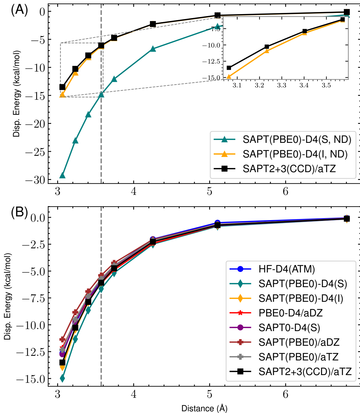
Figure 37: s66x8 24_Benzene-Benzene : Dispersion potential Energy curve for SAPT(PBE0) with aDZ/aTZ and -D4 variants versus the reference SAPT2+3(CCD)/aug-cc-pVTZ dispersion energy. (A) highlights the completely non-damped (ND) D4 curves compared to the reference for both supermolecular (S) and intermolecular (I). The remaining s_8 = 0.89529649 . (B) shows the damped -D4(S), -D4(I), HF-D4, SAPT(PBE0)/aDZ, SAPT(PBE0)/aTZ, and reference dispersion energies. Here, (S) and (I) refer to the supermolecular and intermolecular dispersion energy approaches, respectively. The “ND” states that no damping function is used. For the damped SAPT(PBE0)-D4(S) and SAPT(PBE0)-D4(I) terms, a_1 , a_2 , and s_8 are fit to the residual CCSD(T)/CBS energies on the 4470 dimer dataset.
