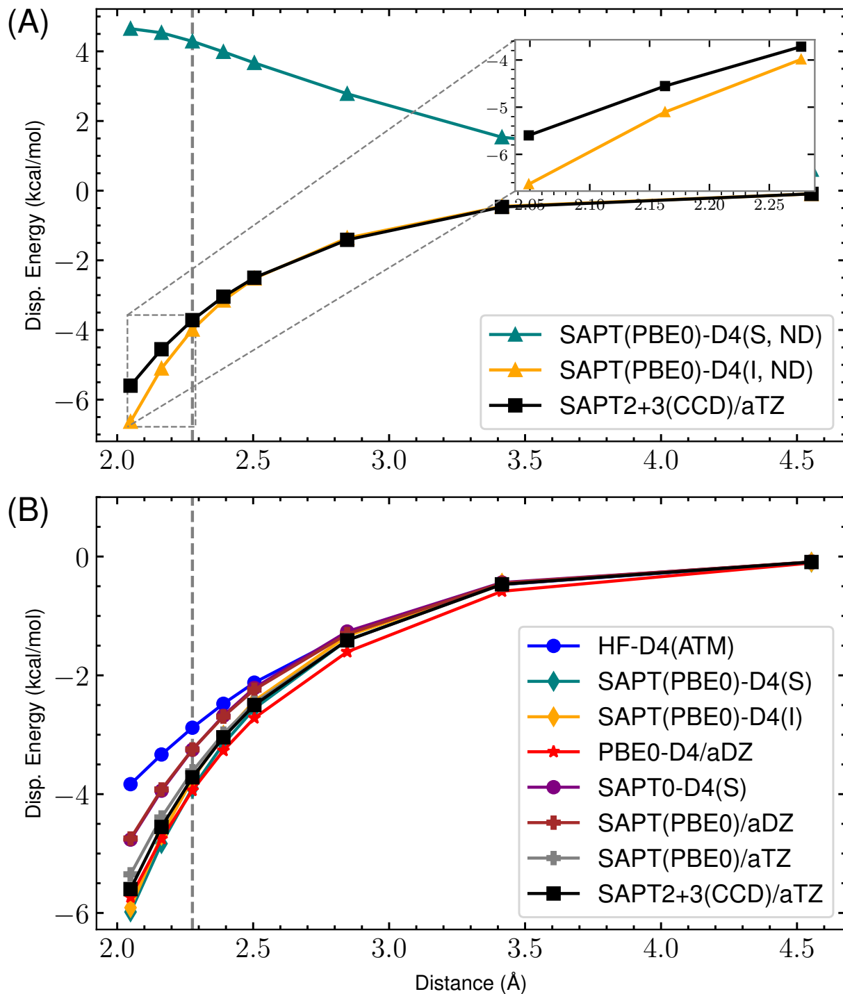
Figure 5: s66x8 10_MeNH 2 -MeNH 2 : Dispersion potential Energy curve for SAPT(PBE0) with aDZ/aTZ and -D4 variants versus the reference SAPT2+3(CCD)/aug-cc-pVTZ dispersion energy. (A) highlights the completely non-damped (ND) D4 curves compared to the reference for both supermolecular (S) and intermolecular (I). The remaining s_8 = 0.89529649 . (B) shows the damped -D4(S), -D4(I), HF-D4, SAPT(PBE0)/aDZ, SAPT(PBE0)/aTZ, and reference dispersion energies. Here, (S) and (I) refer to the supermolecular and intermolecular dispersion energy approaches, respectively. The “ND” states that no damping function is used. For the damped SAPT(PBE0)-D4(S) and SAPT(PBE0)-D4(I) terms, a_1 , a_2 , and s_8 are fit to the residual CCSD(T)/CBS energies on the 4470 dimer dataset.
