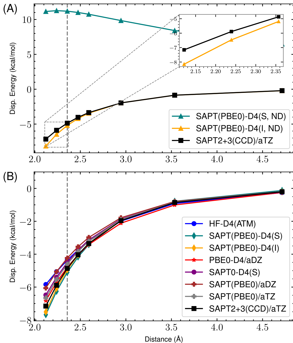
Figure 38: s66x8 66_MeNH2-Pyridine : Dispersion potential Energy curve for SAPT(PBE0) with aDZ/aTZ and -D4 variants versus the reference SAPT2+3(CCD)/aug-cc-pVTZ dispersion energy. (A) highlights the completely non-damped (ND) D4 curves compared to the reference for both supermolecular (S) and intermolecular (I). The remaining s_8 = 0.89529649 . (B) shows the damped -D4(S), -D4(I), HF-D4, SAPT(PBE0)/aDZ, SAPT(PBE0)/aTZ, and reference dispersion energies. Here, (S) and (I) refer to the supermolecular and intermolecular dispersion energy approaches, respectively. The “ND” states that no damping function is used. For the damped SAPT(PBE0)-D4(S) and SAPT(PBE0)-D4(I) terms, a_1 , a_2 , and s_8 are fit to the residual CCSD(T)/CBS energies on the 4470 dimer dataset.
