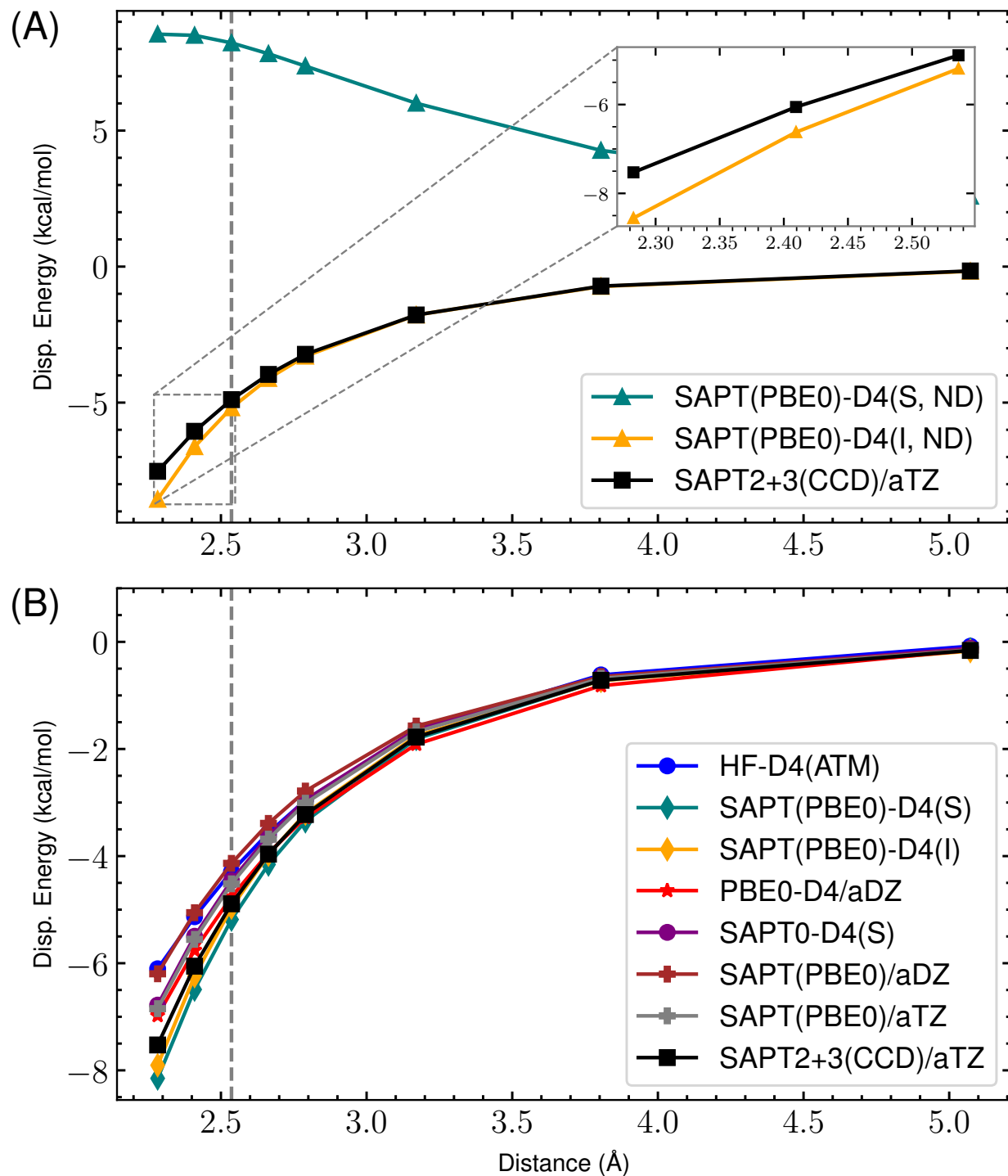
Figure 19: s66x8 55_Benzene-MeOH : Dispersion potential Energy curve for SAPT(PBE0) with aDZ/aTZ and -D4 variants versus the reference SAPT2+3(CCD)/aug-cc-pVTZ dispersion energy. (A) highlights the completely non-damped (ND) D4 curves compared to the reference for both supermolecular (S) and intermolecular (I). The remaining s_8 = 0.89529649 . (B) shows the damped -D4(S), -D4(I), HF-D4, SAPT(PBE0)/aDZ, SAPT(PBE0)/aTZ, and reference dispersion energies. Here, (S) and (I) refer to the supermolecular and intermolecular dispersion energy approaches, respectively. The “ND” states that no damping function is used. For the damped SAPT(PBE0)-D4(S) and SAPT(PBE0)-D4(I) terms, a_1 , a_2 , and s_8 are fit to the residual CCSD(T)/CBS energies on the 4470 dimer dataset.
