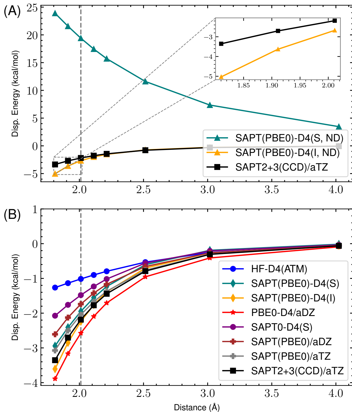
Figure 22: s66x8 01_Water-Water : Dispersion potential Energy curve for SAPT(PBE0) with aDZ/aTZ and -D4 variants versus the reference SAPT2+3(CCD)/aug-cc-pVTZ dispersion energy. (A) highlights the completely non-damped (ND) D4 curves compared to the reference for both supermolecular (S) and intermolecular (I). The remaining s_8 = 0.89529649 . (B) shows the damped -D4(S), -D4(I), HF-D4, SAPT(PBE0)/aDZ, SAPT(PBE0)/aTZ, and reference dispersion energies. Here, (S) and (I) refer to the supermolecular and intermolecular dispersion energy approaches, respectively. The “ND” states that no damping function is used. For the damped SAPT(PBE0)-D4(S) and SAPT(PBE0)-D4(I) terms, a_1 , a_2 , and s_8 are fit to the residual CCSD(T)/CBS energies on the 4470 dimer dataset.
