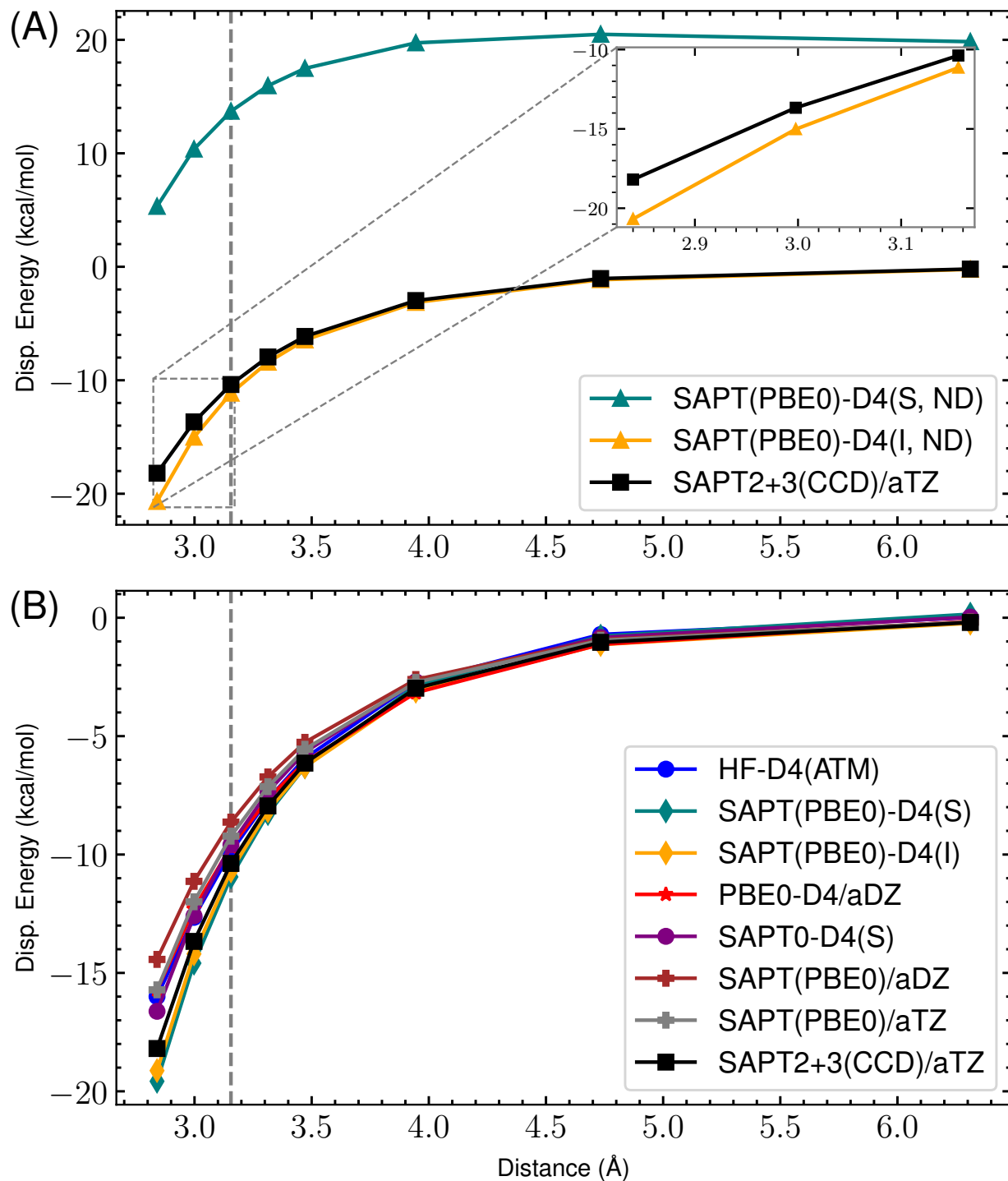
Figure 18: s66x8 29_Pyridine-Uracil : Dispersion potential Energy curve for SAPT(PBE0) with aDZ/aTZ and -D4 variants versus the reference SAPT2+3(CCD)/aug-cc-pVTZ dispersion energy. (A) highlights the completely non-damped (ND) D4 curves compared to the reference for both supermolecular (S) and intermolecular (I). The remaining s_8 = 0.89529649 . (B) shows the damped -D4(S), -D4(I), HF-D4, SAPT(PBE0)/aDZ, SAPT(PBE0)/aTZ, and reference dispersion energies. Here, (S) and (I) refer to the supermolecular and intermolecular dispersion energy approaches, respectively. The “ND” states that no damping function is used. For the damped SAPT(PBE0)-D4(S) and SAPT(PBE0)-D4(I) terms, a_1 , a_2 , and s_8 are fit to the residual CCSD(T)/CBS energies on the 4470 dimer dataset.
