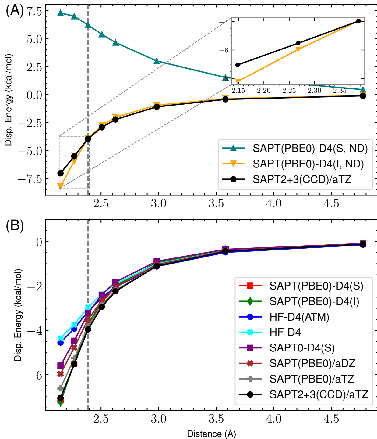
Figure 20: ND vs Damped D4 Dispersion for s66x8 58_Pyridine-Pyridine
