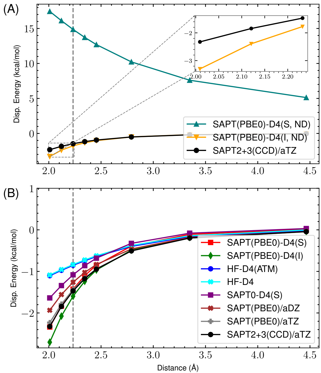
Figure 30: ND vs Damped D4 Dispersion for s66x8 59_Ethyne-Water
