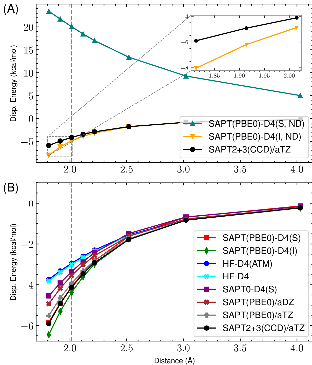
Figure 56: ND vs Damped D4 Dispersion for s66x8 13.Peptide-MeOH
