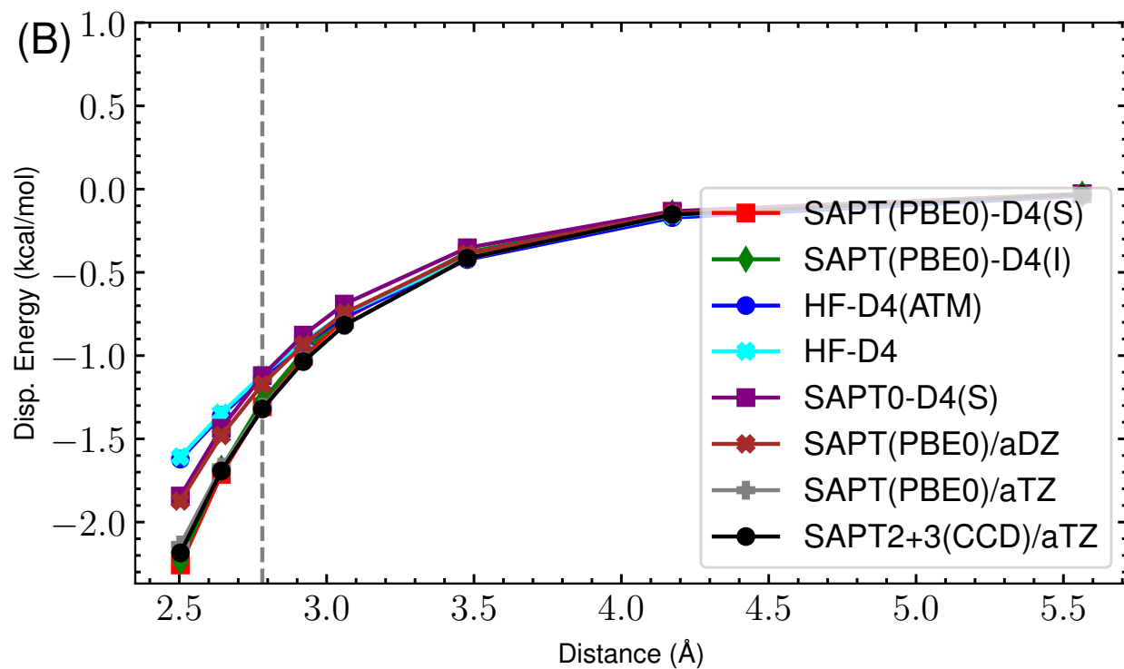
Figure 35: ND vs Damped D4 Dispersion for s66x8 51_Ethyne-Ethyne
