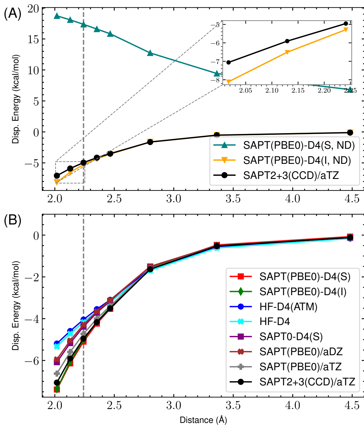
Figure 52: ND vs Damped D4 Dispersion for s66x8 11_MeNH2-Peptide
