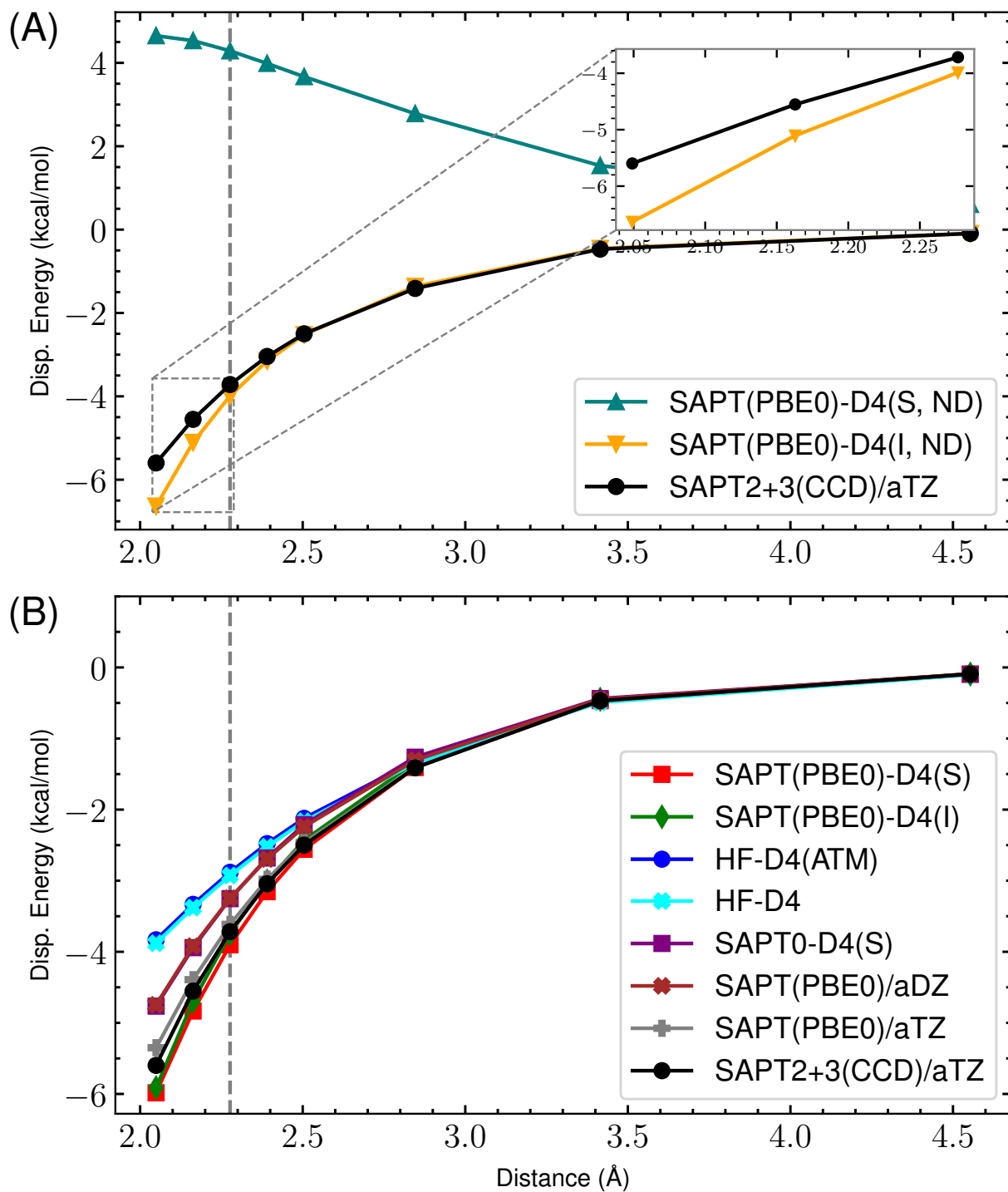
Figure 5: ND vs Damped D4 Dispersion for s66x8 10_MeNH2-MeNH2
