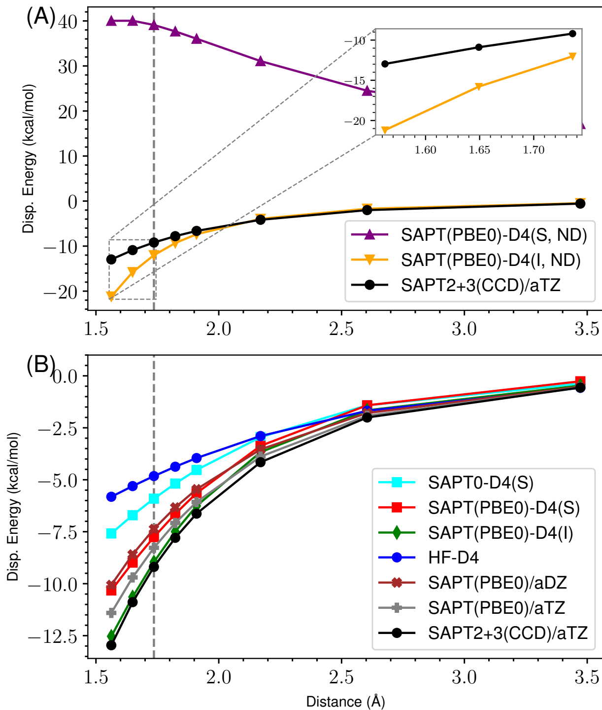
Figure 26: ND vs Damped D4 Dispersion for s66x8 23_AcNH2-Uracil
