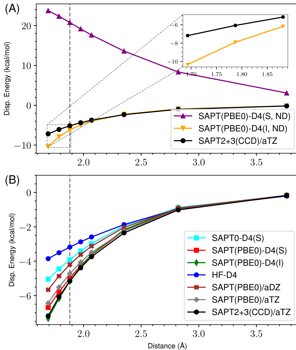
Figure 32: ND vs Damped D4 Dispersion for s66x8 07_MeOH-Peptide
