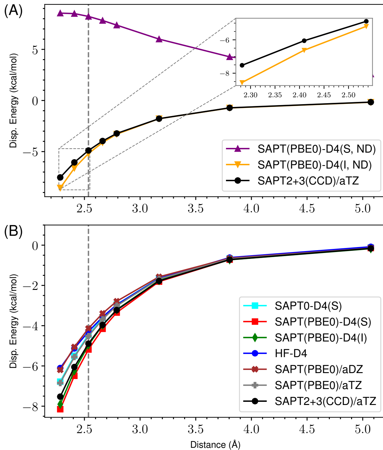
Figure 19: ND vs Damped D4 Dispersion for s66x8 55_Benzene-MeOH
