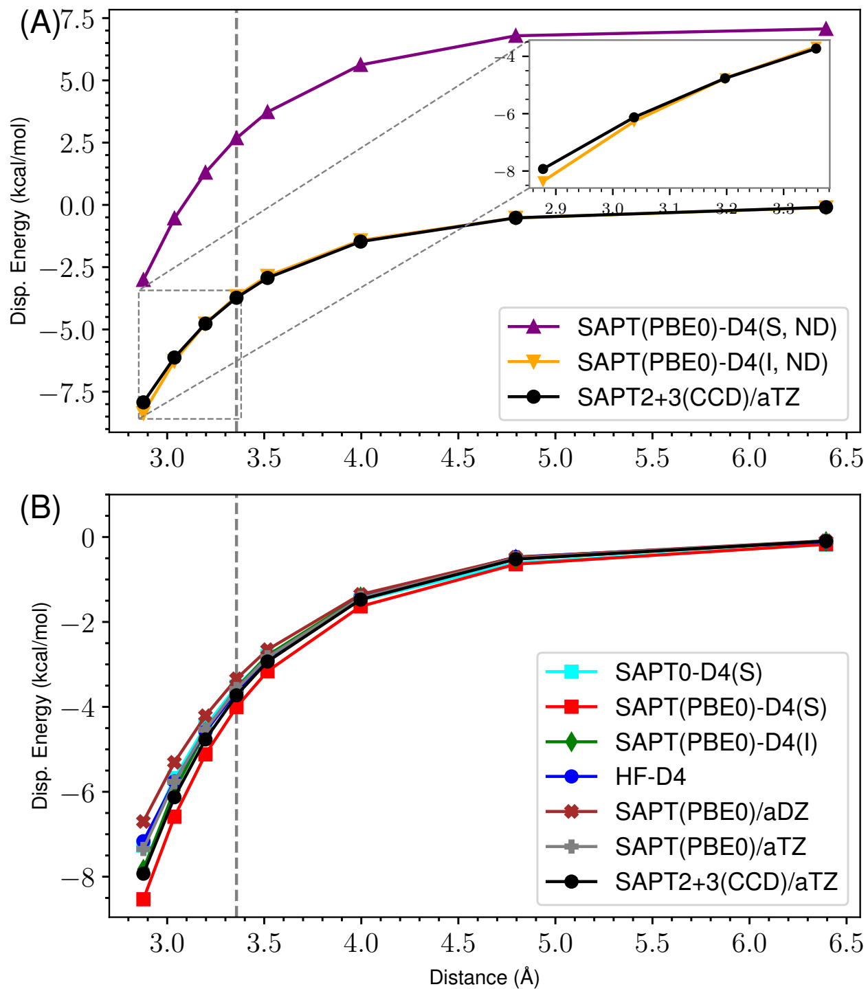
Figure 14: ND vs Damped D4 Dispersion for s66x8 33_Pyridine-Ethene
