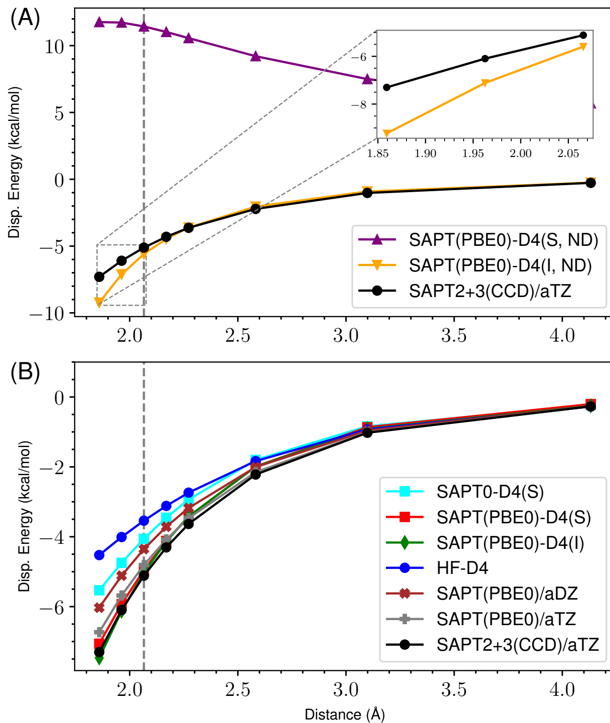
Figure 1: ND vs Damped D4 Dispersion for s66x8 14_Peptide-MeNH2
