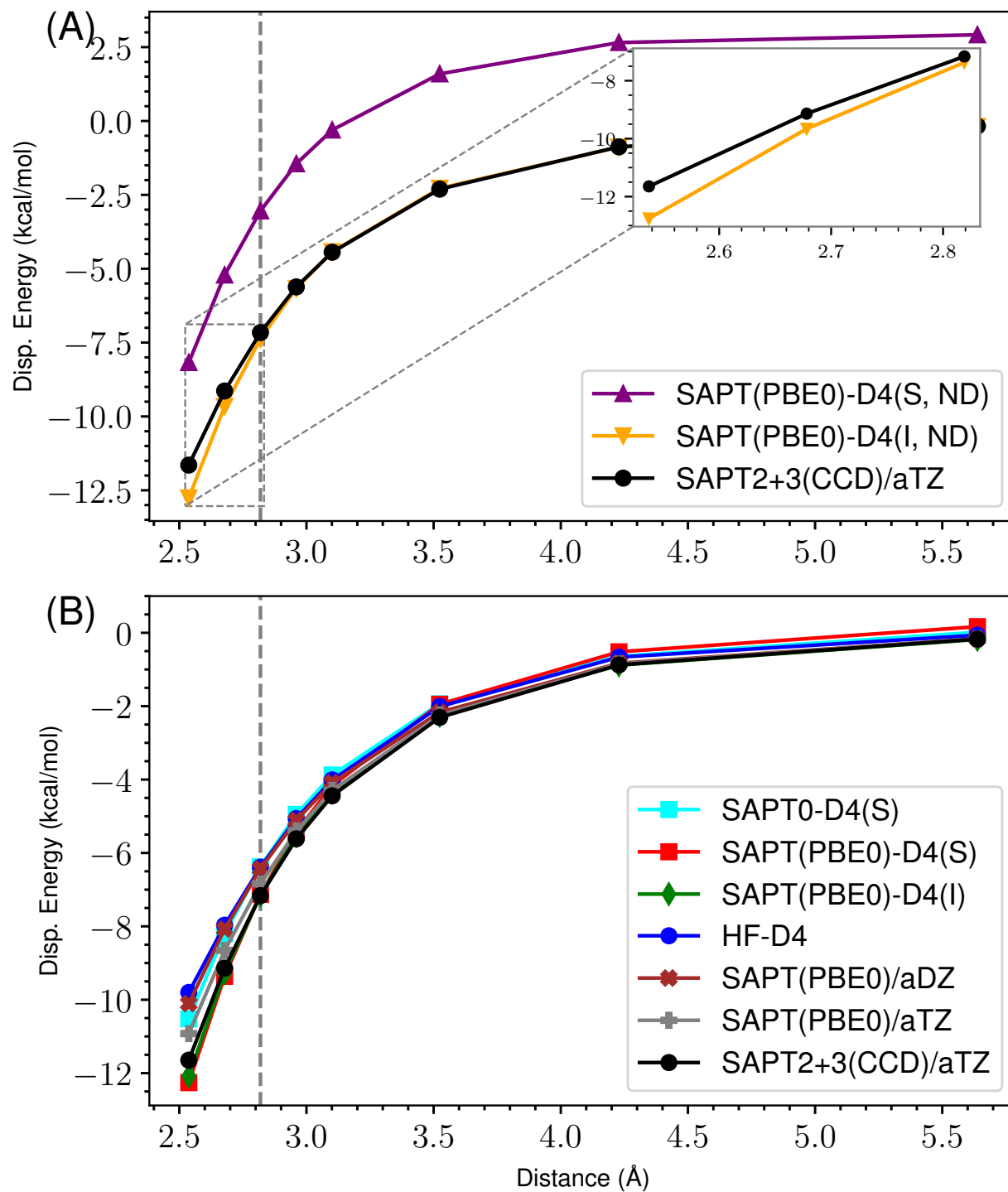
Figure 54: ND vs Damped D4 Dispersion for s66x8 39_Benzene-Cyclopentane
