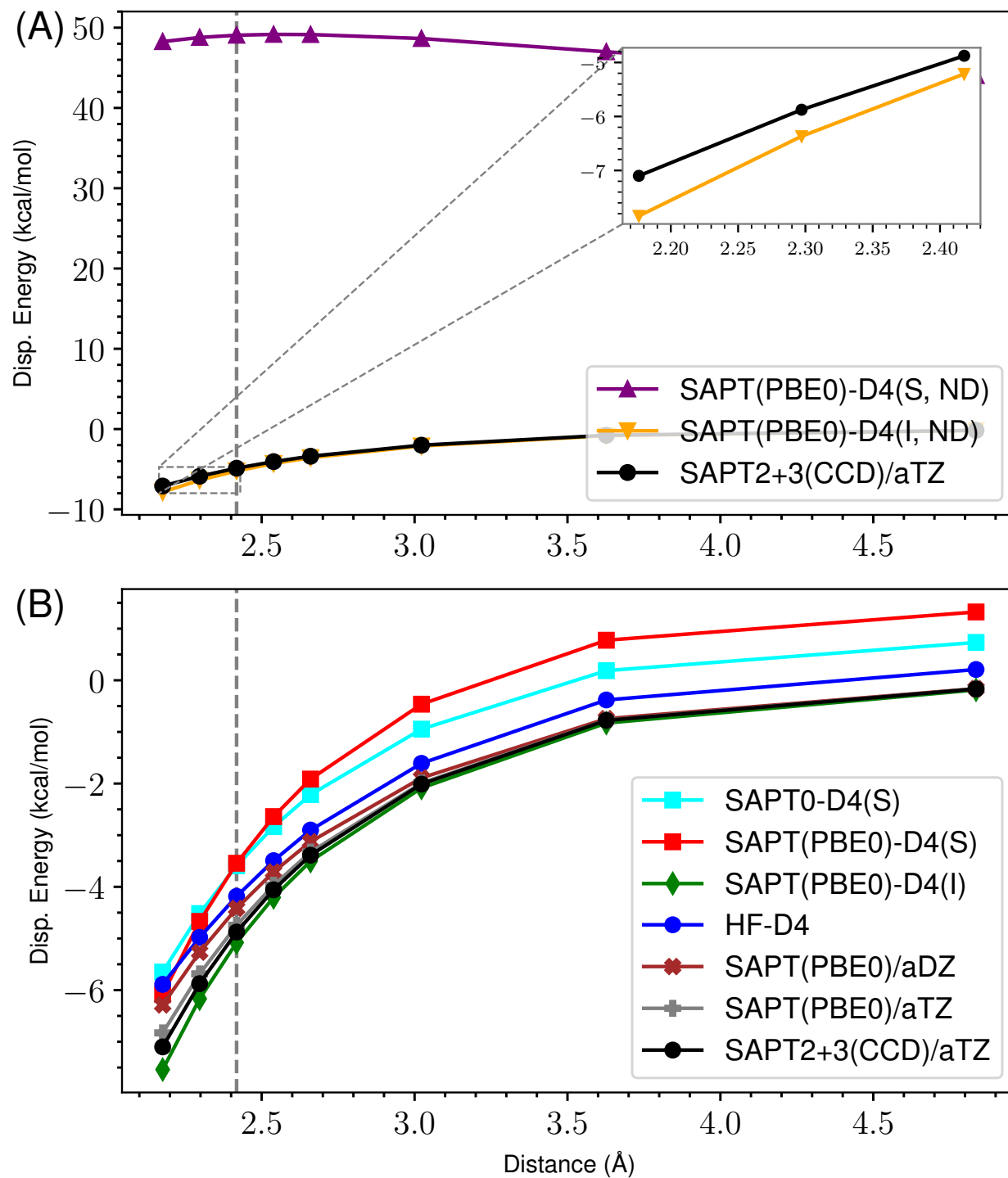
Figure 61: ND vs Damped D4 Dispersion for s66x8 61_Pentane-AcOH
