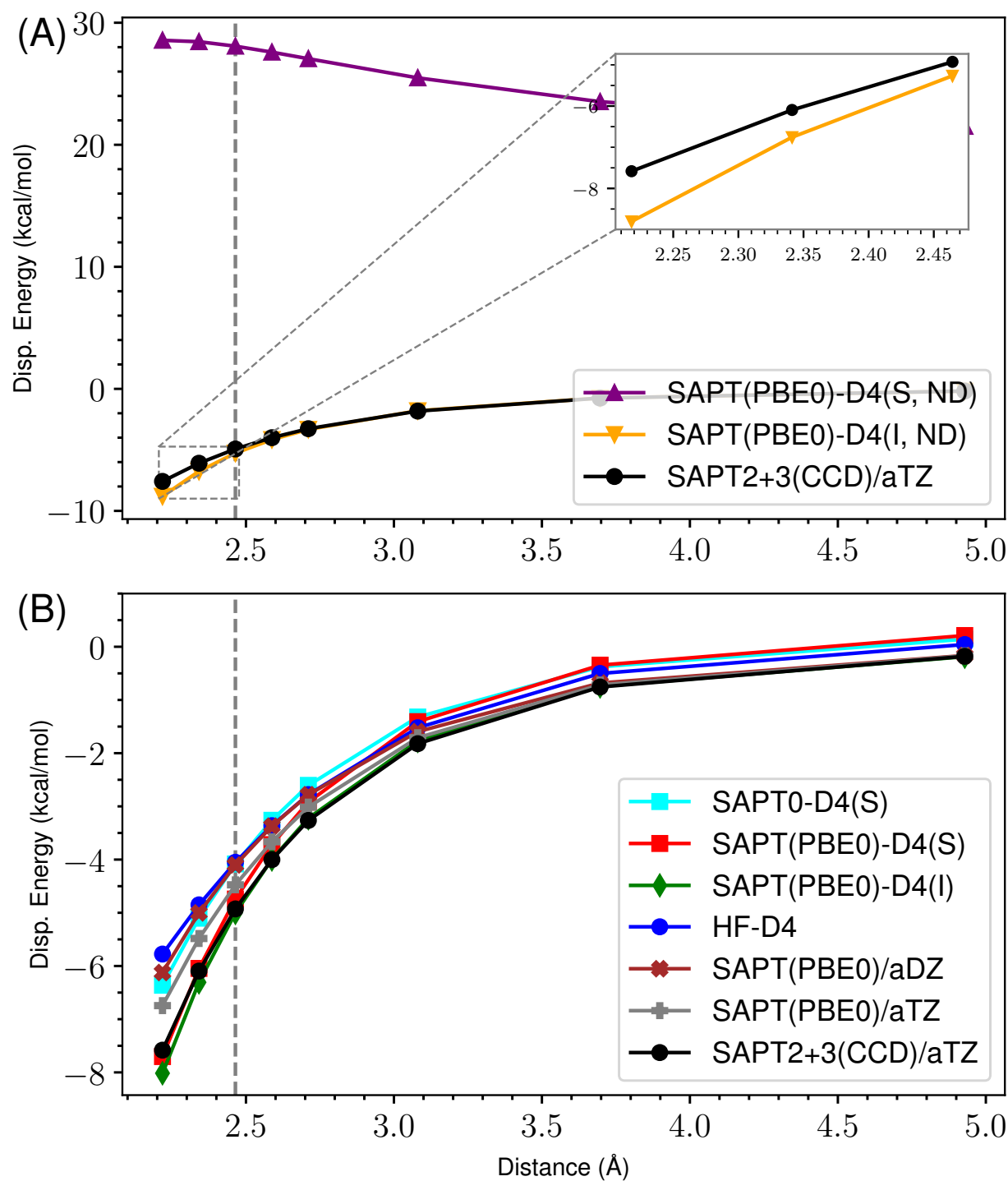
Figure 9: ND vs Damped D4 Dispersion for s66x8 52_Benzene-AcOH
