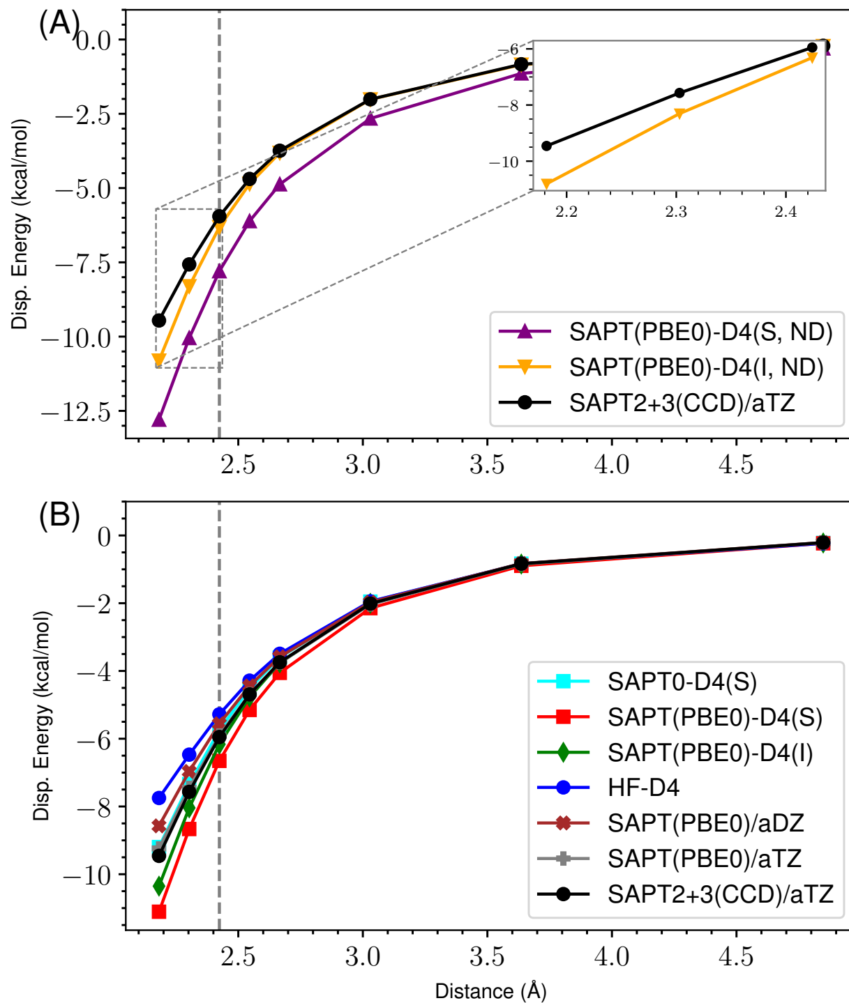
Figure 57: ND vs Damped D4 Dispersion for s66x8 38_Cyclopentane-Cyclopentane
