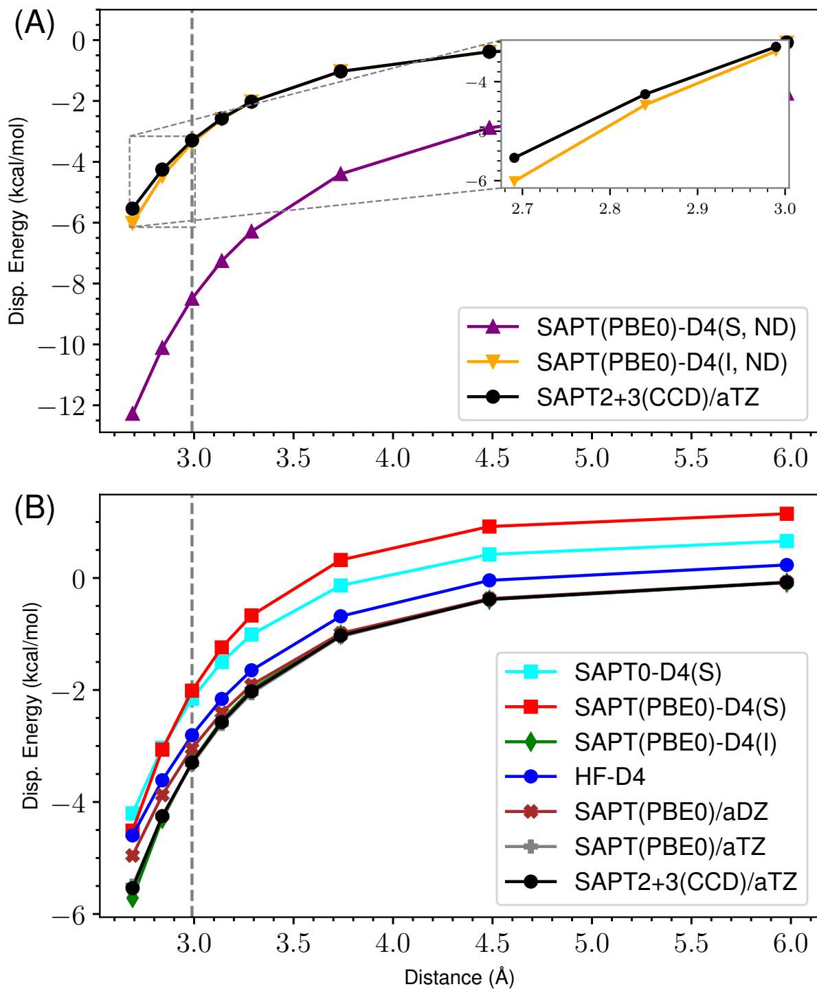
Figure 2: ND vs Damped D4 Dispersion for s66x8 45_Ethyne-Pentane
