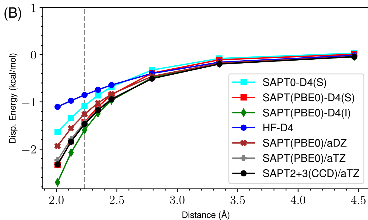
Figure 30: ND vs Damped D4 Dispersion for s66x8 59_Ethyne-Water
