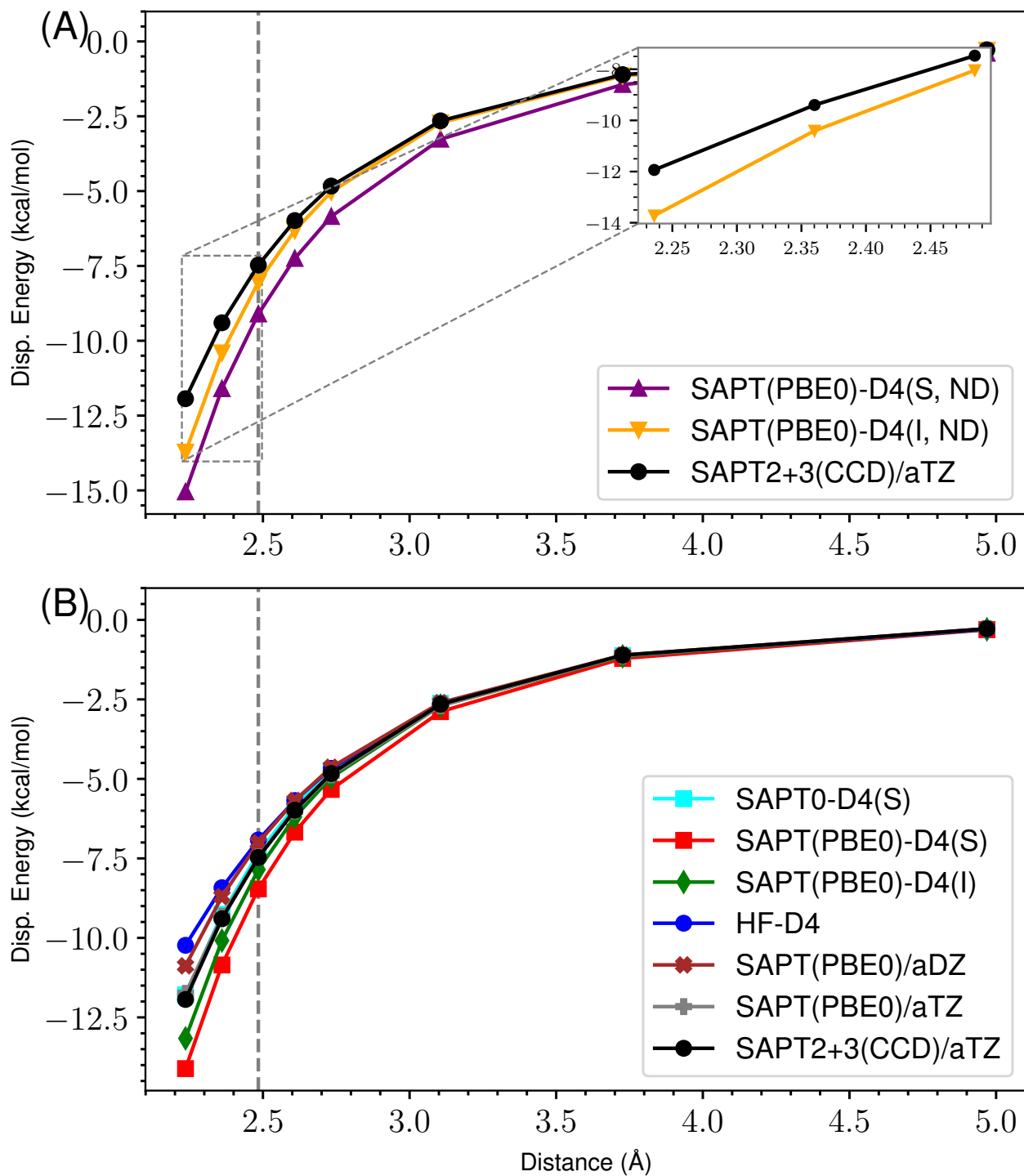
Figure 40: ND vs Damped D4 Dispersion for s66x8 34_Pentane-Pentane
