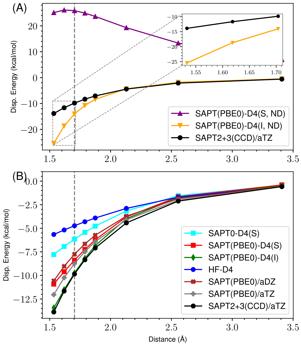
Figure 15: ND vs Damped D4 Dispersion for s66x8 22_AcOH-Uracil
