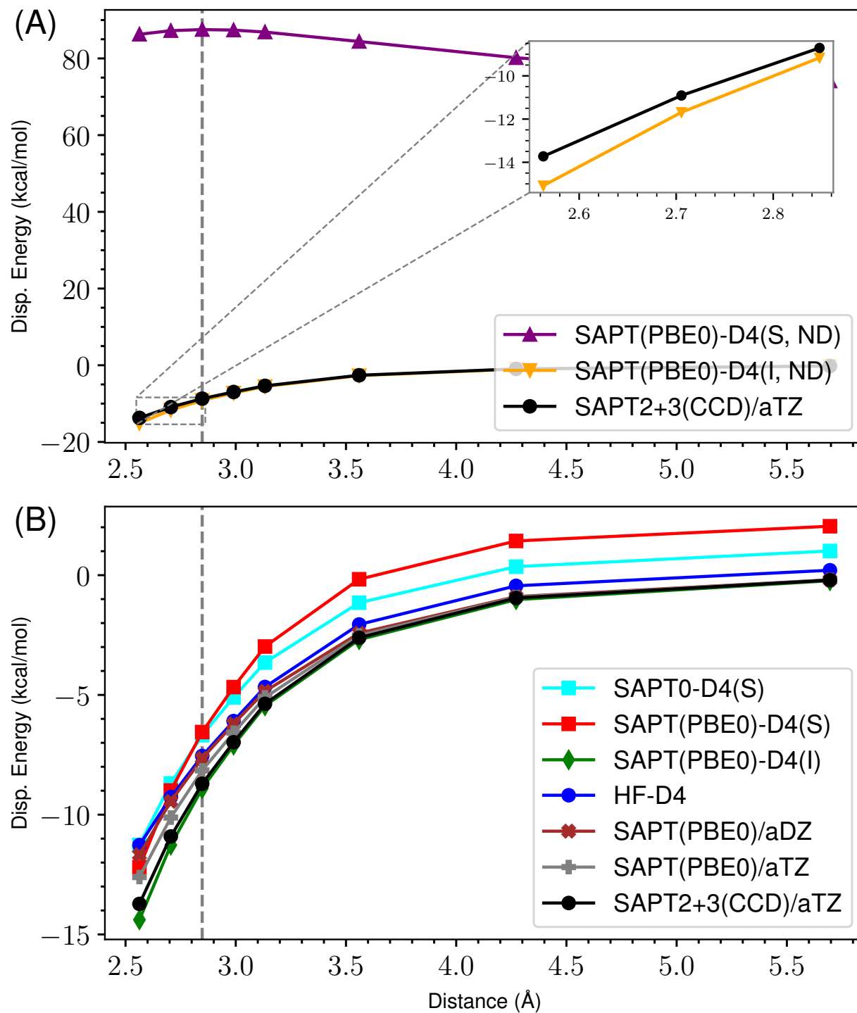
Figure 3: ND vs Damped D4 Dispersion for s66x8 41_Uracil-Pentane
