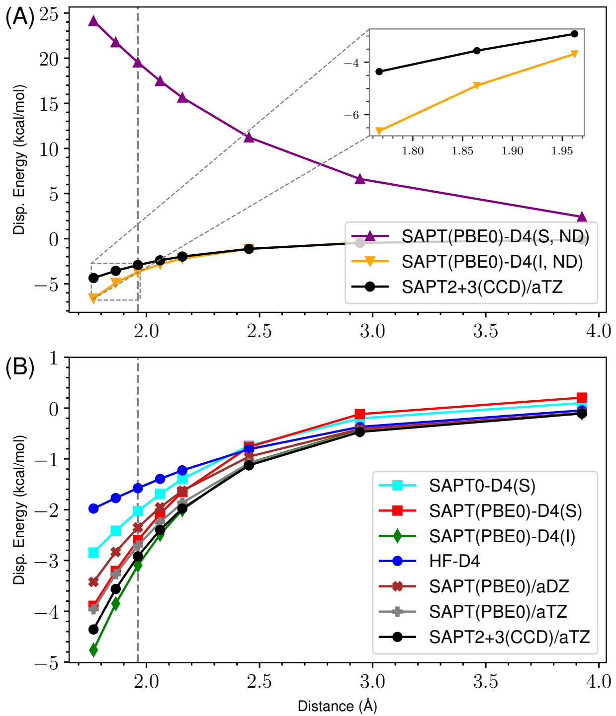
Figure 8: ND vs Damped D4 Dispersion for s66x8 02_Water-MeOH
