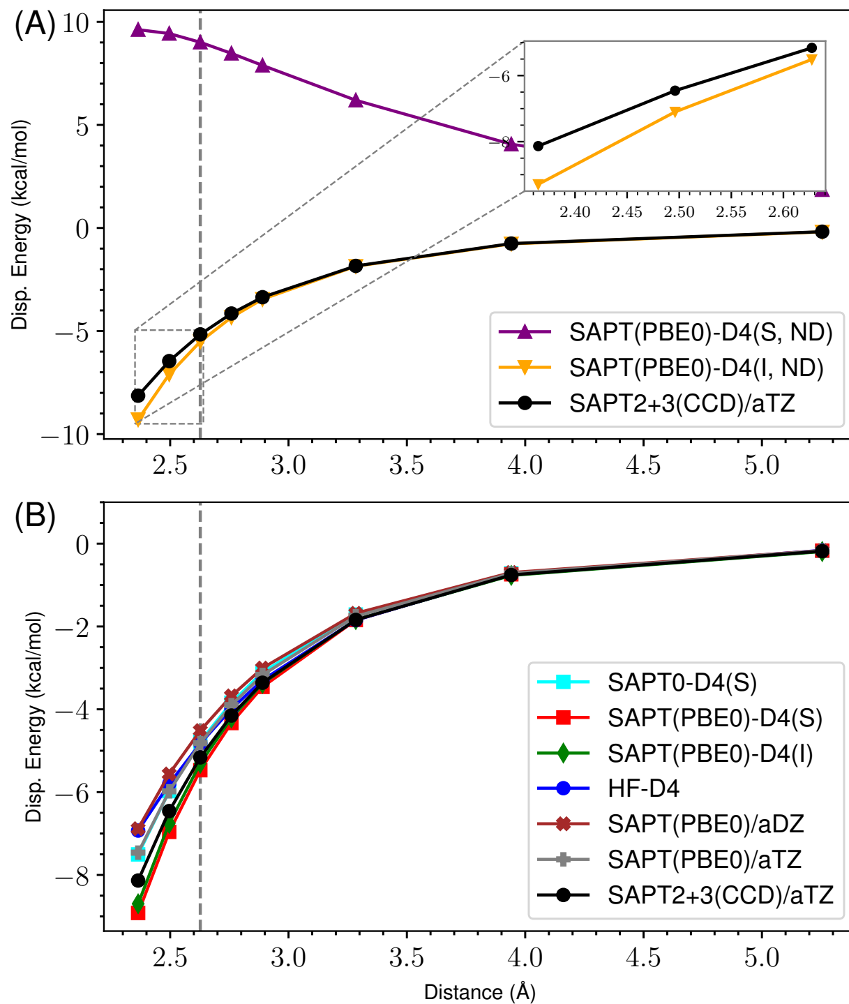
Figure 28: ND vs Damped D4 Dispersion for s66x8 48_Pyridine-Pyridine
