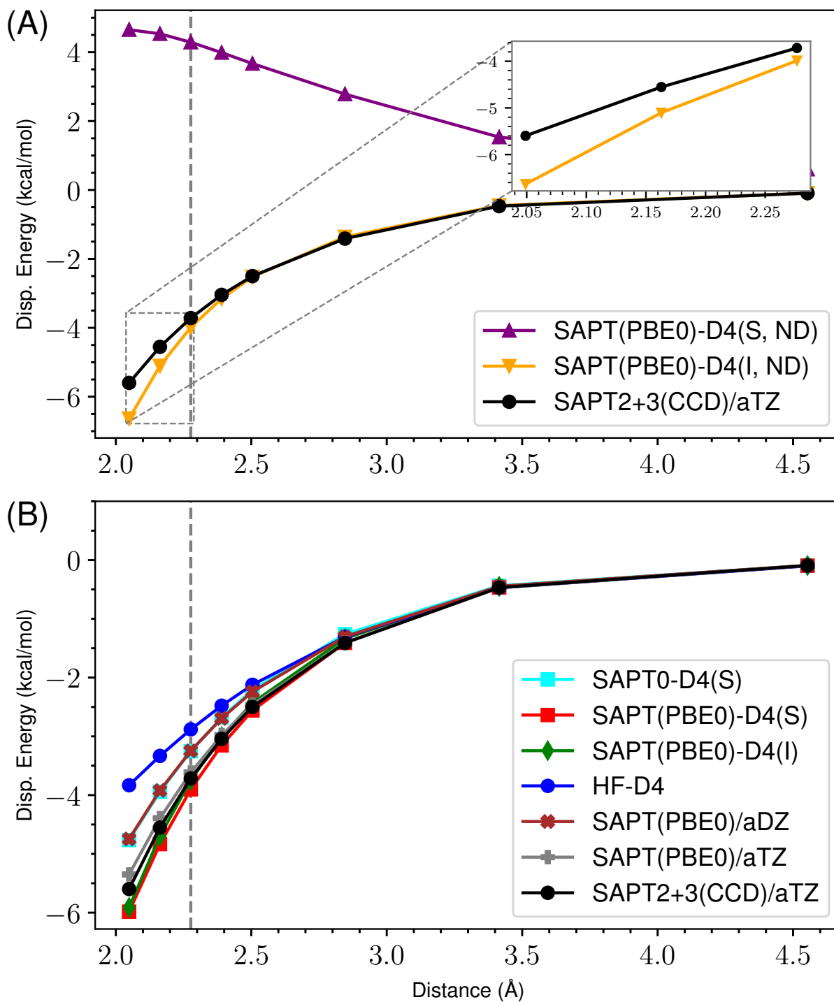
Figure 5: ND vs Damped D4 Dispersion for s66x8 10_MeNH2-MeNH2
