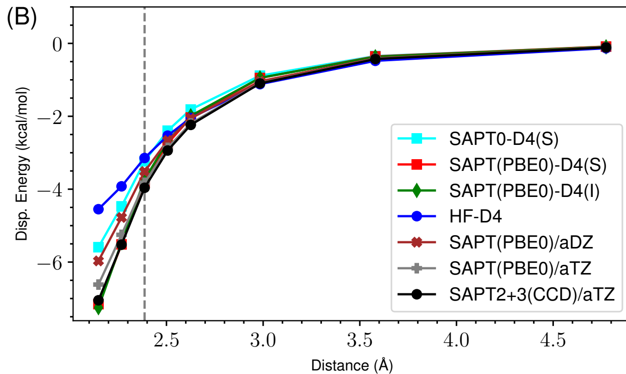
Figure 20: ND vs Damped D4 Dispersion for s66x8 58_Pyridine-Pyridine
