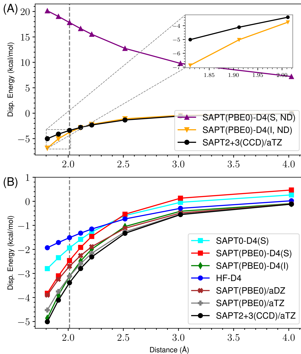
Figure 41: ND vs Damped D4 Dispersion for s66x8 03_Water-MeNH2
