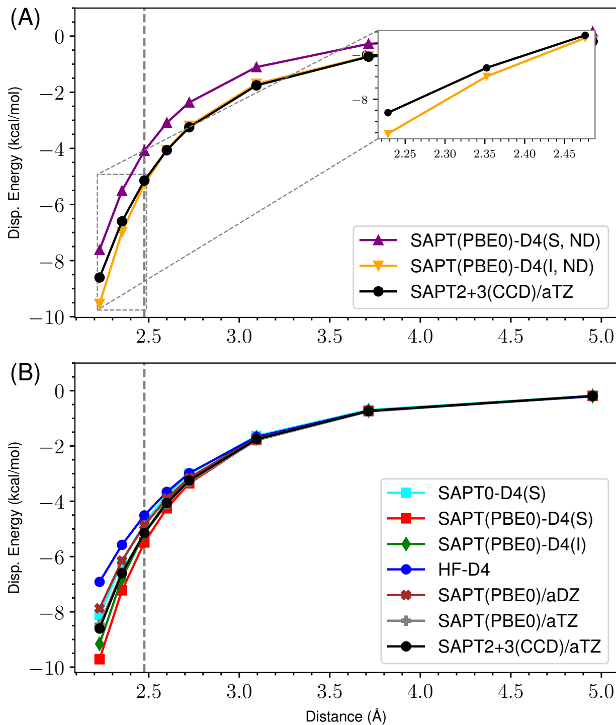
Figure 47: ND vs Damped D4 Dispersion for s66x8 35_Neopentane-Pentane
