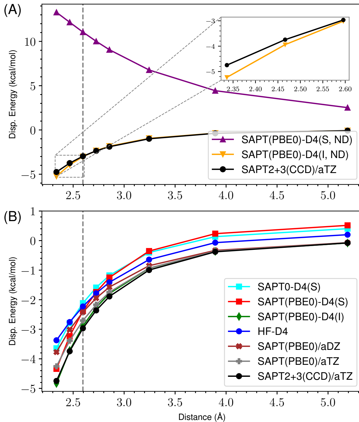
Figure 13: ND vs Damped D4 Dispersion for s66x8 54_Benzene-Water
