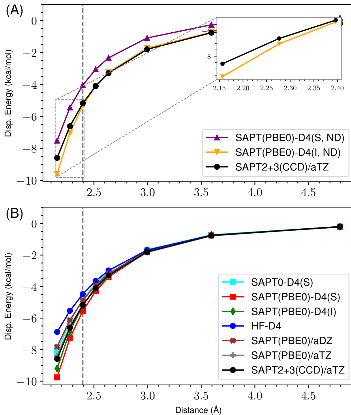
Figure 63: ND vs Damped D4 Dispersion for s66x8 37_Cyclopentane-Neopentane
