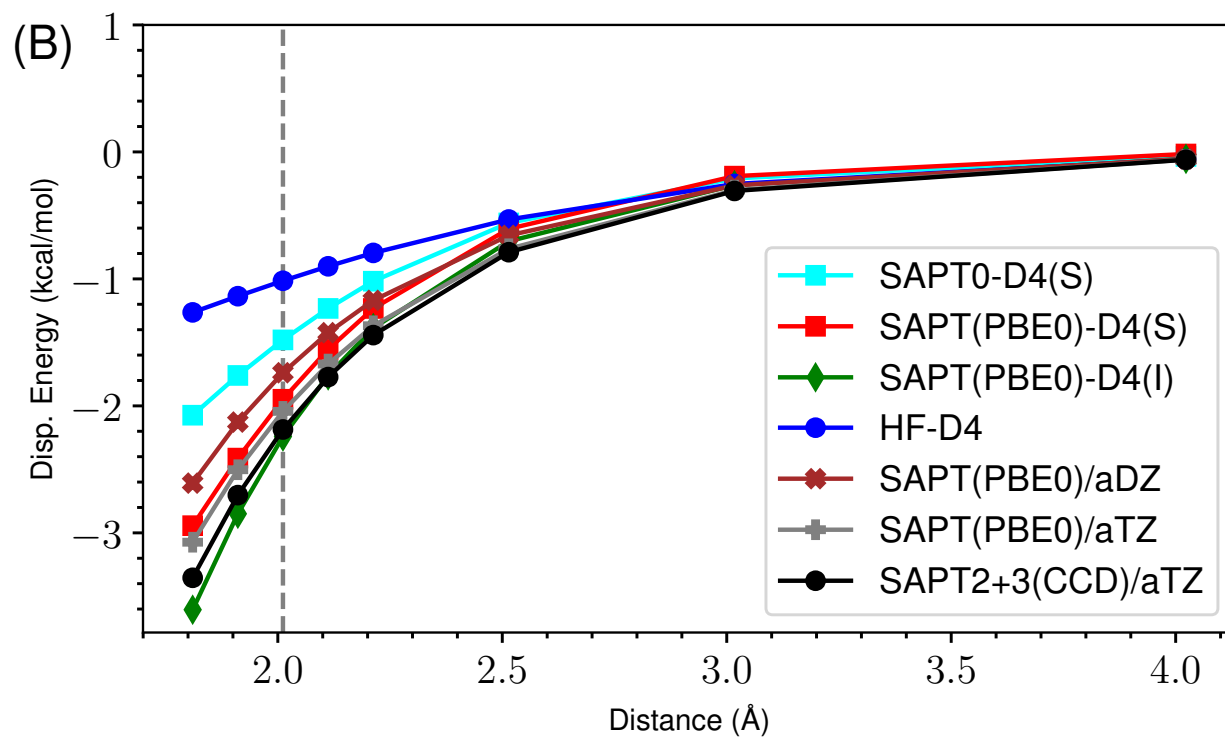
Figure 22: ND vs Damped D4 Dispersion for s66x8 01_Water-Water
