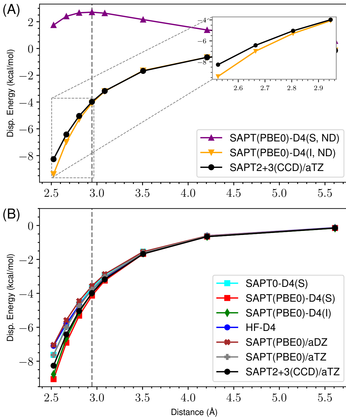
Figure 17: ND vs Damped D4 Dispersion for s66x8 47_Benzene-Benzene
