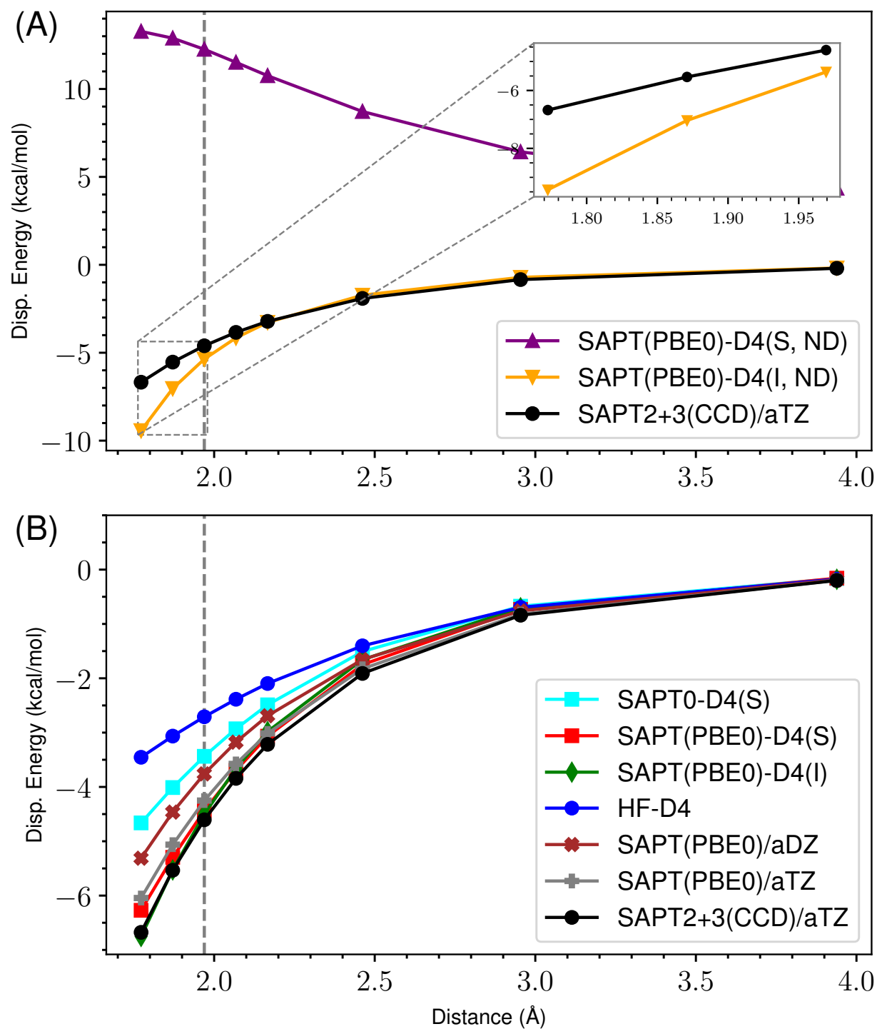
Figure 48: ND vs Damped D4 Dispersion for s66x8 06_MeOH-MeNH2
