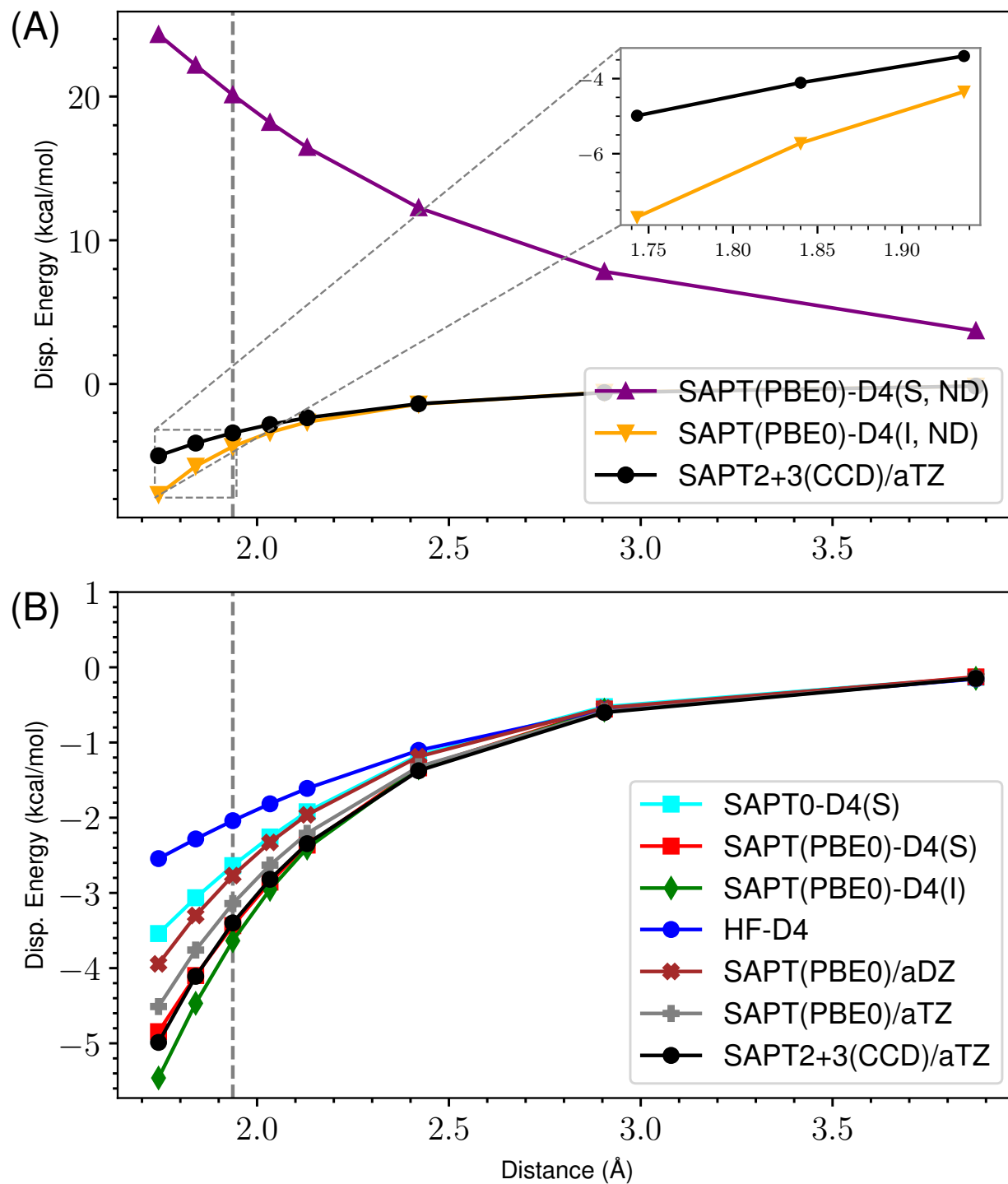
Figure 33: ND vs Damped D4 Dispersion for s66x8 05_MeOH-MeOH
