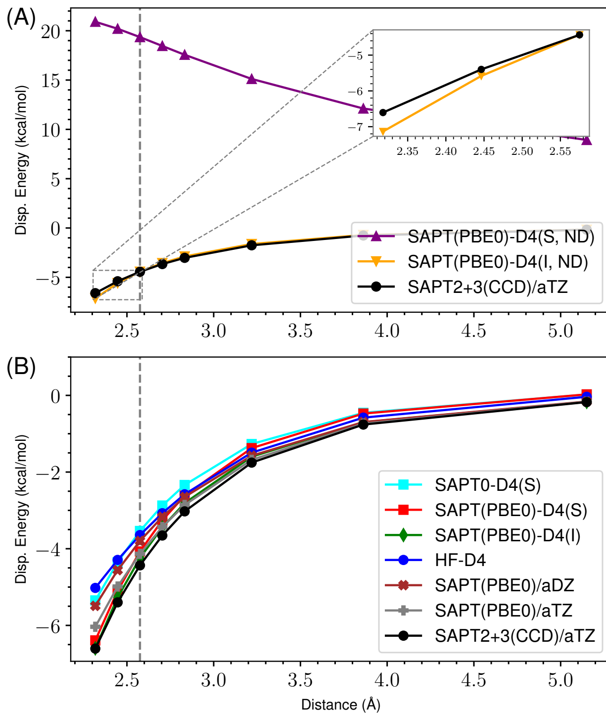
Figure 36: ND vs Damped D4 Dispersion for s66x8 53_Benzene-AcNH2
