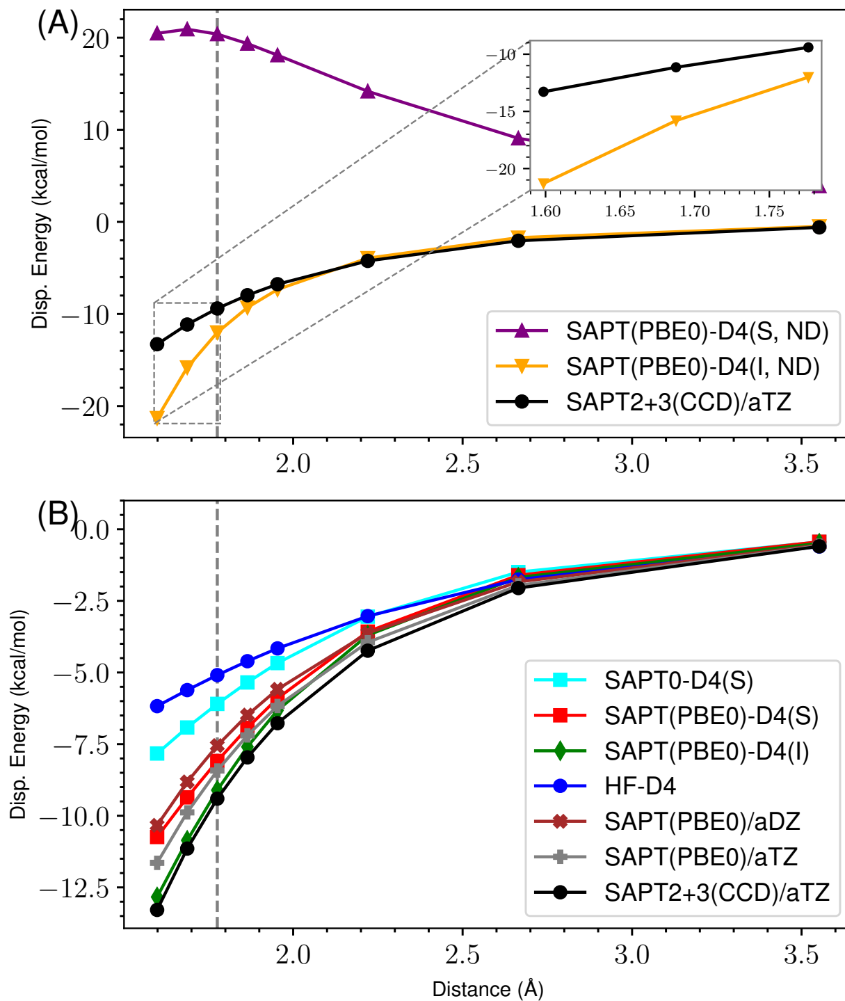
Figure 46: ND vs Damped D4 Dispersion for s66x8 17_Uracil-Uracil
