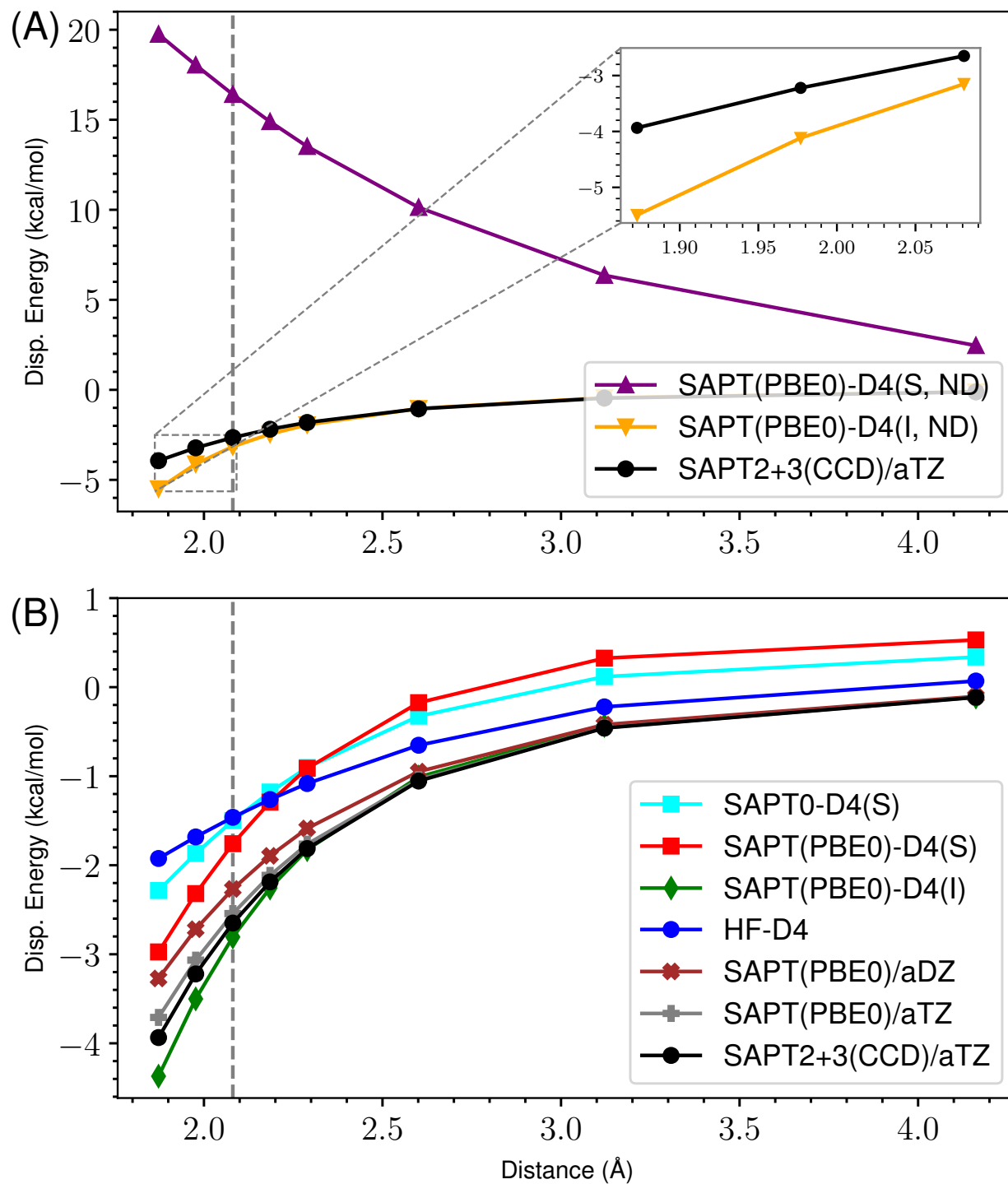
Figure 6: ND vs Damped D4 Dispersion for s66x8 16_Peptide-Water
