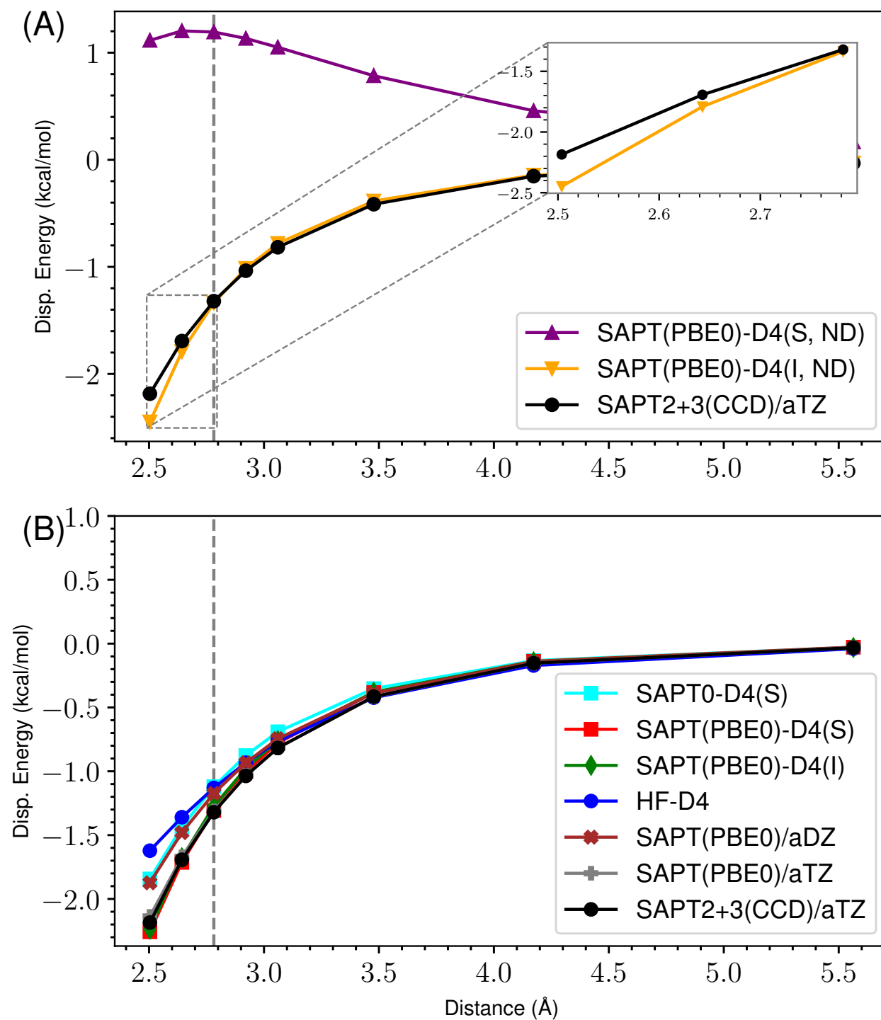
Figure 35: ND vs Damped D4 Dispersion for s66x8 51_Ethyne-Ethyne
