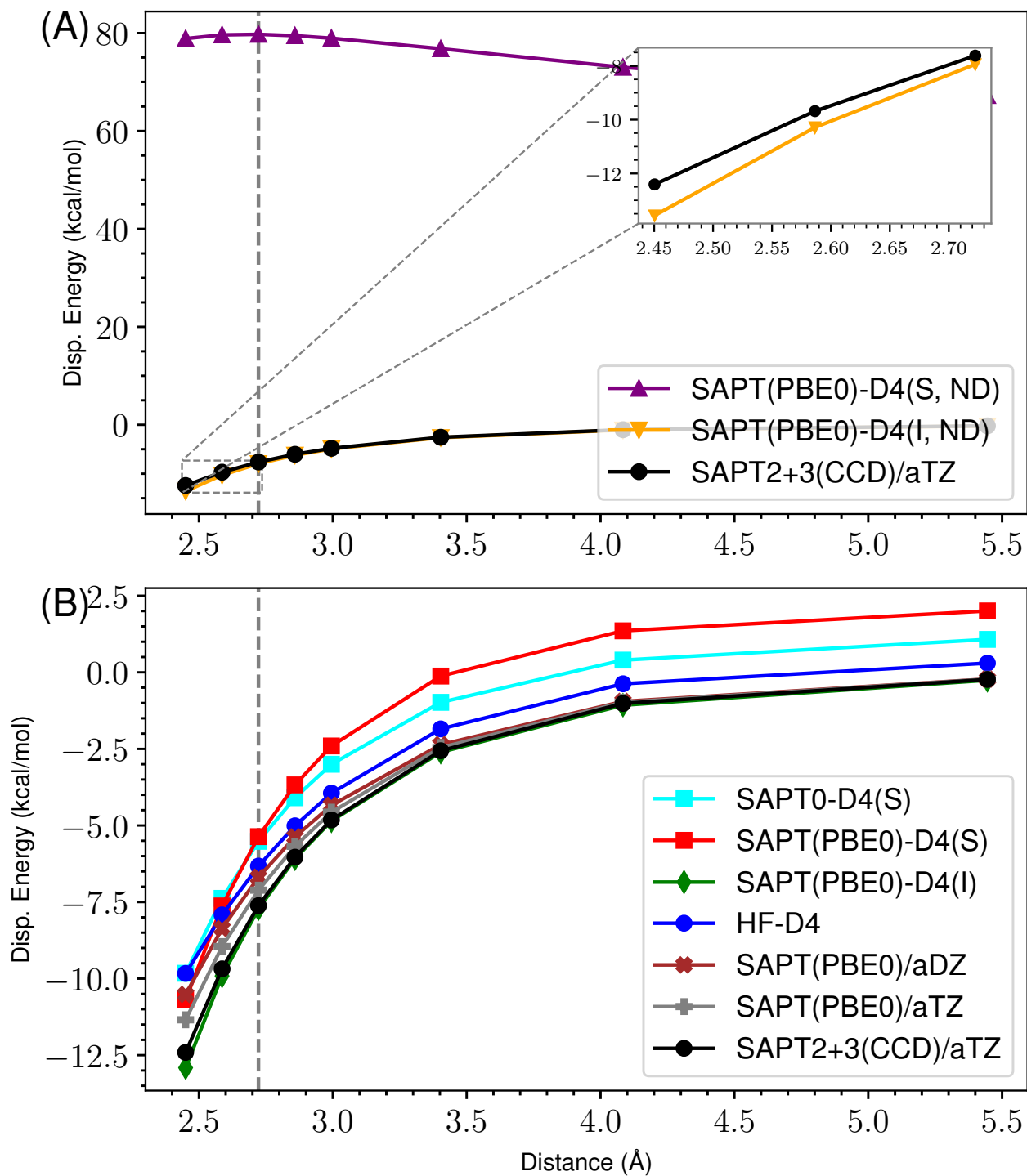
Figure 29: ND vs Damped D4 Dispersion for s66x8 42_Uracil-Cyclopentane
