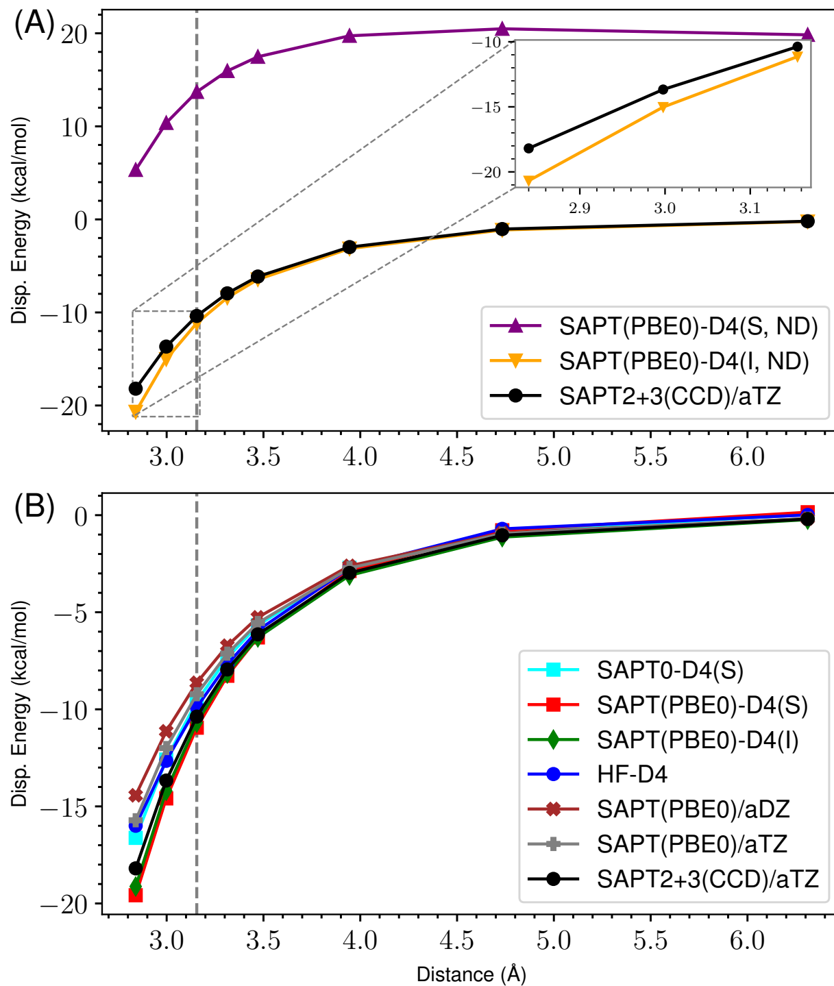
Figure 18: ND vs Damped D4 Dispersion for s66x8 29_Pyridine-Uracil
