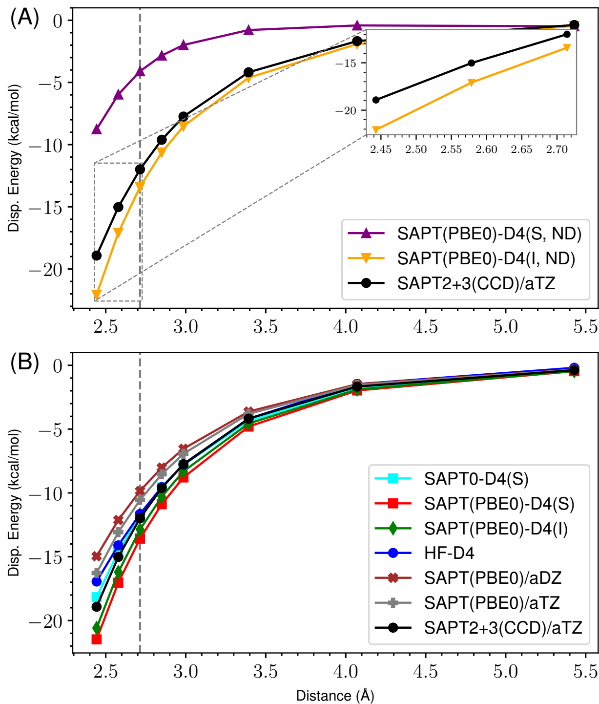
Figure 10: ND vs Damped D4 Dispersion for s66x8 26_Uracil-Uracil
