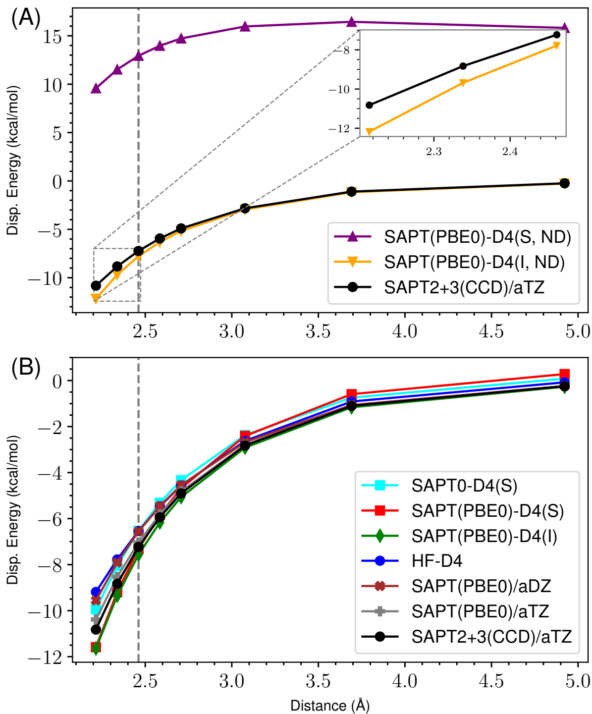
Figure 45: ND vs Damped D4 Dispersion for s66x8 46_Peptide-Pentane
