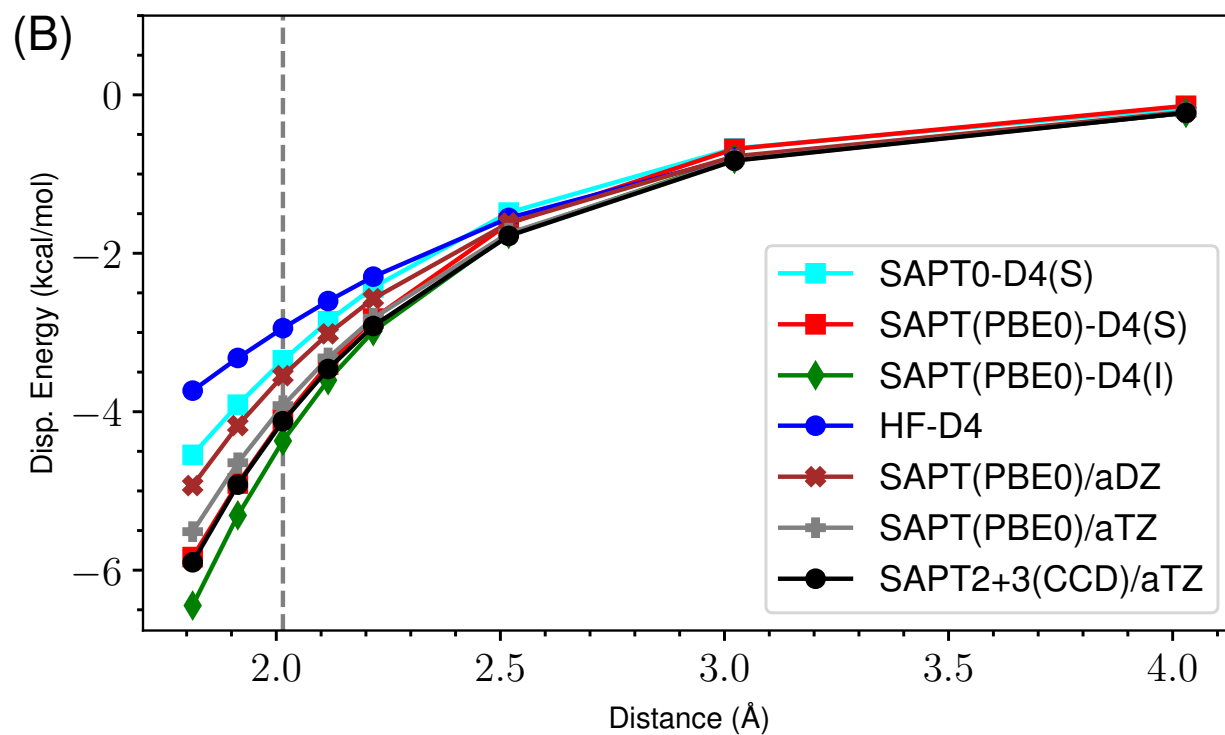
Figure 56: ND vs Damped D4 Dispersion for s66x8 13.Peptide-MeOH
