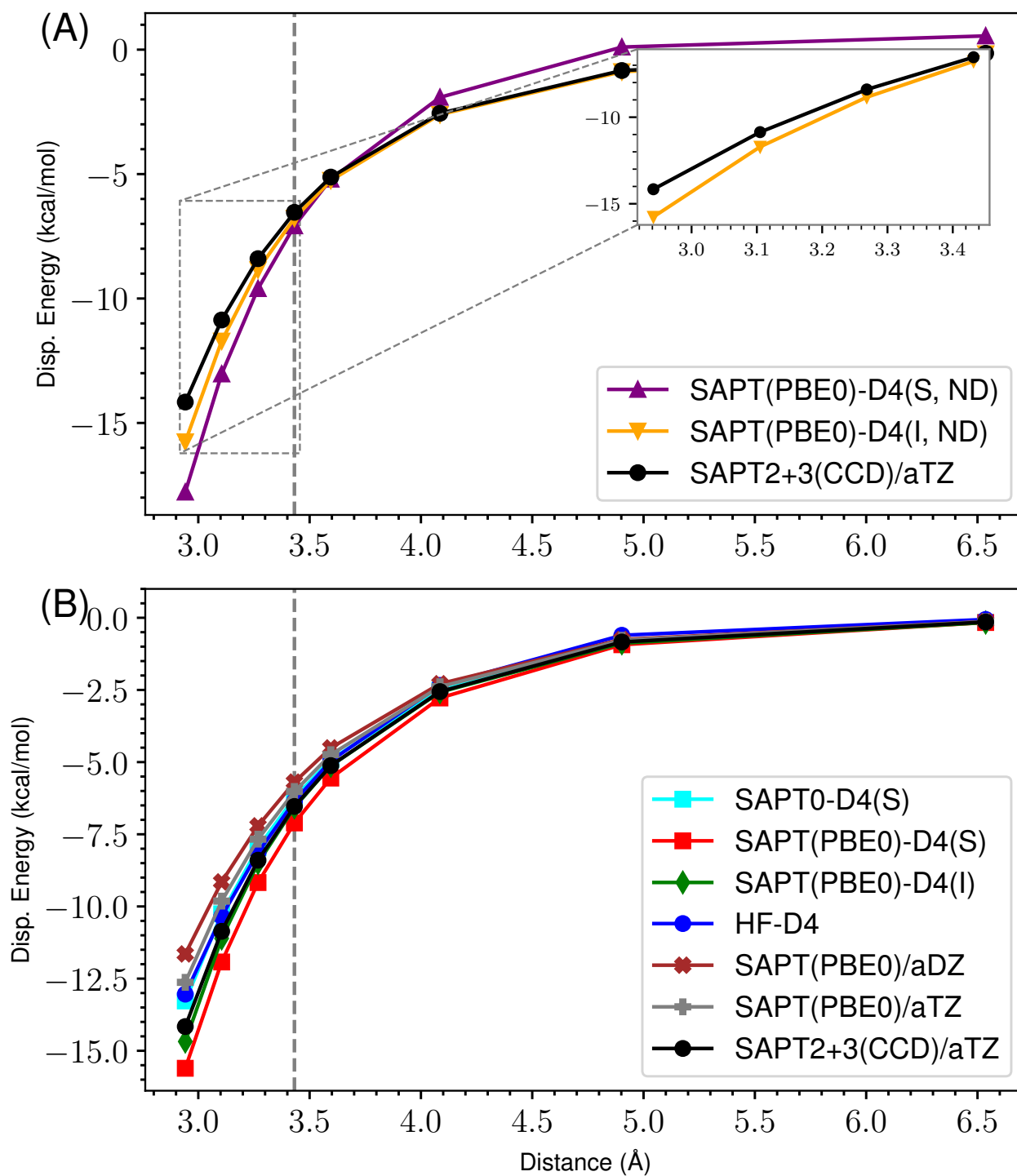
Figure 12: ND vs Damped D4 Dispersion for s66x8 25_Pyridine-Pyridine
