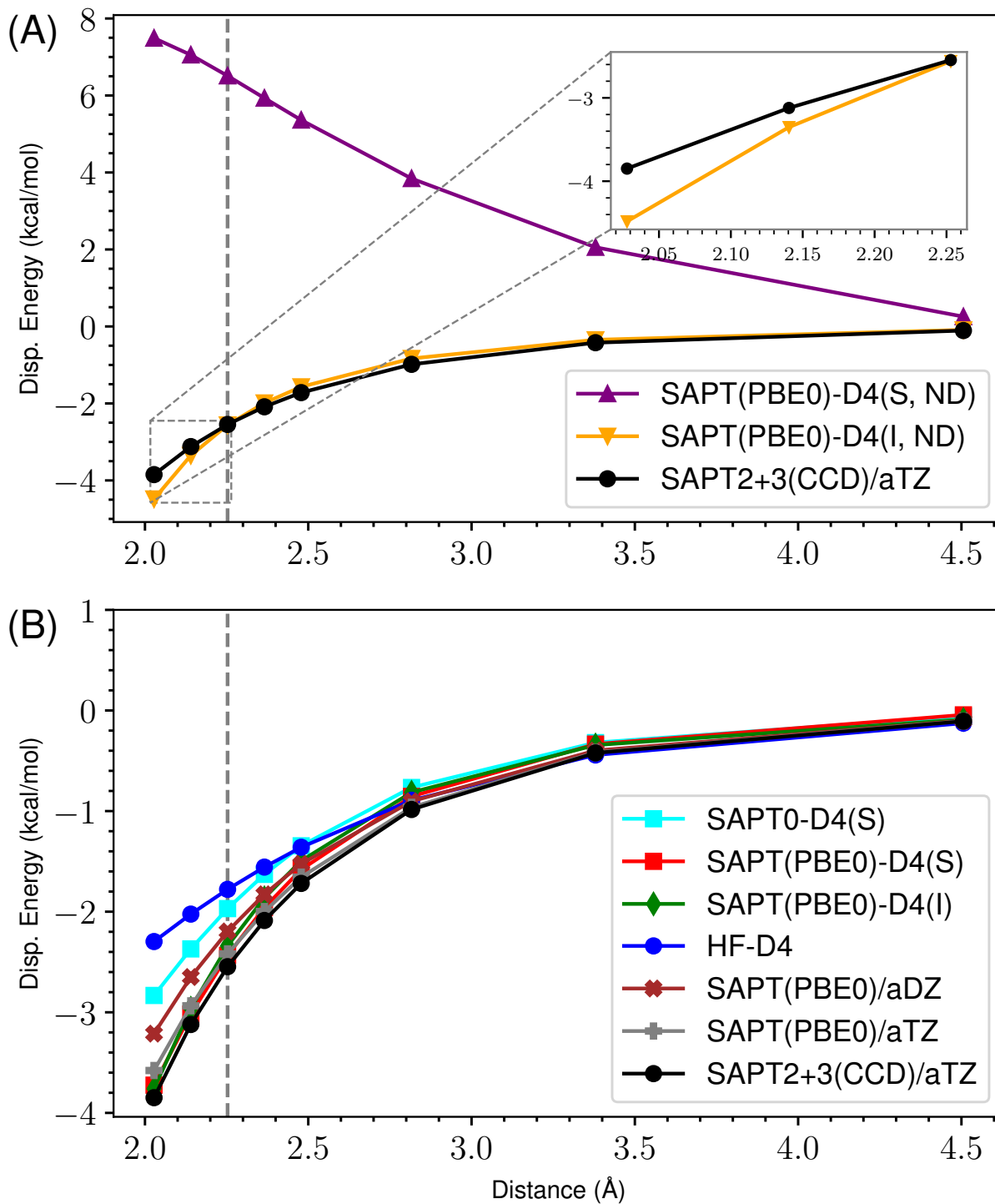
Figure 16: ND vs Damped D4 Dispersion for s66x8 65_Pyridine-Ethyne
