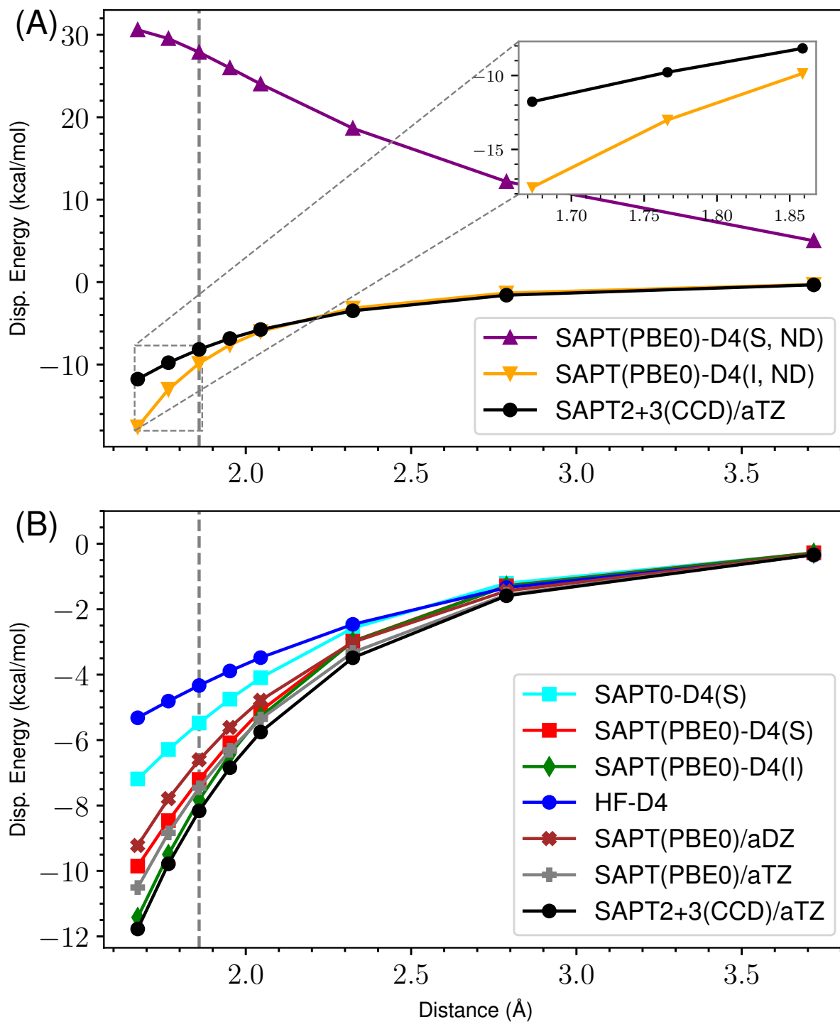
Figure 50: ND vs Damped D4 Dispersion for s66x8 21_AcNH2-AcNH2
