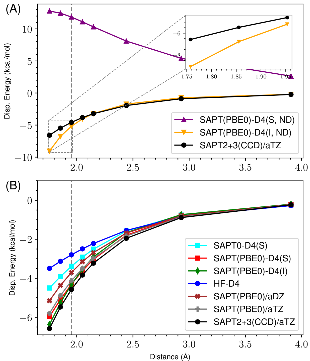
Figure 66: ND vs Damped D4 Dispersion for s66x8 19_MeOH-Pyridine
