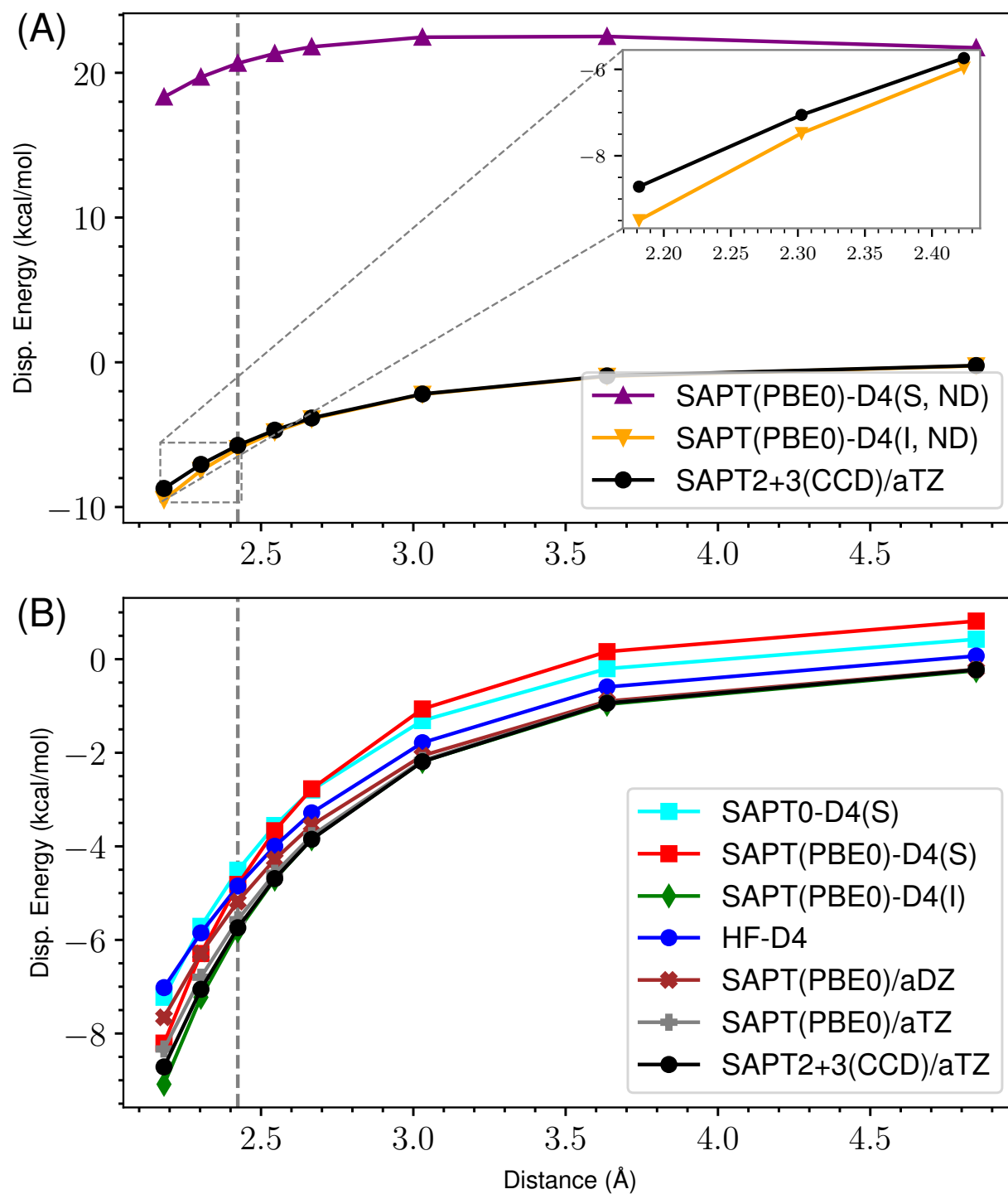
Figure 51: ND vs Damped D4 Dispersion for s66x8 62_Pentane-AcNH2
