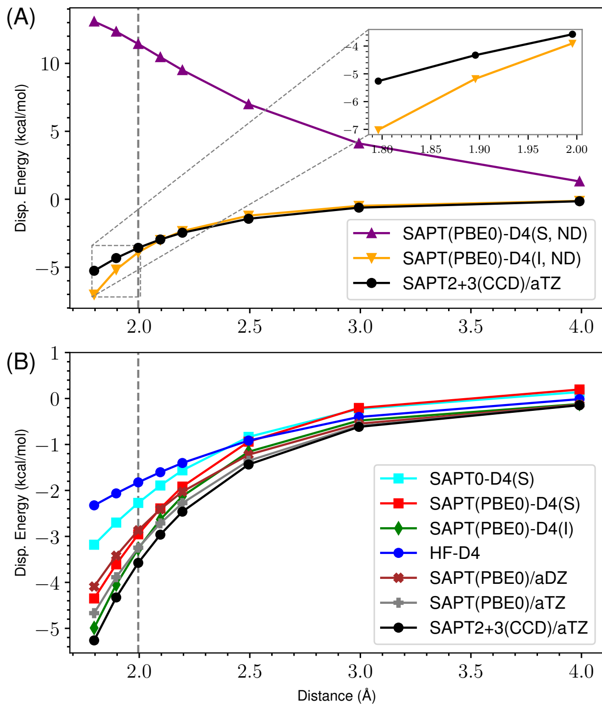
Figure 49: ND vs Damped D4 Dispersion for s66x8 18_Water-Pyridine
