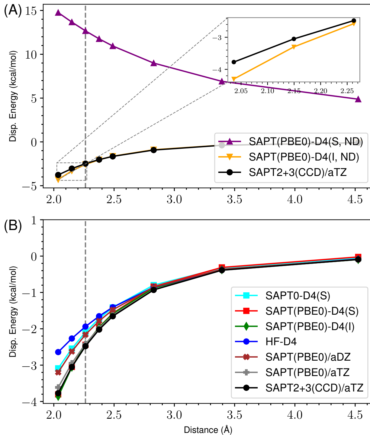
Figure 42: ND vs Damped D4 Dispersion for s66x8 09_MeNH2-MeOH
