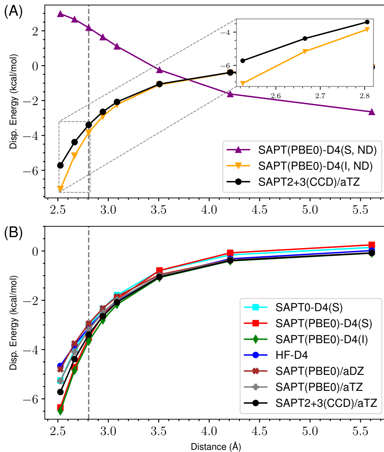
Figure 21: ND vs Damped D4 Dispersion for s66x8 50_Benzene-Ethyne
