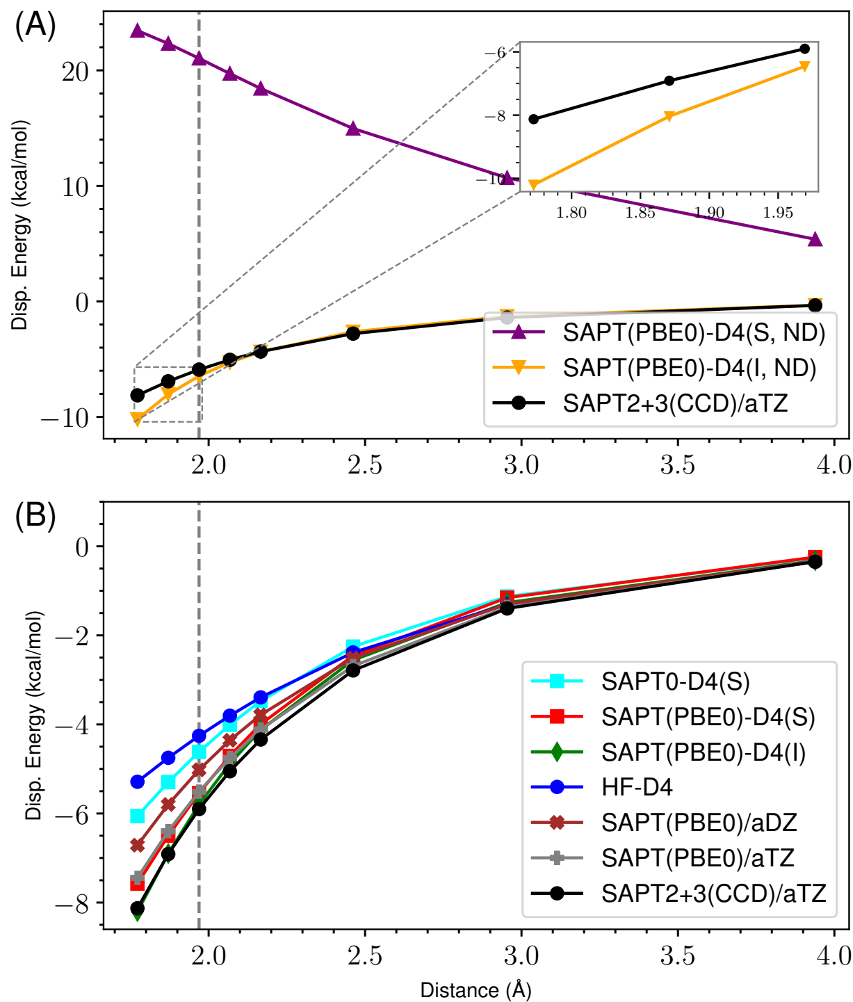
Figure 27: ND vs Damped D4 Dispersion for s66x8 15_Peptide-Peptide
