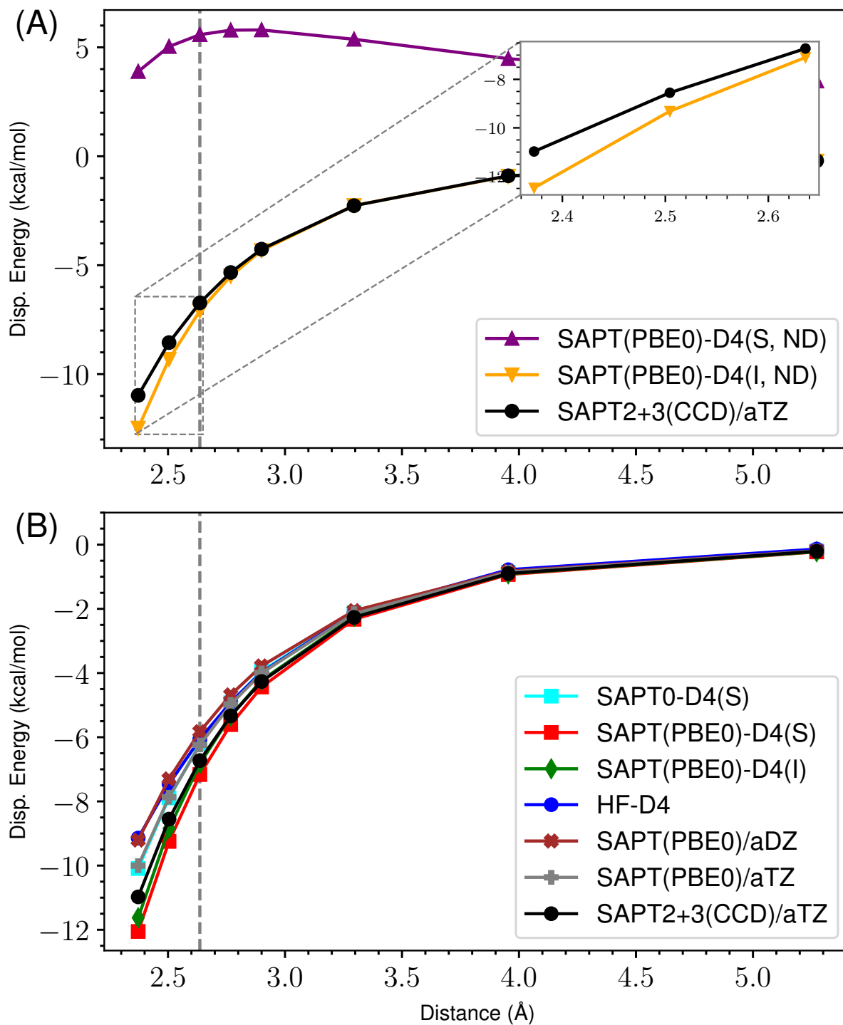
Figure 24: ND vs Damped D4 Dispersion for s66x8 57_Benzene-Peptide
