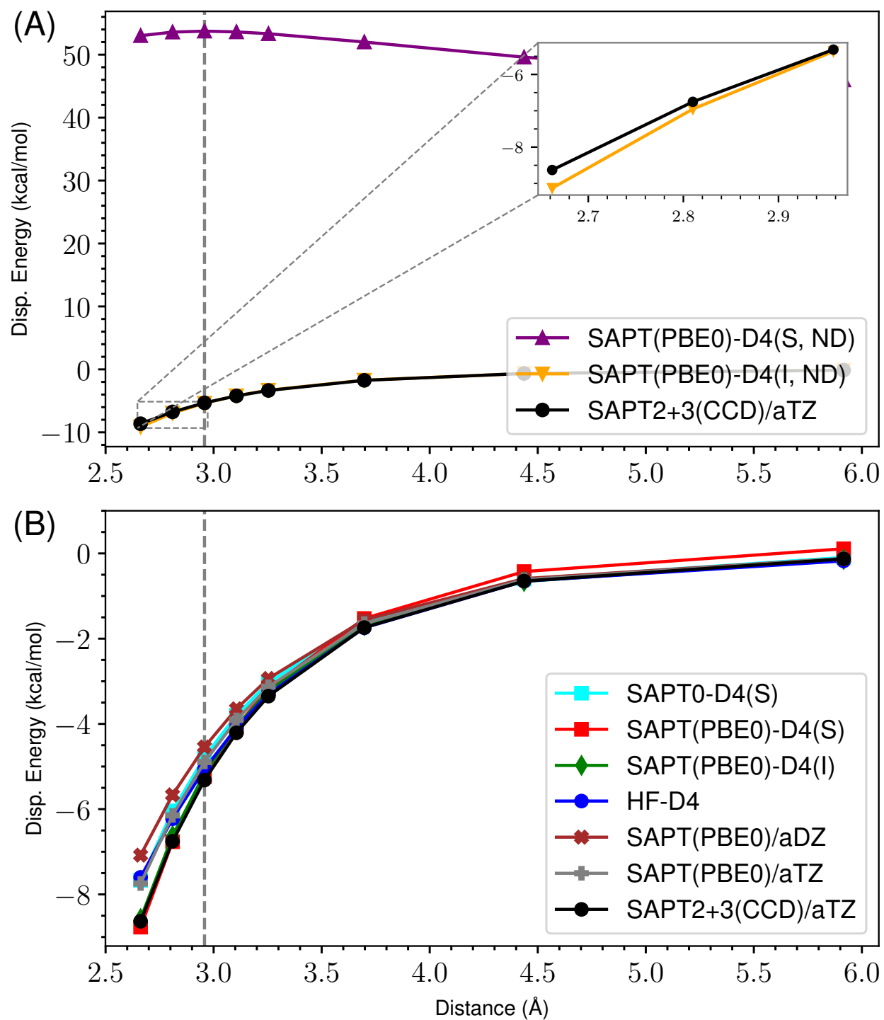
Figure 23: ND vs Damped D4 Dispersion for s66x8 31_Uracil-Ethene
