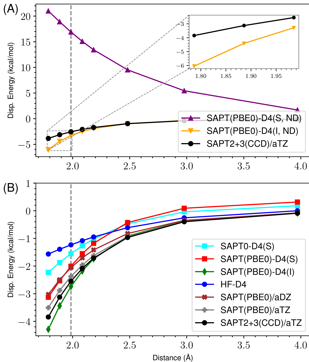
Figure 55: ND vs Damped D4 Dispersion for s66x8 08_MeOH-Water
