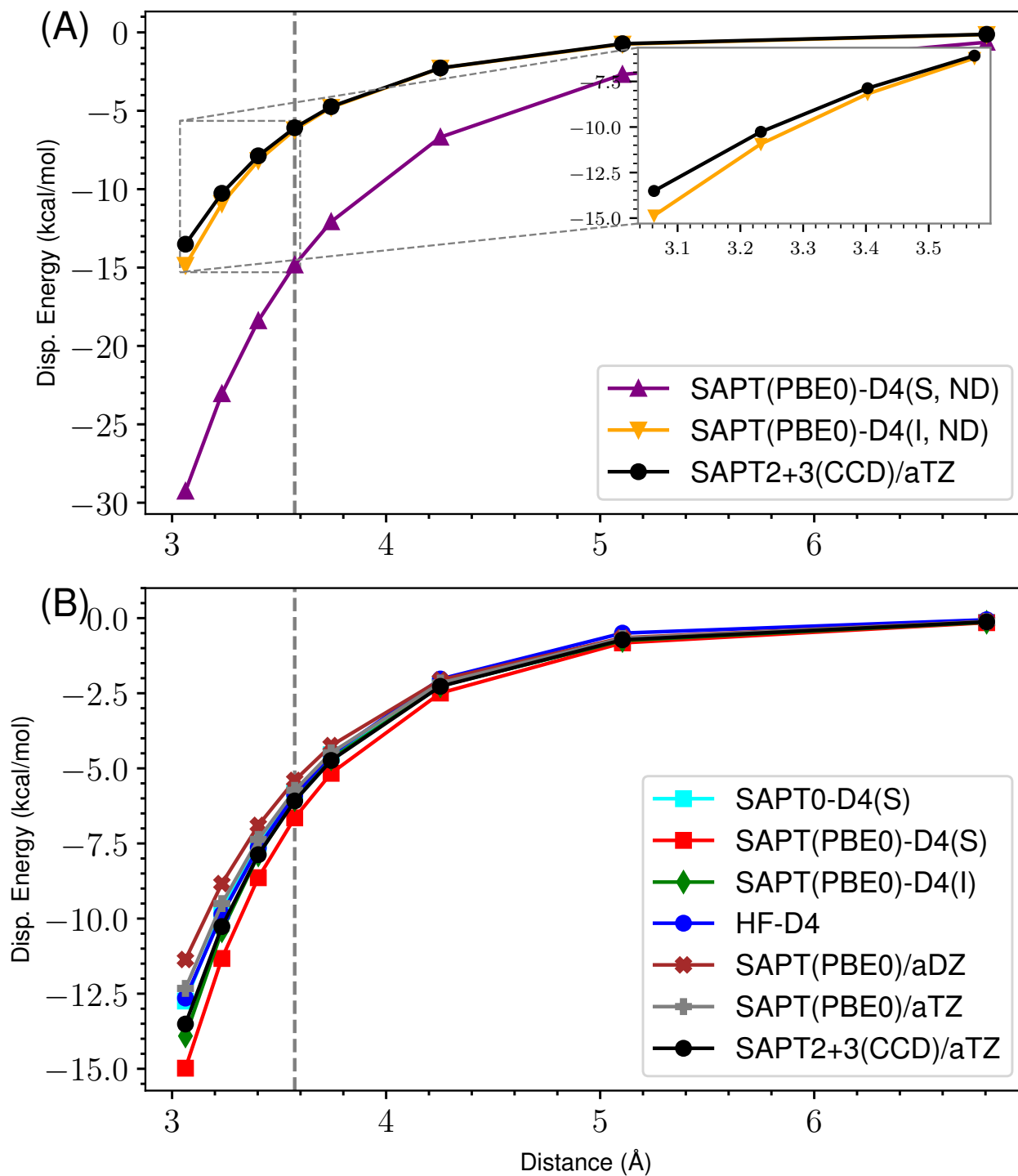
Figure 37: ND vs Damped D4 Dispersion for s66x8 24_Benzene-Benzene
