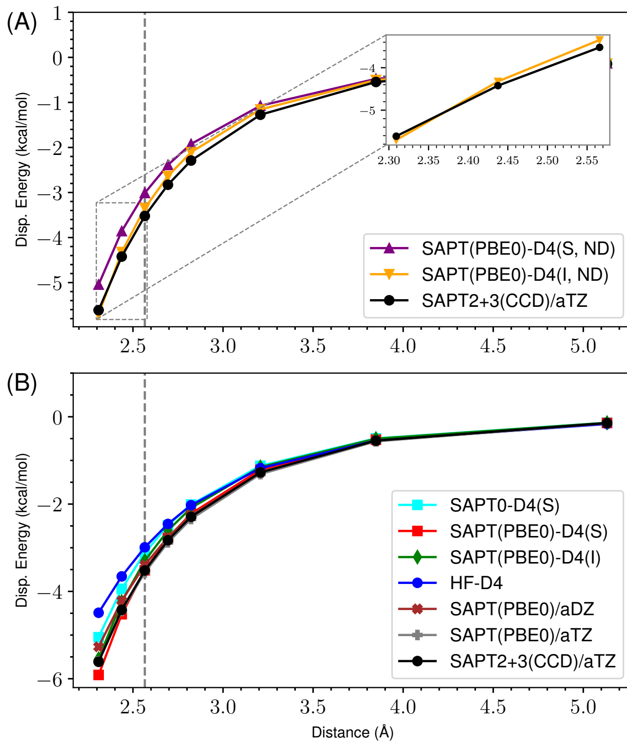
Figure 62: ND vs Damped D4 Dispersion for s66x8 36_Neopentane-Neopentane
