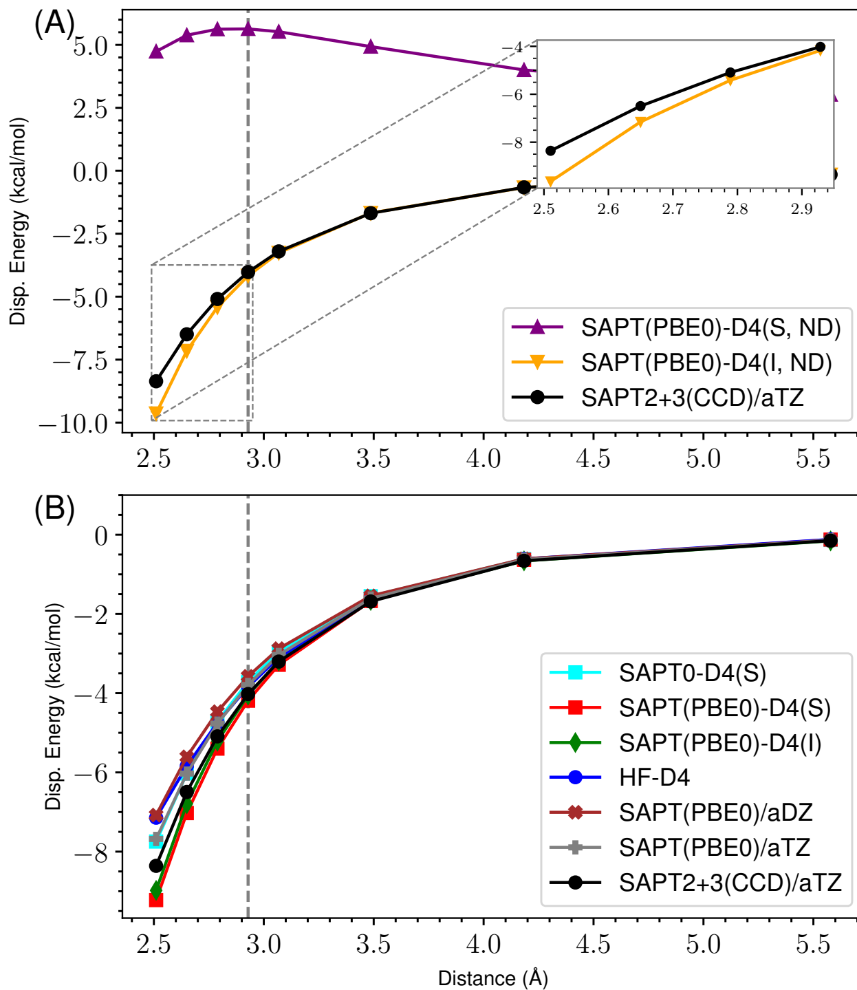
Figure 64: ND vs Damped D4 Dispersion for s66x8 49_Benzene-Pyridine
