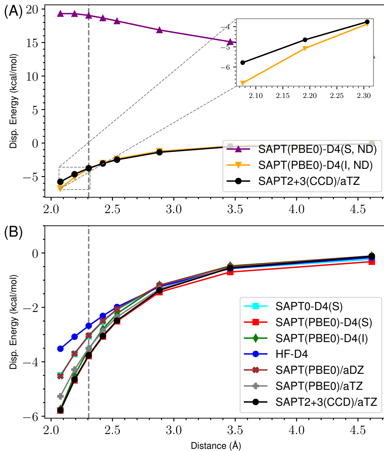
Figure 58: ND vs Damped D4 Dispersion for s66x8 60_Ethyne-AcOH
