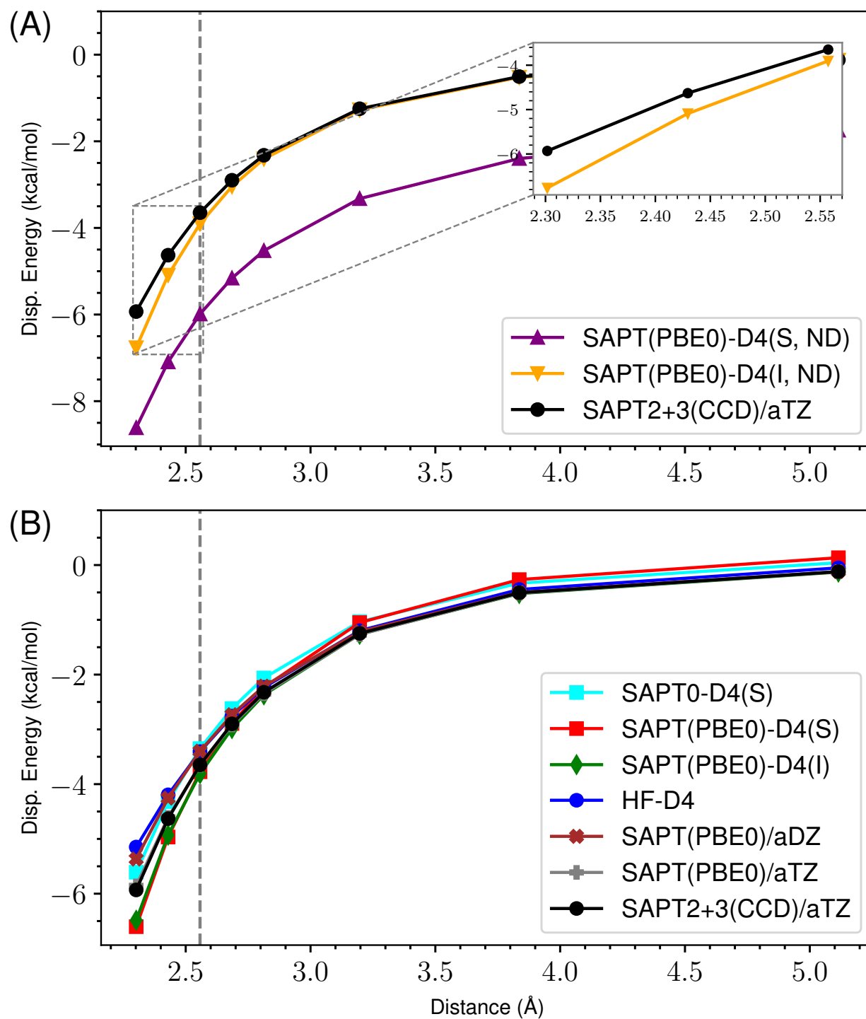
Figure 7: ND vs Damped D4 Dispersion for s66x8 44_Ethene-Pentane
