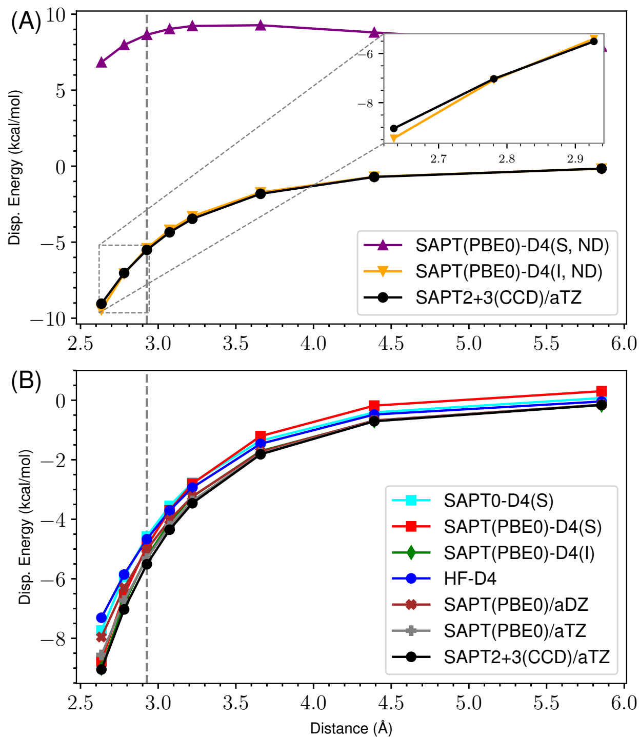
Figure 59: ND vs Damped D4 Dispersion for s66x8 40_Benzene-Neopentane
