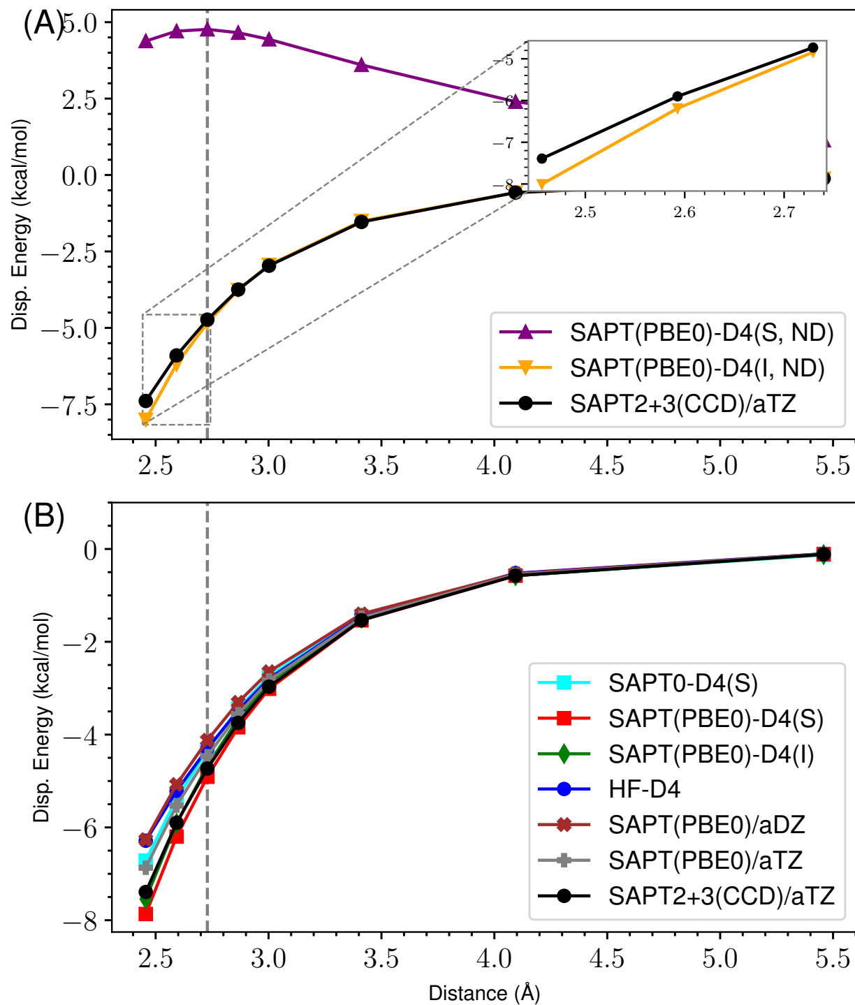
Figure 44: ND vs Damped D4 Dispersion for s66x8 56_Benzene-MeNH2
