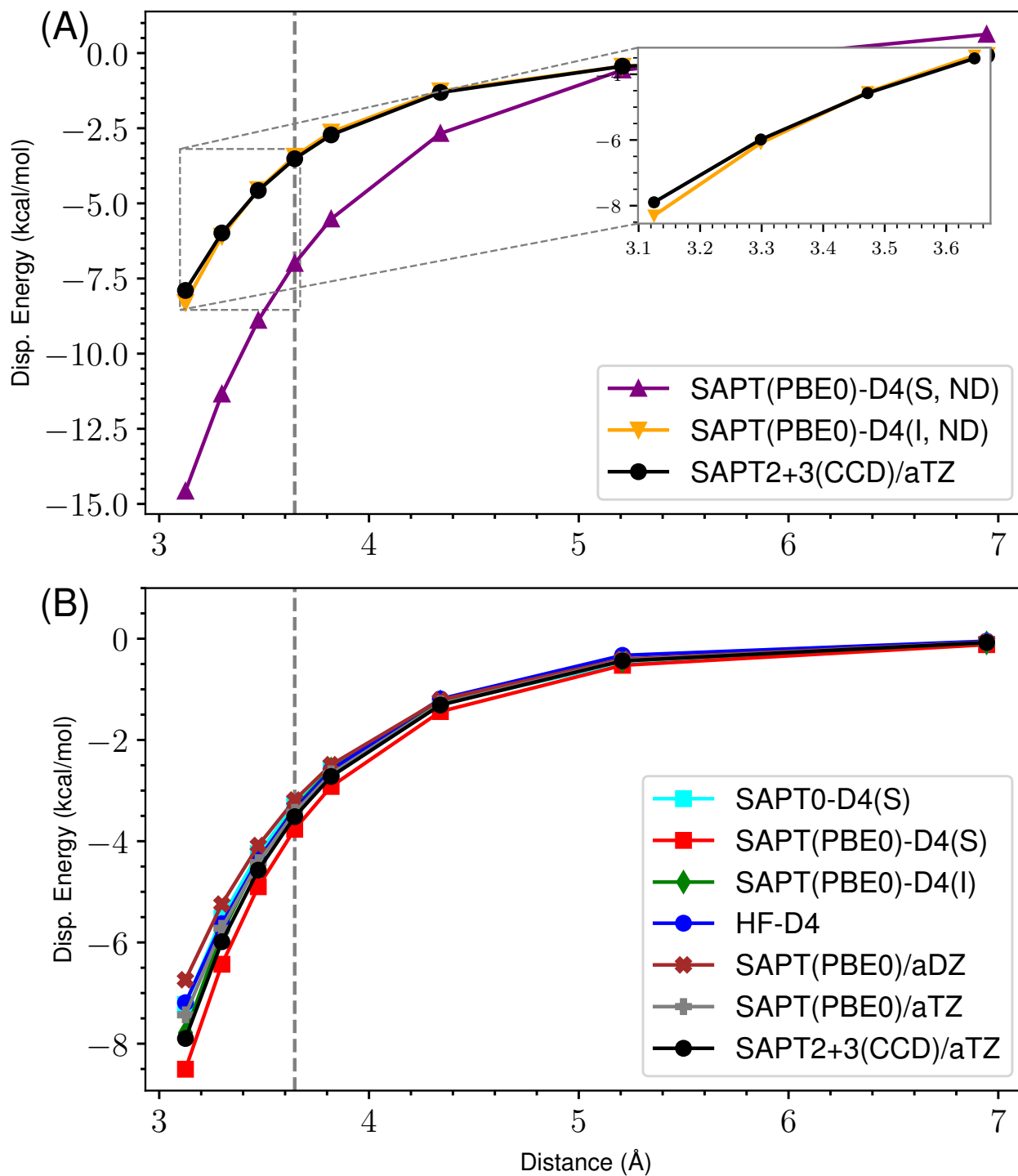
Figure 43: ND vs Damped D4 Dispersion for s66x8 30_Benzene-Ethene
