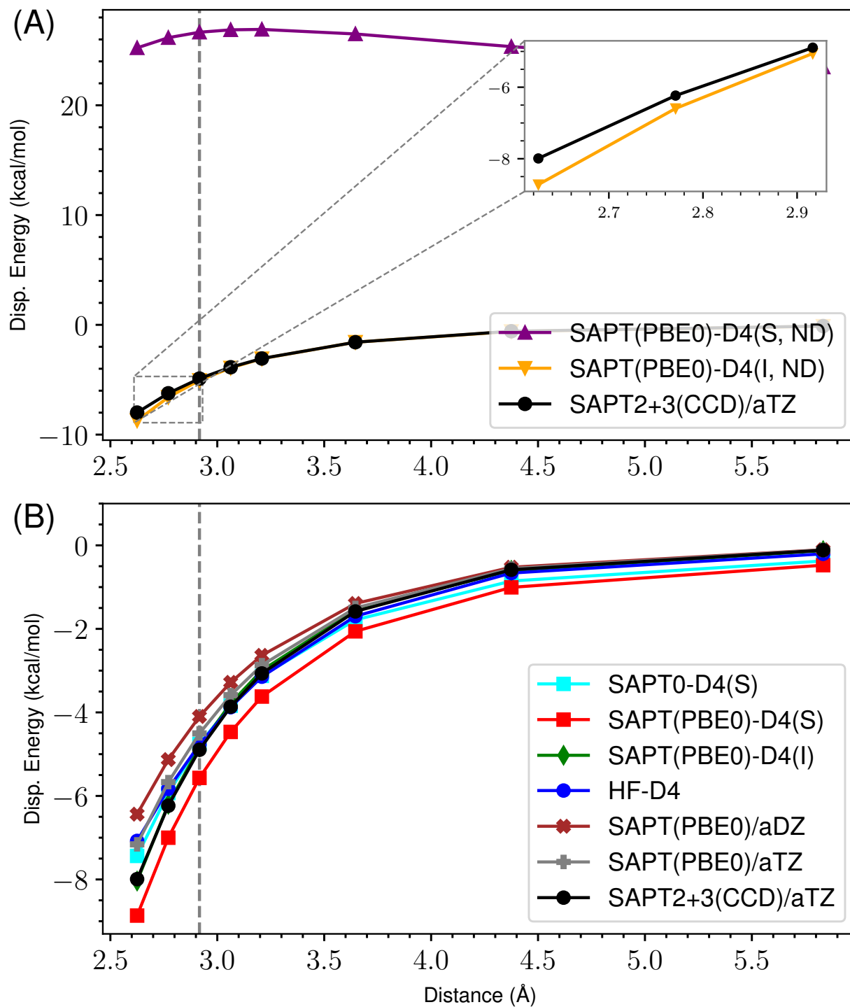
Figure 65: ND vs Damped D4 Dispersion for s66x8 32_Uracil-Ethyne
