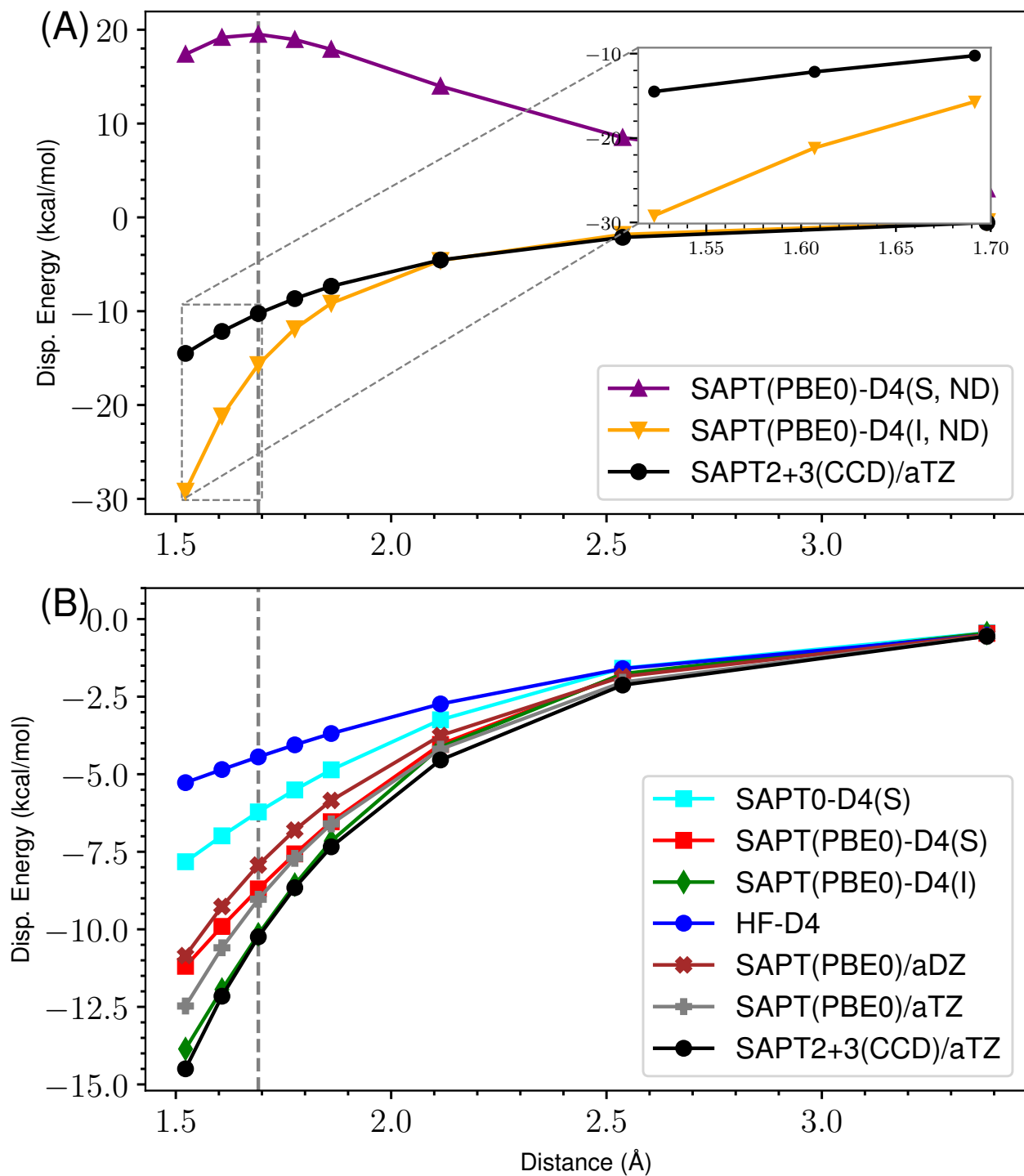
Figure 34: ND vs Damped D4 Dispersion for s66x8 20_AcOH-AcOH
