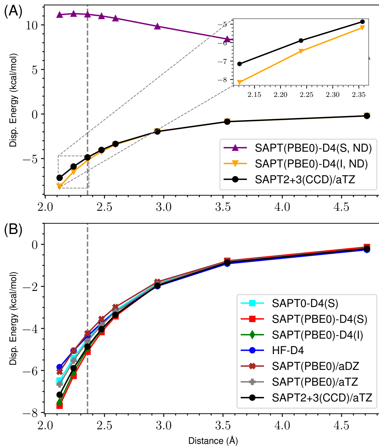
Figure 38: ND vs Damped D4 Dispersion for s66x8 66_MeNH2-Pyridine
