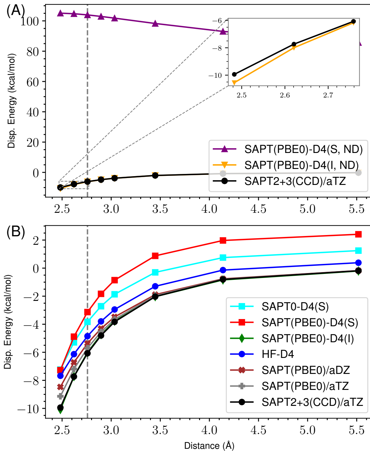
Figure 53: ND vs Damped D4 Dispersion for s66x8 43_Uracil-Neopentane
