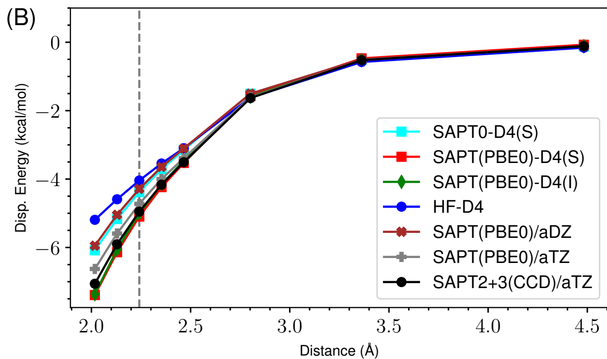
Figure 52: ND vs Damped D4 Dispersion for s66x8 11_MeNH2-Peptide
