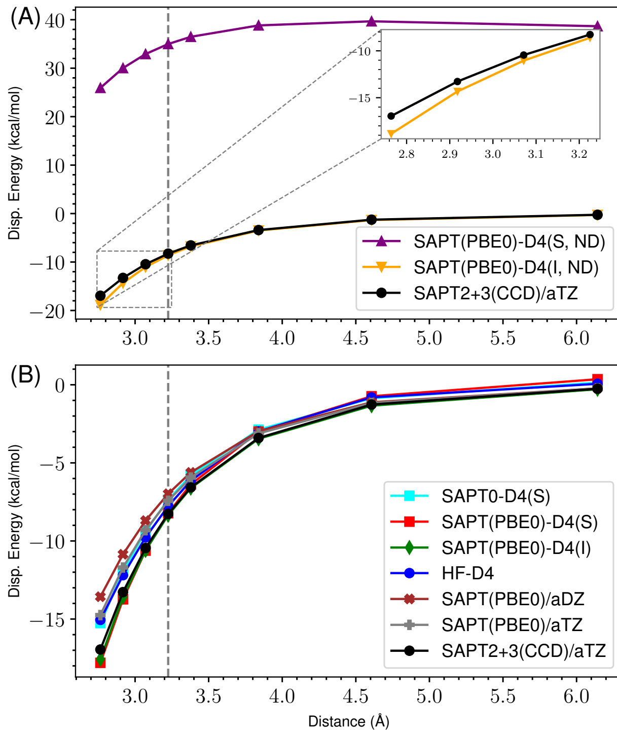
Figure 4: ND vs Damped D4 Dispersion for s66x8 28_Benzene-Uracil
