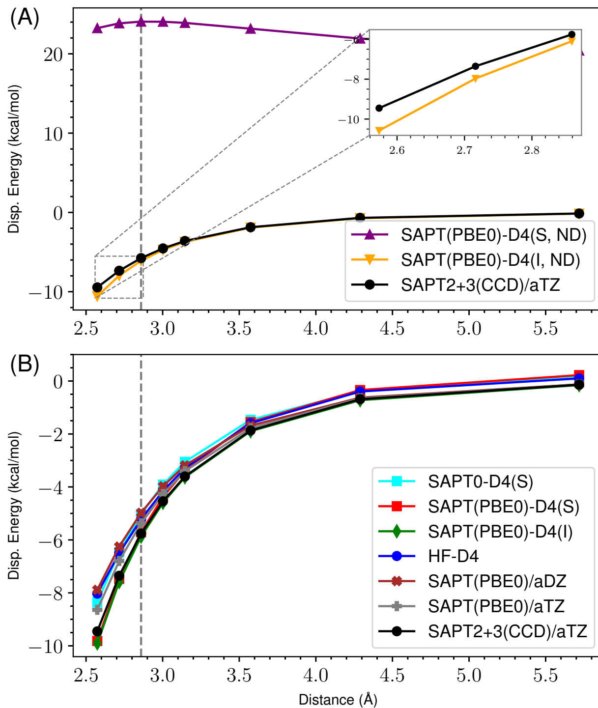
Figure 39: ND vs Damped D4 Dispersion for s66x8 63.Benzene-AcOH
