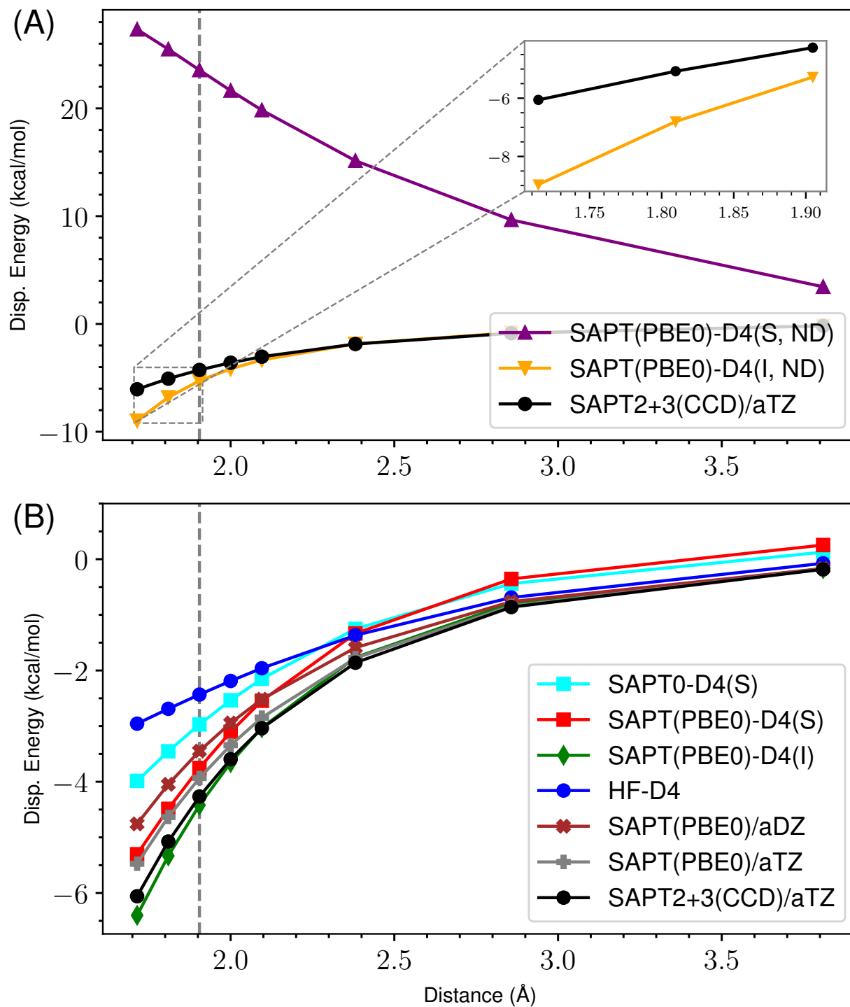
Figure 25: ND vs Damped D4 Dispersion for s66x8 04_Water-Peptide
