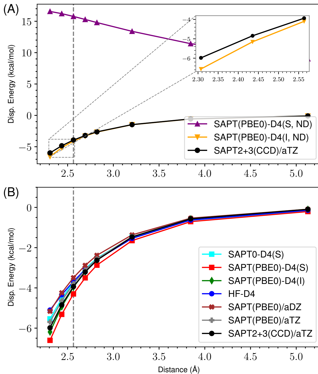
Figure 31: ND vs Damped D4 Dispersion for s66x8 64_Peptide-Ethene
