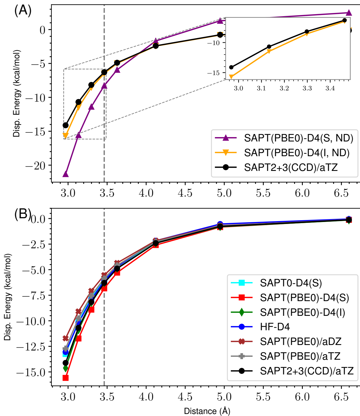
Figure 11: ND vs Damped D4 Dispersion for s66x8 27_Benzene-Pyridine
