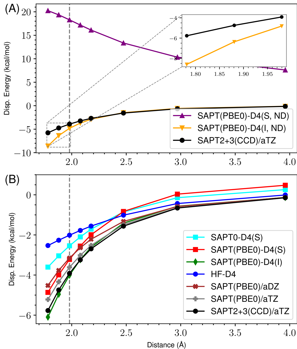
Figure 60: ND vs Damped D4 Dispersion for s66x8 12_MeNH2-Water
