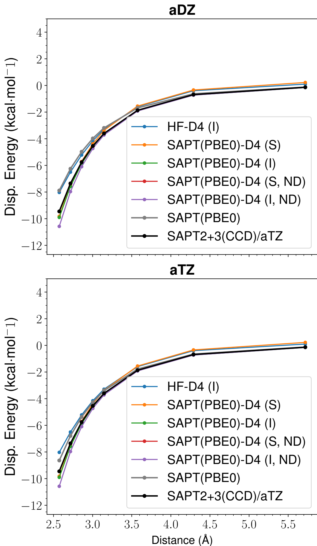
Figure 8: LoS Dispersion Curves for s66x8 63_Benzene-AcOH
