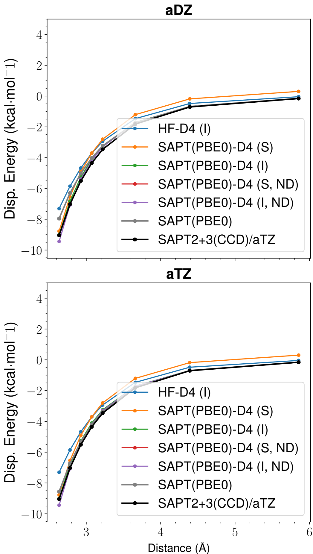
Figure 42: LoS Dispersion Curves for s66x8 40_Benzene-Neopentane
