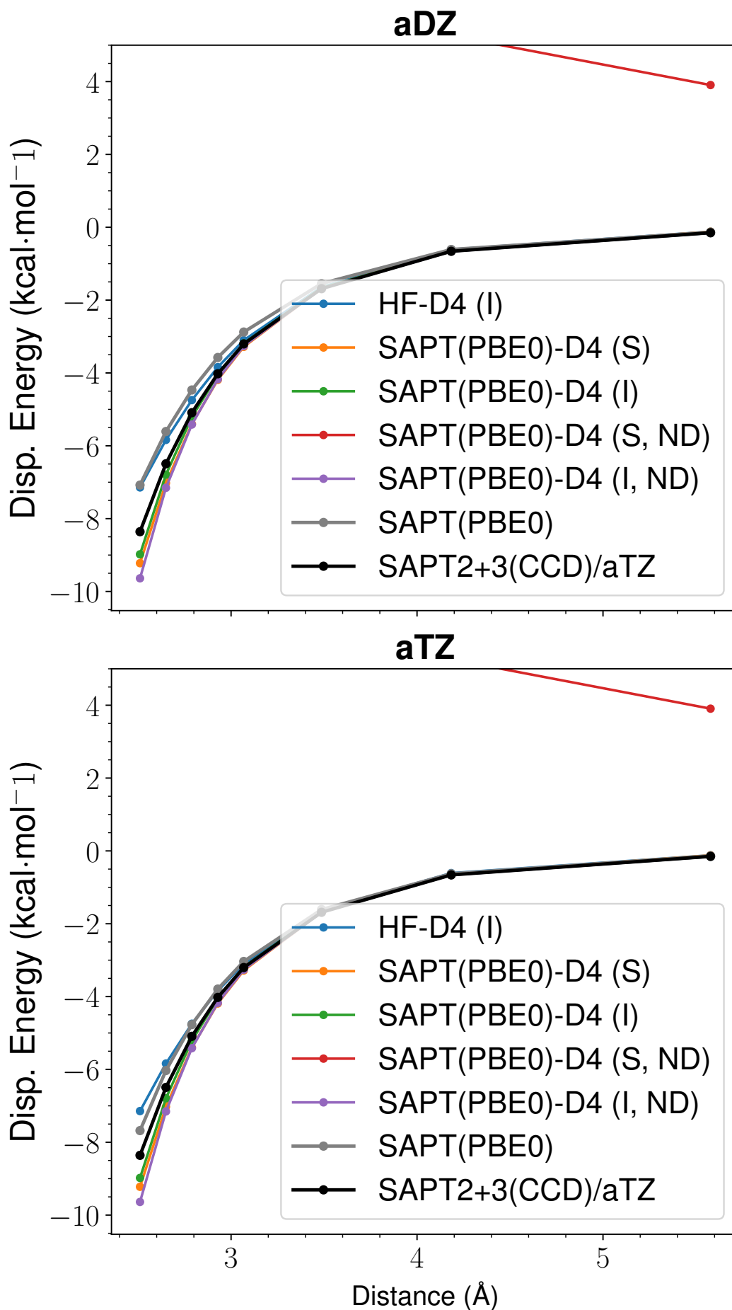
Figure 6: LoS Dispersion Curves for s66x8 49_Benzene-Pyridine
