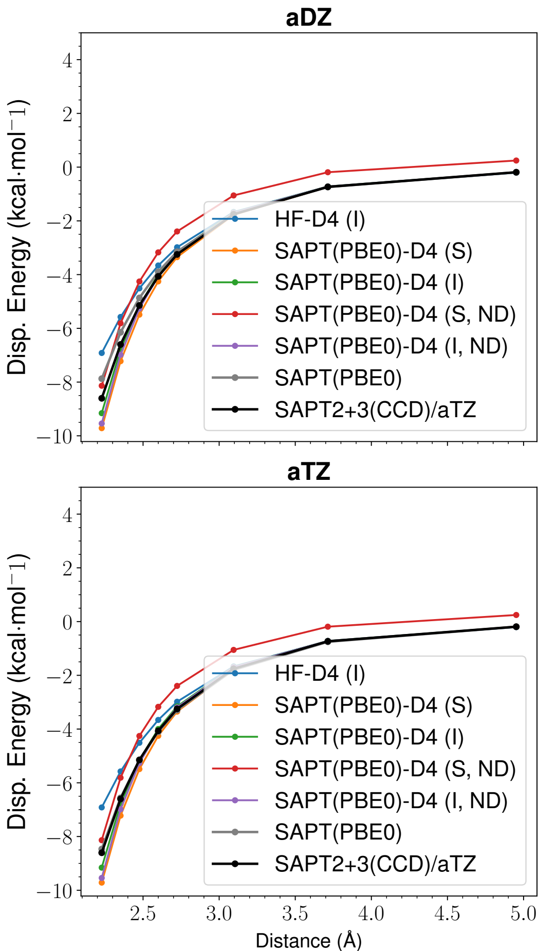
Figure 30: LoS Dispersion Curves for s66x8 35_Neopentane-Pentane
