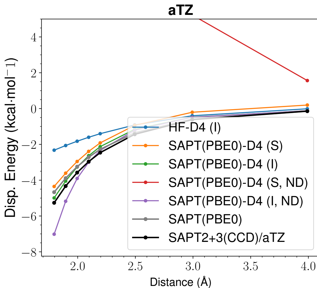
Figure 55: LoS Dispersion Curves for s66x8 18_Water-Pyridine
