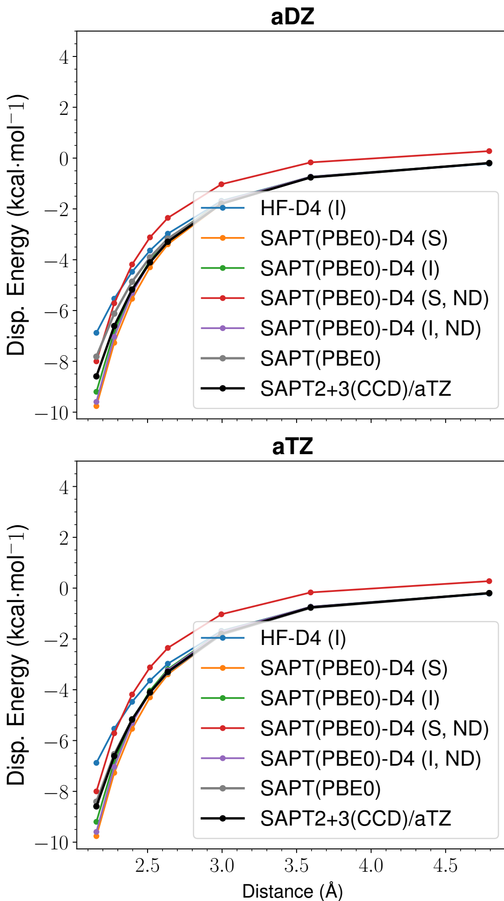
Figure 66: LoS Dispersion Curves for s66x8 37_Cyclopentane-Neopentane
