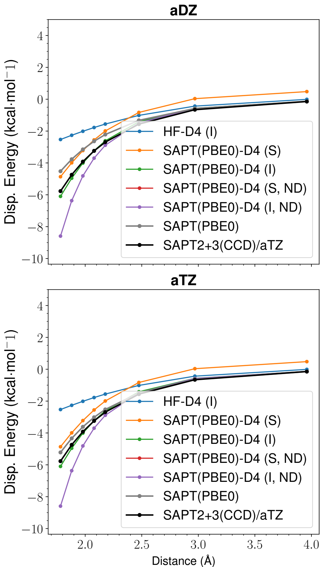
Figure 21: LoS Dispersion Curves for s66x8 12_MeNH2-Water
