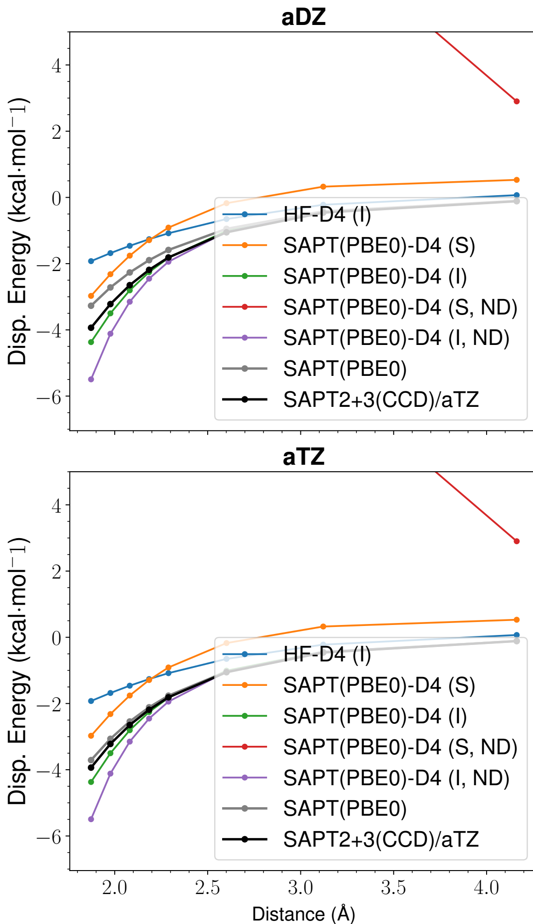
Figure 51: LoS Dispersion Curves for s66x8 16_Peptide-Water
