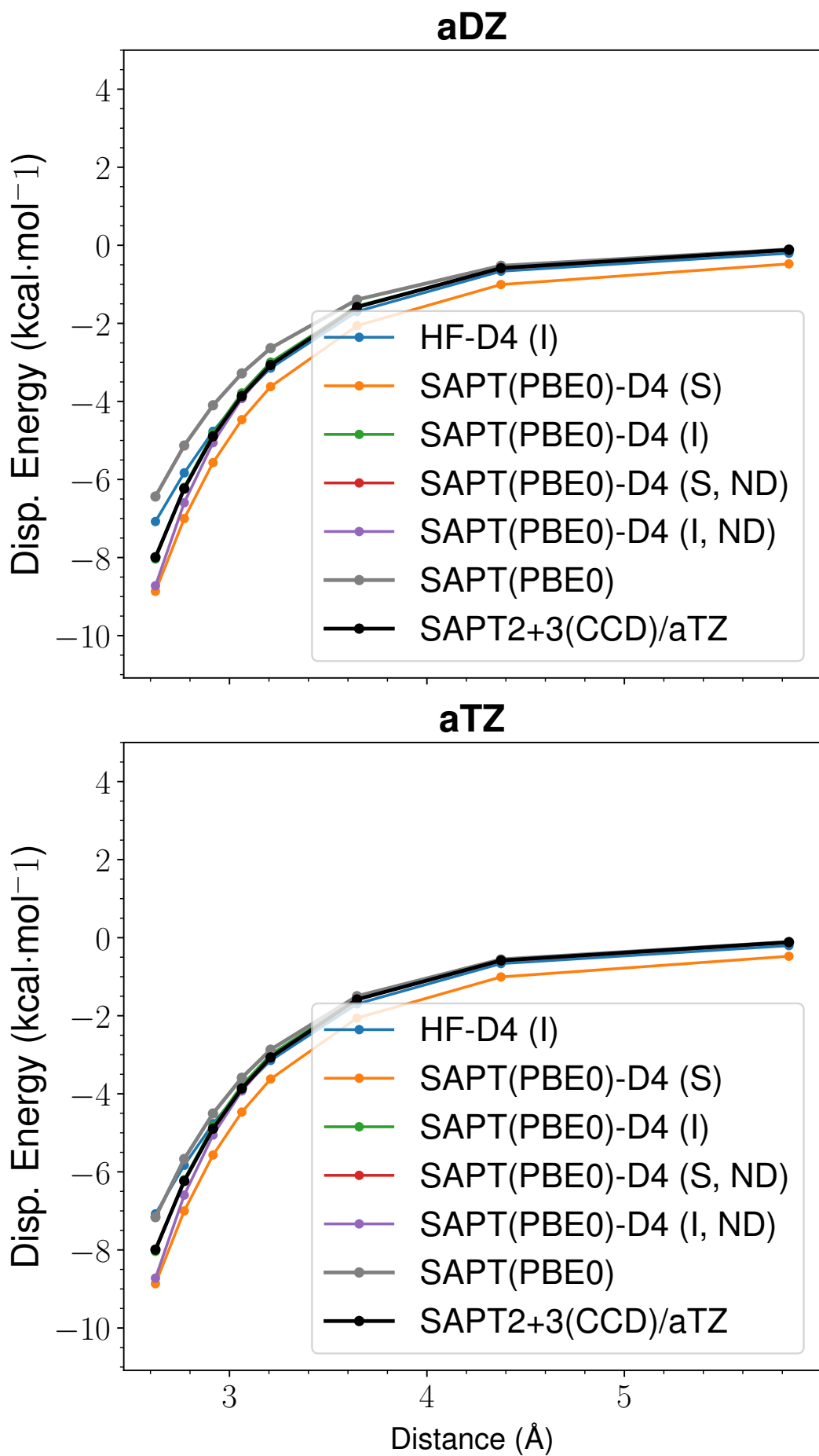
Figure 24: LoS Dispersion Curves for s66x8 32_Uracil-Ethyne
