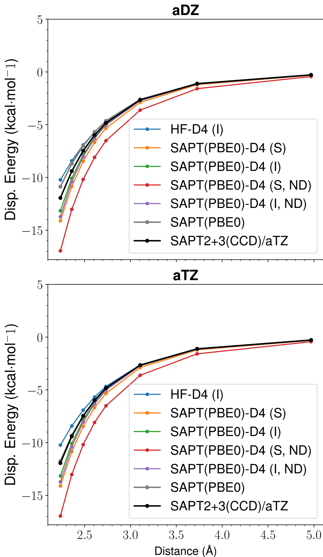
Figure 29: LoS Dispersion Curves for s66x8 34_Pentane-Pentane
