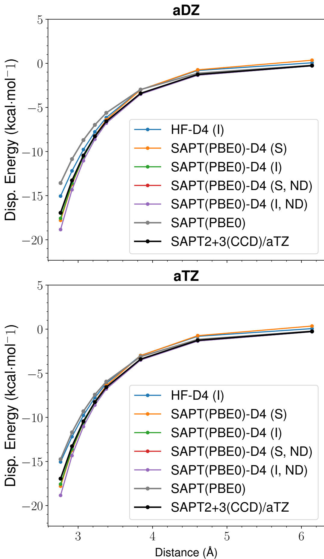
Figure 5: LoS Dispersion Curves for s66x8 28_Benzene-Uracil
