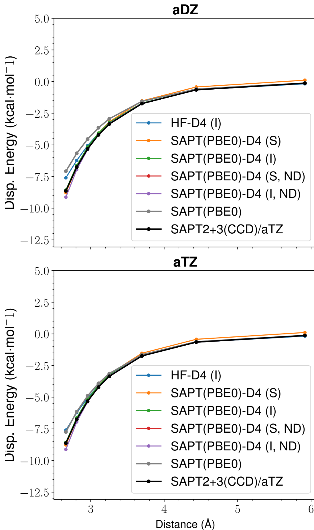
Figure 26: LoS Dispersion Curves for s66x8 31_Uracil-Ethene
