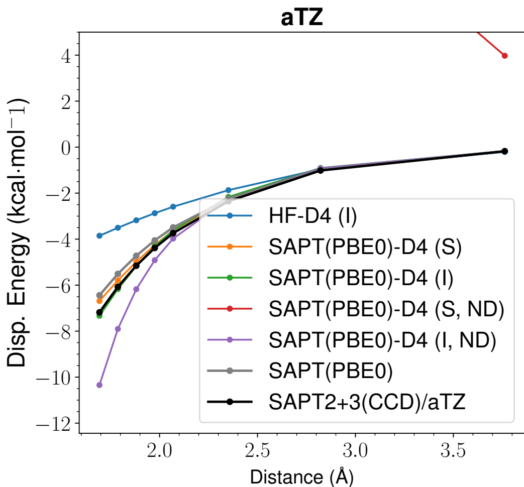
Figure 62: LoS Dispersion Curves for s66x8 07_MeOH-Peptide
