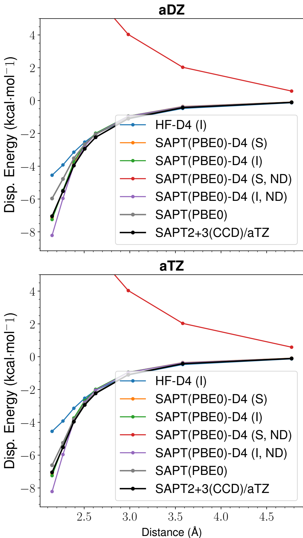
Figure 18: LoS Dispersion Curves for s66x8 58_Pyridine-Pyridine
