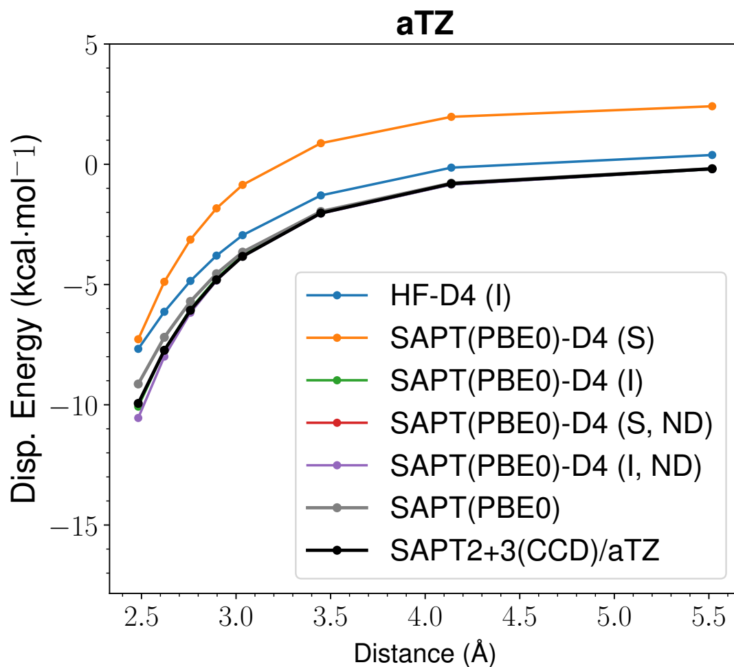
Figure 39: LoS Dispersion Curves for s66x8 43_Uracil-Neopentane
