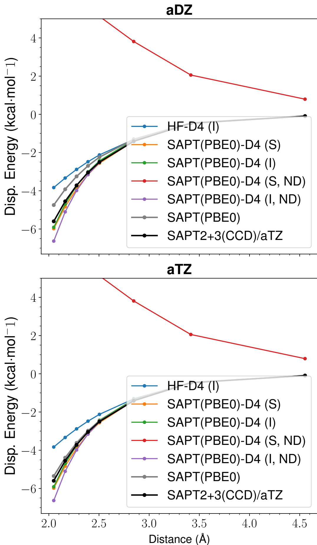
Figure 17: LoS Dispersion Curves for s66x8 10_MeNH2-MeNH2
