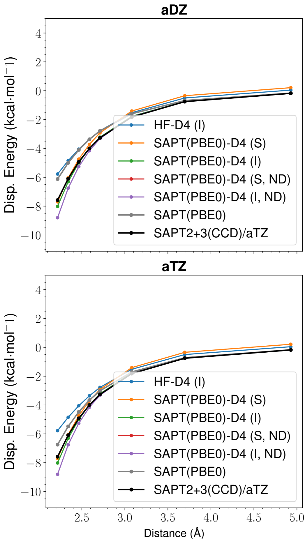
Figure 14: LoS Dispersion Curves for s66x8 52_Benzene-AcOH
