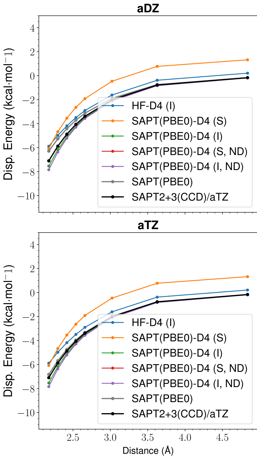
Figure 35: LoS Dispersion Curves for s66x8 61_Pentane-AcOH
