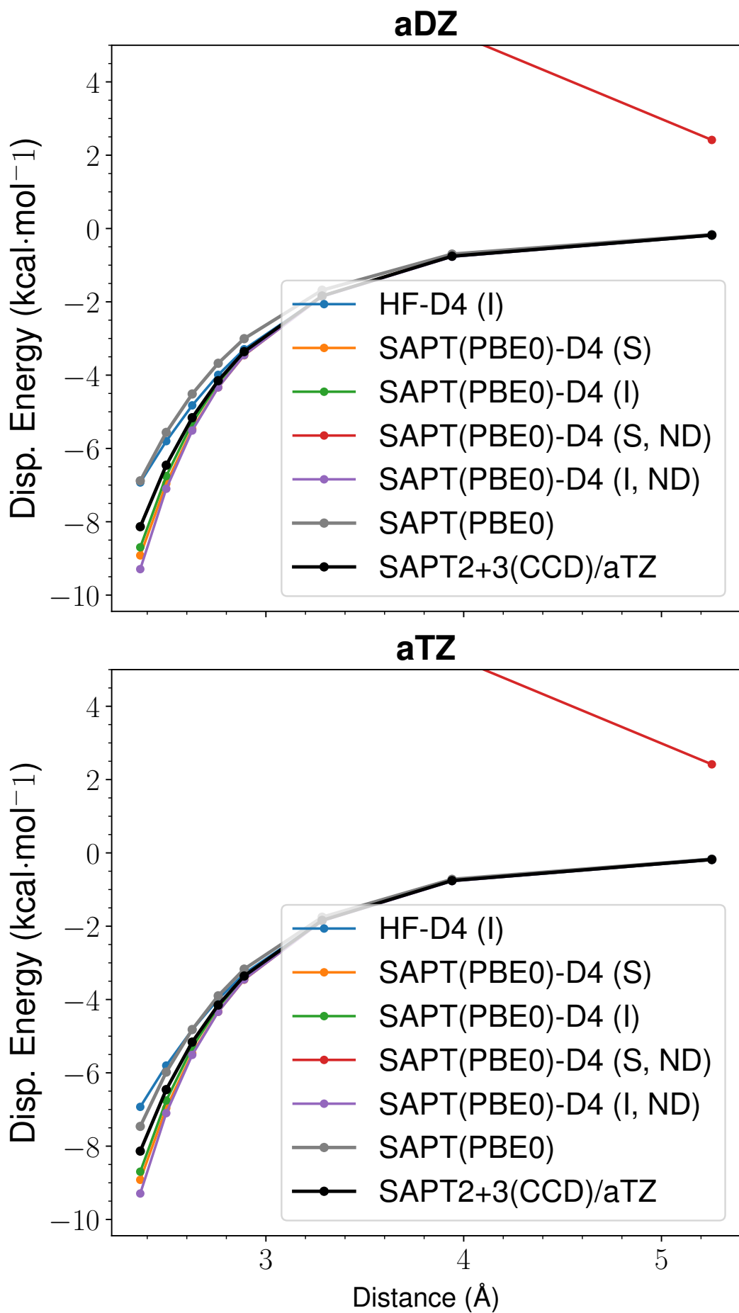
Figure 40: LoS Dispersion Curves for s66x8 48_Pyridine-Pyridine
