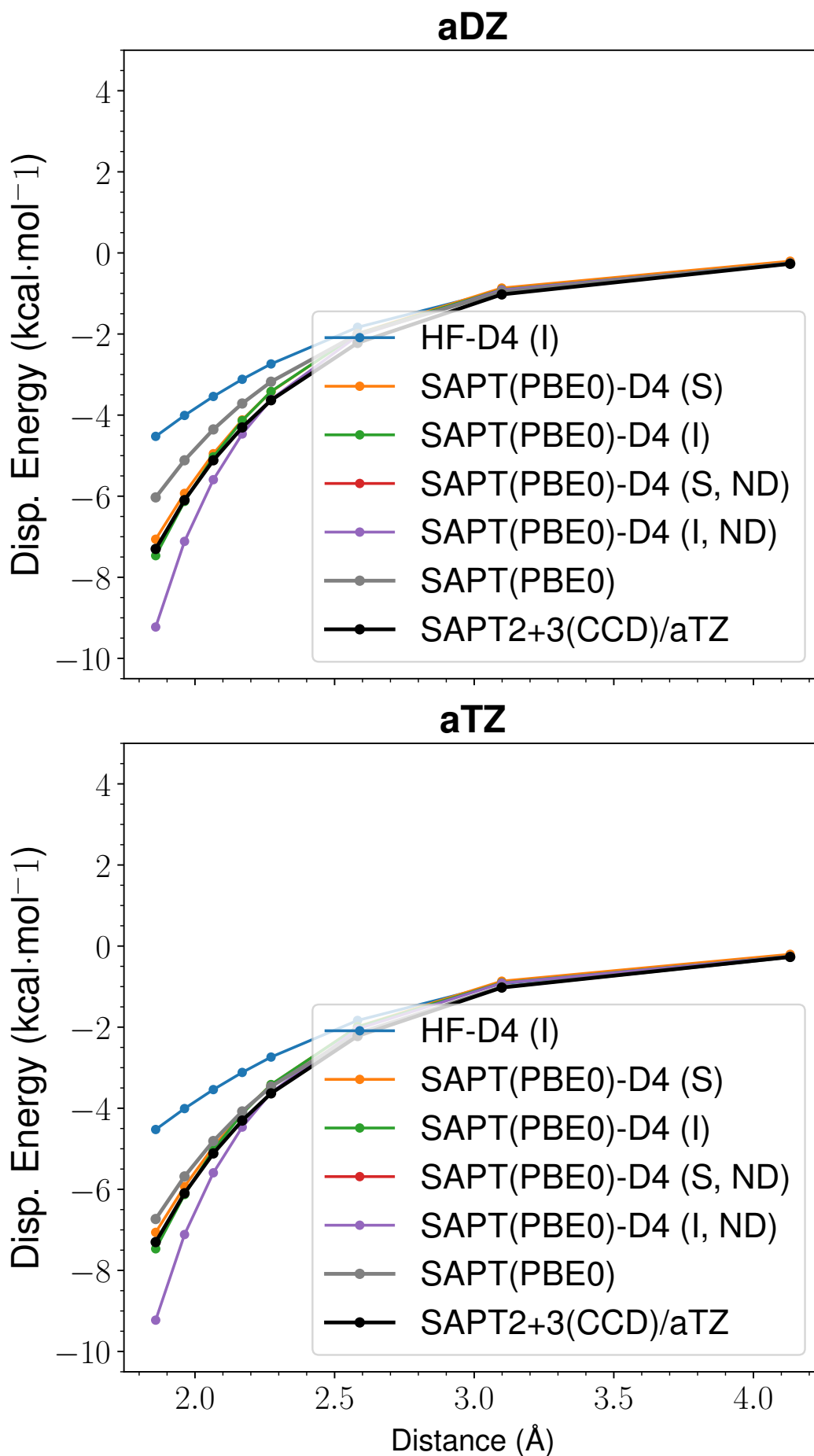
Figure 63: LoS Dispersion Curves for s66x8 14_Peptide-MeNH2
