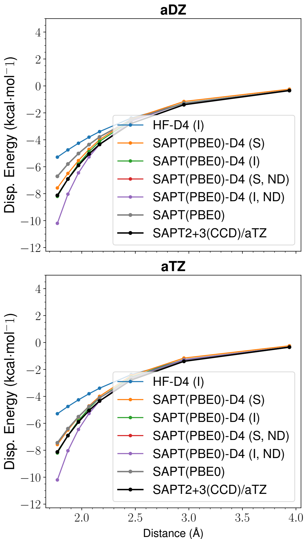
Figure 36: LoS Dispersion Curves for s66x8 15_Peptide-Peptide
