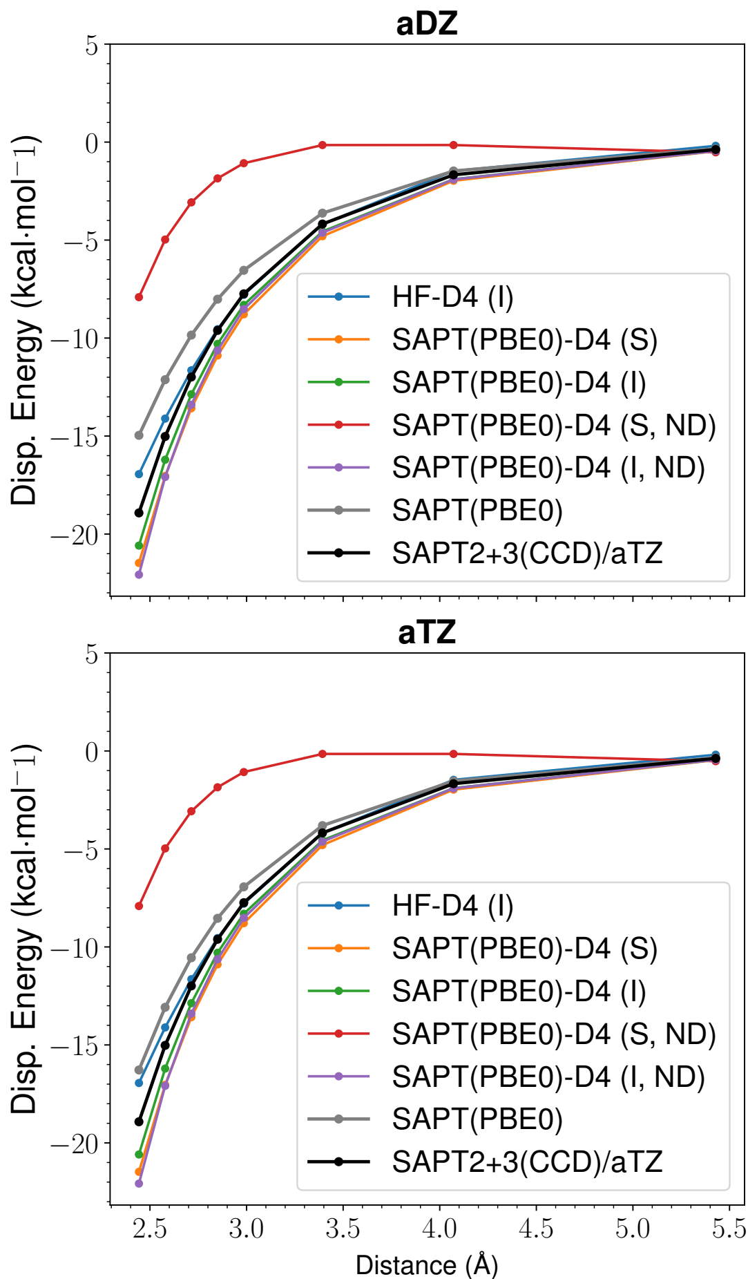
Figure 53: LoS Dispersion Curves for s66x8 26_Uracil-Uracil
