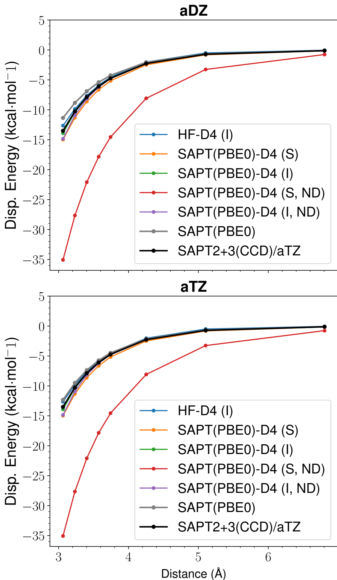
Figure 31: LoS Dispersion Curves for s66x8 24_Benzene-Benzene
