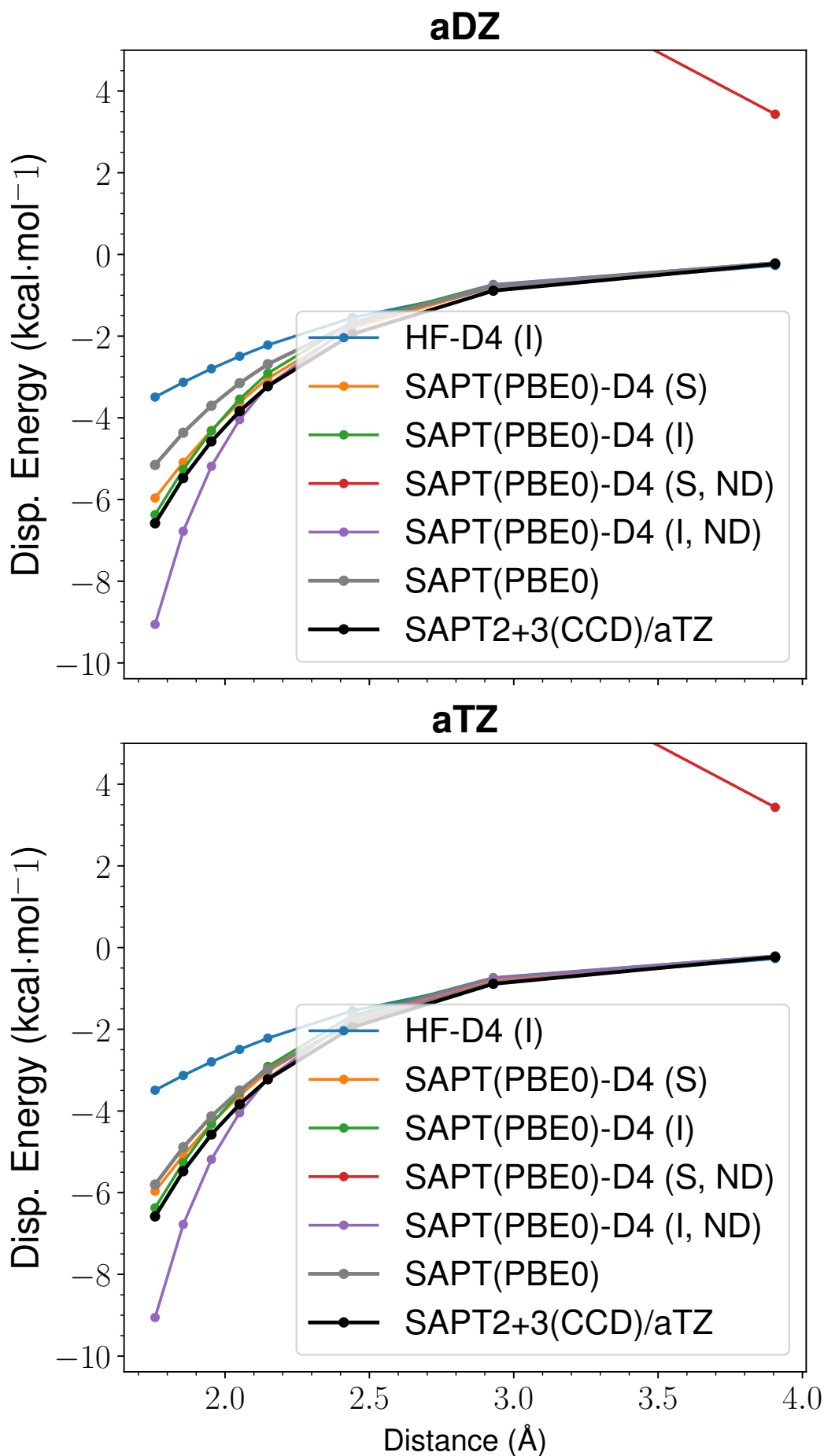
Figure 57: LoS Dispersion Curves for s66x8 19_MeOH-Pyridine
