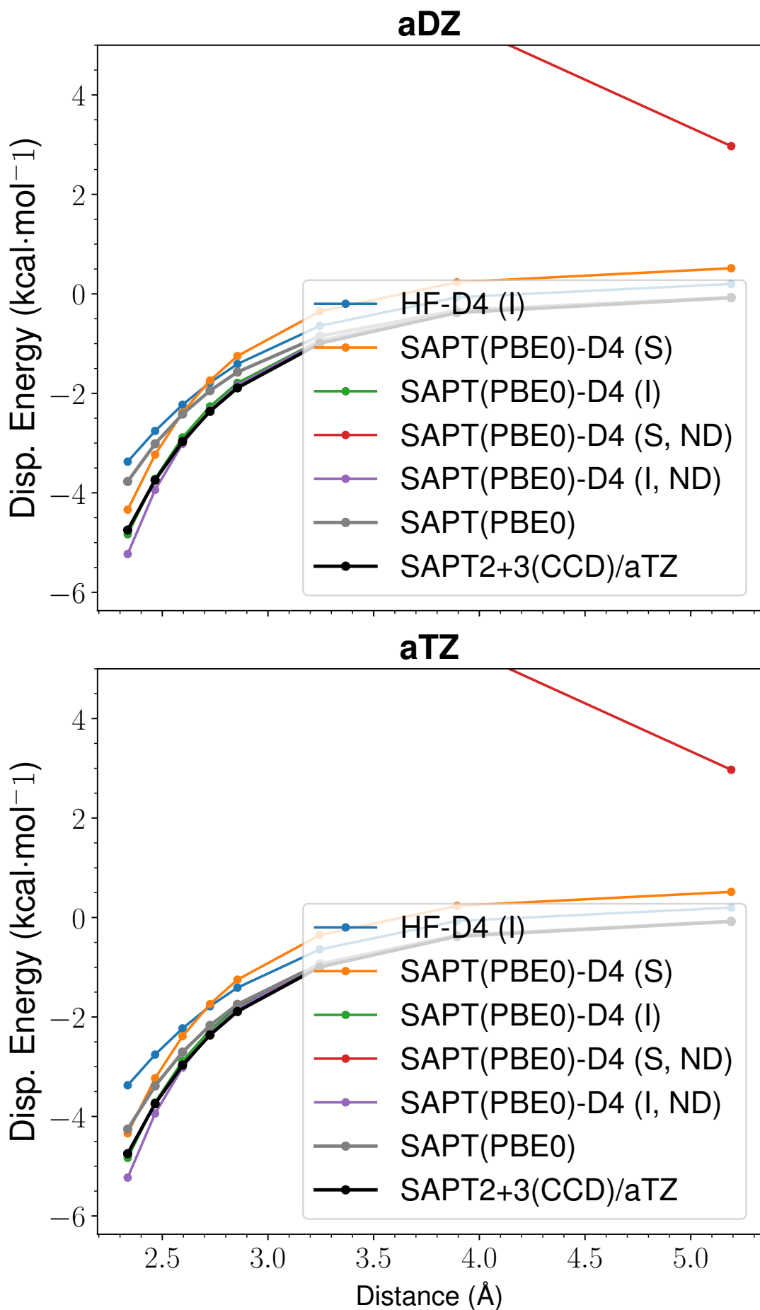
Figure 12: LoS Dispersion Curves for s66x8 54_Benzene-Water
