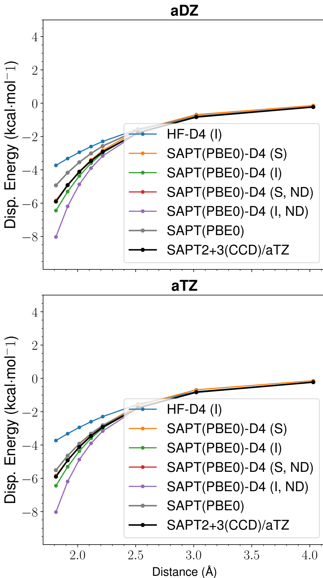
Figure 47: LoS Dispersion Curves for s66x8 13_Peptide-MeOH
