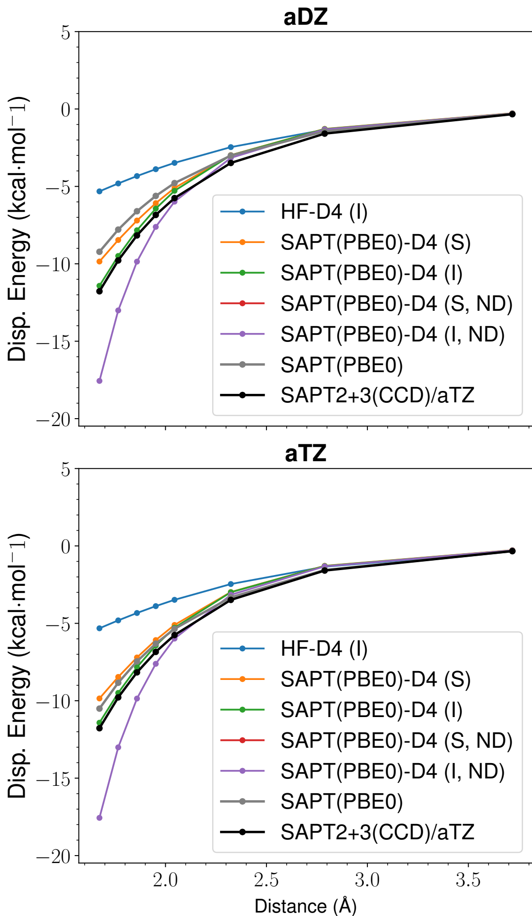
Figure 43: LoS Dispersion Curves for s66x8 21_AcNH2-AcNH2
