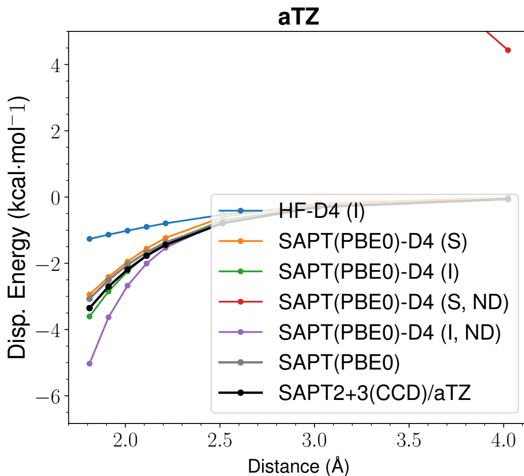
Figure 2: LoS Dispersion Curves for s66x8 01_Water-Water
