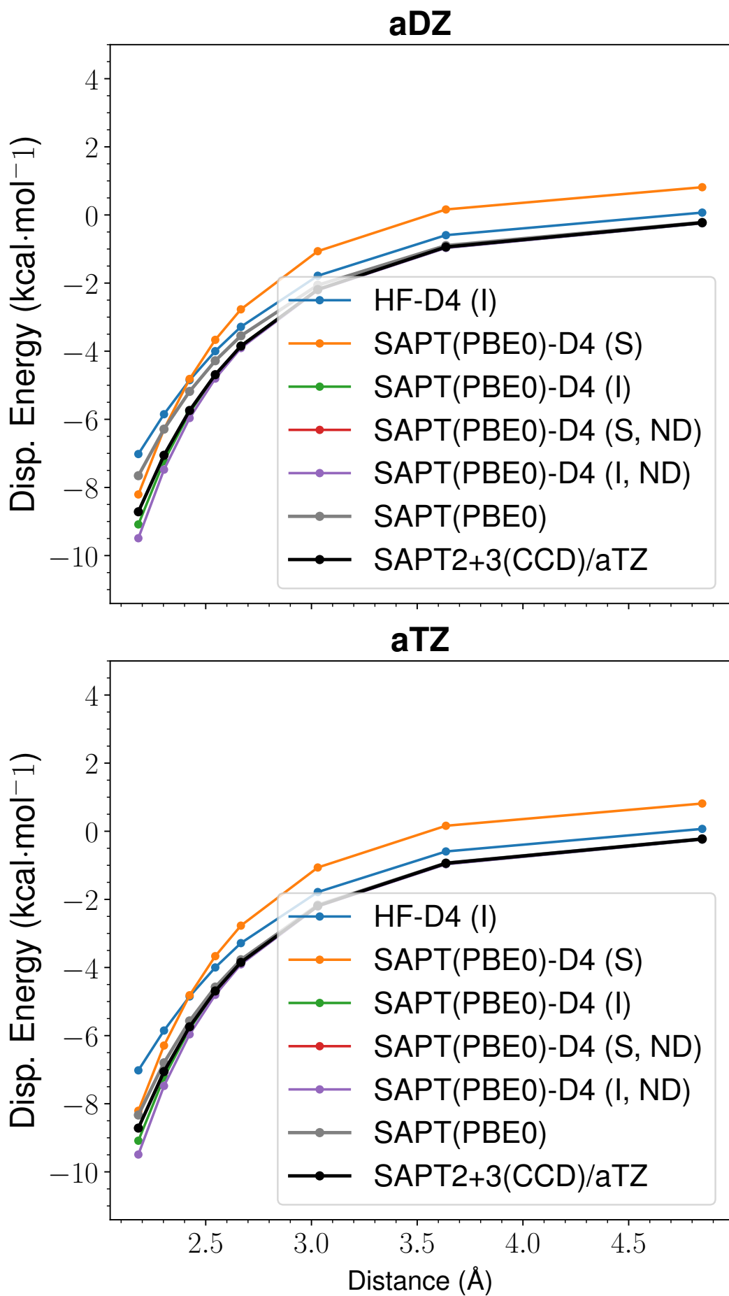
Figure 28: LoS Dispersion Curves for s66x8 62_Pentane-AcNH2
