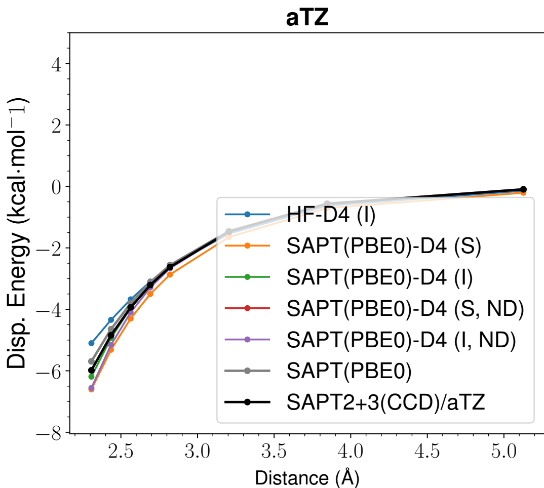
Figure 45: LoS Dispersion Curves for s66x8 64.Peptide-Ethene
