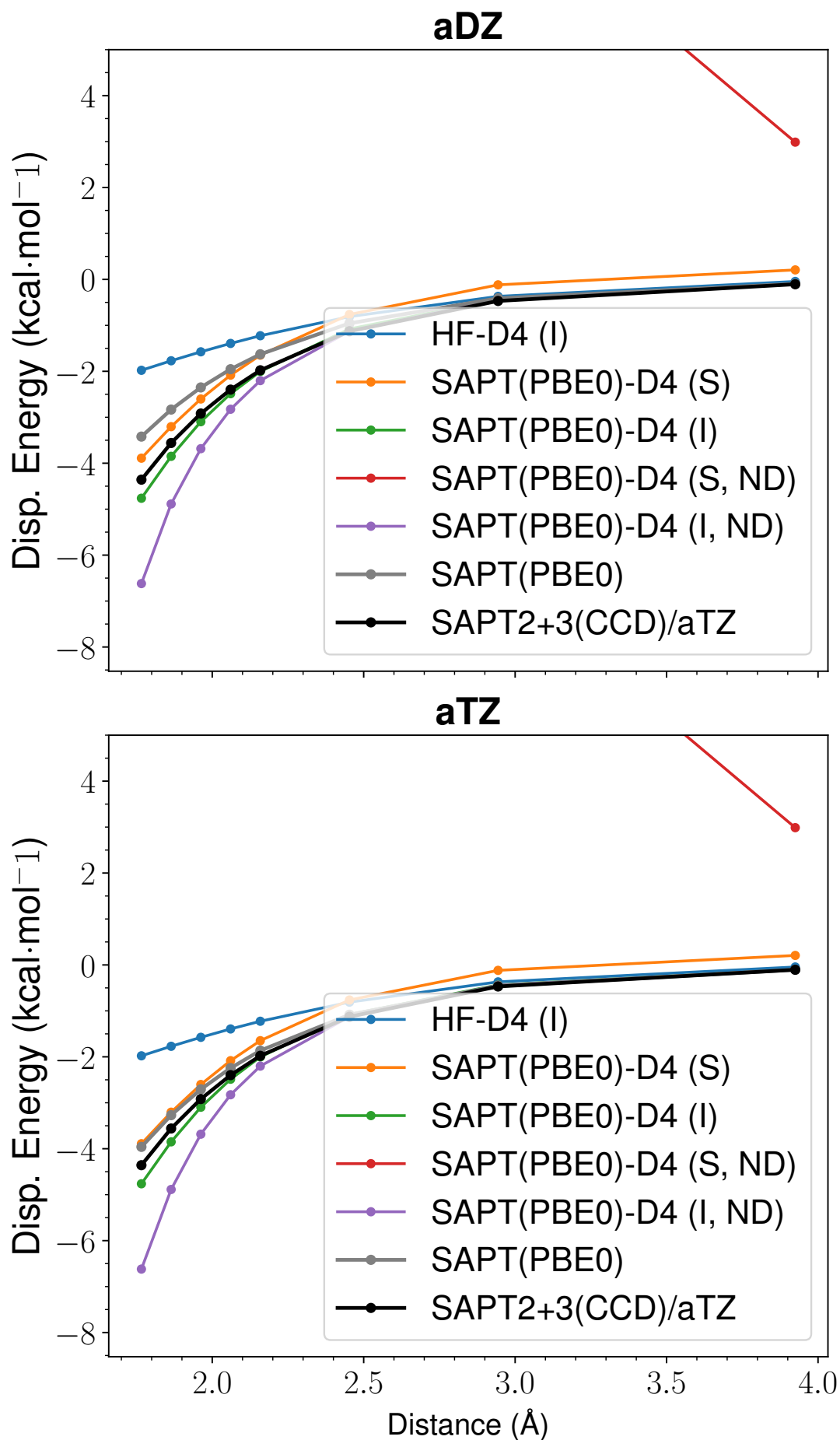
Figure 58: LoS Dispersion Curves for s66x8 02_Water-MeOH
