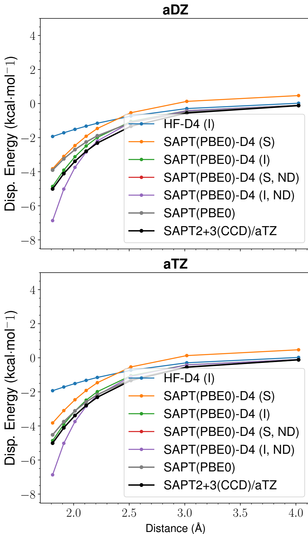
Figure 48: LoS Dispersion Curves for s66x8 03_Water-MeNH2
