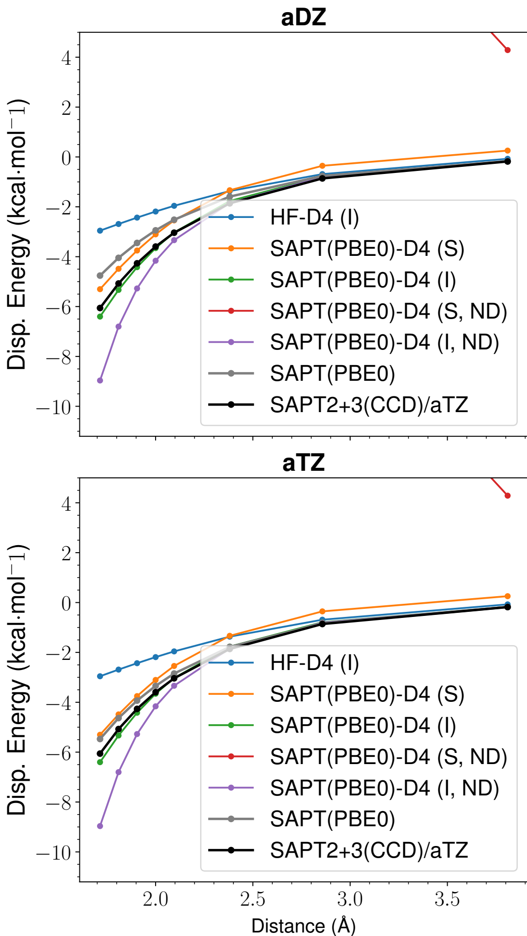
Figure 59: LoS Dispersion Curves for s66x8 04_Water-Peptide
