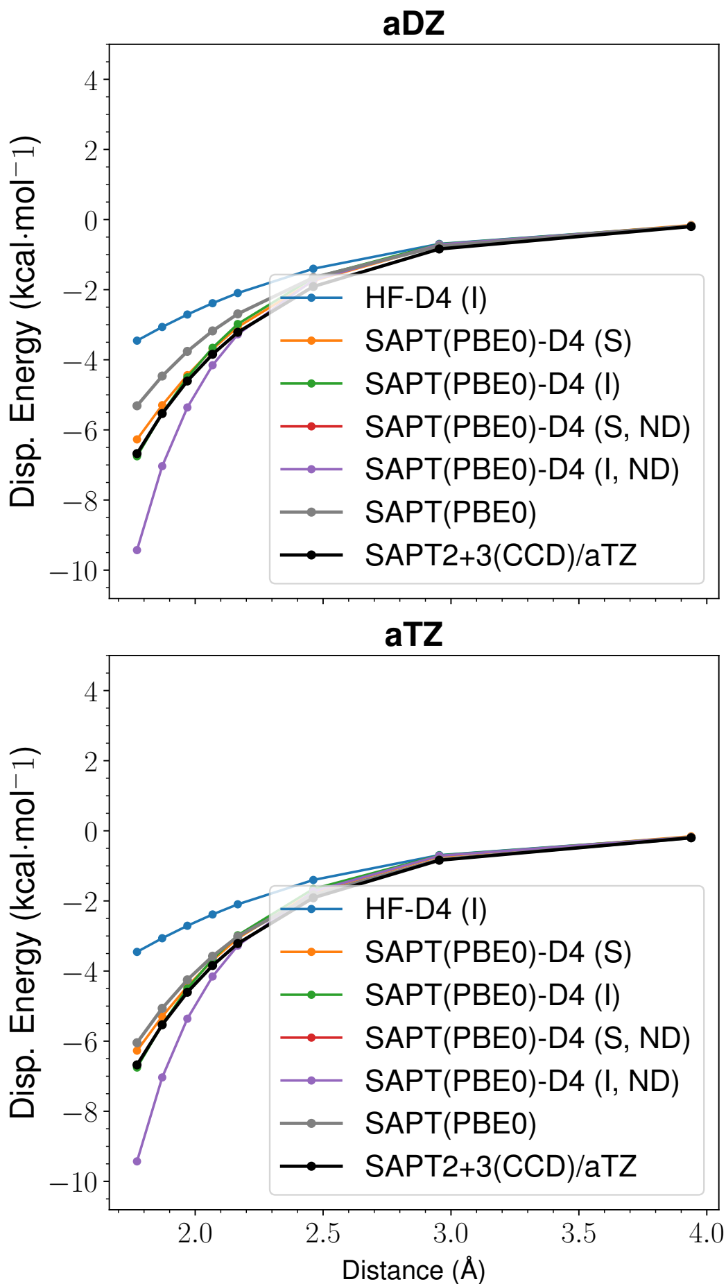
Figure 46: LoS Dispersion Curves for s66x8 06_MeOH-MeNH 2
