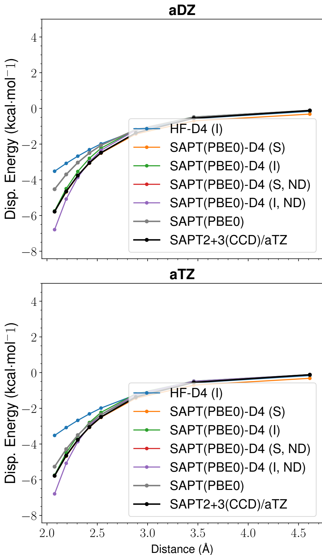
Figure 64: LoS Dispersion Curves for s66x8 60_Ethyne-AcOH
