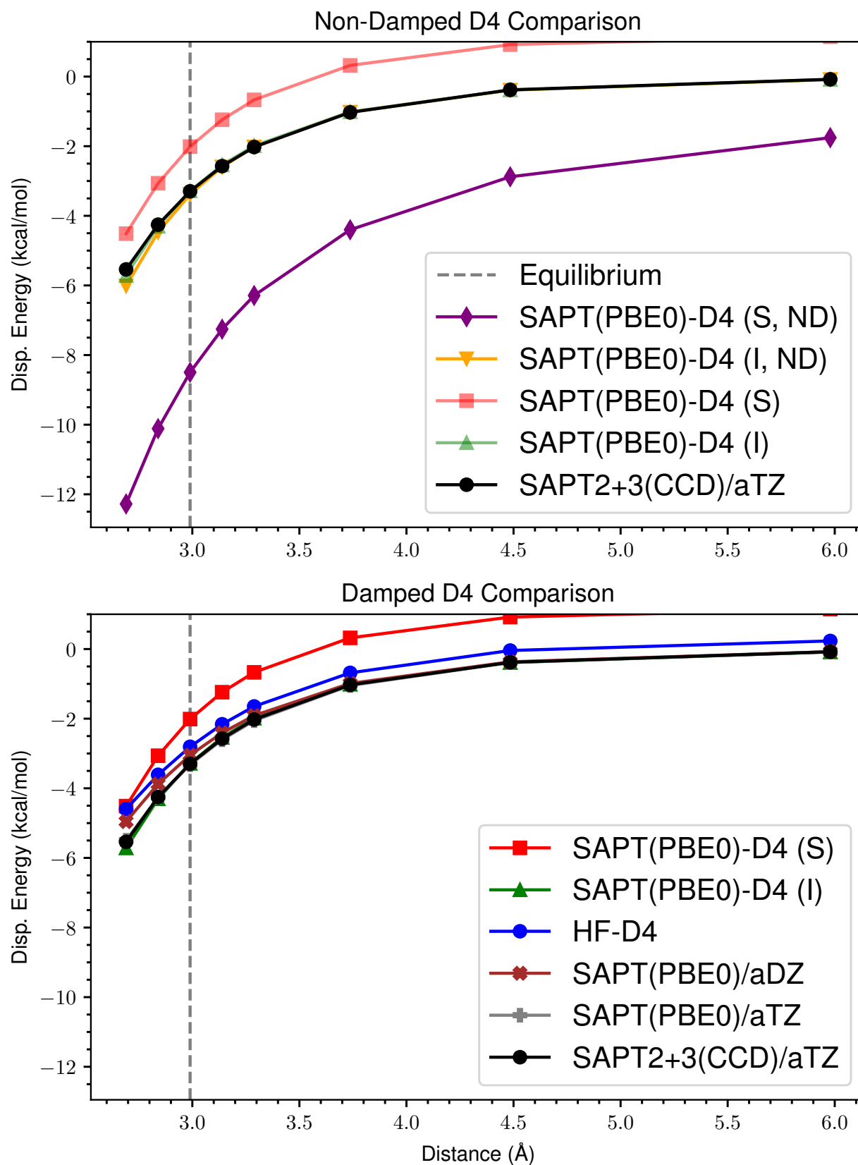
Figure 2: ND vs Damped D4 Dispersion for s66x8 45 Ethyne-Pentane
