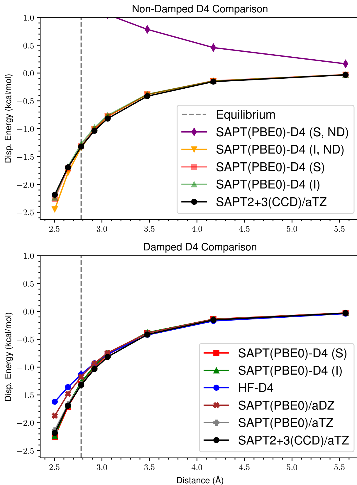
Figure 35: ND vs Damped D4 Dispersion for s66x8 51_Ethyne-Ethyne
