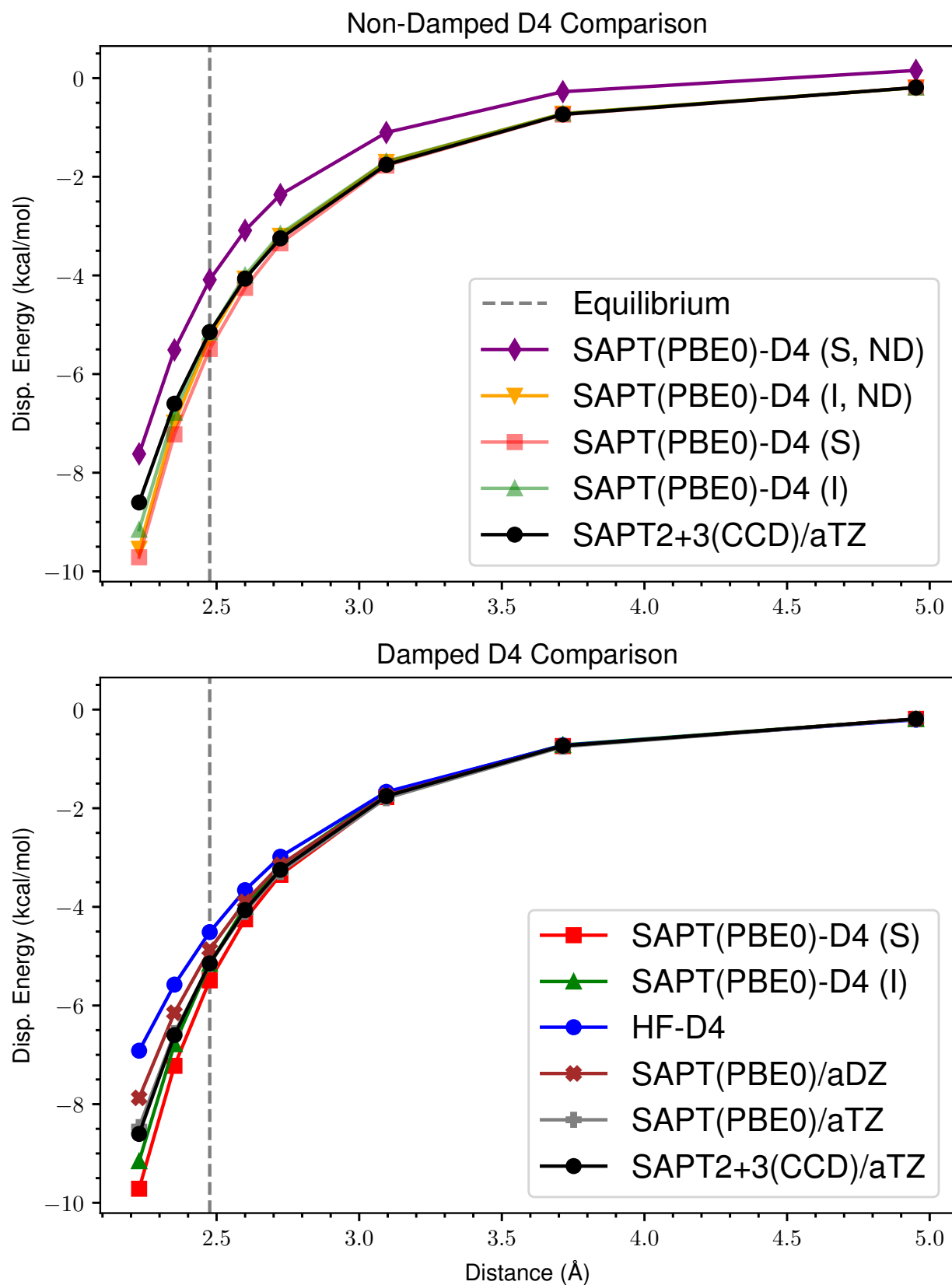
Figure 47: ND vs Damped D4 Dispersion for s66x8 35_Neopentane-Pentane
