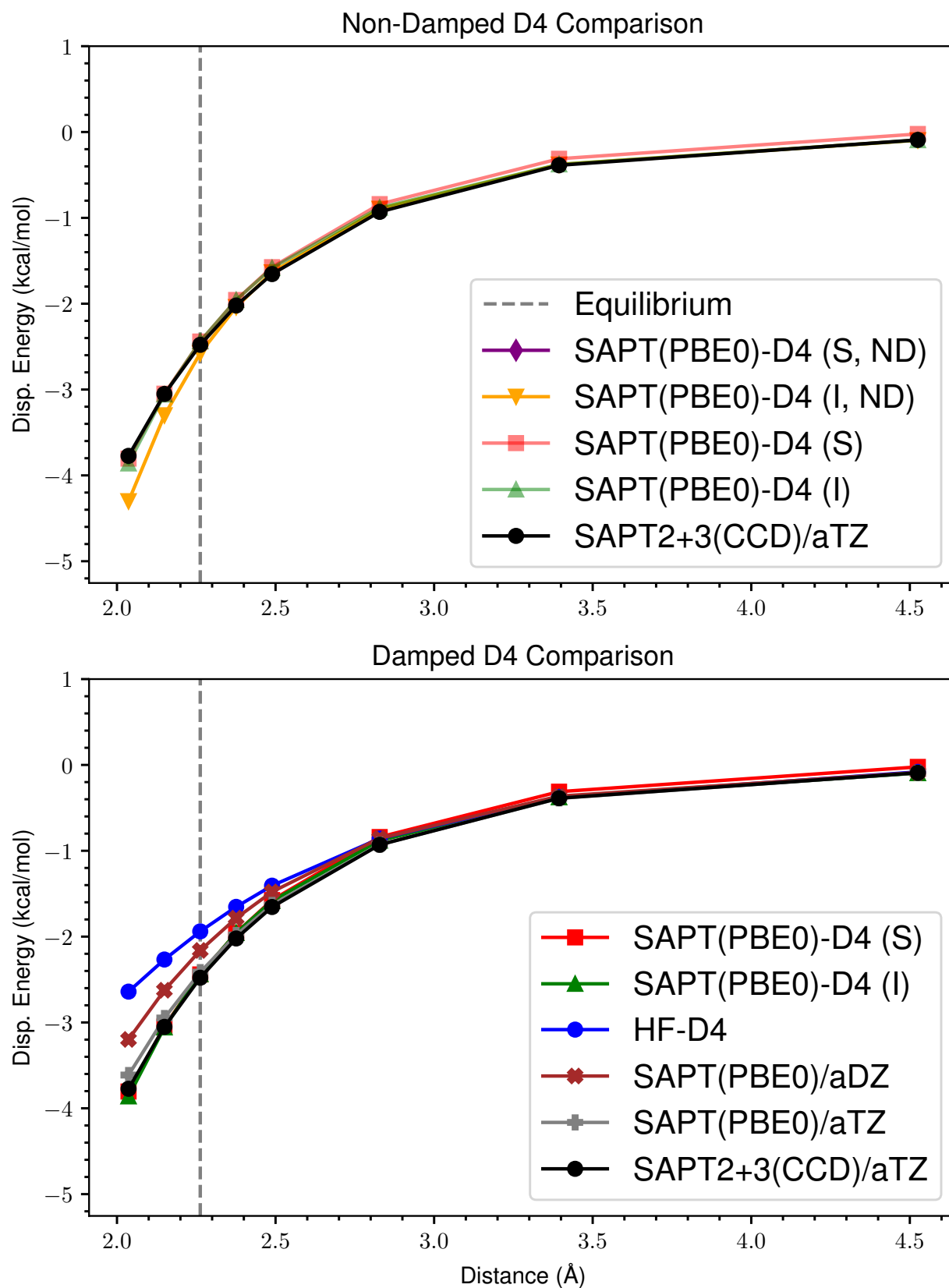
Figure 42: ND vs Damped D4 Dispersion for s66x8 09_MeNH2-MeOH
