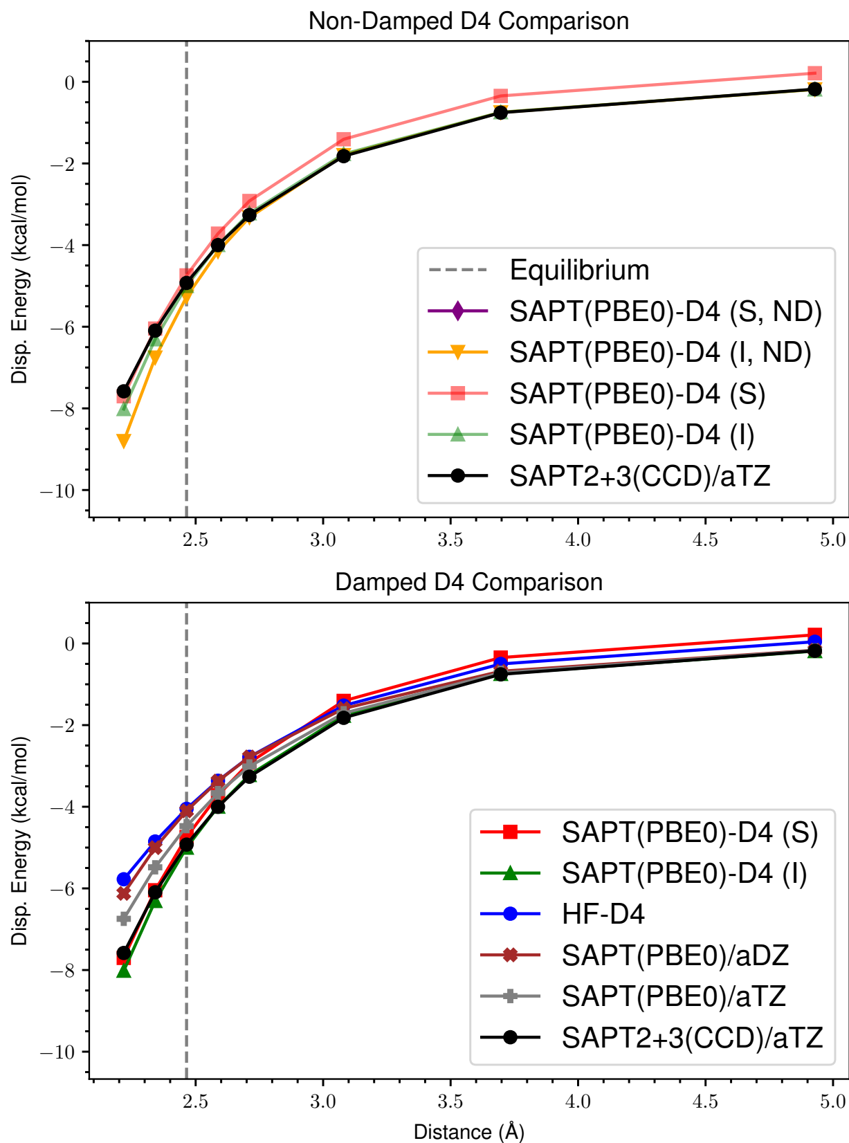
Figure 9: ND vs Damped D4 Dispersion for s66x8 52_Benzene-AcOH
