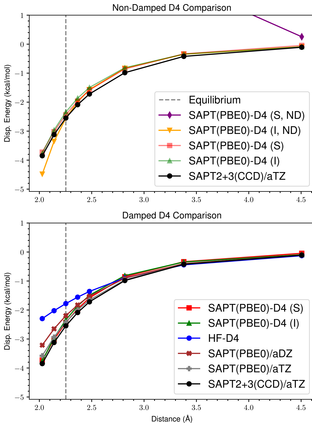
Figure 16: ND vs Damped D4 Dispersion for s66x8 65_Pyridine-Ethyne
