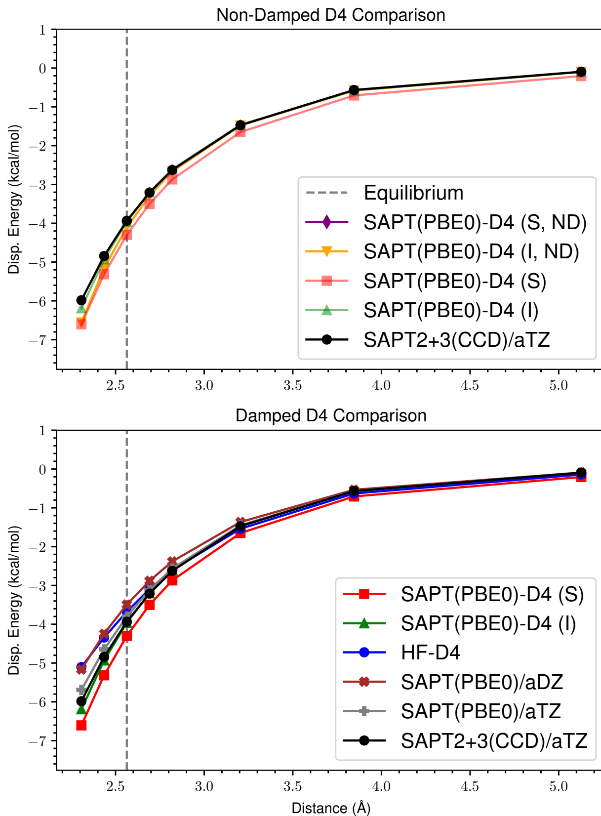
Figure 31: ND vs Damped D4 Dispersion for s66x8 64_Peptide-Ethene
