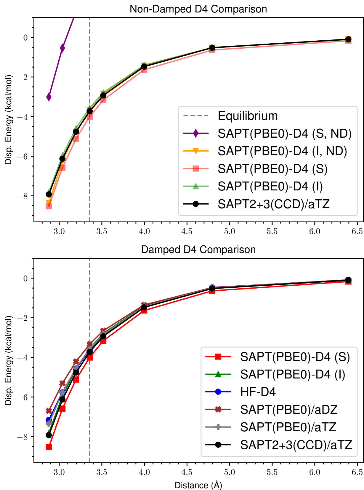
Figure 14: ND vs Damped D4 Dispersion for s66x8 33_Pyridine-Ethene
