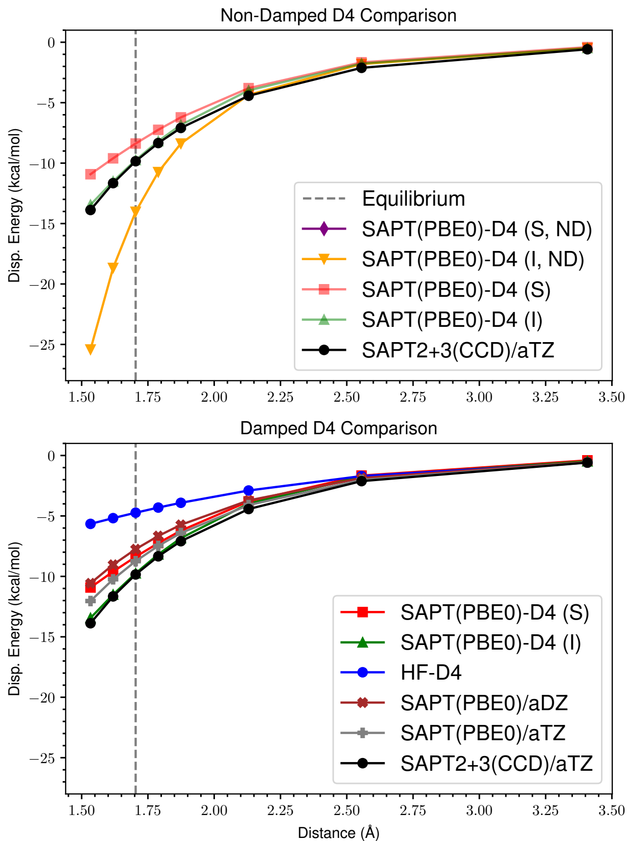
Figure 15: ND vs Damped D4 Dispersion for s66x8 22_AcOH-Uracil
