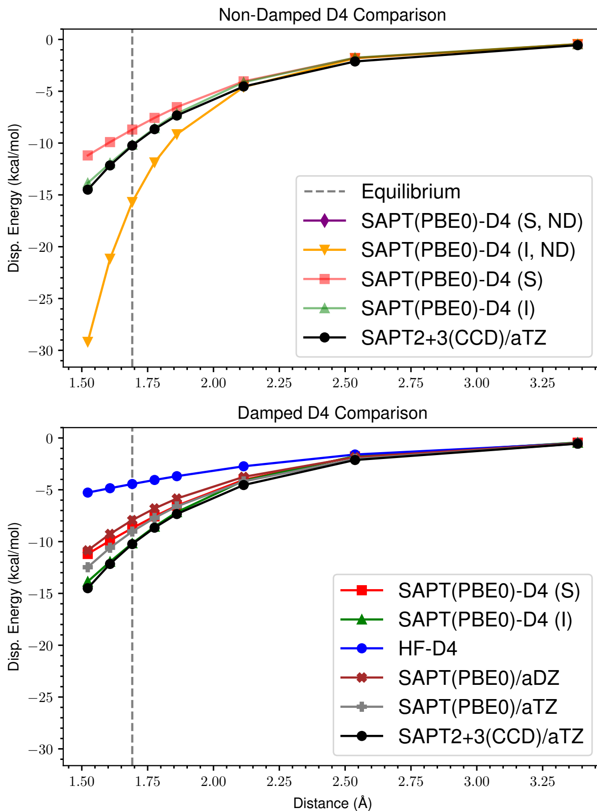
Figure 34: ND vs Damped D4 Dispersion for s66x8 20_AcOH-AcOH
