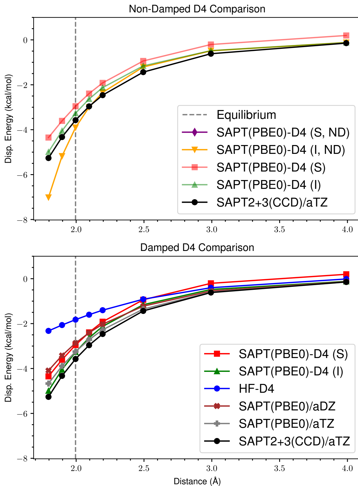
Figure 49: ND vs Damped D4 Dispersion for s66x8 18_Water-Pyridine
