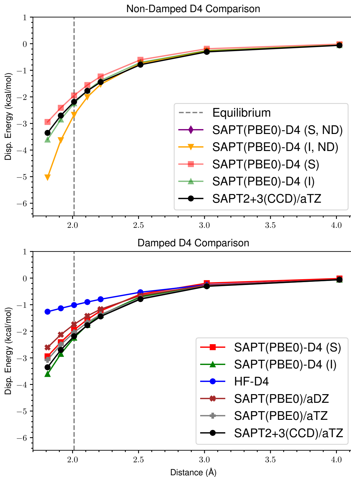
Figure 22: ND vs Damped D4 Dispersion for s66x8 01_Water-Water
