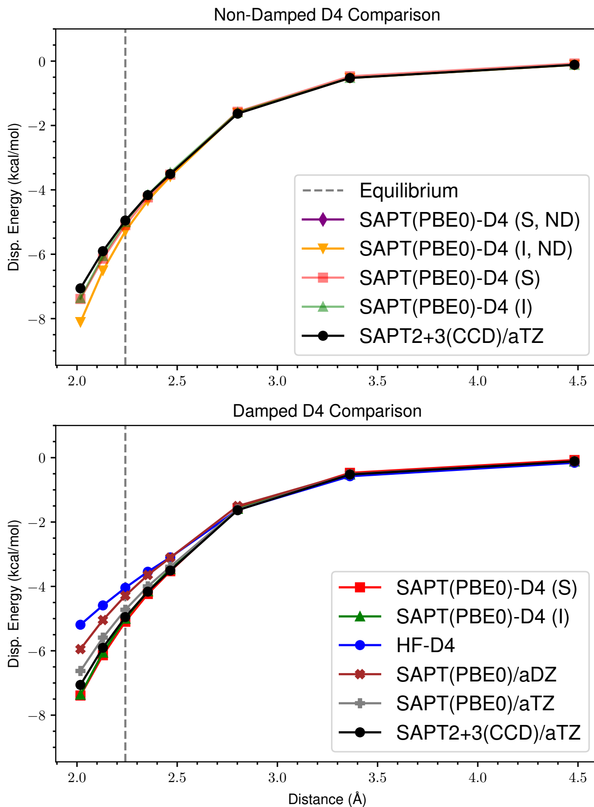
Figure 52: ND vs Damped D4 Dispersion for s66x8 11_MeNH2-Peptide
