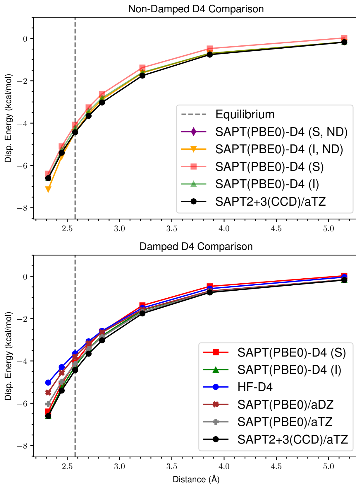
Figure 36: ND vs Damped D4 Dispersion for s66x8 53_Benzene-AcNH2
