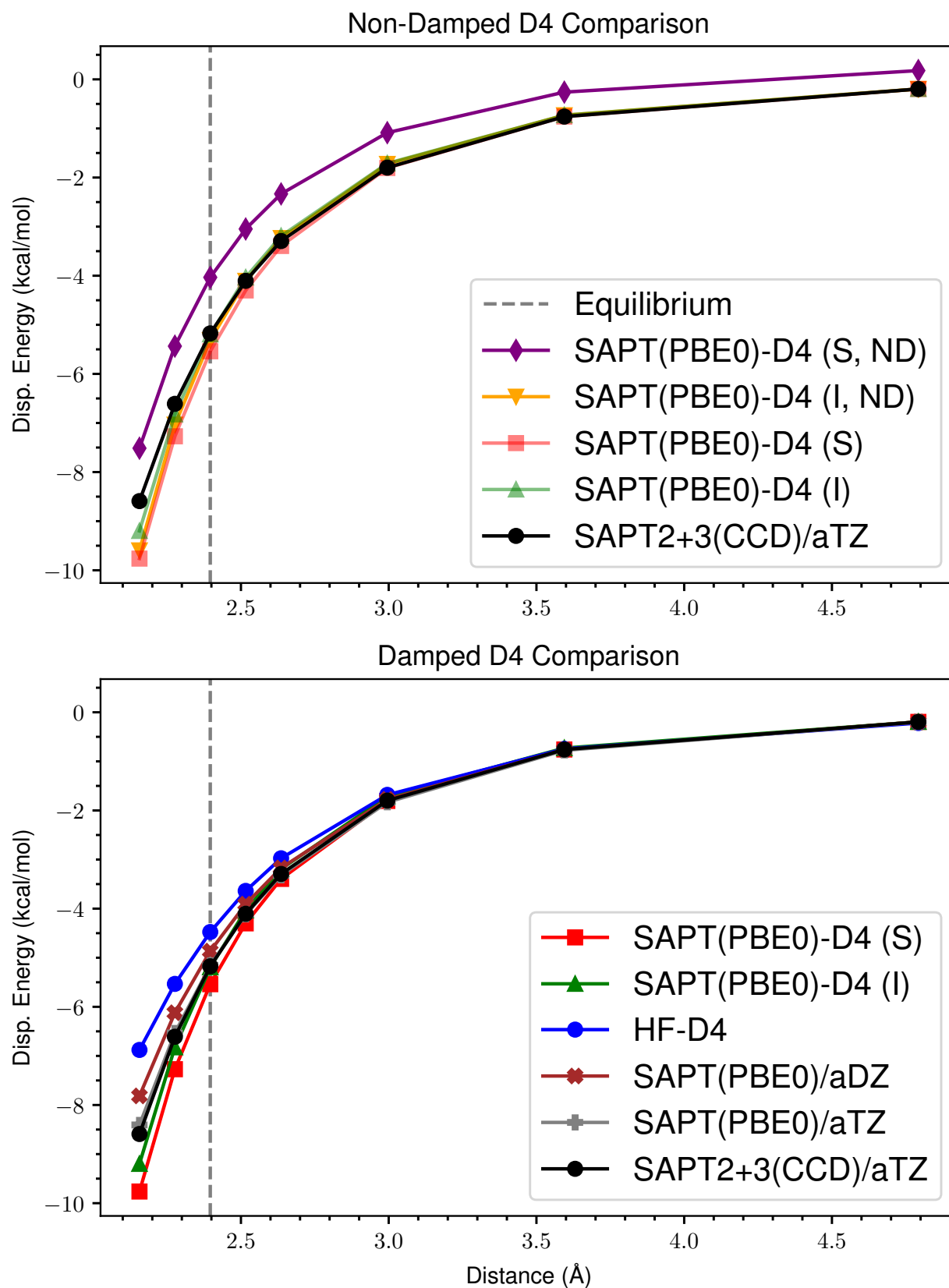
Figure 63: ND vs Damped D4 Dispersion for s66x8 37_Cyclopentane-Neopentane
