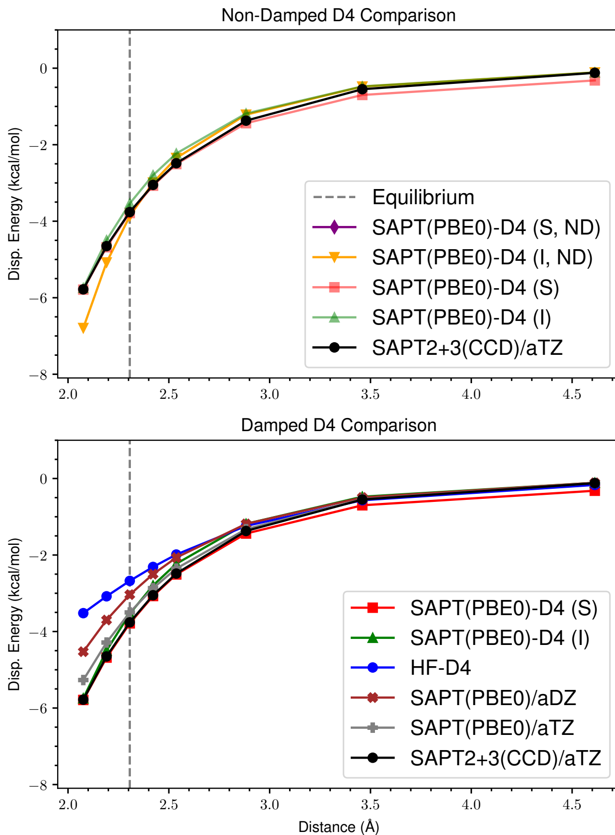
Figure 58: ND vs Damped D4 Dispersion for s66x8 60_Ethyne-AcOH
