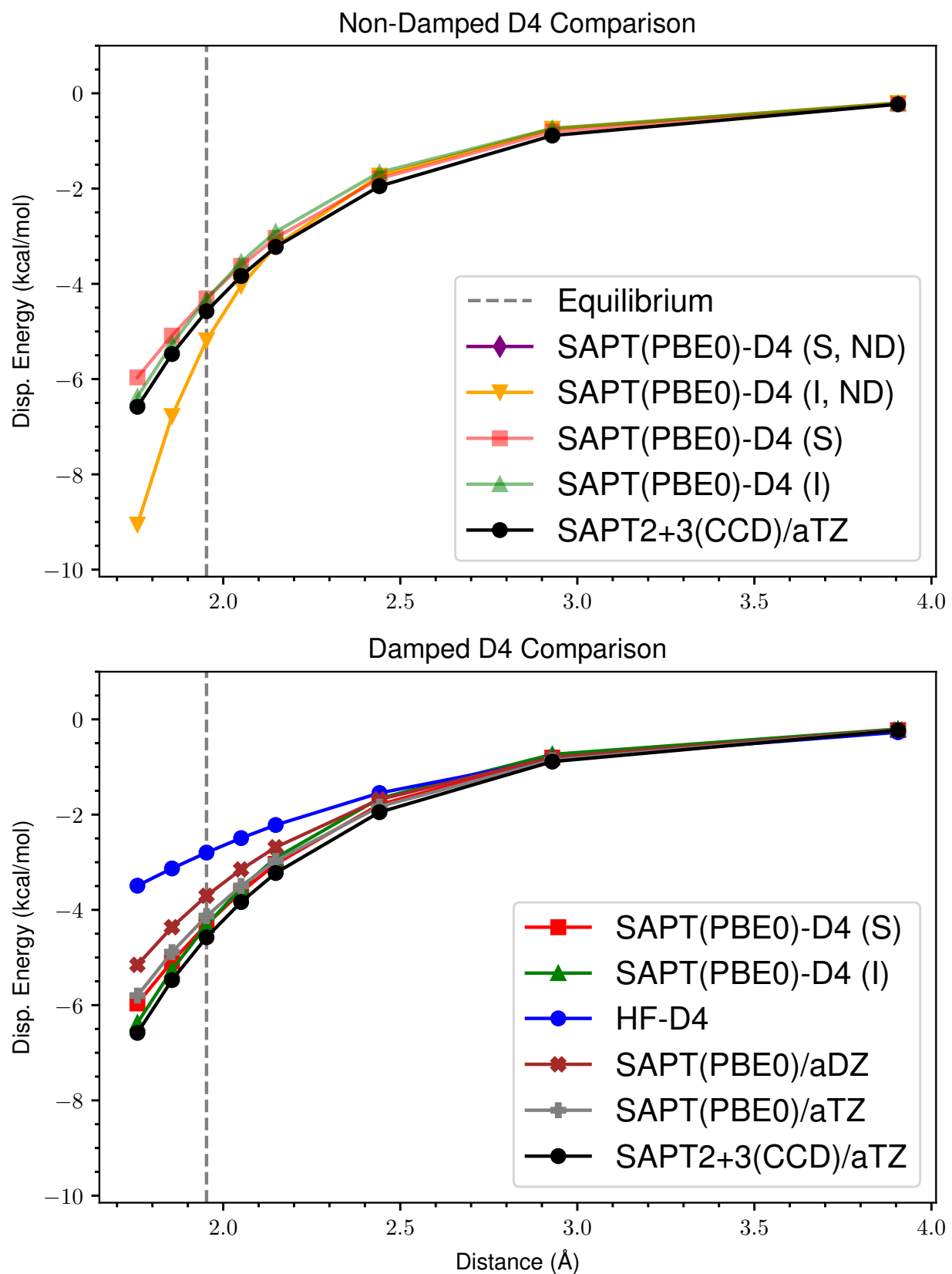
Figure 66: ND vs Damped D4 Dispersion for s66x8 19_MeOH-Pyridine
