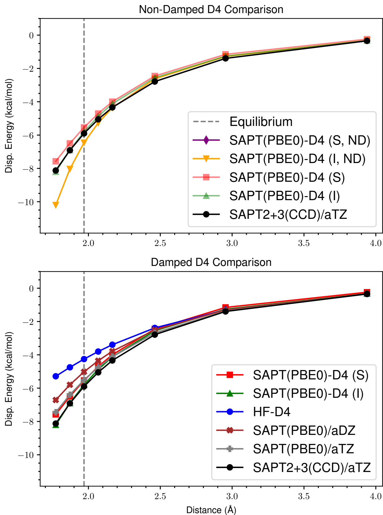
Figure 27: ND vs Damped D4 Dispersion for s66x8 15_Peptide-Peptide
