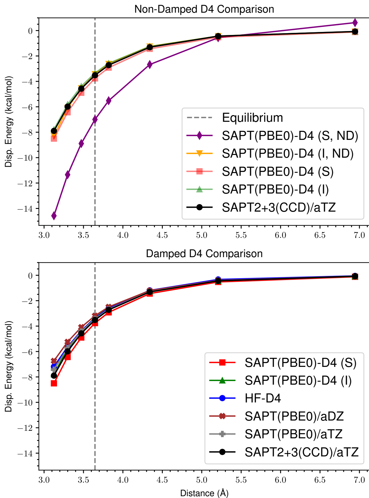
Figure 43: ND vs Damped D4 Dispersion for s66x8 30_Benzene-Ethene
