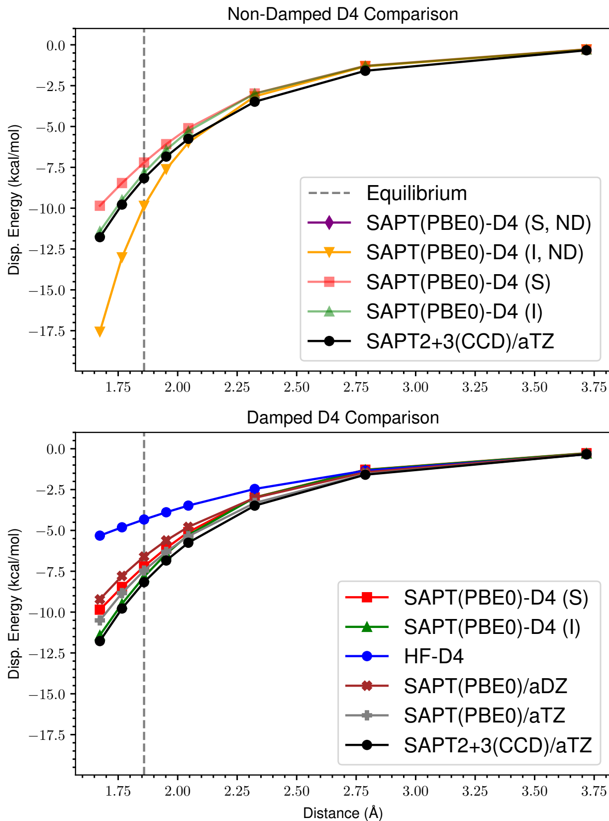
Figure 50: ND vs Damped D4 Dispersion for s66x8 21_AcNH2-AcNH2
