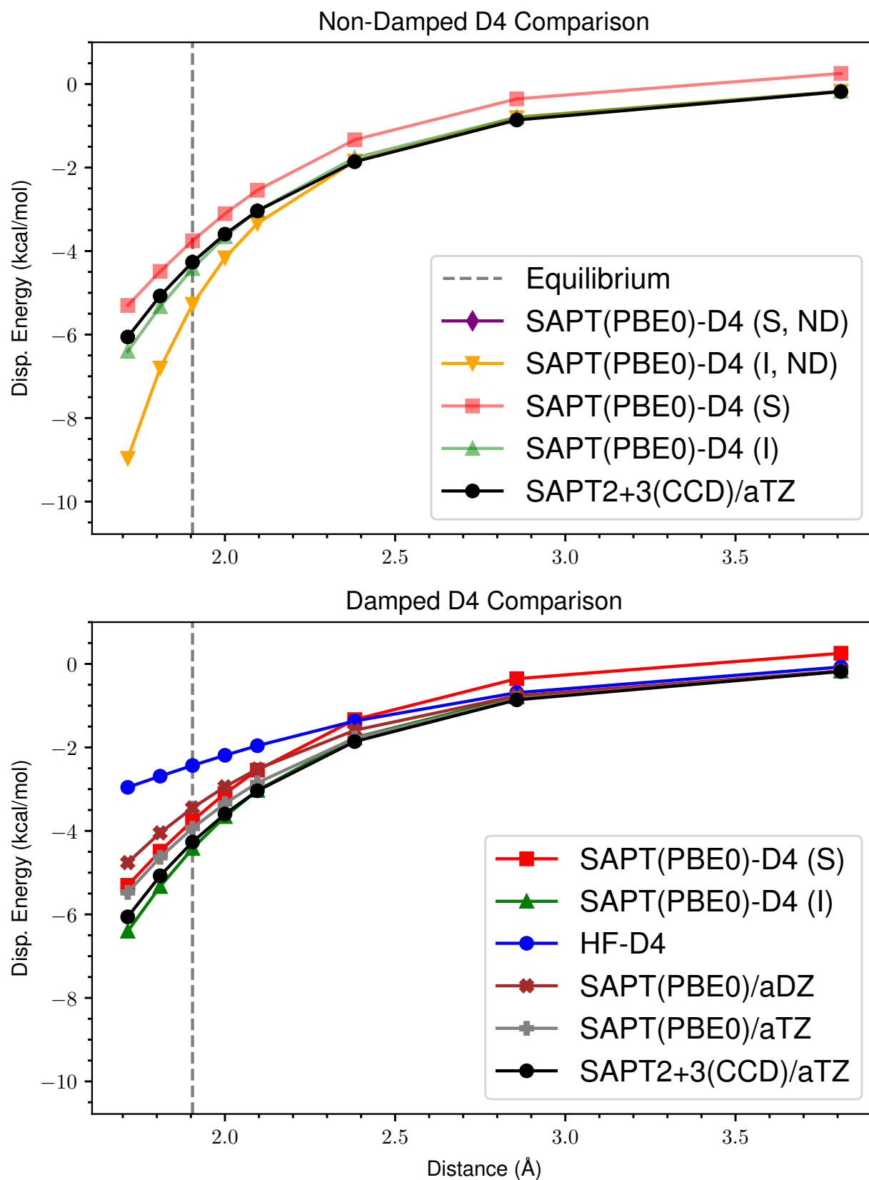
Figure 25: ND vs Damped D4 Dispersion for s66x8 04_Water-Peptide
