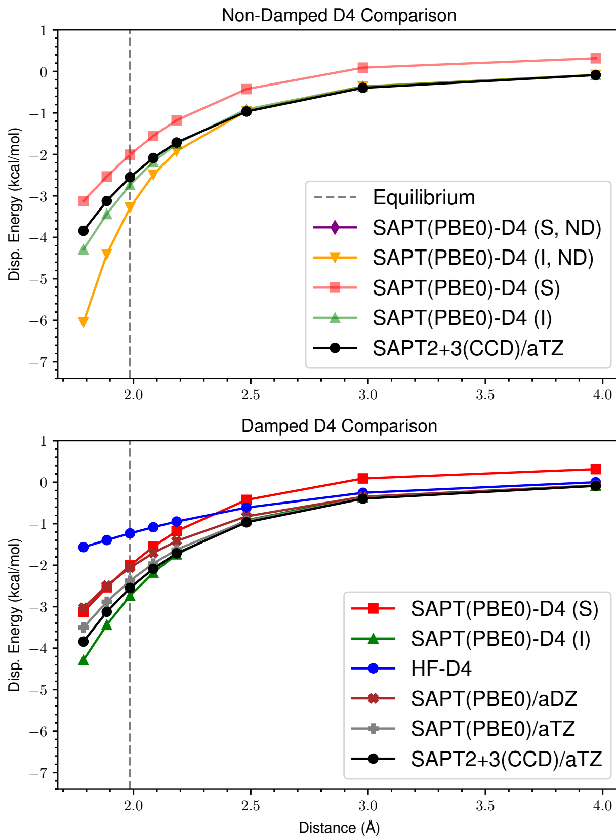
Figure 55: ND vs Damped D4 Dispersion for s66x8 08_MeOH-Water
