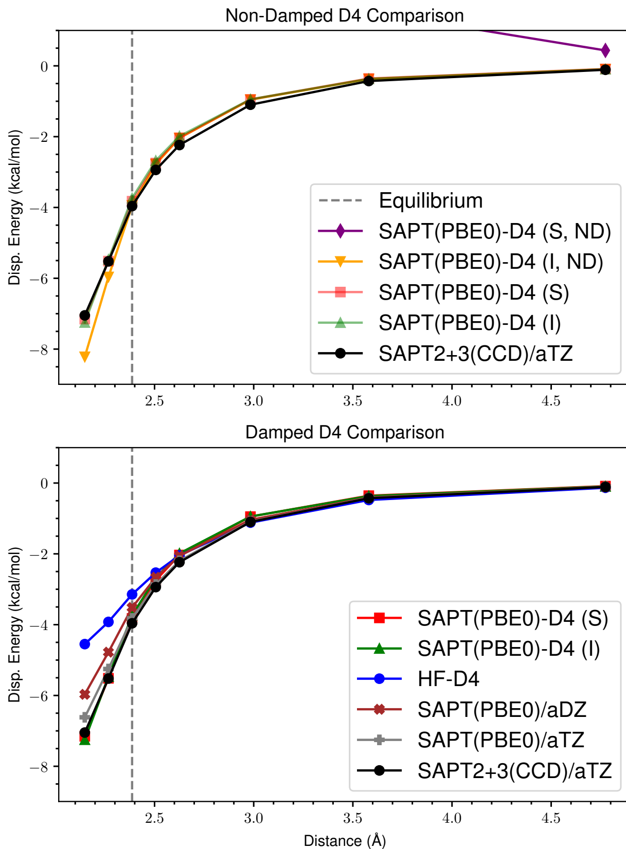
Figure 20: ND vs Damped D4 Dispersion for s66x8 58_Pyridine-Pyridine
