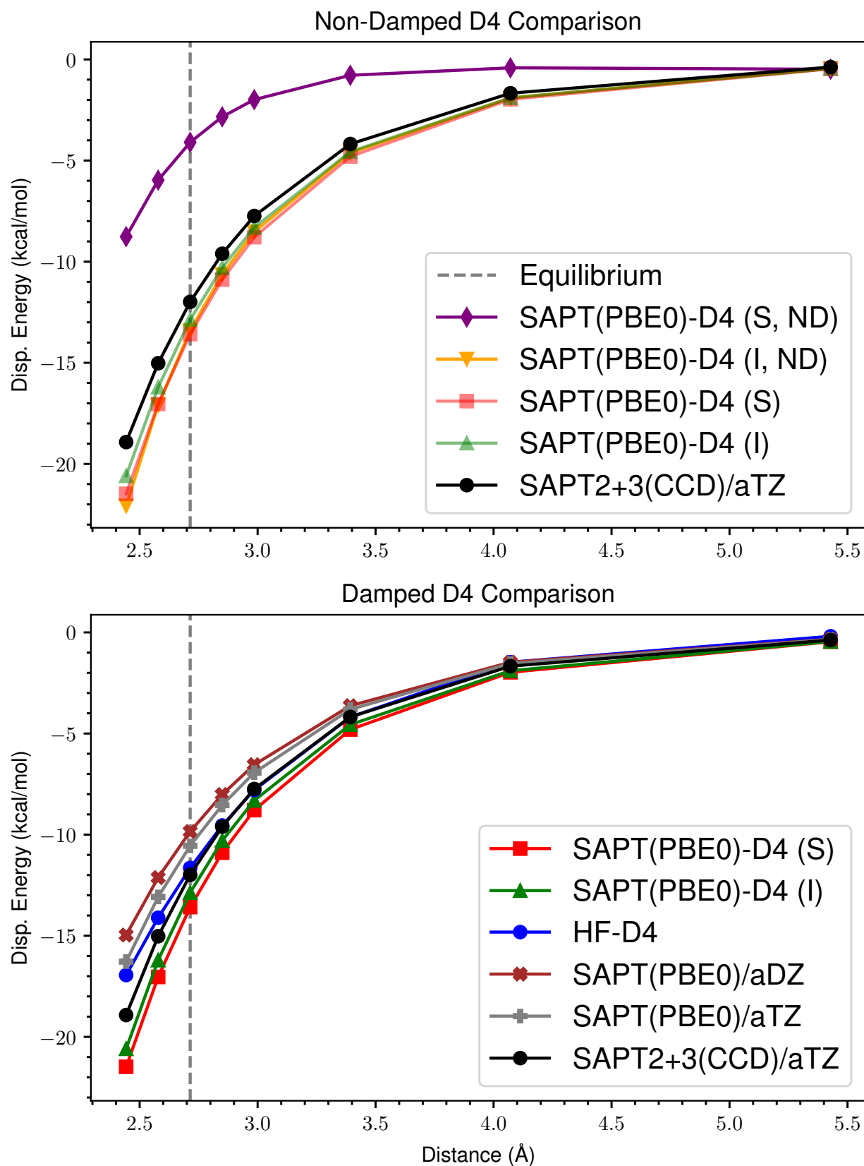
Figure 10: ND vs Damped D4 Dispersion for s66x8 26_Uracil-Uracil
