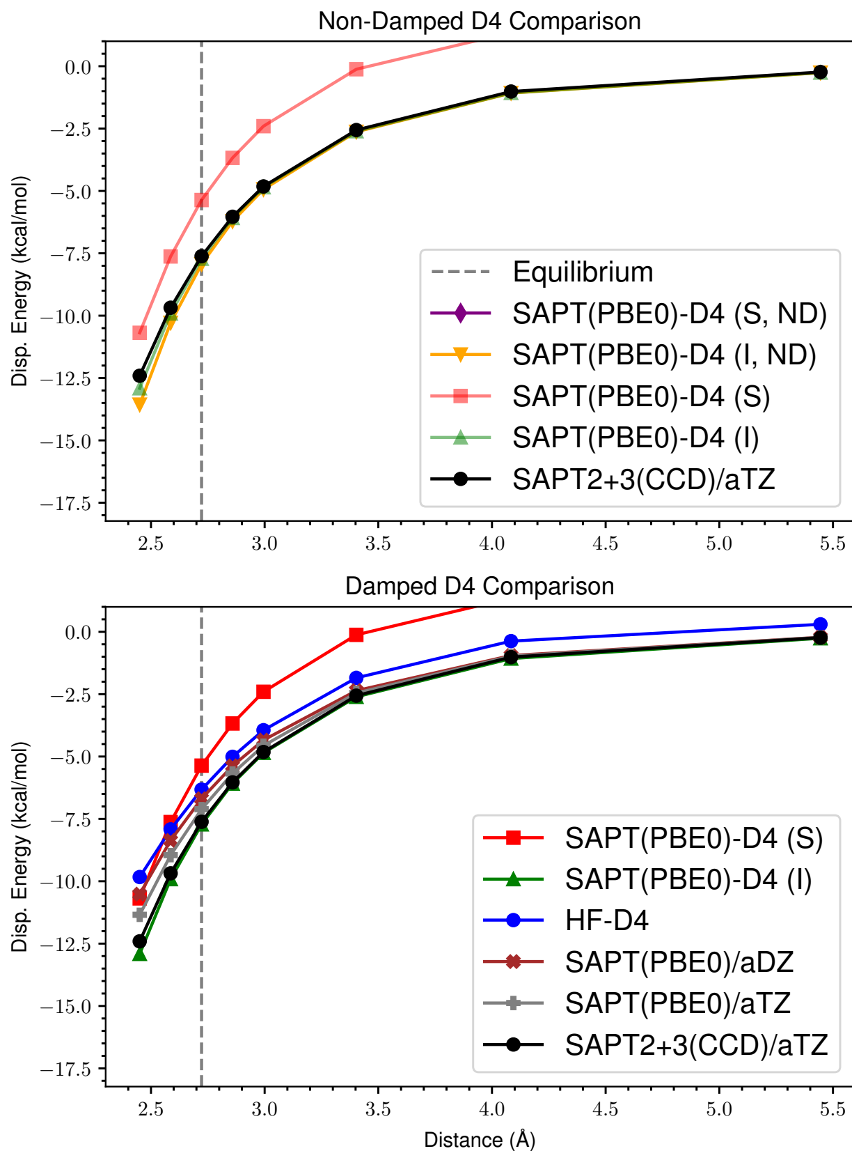
Figure 29: ND vs Damped D4 Dispersion for s66x8 42_Uracil-Cyclopentane
