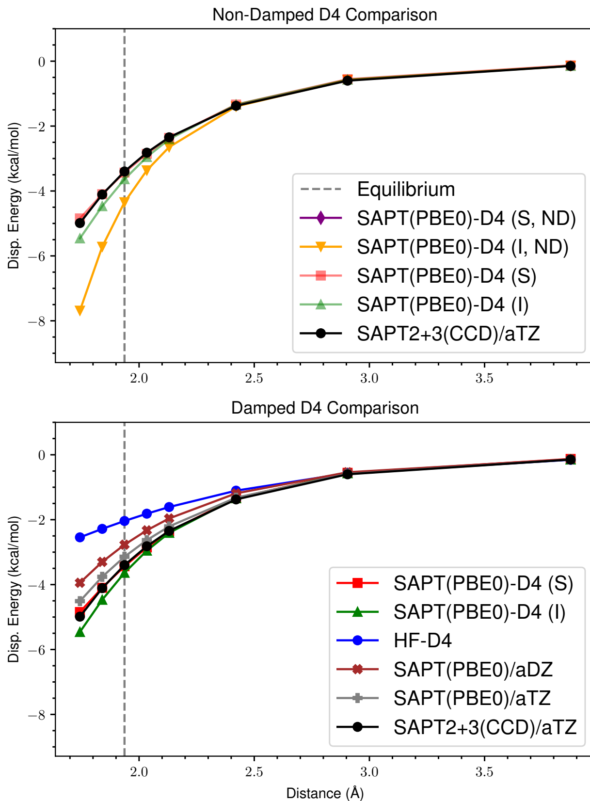
Figure 33: ND vs Damped D4 Dispersion for s66x8 05_MeOH-MeOH
