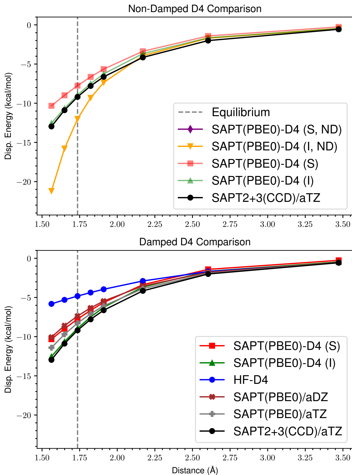
Figure 26: ND vs Damped D4 Dispersion for s66x8 23_AcNH2-Uracil
