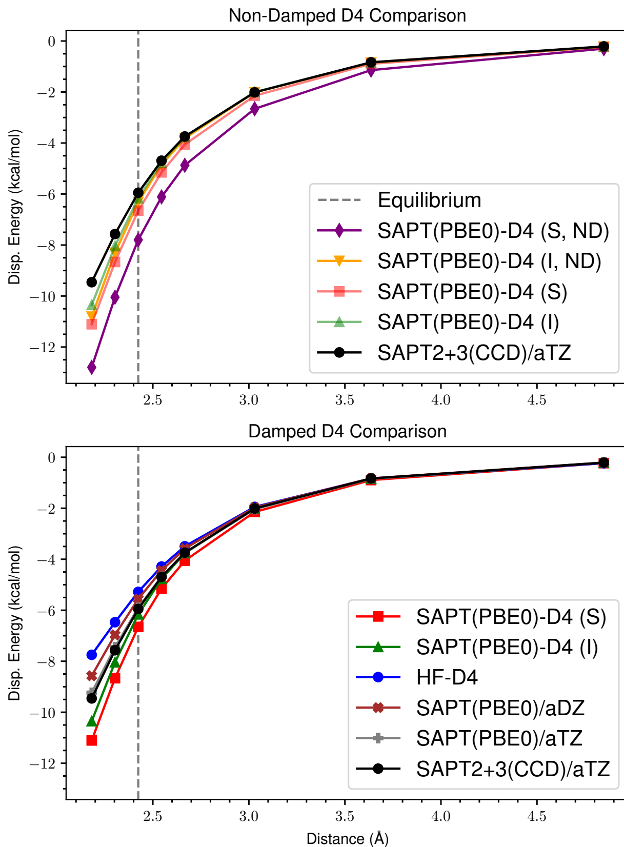
Figure 57: ND vs Damped D4 Dispersion for s66x8 38_Cyclopentane-Cyclopentane
