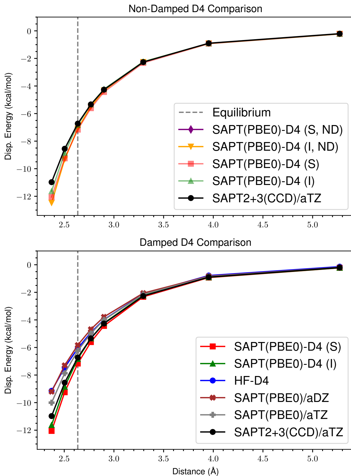
Figure 24: ND vs Damped D4 Dispersion for s66x8 57 Benzene-Peptide
