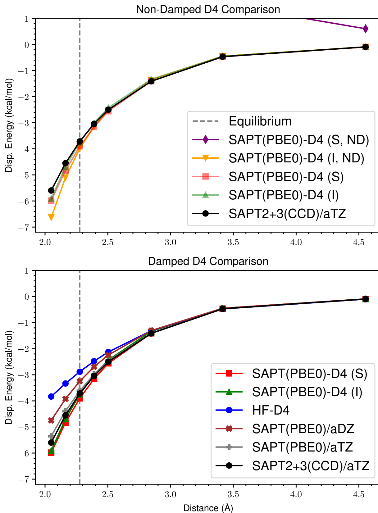
Figure 5: ND vs Damped D4 Dispersion for s66x8 10_MeNH2-MeNH2
