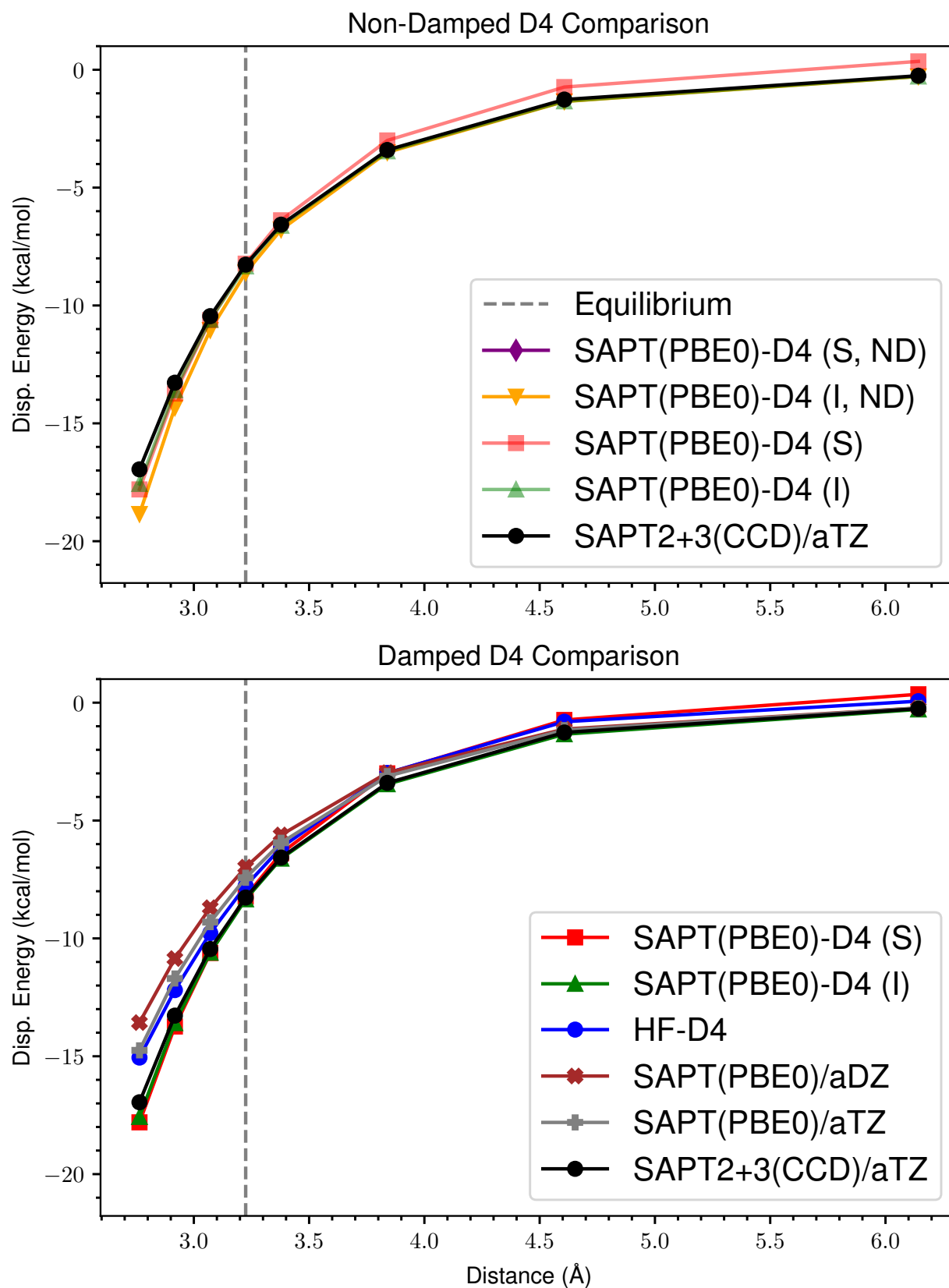
Figure 4: ND vs Damped D4 Dispersion for s66x8 28_Benzene-Uracil
