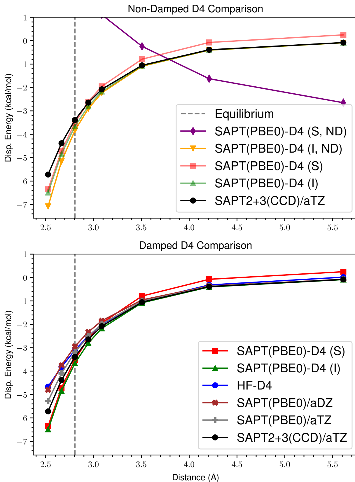
Figure 21: ND vs Damped D4 Dispersion for s66x8 50_Benzene-Ethyne
