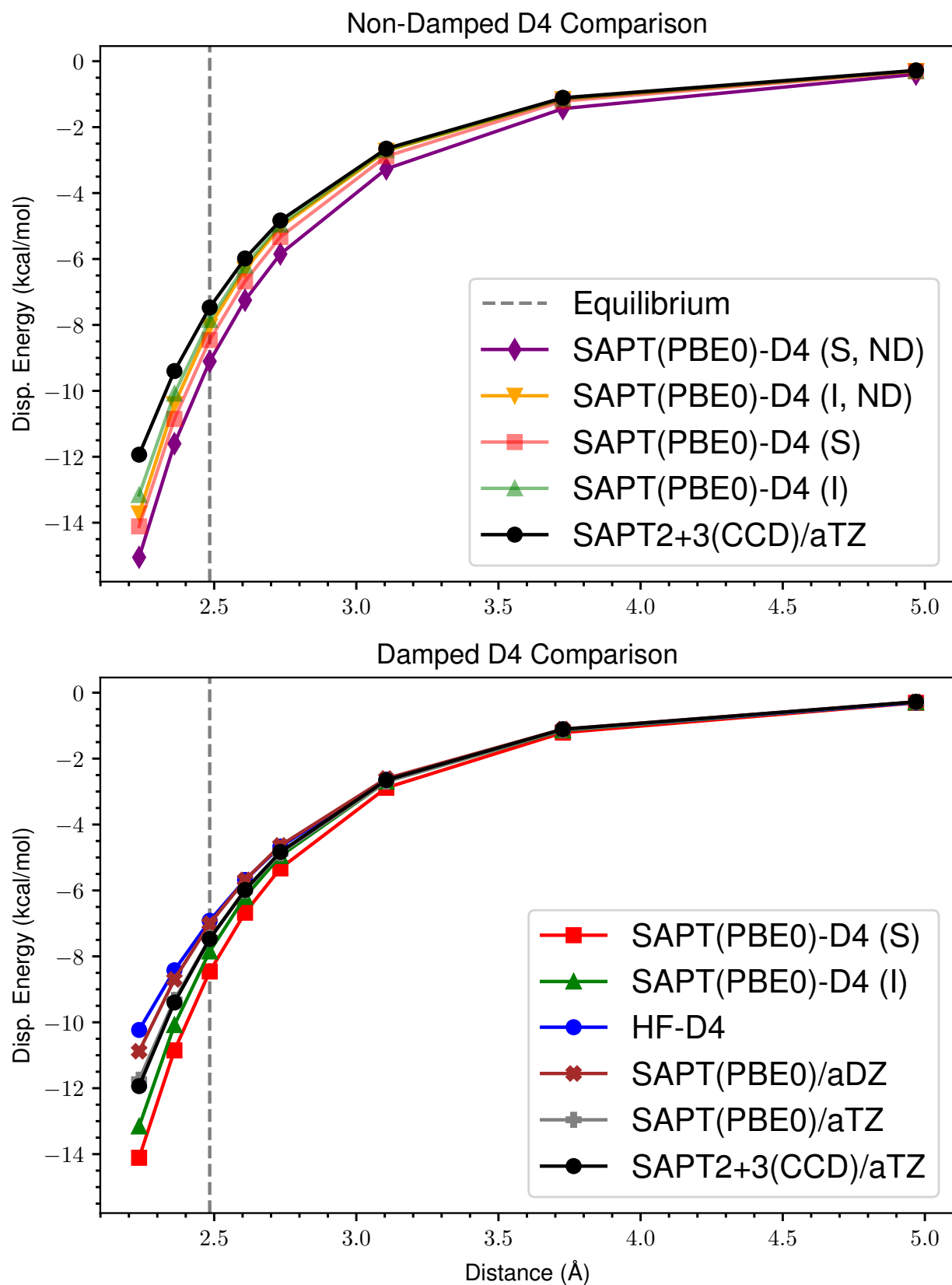
Figure 40: ND vs Damped D4 Dispersion for s66x8 34 Pentane-Pentane
