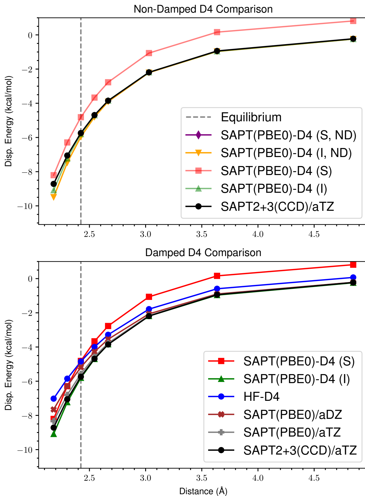
Figure 51: ND vs Damped D4 Dispersion for s66x8 62_Pentane-AcNH2
