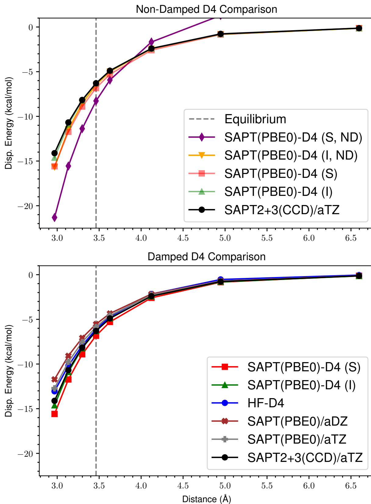
Figure 11: ND vs Damped D4 Dispersion for s66x8 27_Benzene-Pyridine
