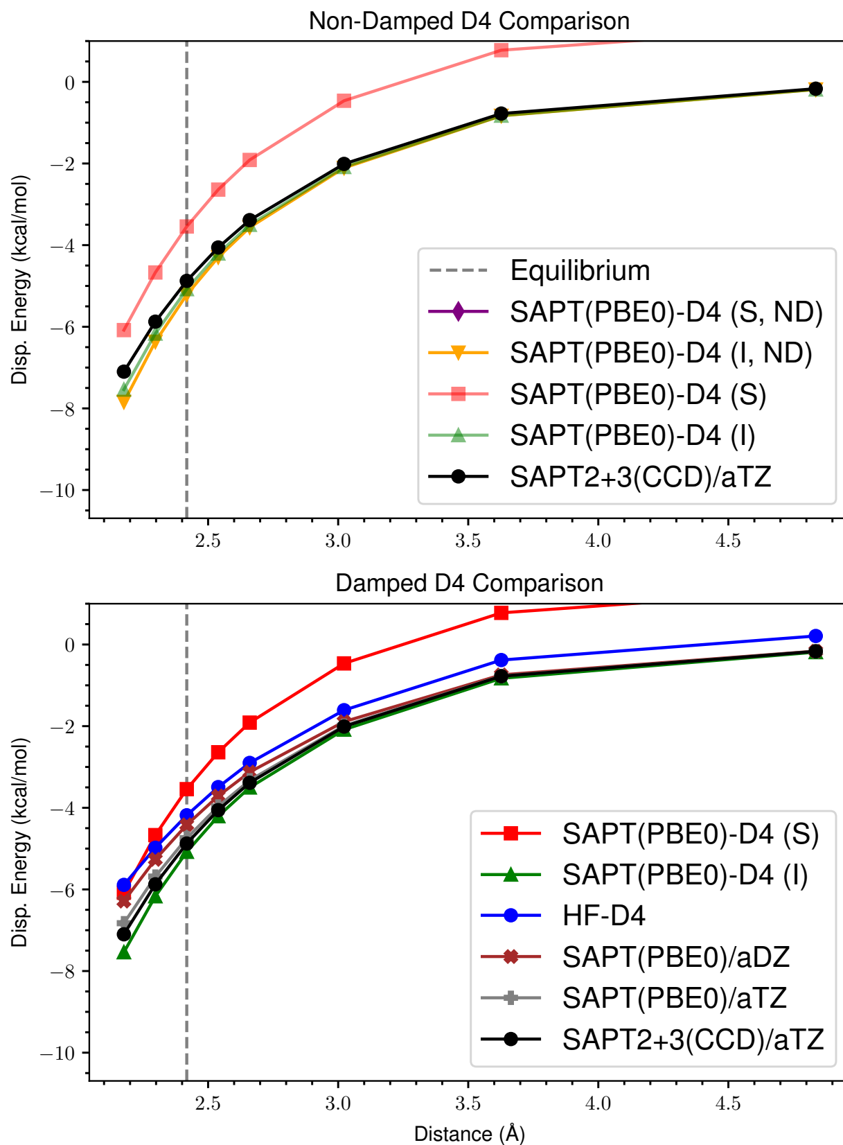
Figure 61: ND vs Damped D4 Dispersion for s66x8 61_Pentane-AcOH
