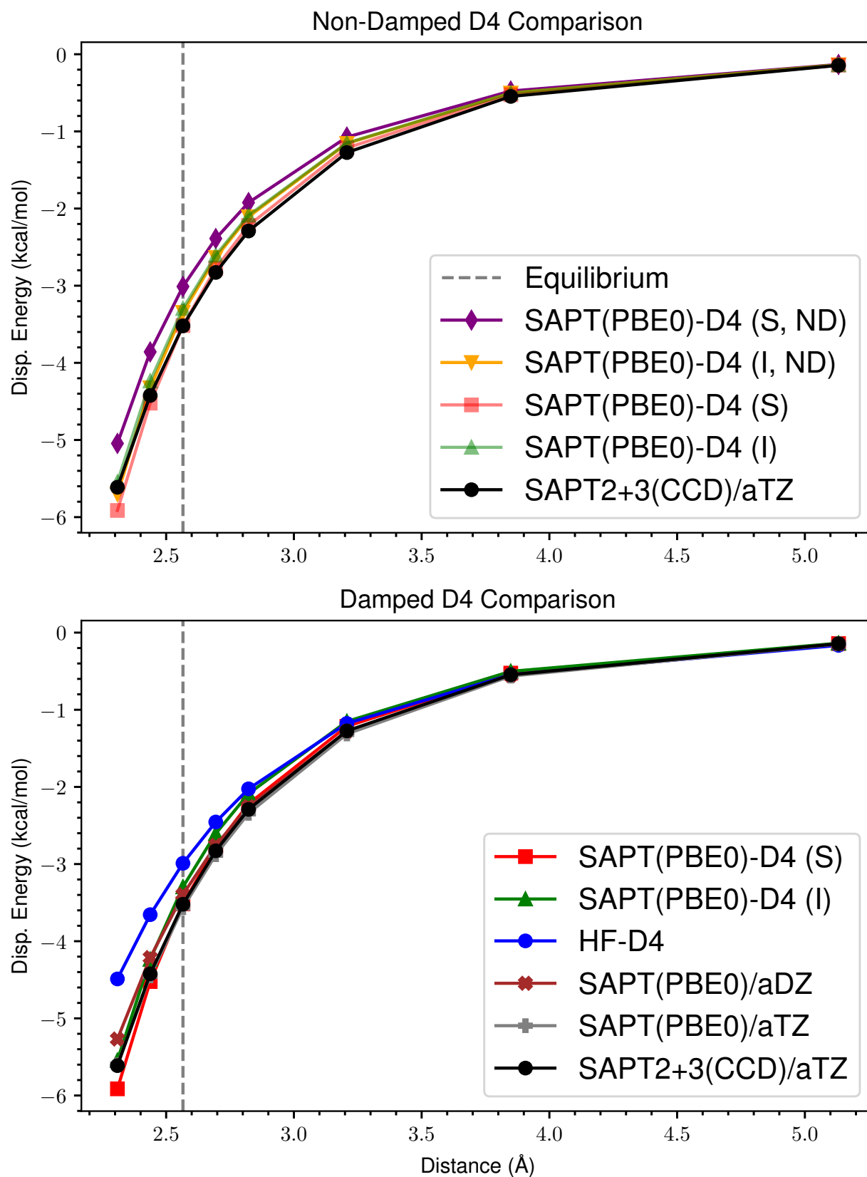
Figure 62: ND vs Damped D4 Dispersion for s66x8 36_Neopentane-Neopentane
