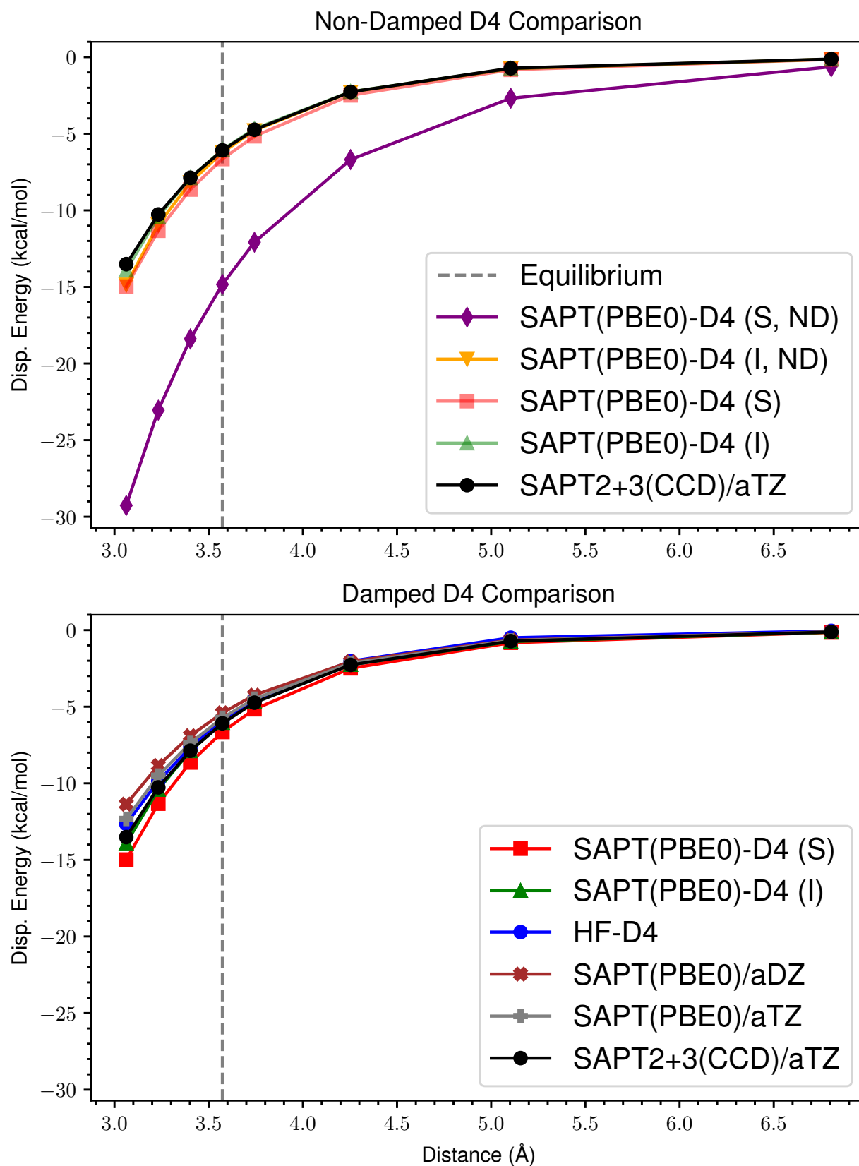
Figure 37: ND vs Damped D4 Dispersion for s66x8 24_Benzene-Benzene
