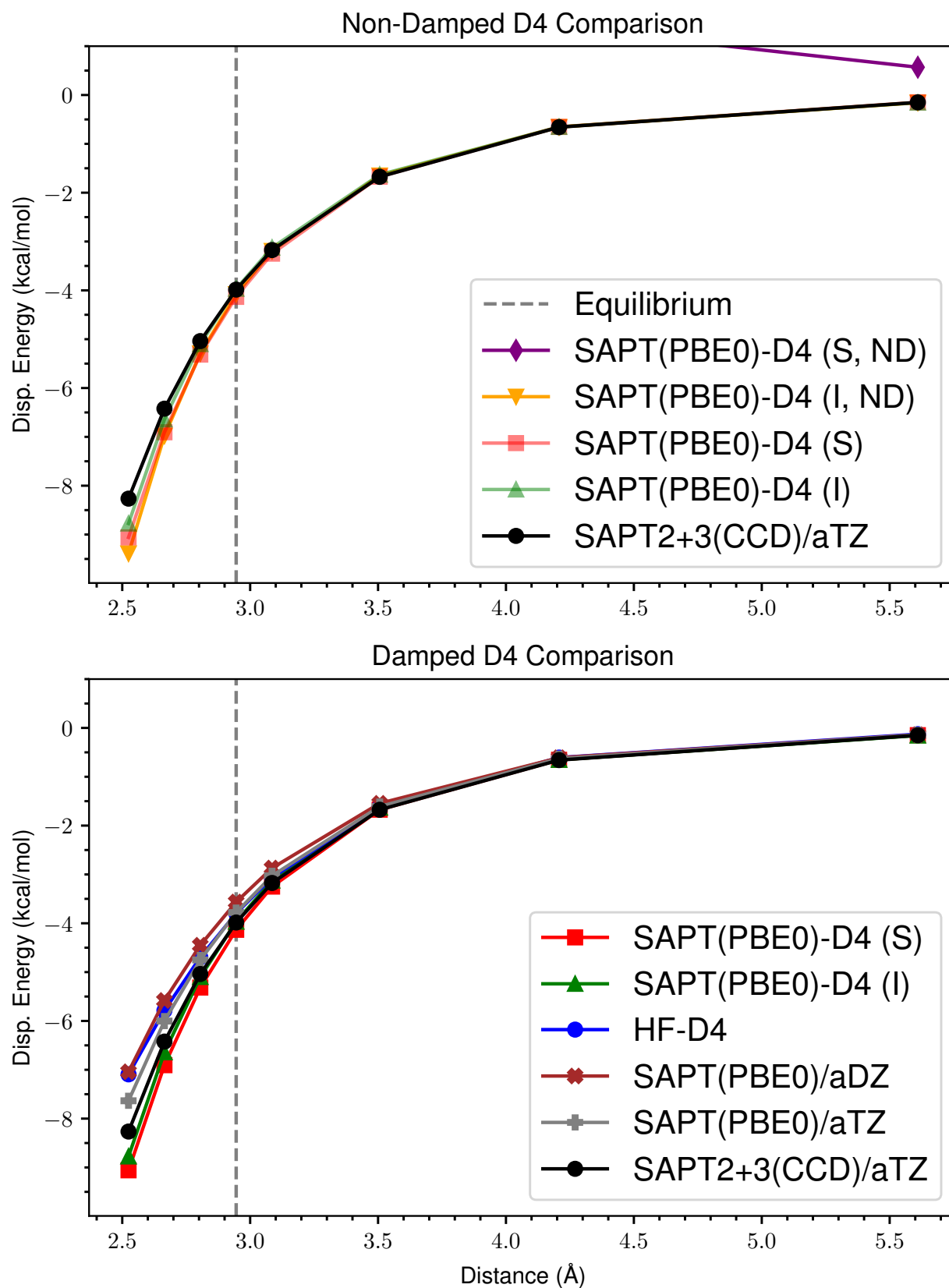
Figure 17: ND vs Damped D4 Dispersion for s66x8 47_Benzene-Benzene
