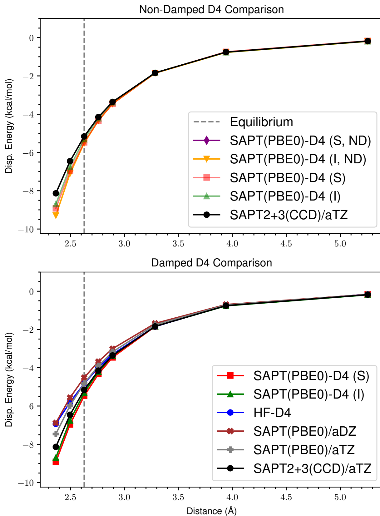
Figure 28: ND vs Damped D4 Dispersion for s66x8 48_Pyridine-Pyridine
