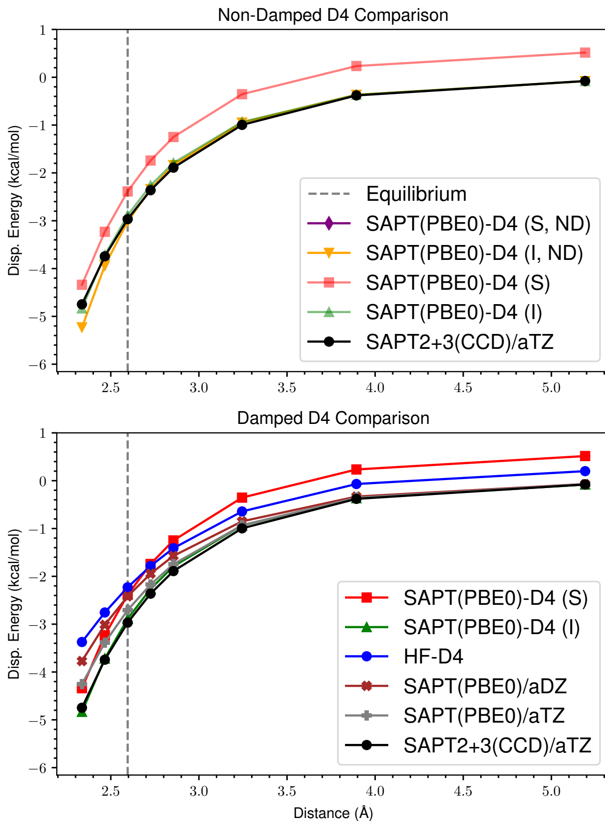
Figure 13: ND vs Damped D4 Dispersion for s66x8 54_Benzene-Water
