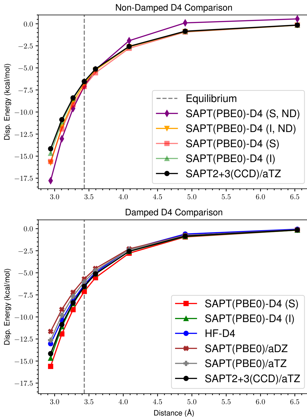
Figure 12: ND vs Damped D4 Dispersion for s66x8 25_Pyridine-Pyridine
