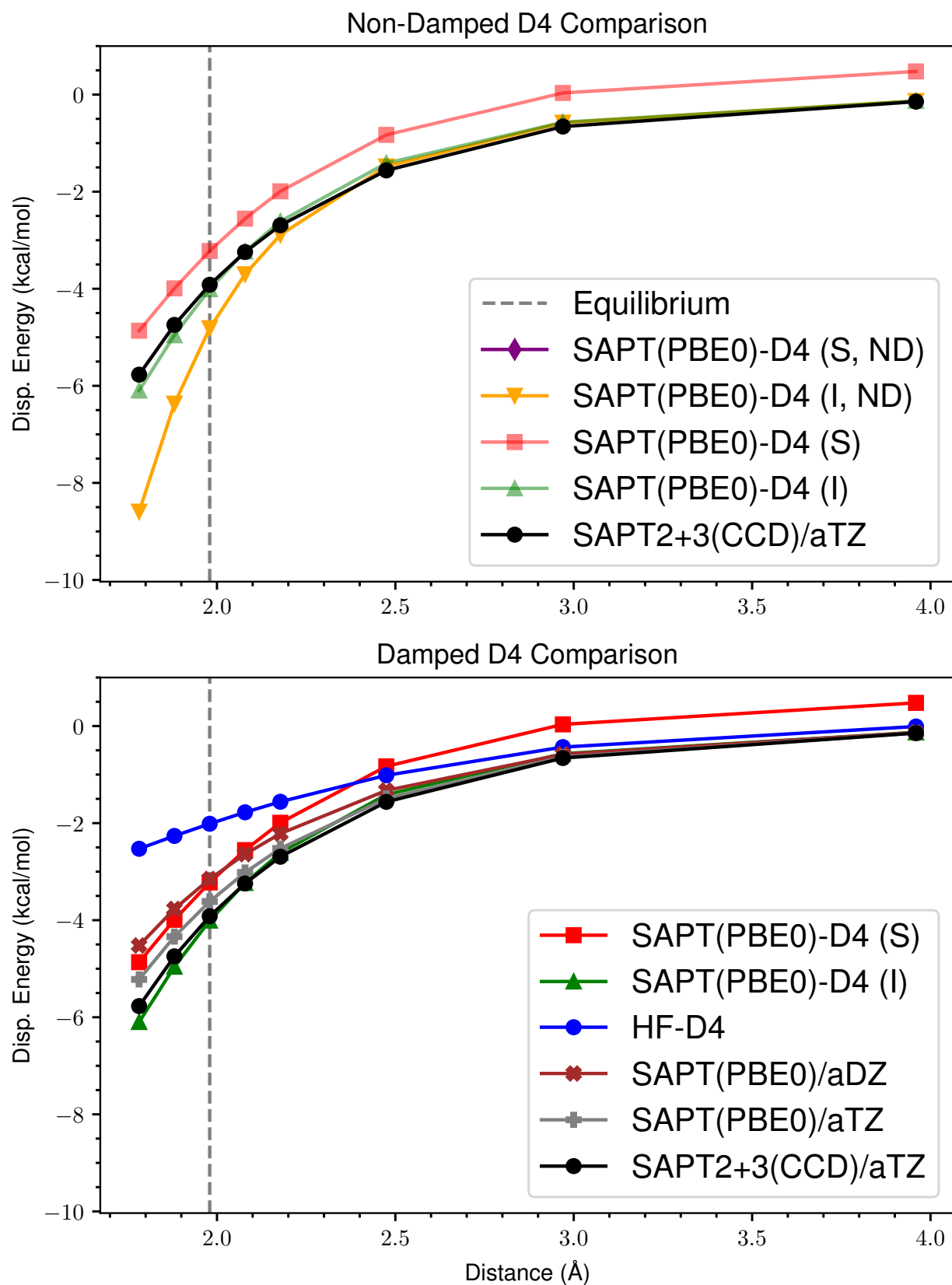
Figure 60: ND vs Damped D4 Dispersion for s66x8 12_MeNH2-Water
