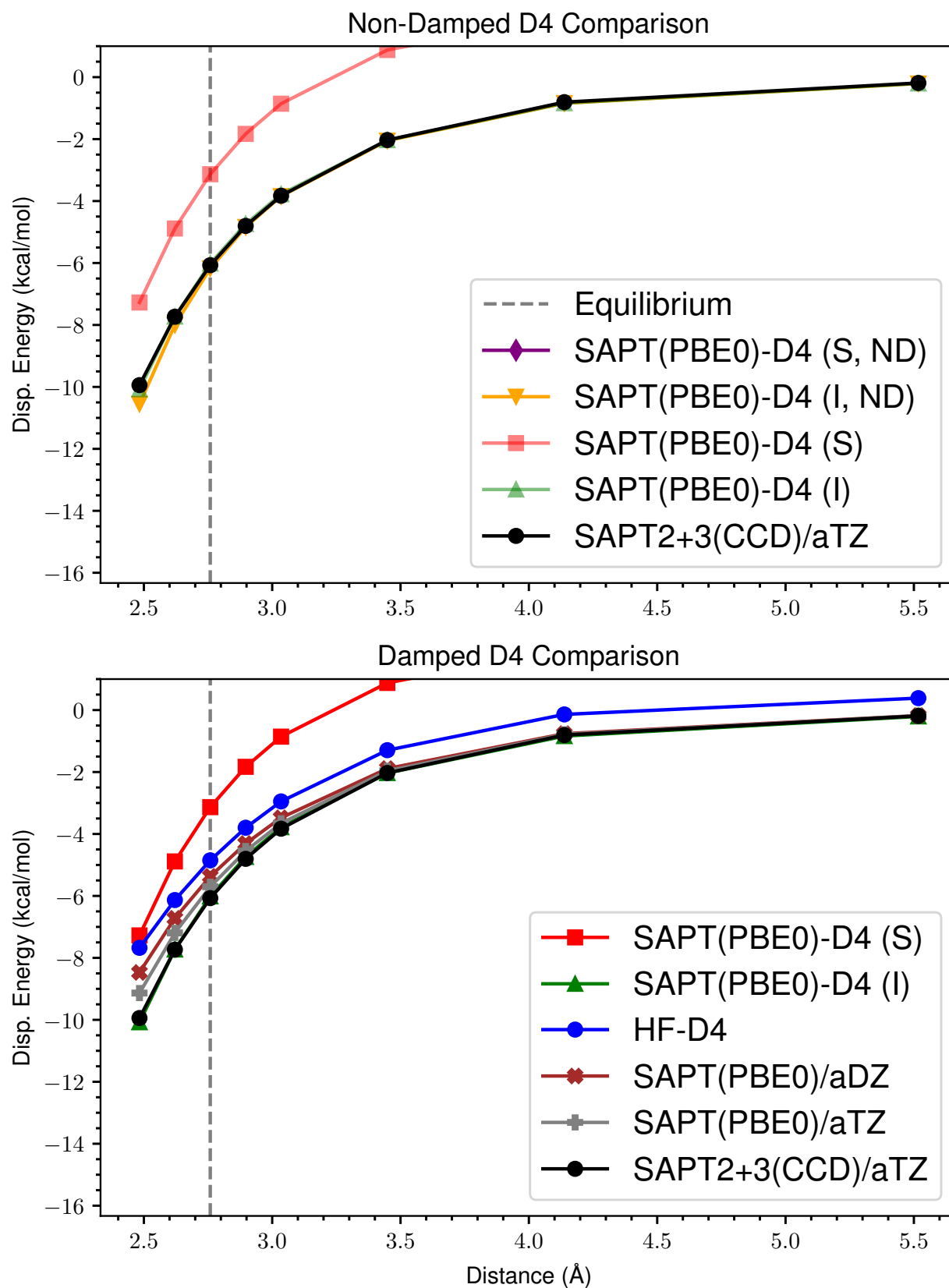
Figure 53: ND vs Damped D4 Dispersion for s66x8 43_Uracil-Neopentane
