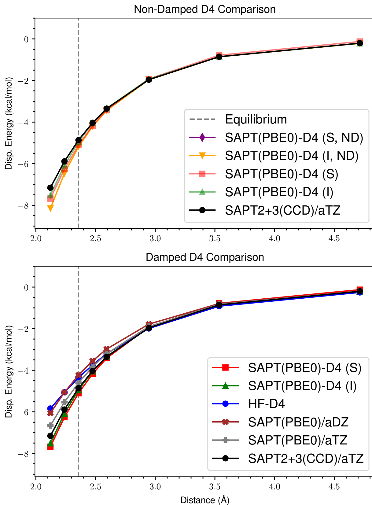
Figure 38: ND vs Damped D4 Dispersion for s66x8 66_MeNH2-Pyridine
