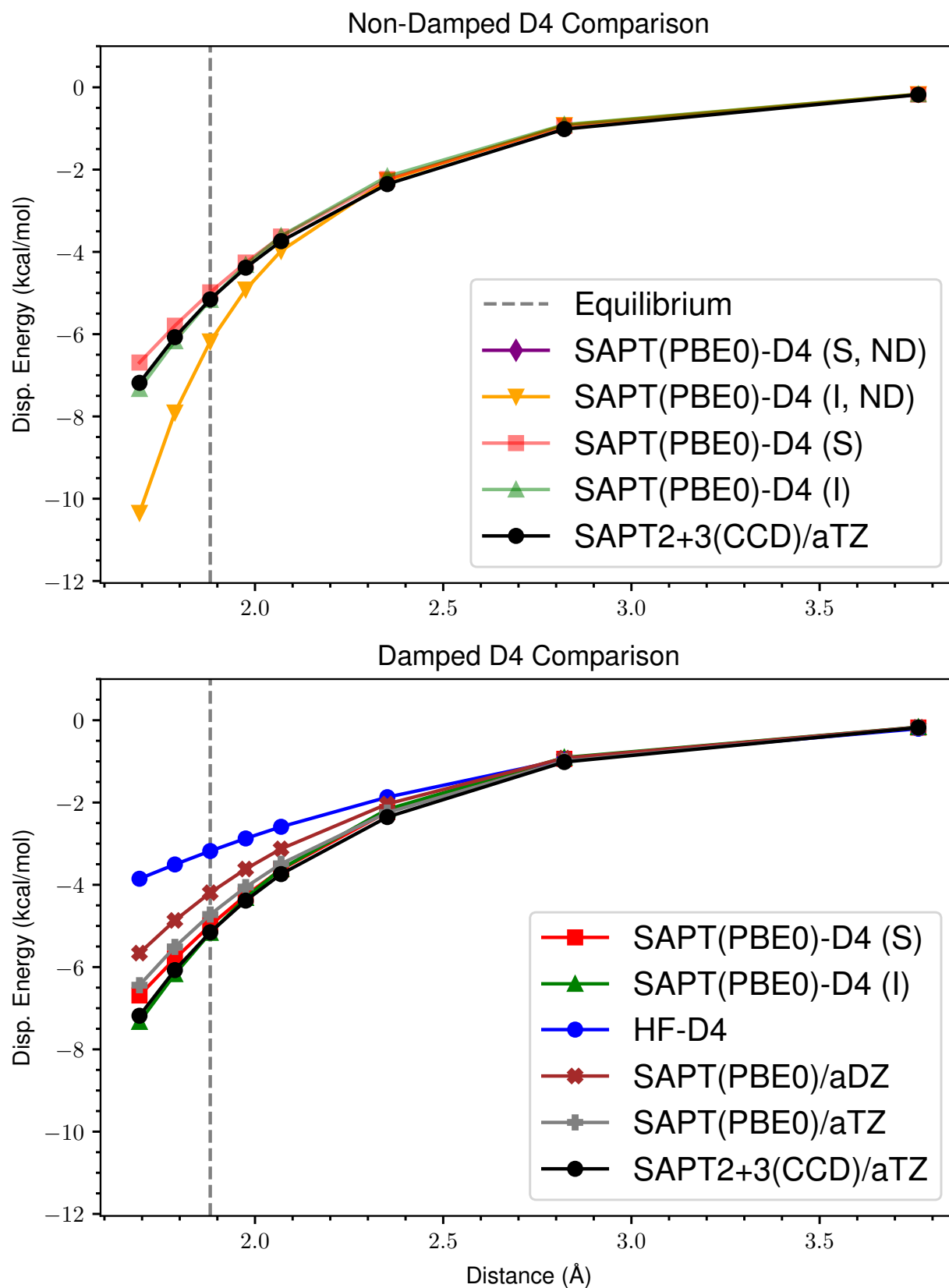
Figure 32: ND vs Damped D4 Dispersion for s66x8 07_MeOH-Peptide
