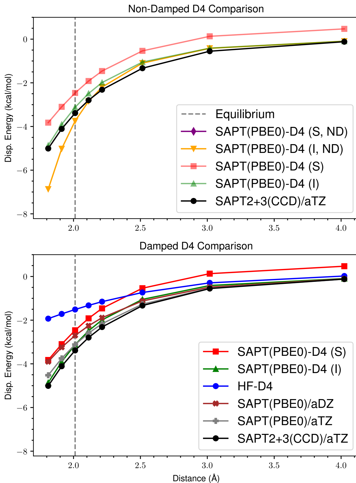
Figure 41: ND vs Damped D4 Dispersion for s66x8 03_Water-MeNH2
