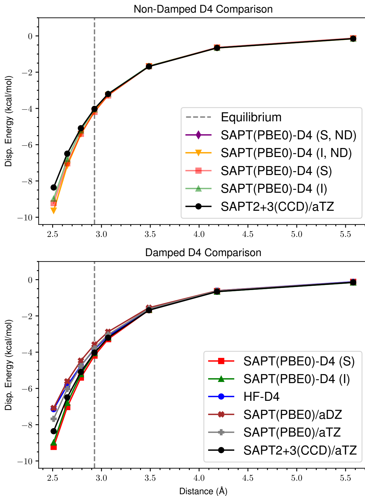
Figure 64: ND vs Damped D4 Dispersion for s66x8 49_Benzene-Pyridine
