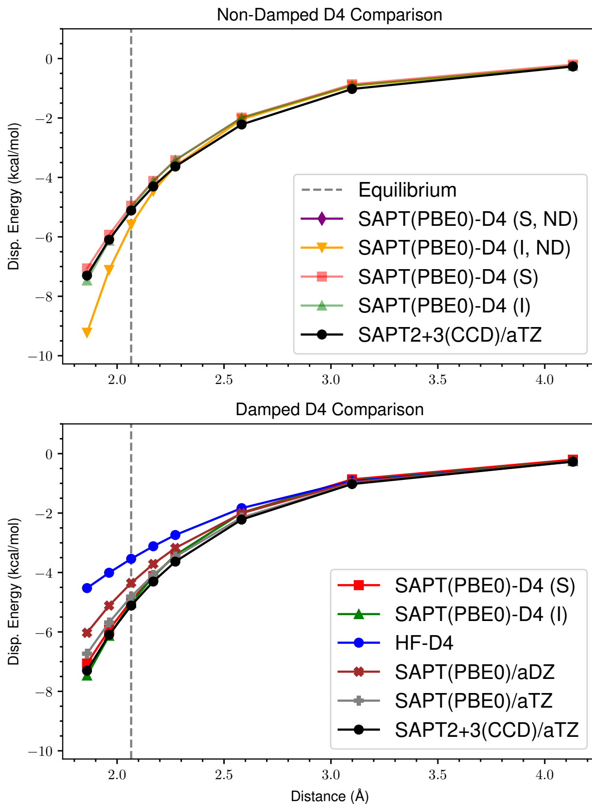
Figure 1: ND vs Damped D4 Dispersion for s66x8 14.Peptide-MeNH2
