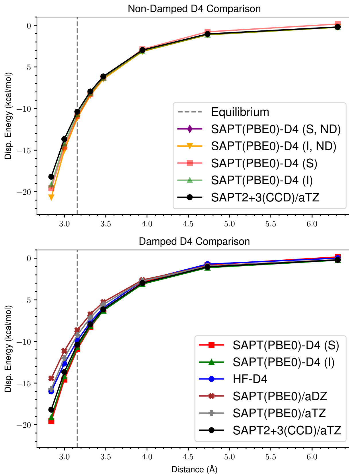
Figure 18: ND vs Damped D4 Dispersion for s66x8 29_Pyridine-Uracil
