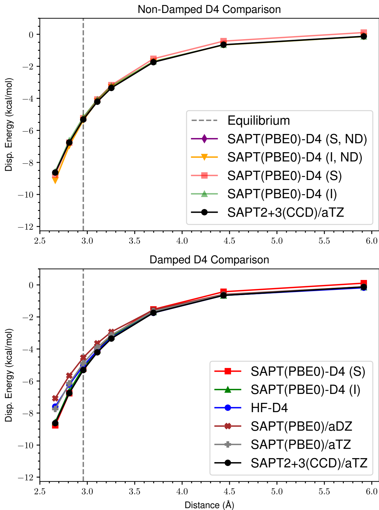
Figure 23: ND vs Damped D4 Dispersion for s66x8 31_Uracil-Ethene
