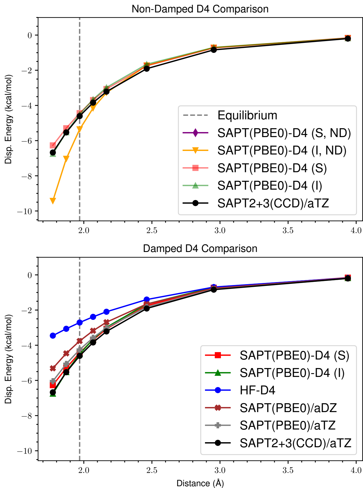
Figure 48: ND vs Damped D4 Dispersion for s66x8 06_MeOH-MeNH2
