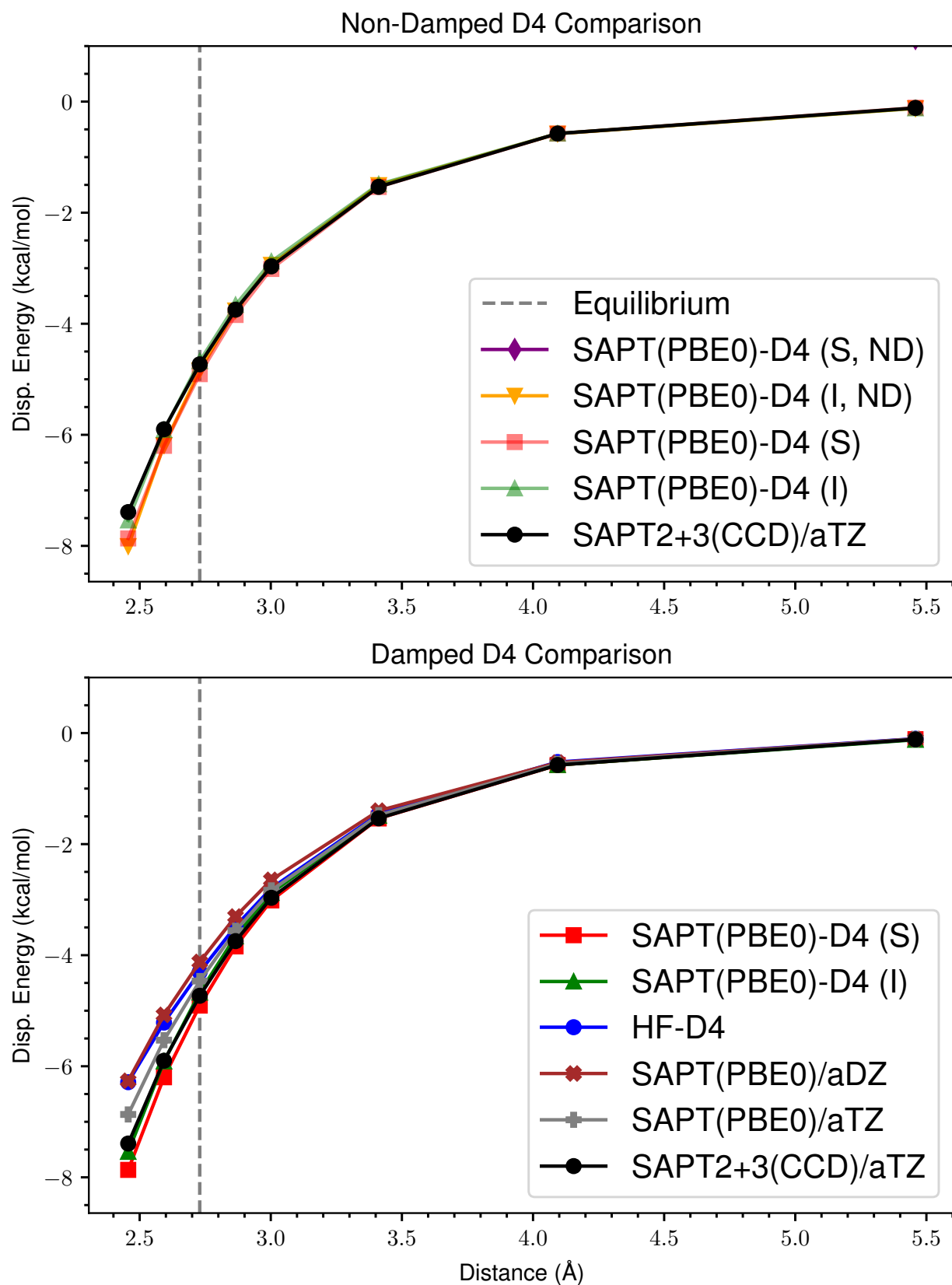
Figure 44: ND vs Damped D4 Dispersion for s66x8 56 Benzene-MeNH2
