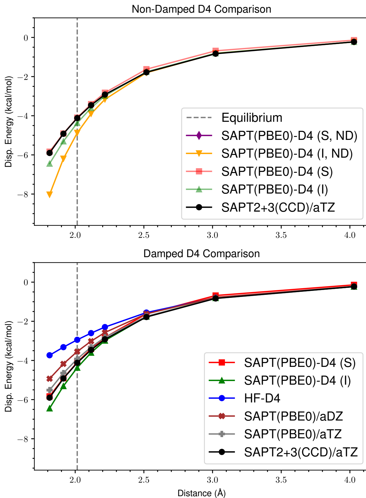
Figure 56: ND vs Damped D4 Dispersion for s66x8 13_Peptide-MeOH
