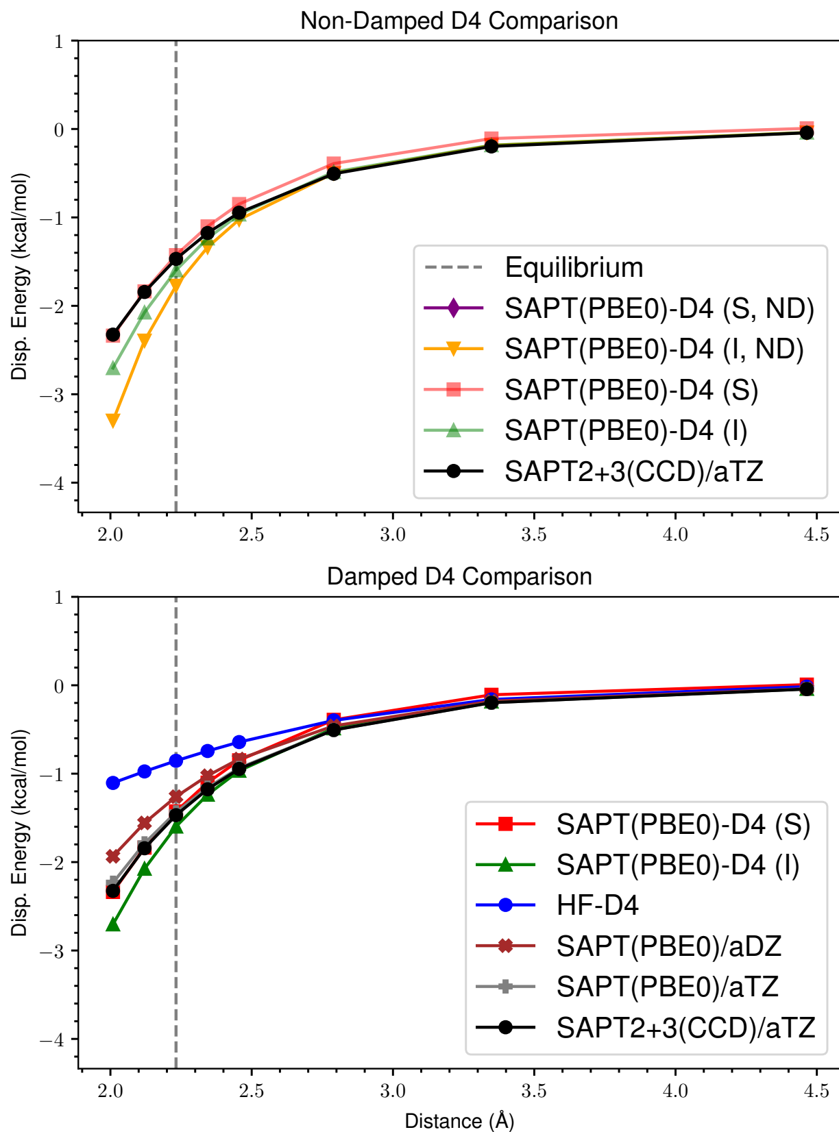
Figure 30: ND vs Damped D4 Dispersion for s66x8 59_Ethyne-Water
