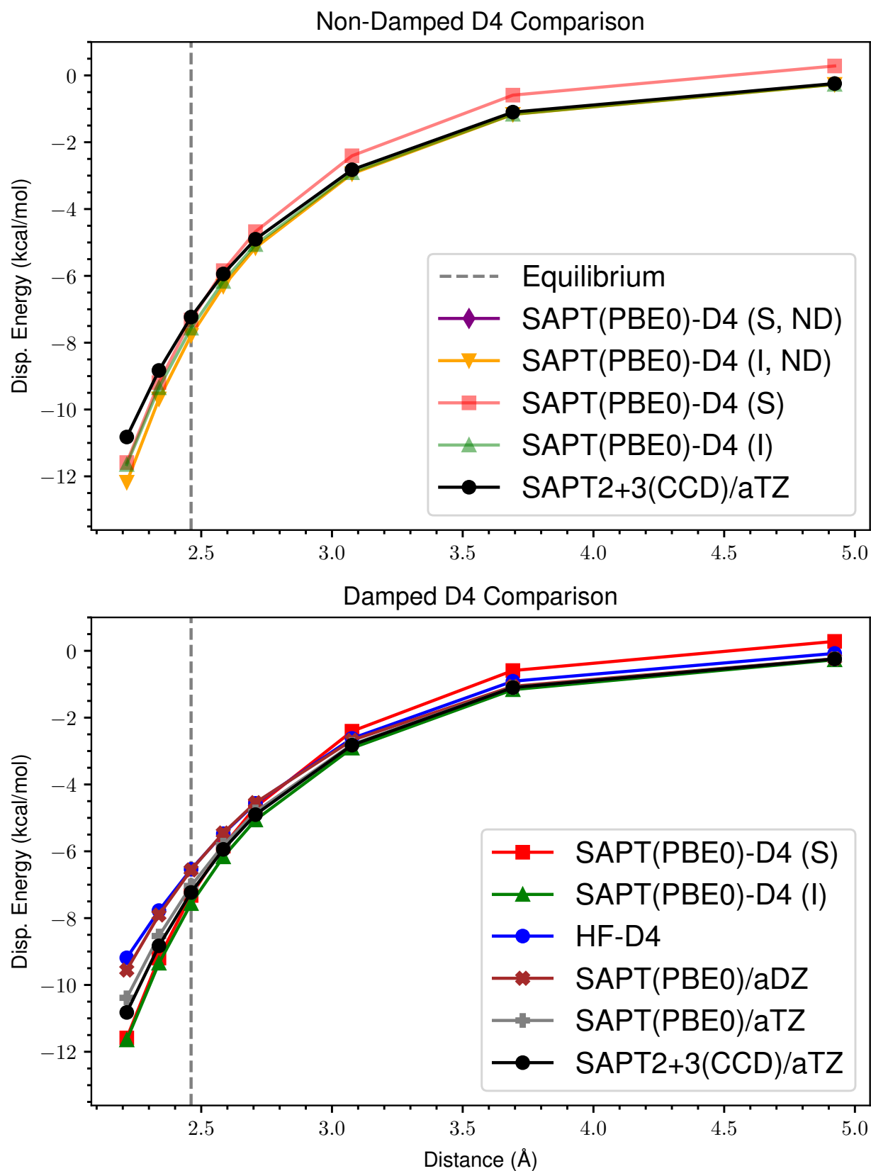
Figure 45: ND vs Damped D4 Dispersion for s66x8 46_Peptide-Pentane
