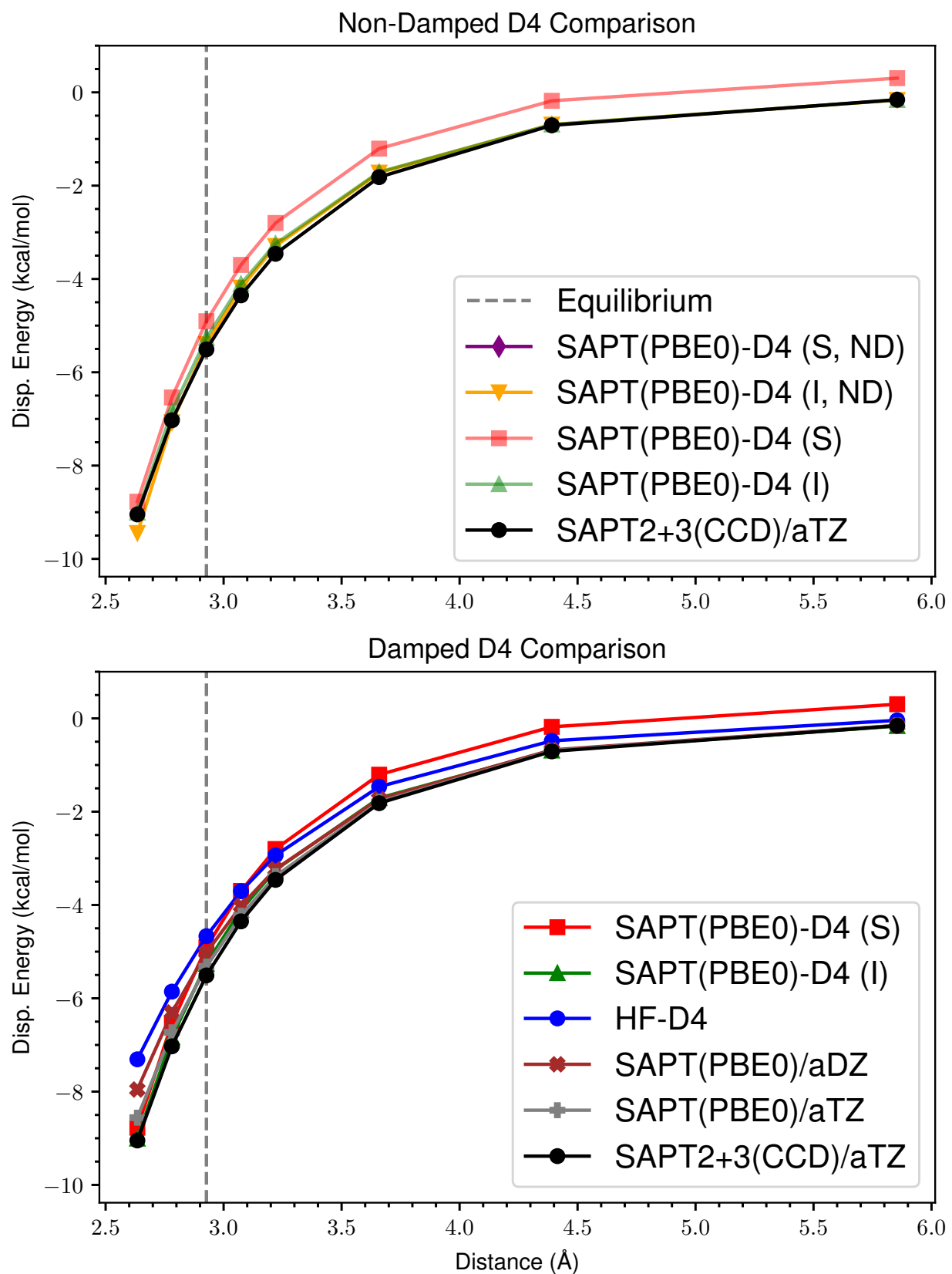
Figure 59: ND vs Damped D4 Dispersion for s66x8 40_Benzene-Neopentane
