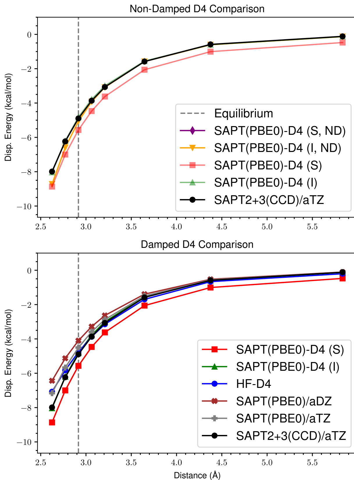
Figure 65: ND vs Damped D4 Dispersion for s66x8 32_Uracil-Ethyne
