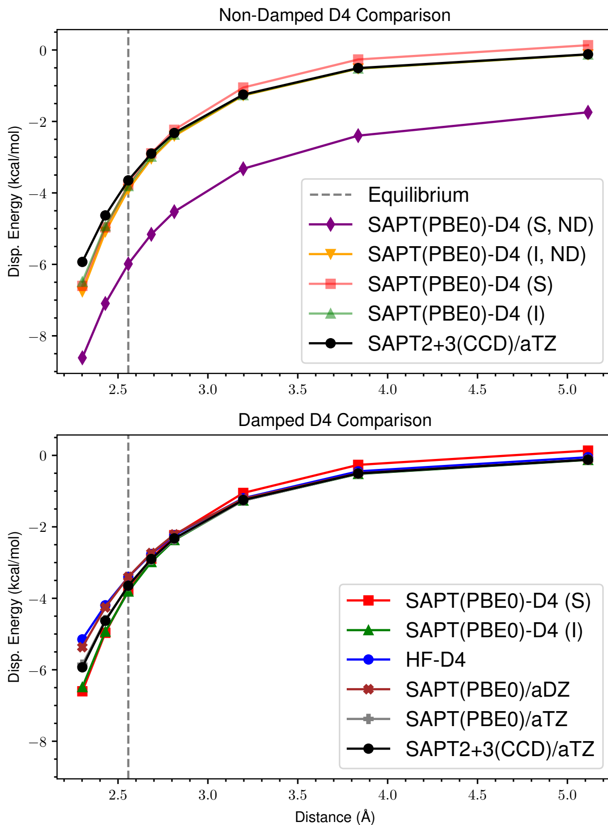
Figure 7: ND vs Damped D4 Dispersion for s66x8 44 Ethene-Pentane
