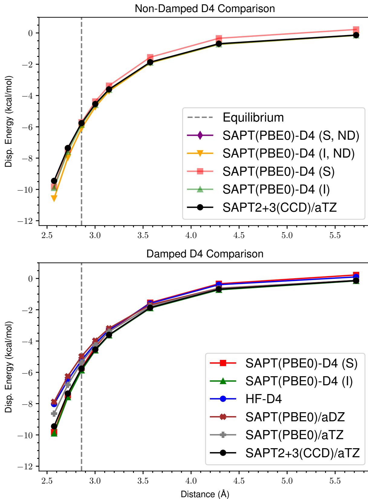
Figure 39: ND vs Damped D4 Dispersion for s66x8 63_Benzene-AcOH
