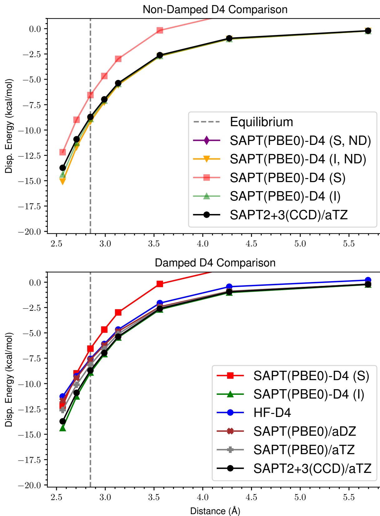
Figure 3: ND vs Damped D4 Dispersion for s66x8 41_Uracil-Pentane
