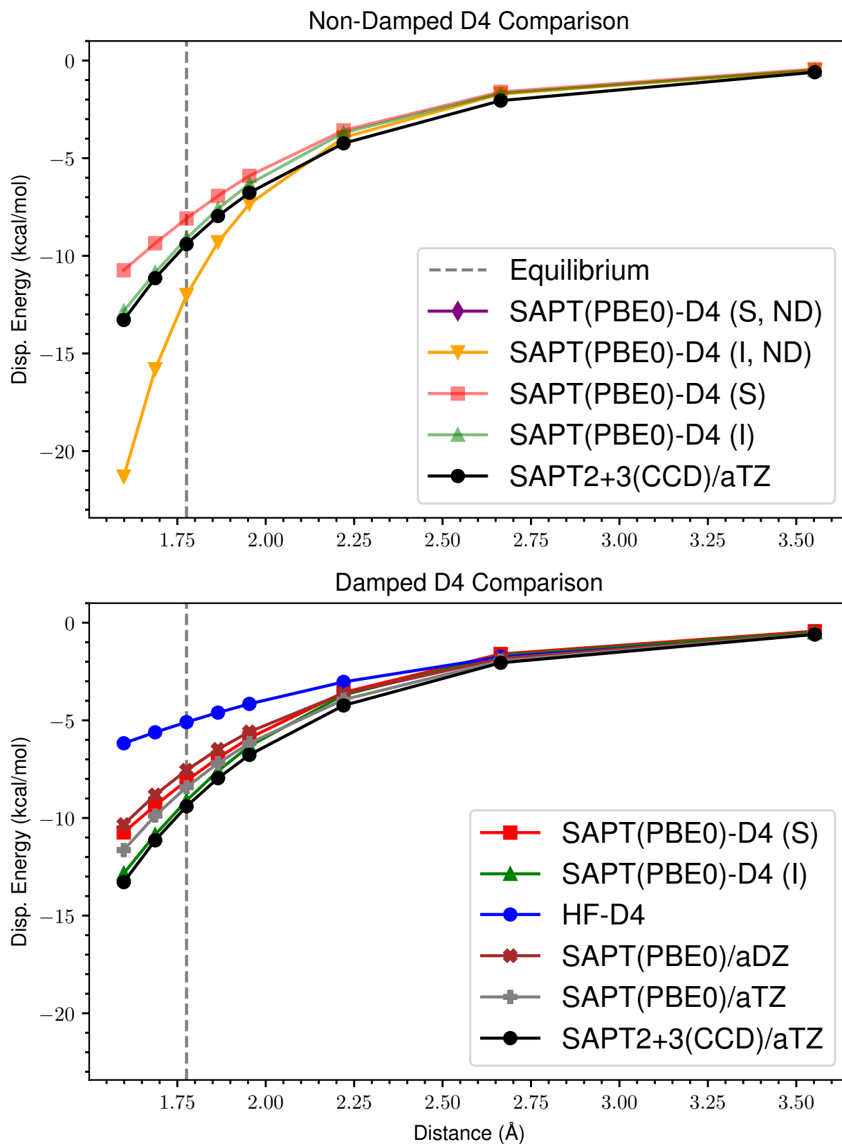
Figure 46: ND vs Damped D4 Dispersion for s66x8 17_Uracil-Uracil
