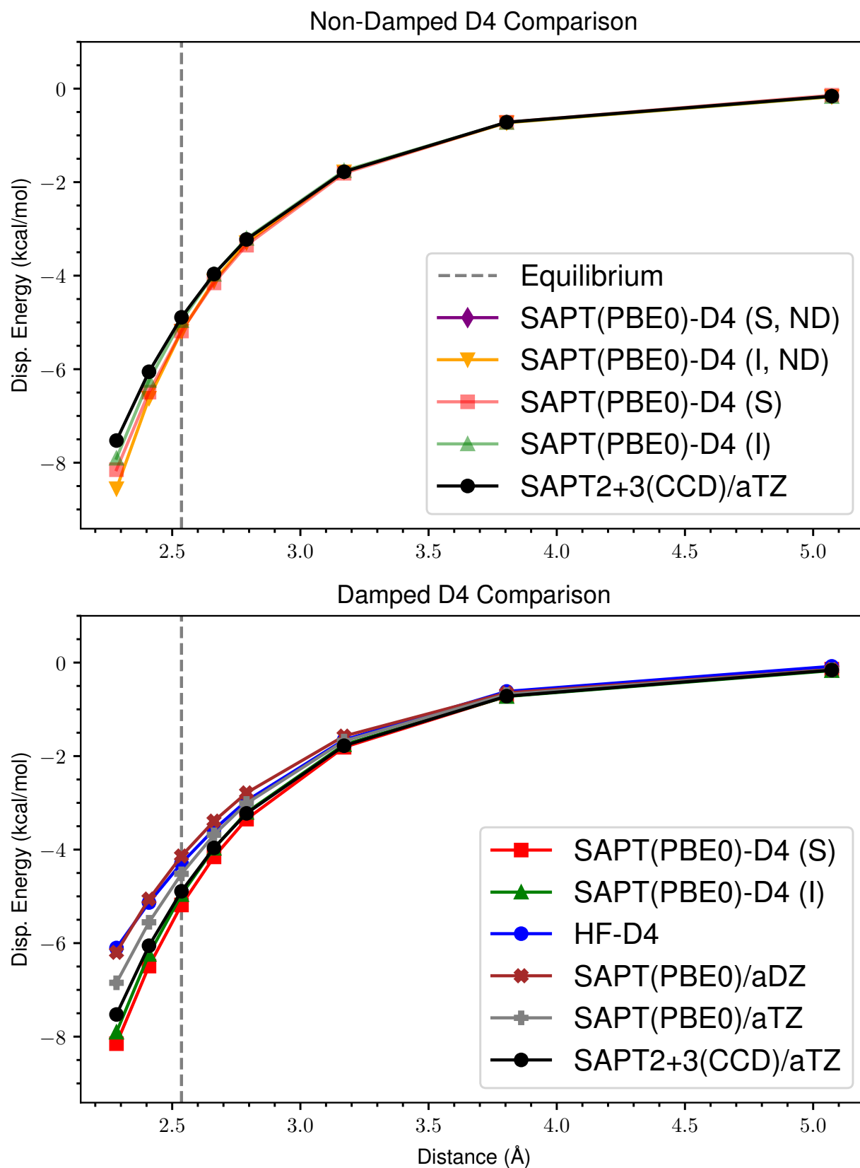
Figure 19: ND vs Damped D4 Dispersion for s66x8 55_Benzene-MeOH
