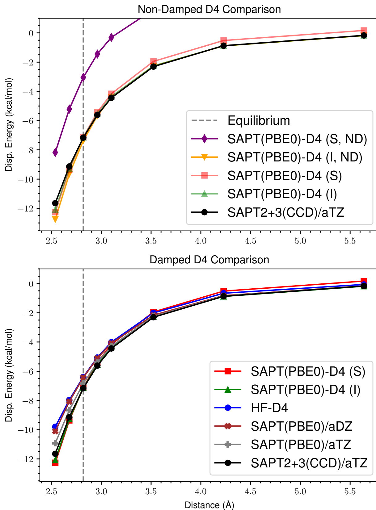
Figure 54: ND vs Damped D4 Dispersion for s66x8 39_Benzene-Cyclopentane
