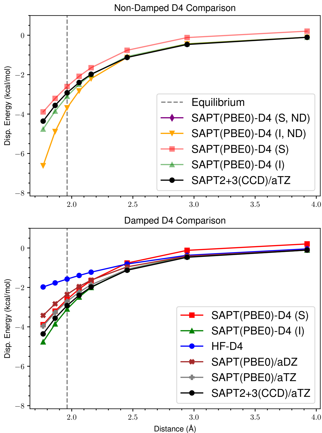
Figure 8: ND vs Damped D4 Dispersion for s66x8 02 Water-MeOH
