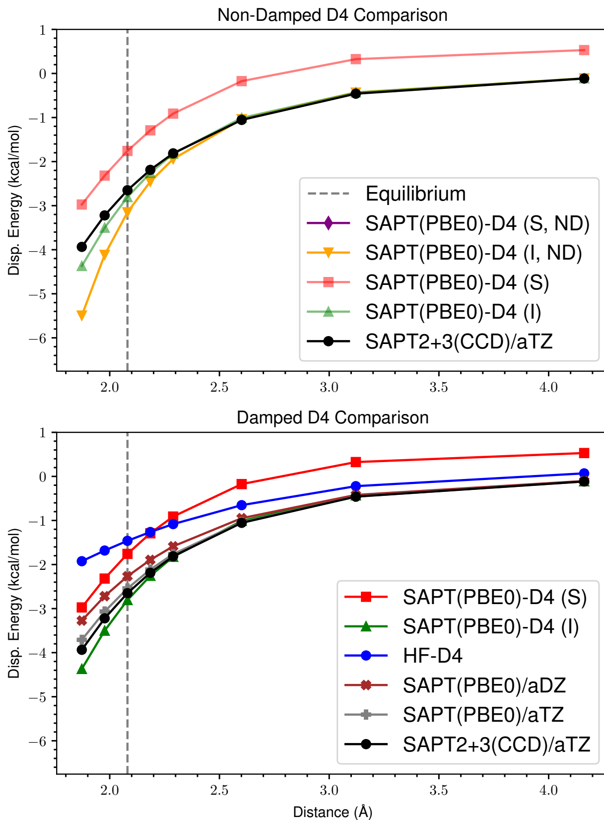
Figure 6: ND vs Damped D4 Dispersion for s66x8 16_Peptide-Water
