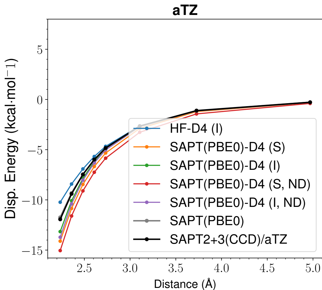
Figure 29: LoS Dispersion Curves for s66x8 34_Pentane-Pentane
