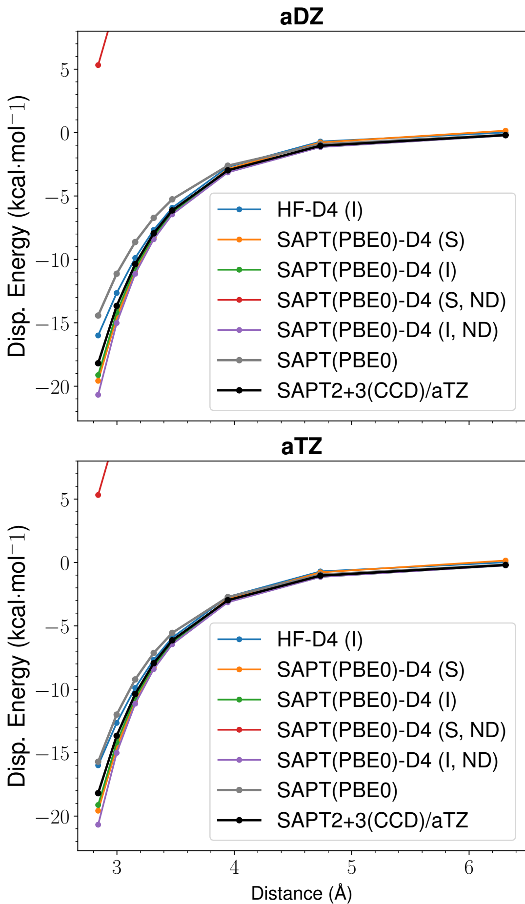
Figure 38: LoS Dispersion Curves for s66x8 29_Pyridine-Uracil
