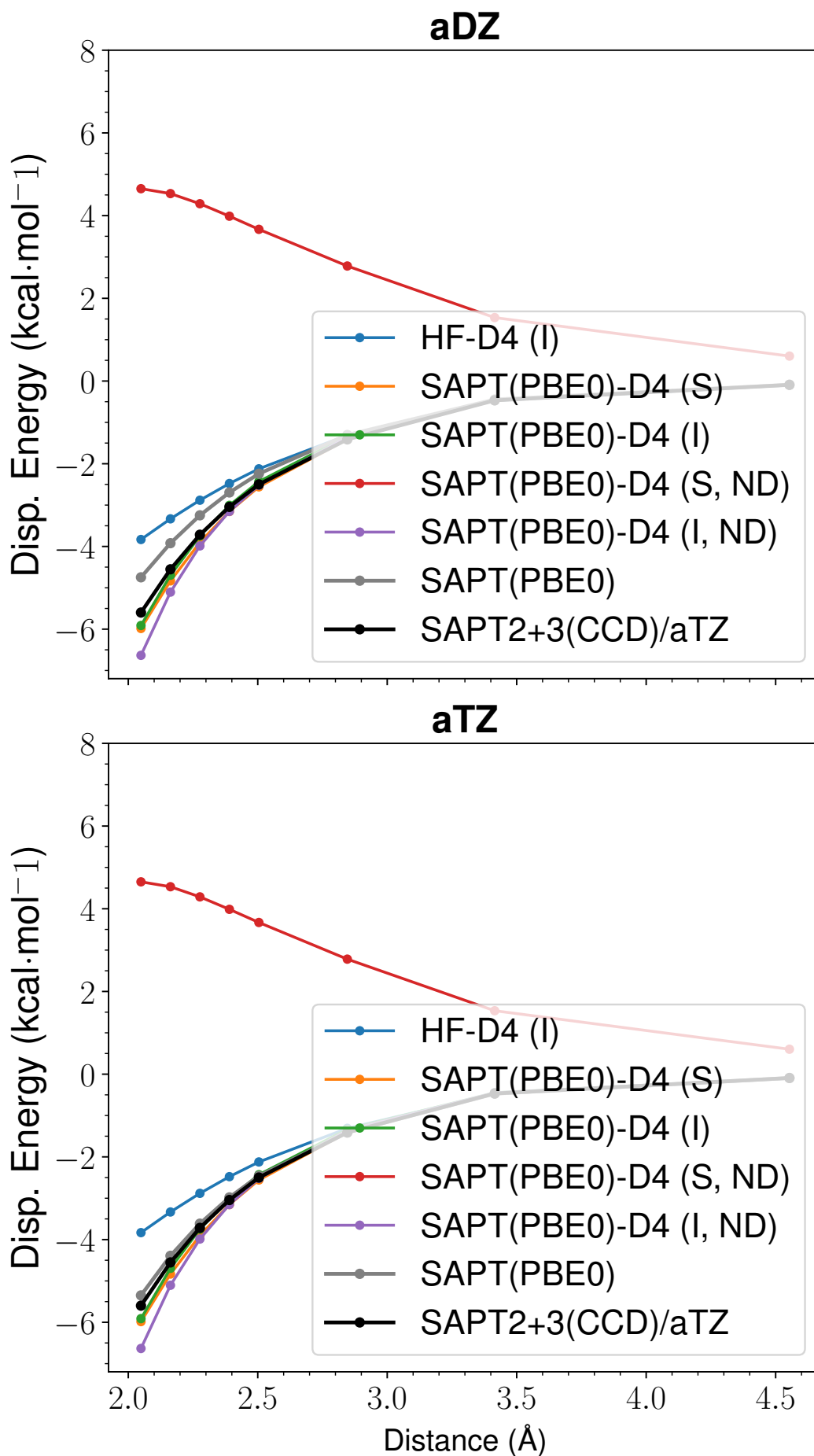
Figure 17: LoS Dispersion Curves for s66x8 10_MeNH2-MeNH2
