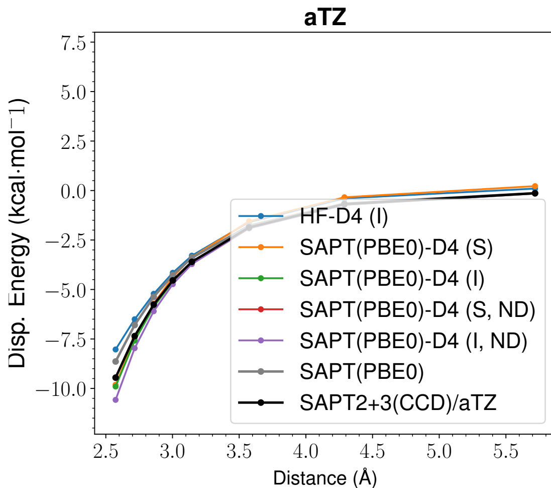
Figure 8: LoS Dispersion Curves for s66x8 63_Benzene-AcOH
