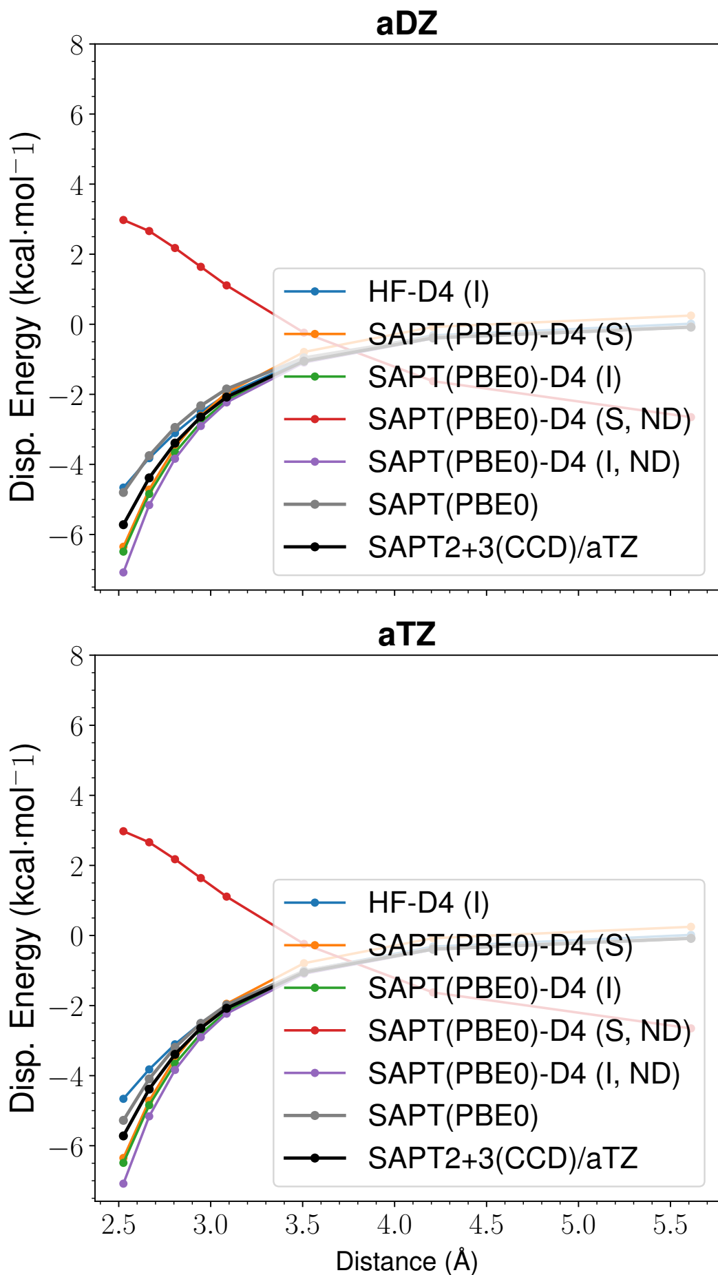
Figure 4: LoS Dispersion Curves for s66x8 50 Benzene-Ethyne
