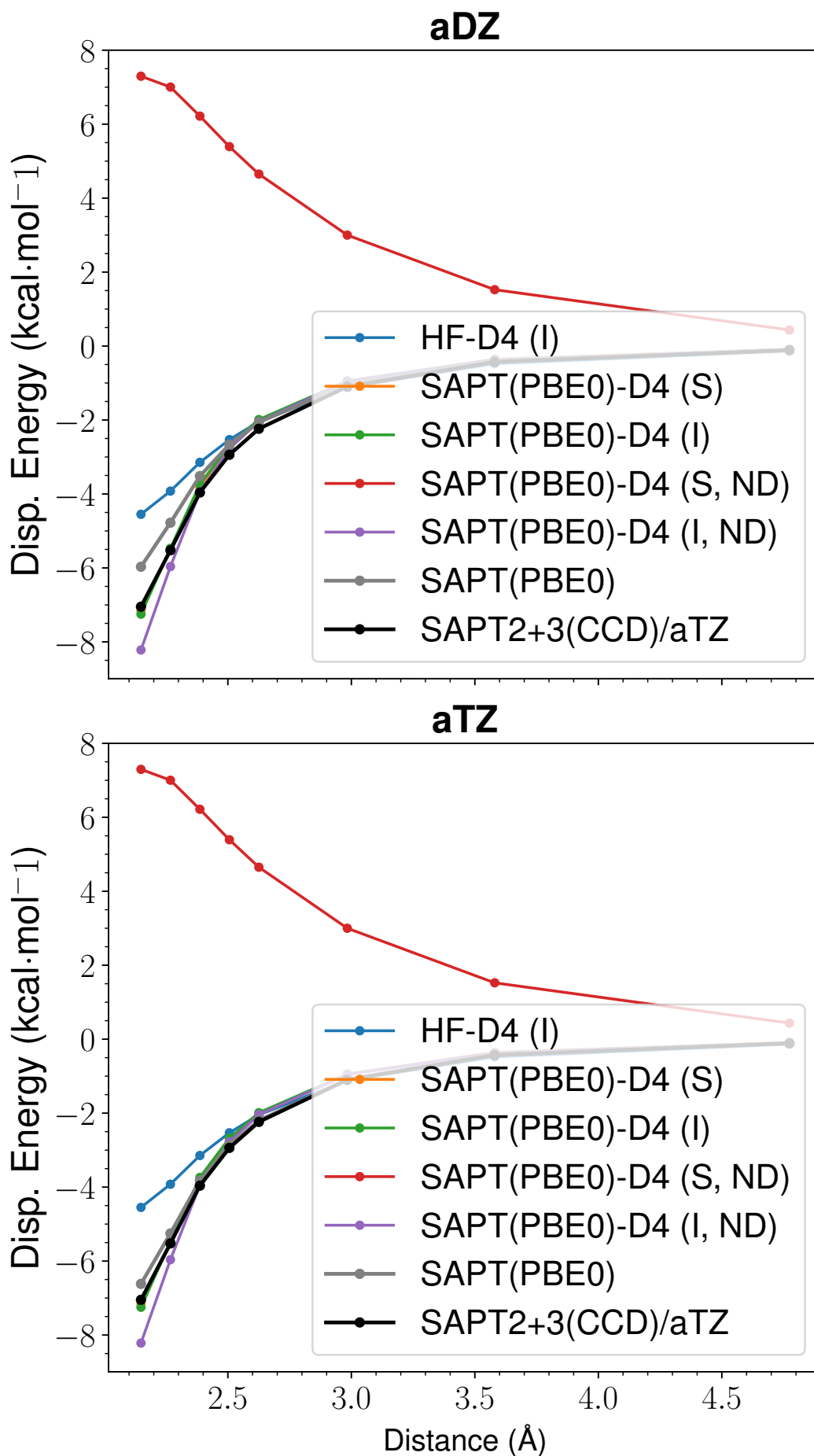
Figure 18: LoS Dispersion Curves for s66x8 58_Pyridine-Pyridine
