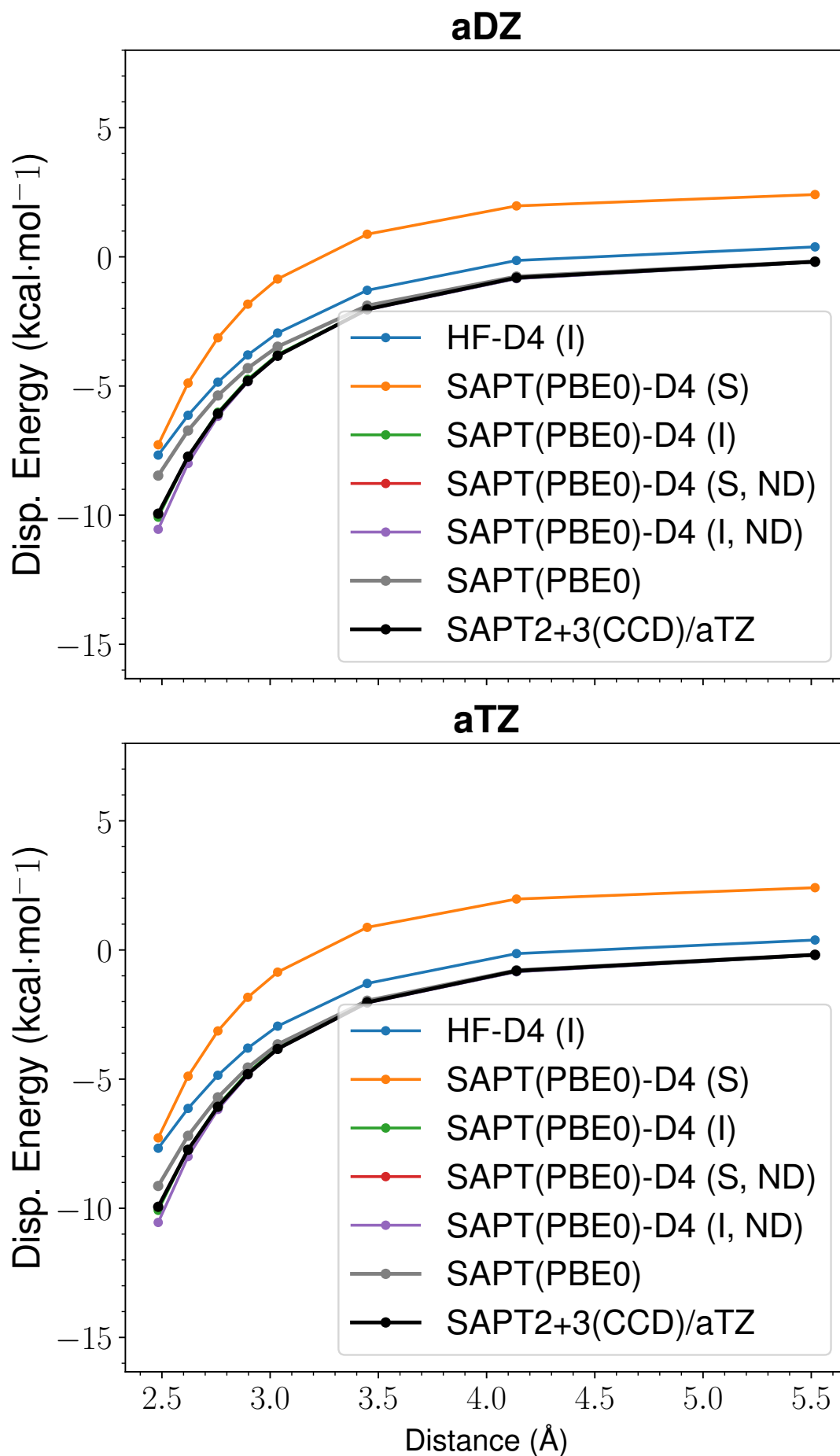
Figure 39: LoS Dispersion Curves for s66x8 43_Uracil-Neopentane
