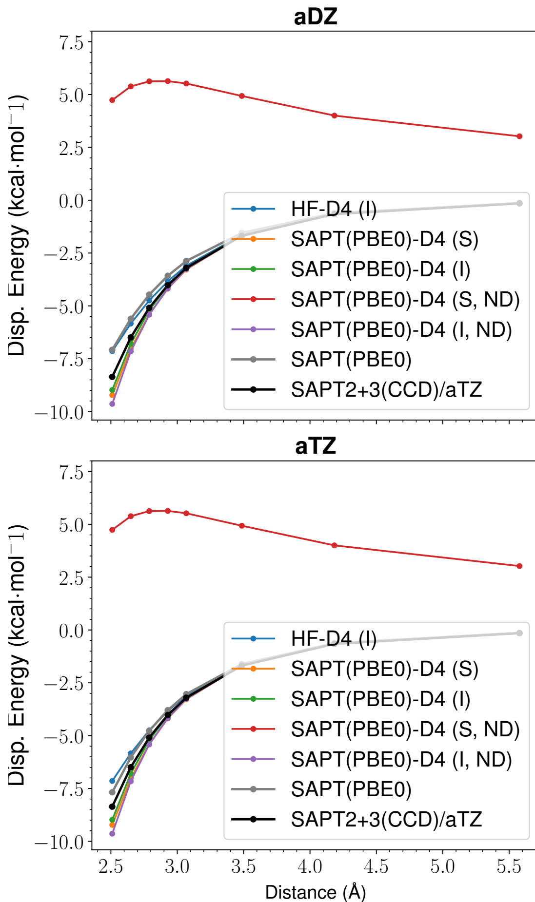
Figure 6: LoS Dispersion Curves for s66x8 49_Benzene-Pyridine
