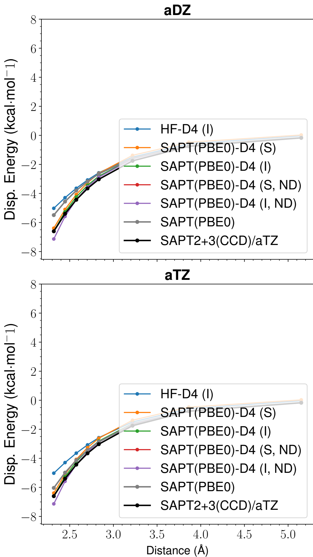
Figure 7: LoS Dispersion Curves for s66x8 53_Benzene-AcNH2
