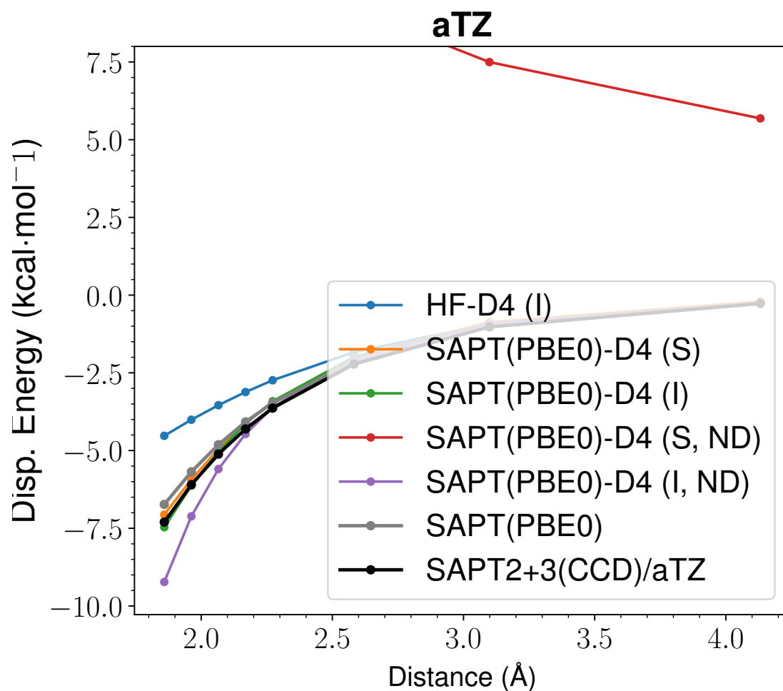
Figure 63: LoS Dispersion Curves for s66x8 14_Peptide-MeNH2
