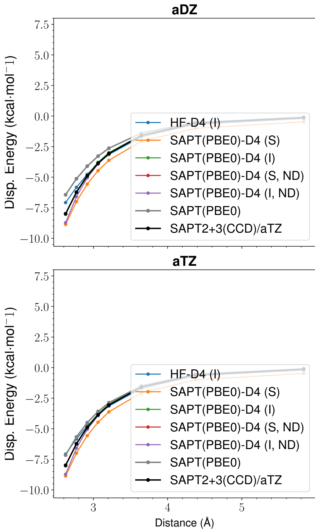
Figure 24: LoS Dispersion Curves for s66x8 32_Uracil-Ethyne
