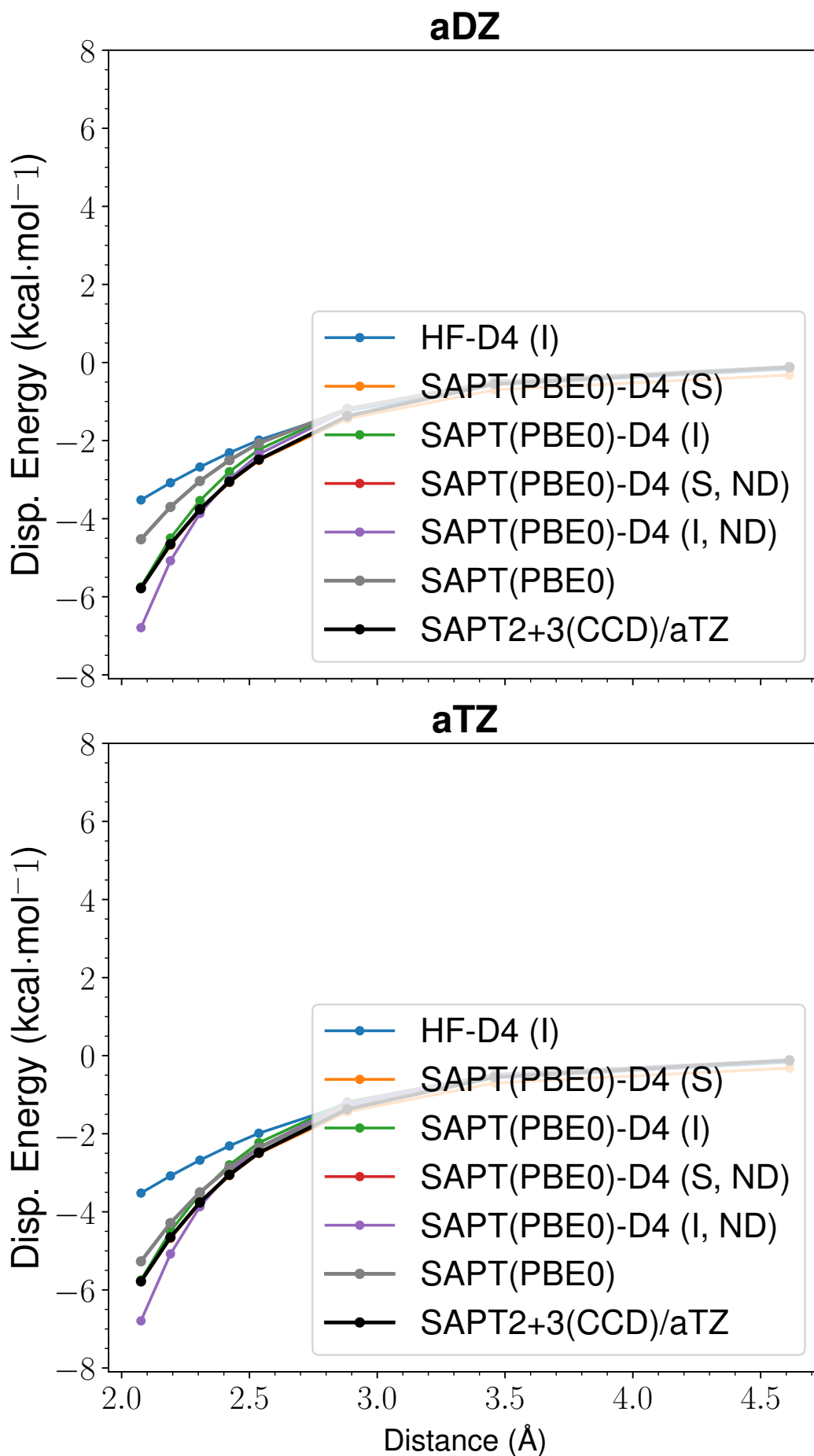
Figure 64: LoS Dispersion Curves for s66x8 60_Ethyne-AcOH
