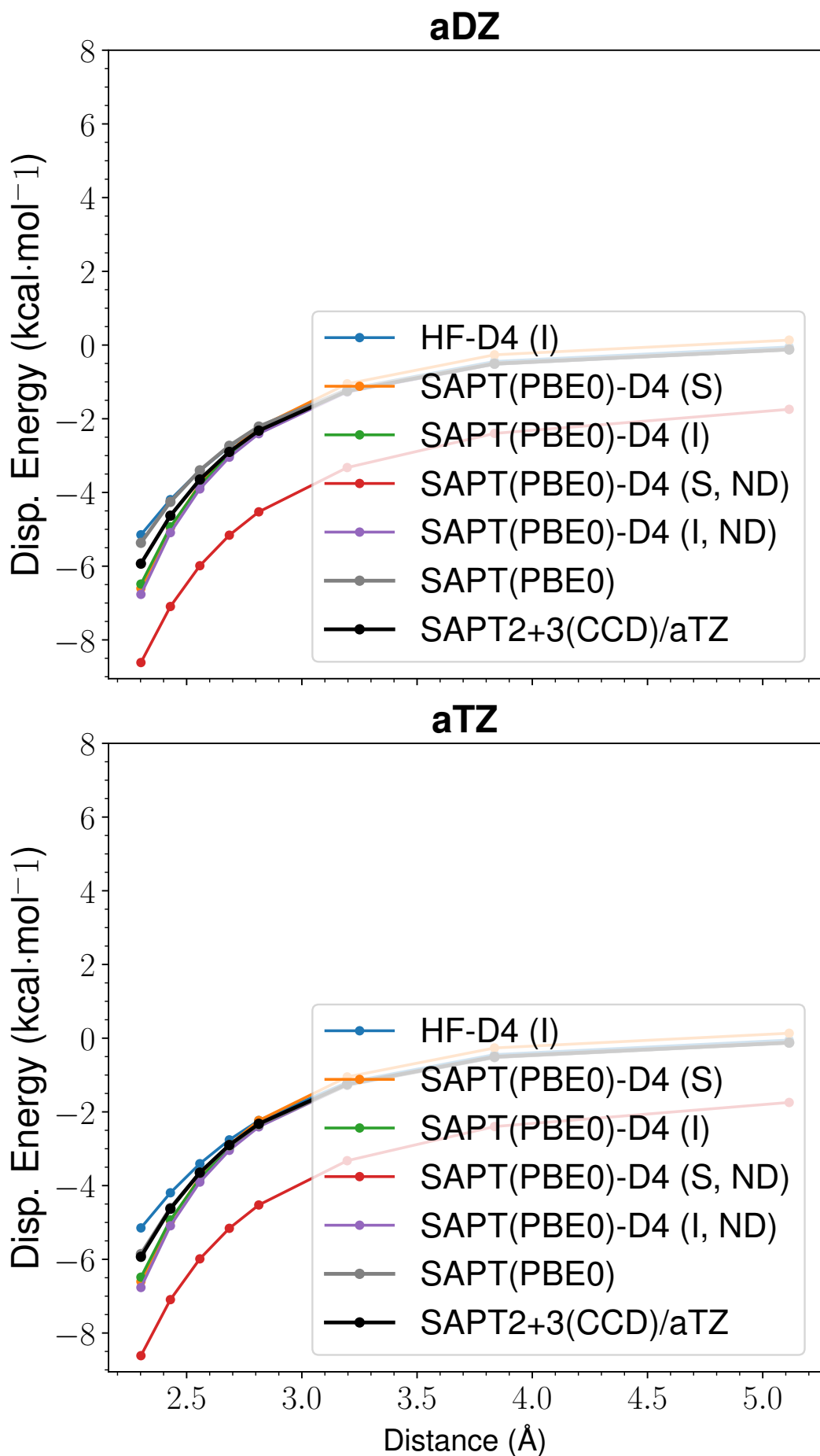
Figure 13: LoS Dispersion Curves for s66x8 44_Ethene-Pentane
