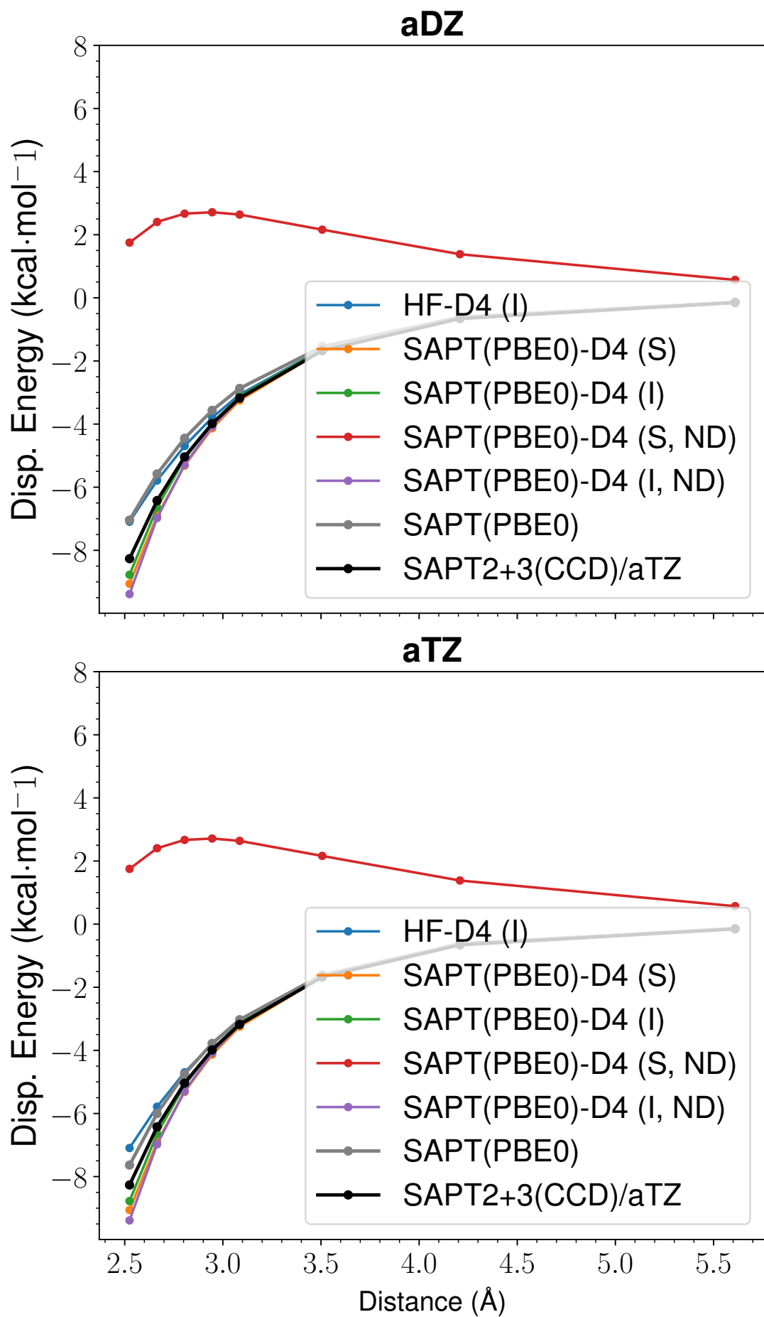
Figure 34: LoS Dispersion Curves for s66x8 47_Benzene-Benzene
