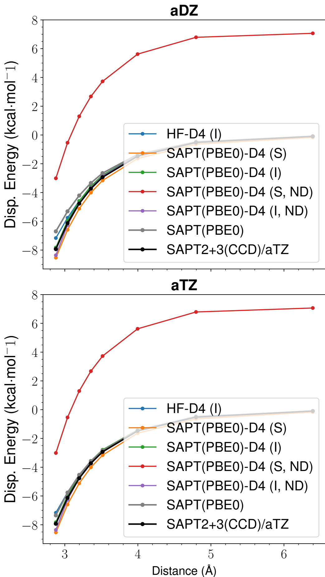
Figure 41: LoS Dispersion Curves for s66x8 33_Pyridine-Ethene
