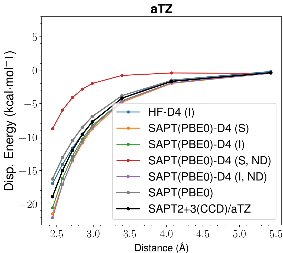
Figure 53: LoS Dispersion Curves for s66x8 26_Uracil-Uracil
