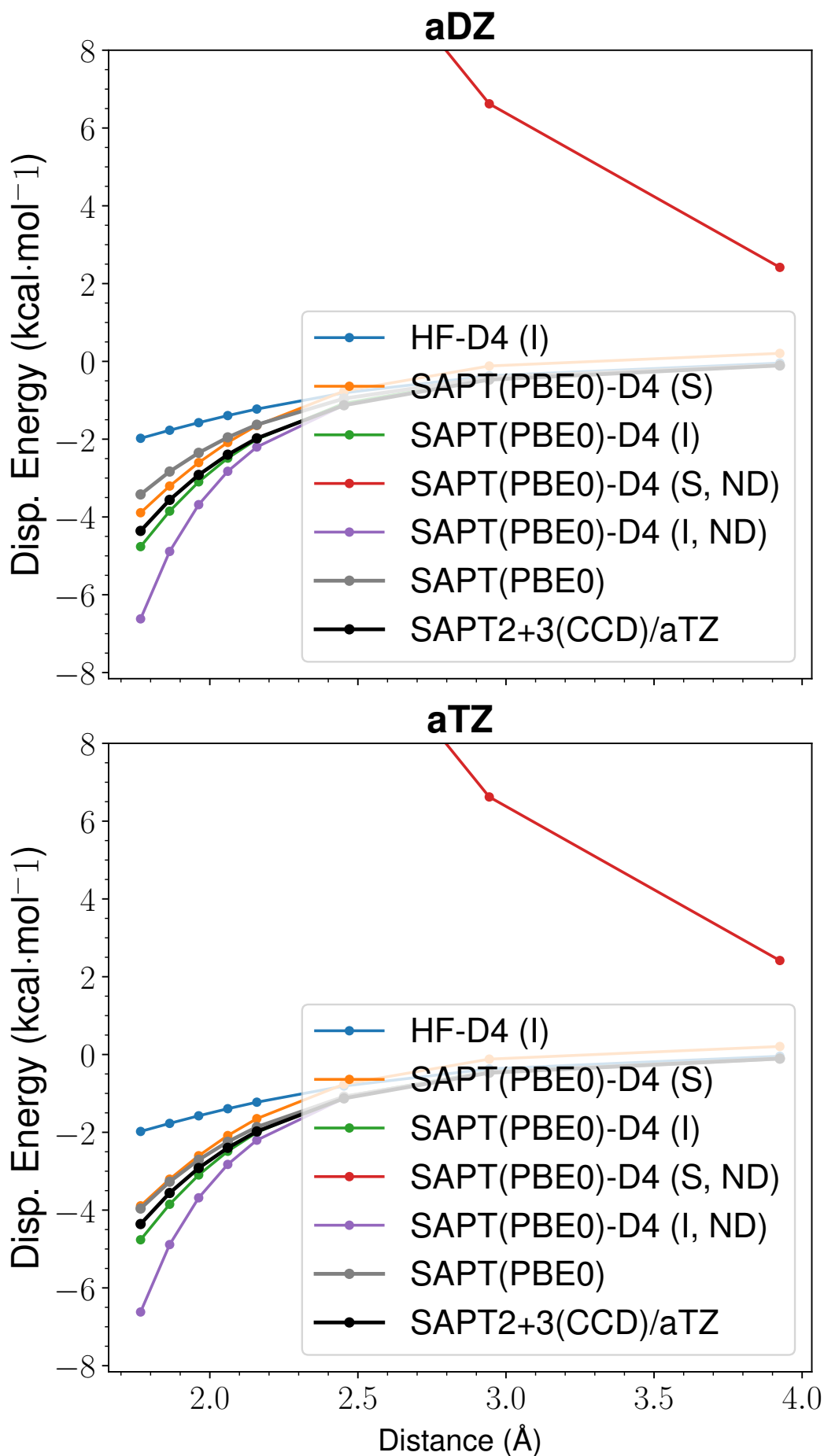
Figure 58: LoS Dispersion Curves for s66x8 02_Water-MeOH
