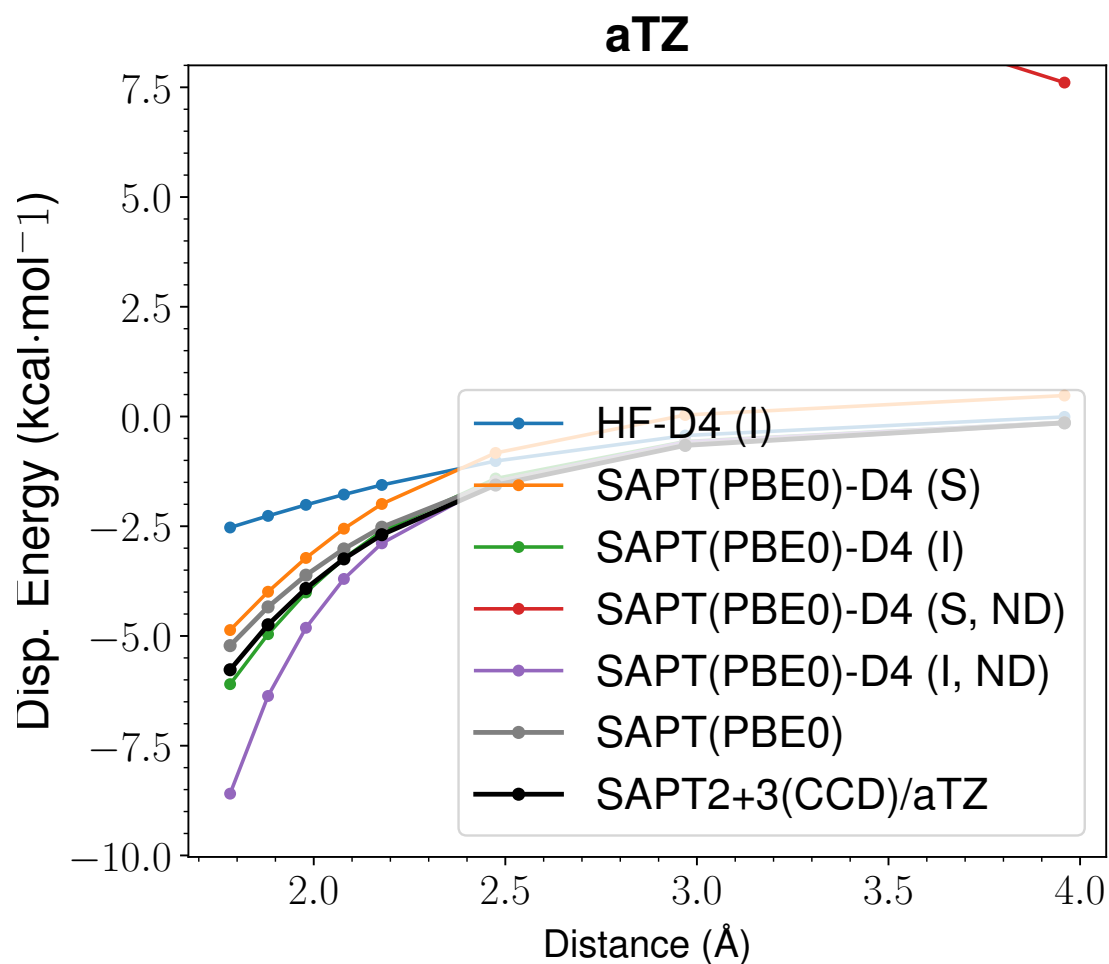
Figure 21: LoS Dispersion Curves for s66x8 12_MeNH2-Water
