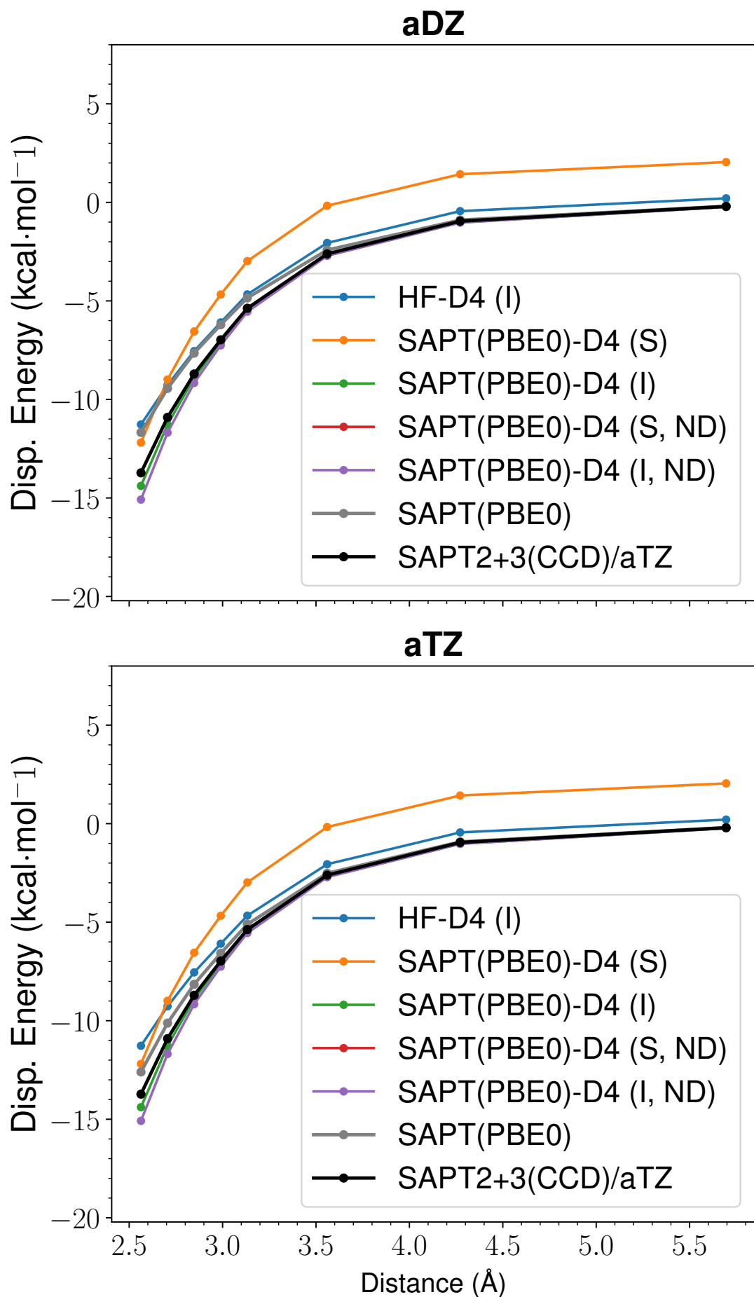
Figure 32: LoS Dispersion Curves for s66x8 41_Uracil-Pentane
