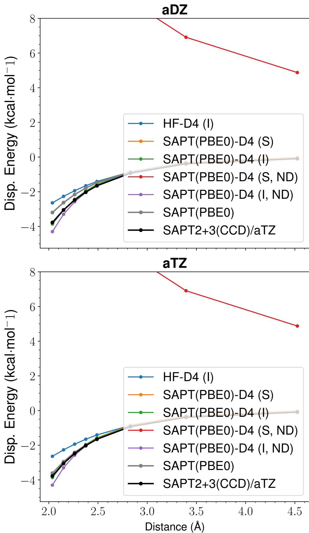
Figure 16: LoS Dispersion Curves for s66x8 09_MeNH2-MeOH
