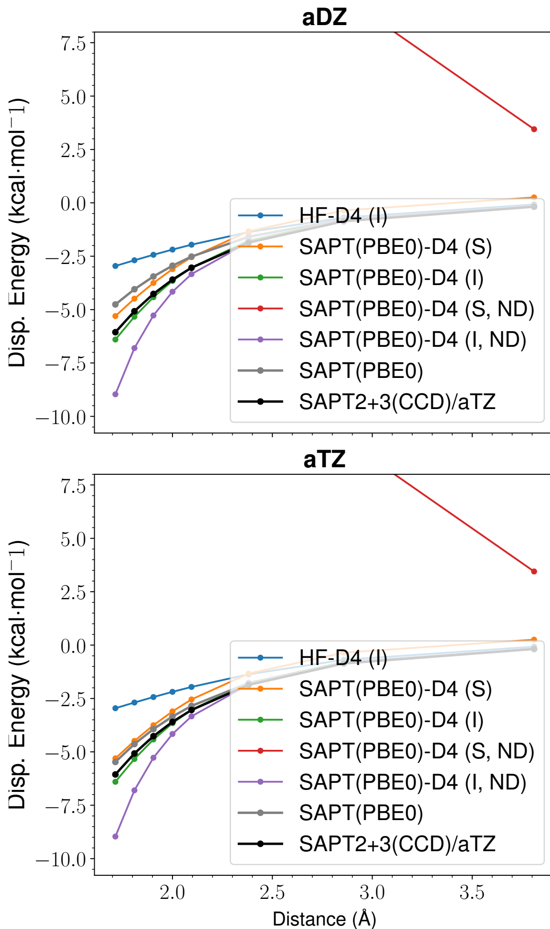
Figure 59: LoS Dispersion Curves for s66x8 04_Water-Peptide
