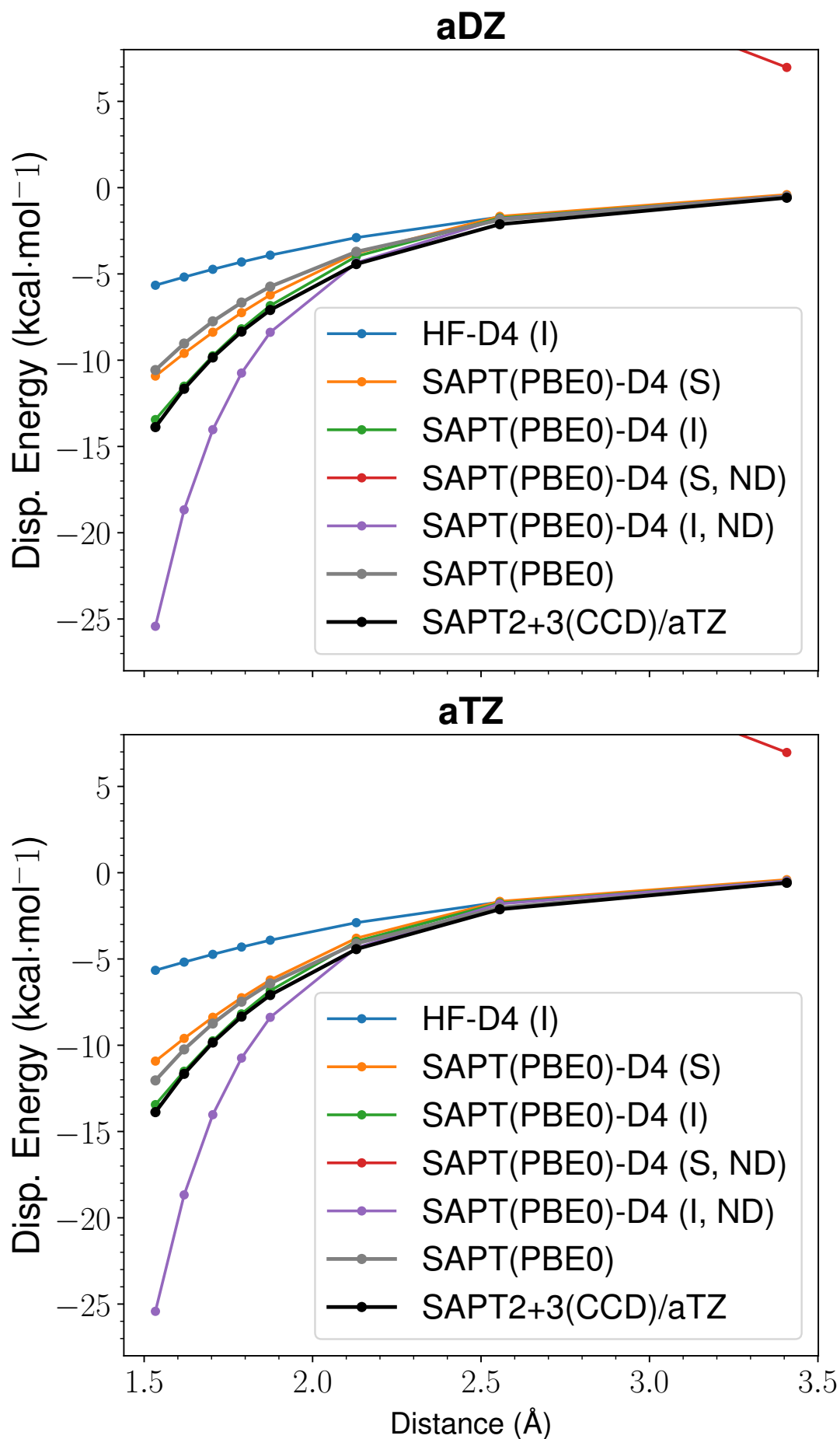
Figure 61: LoS Dispersion Curves for s66x8 22_AcOH-Uracil
