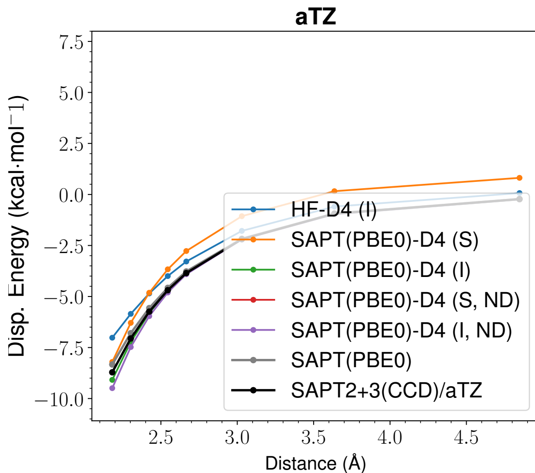
Figure 28: LoS Dispersion Curves for s66x8 62_Pentane-AcNH2
