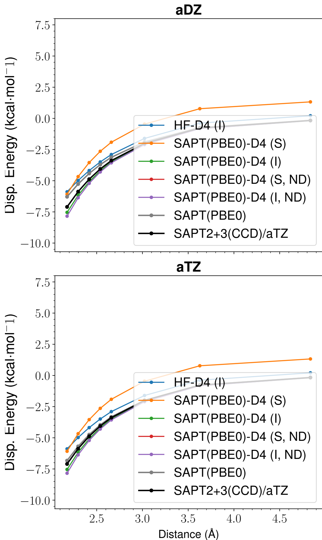
Figure 35: LoS Dispersion Curves for s66x8 61.Pentane-AcOH
