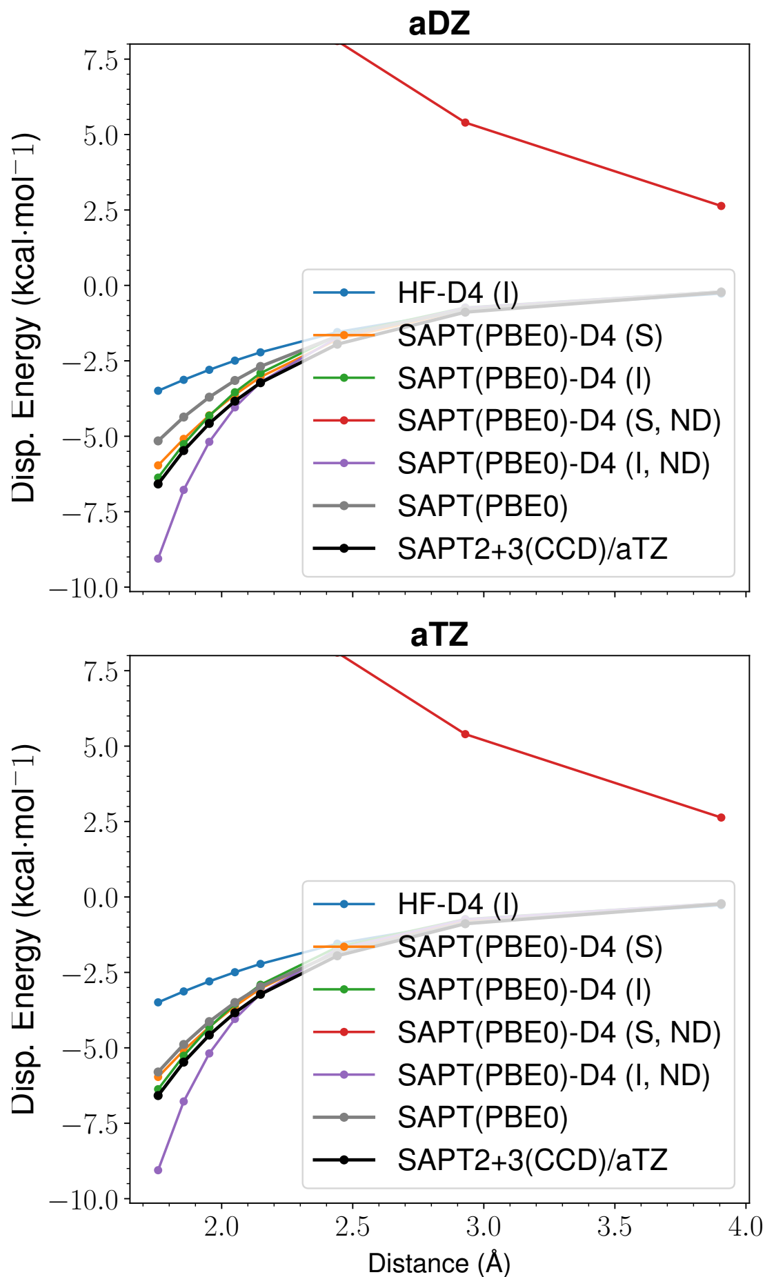
Figure 57: LoS Dispersion Curves for s66x8 19_MeOH-Pyridine
