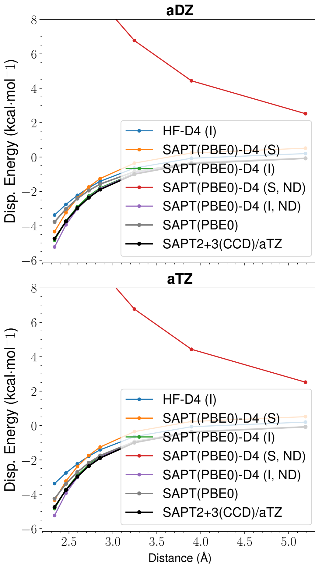
Figure 12: LoS Dispersion Curves for s66x8 54. Benzene-Water
