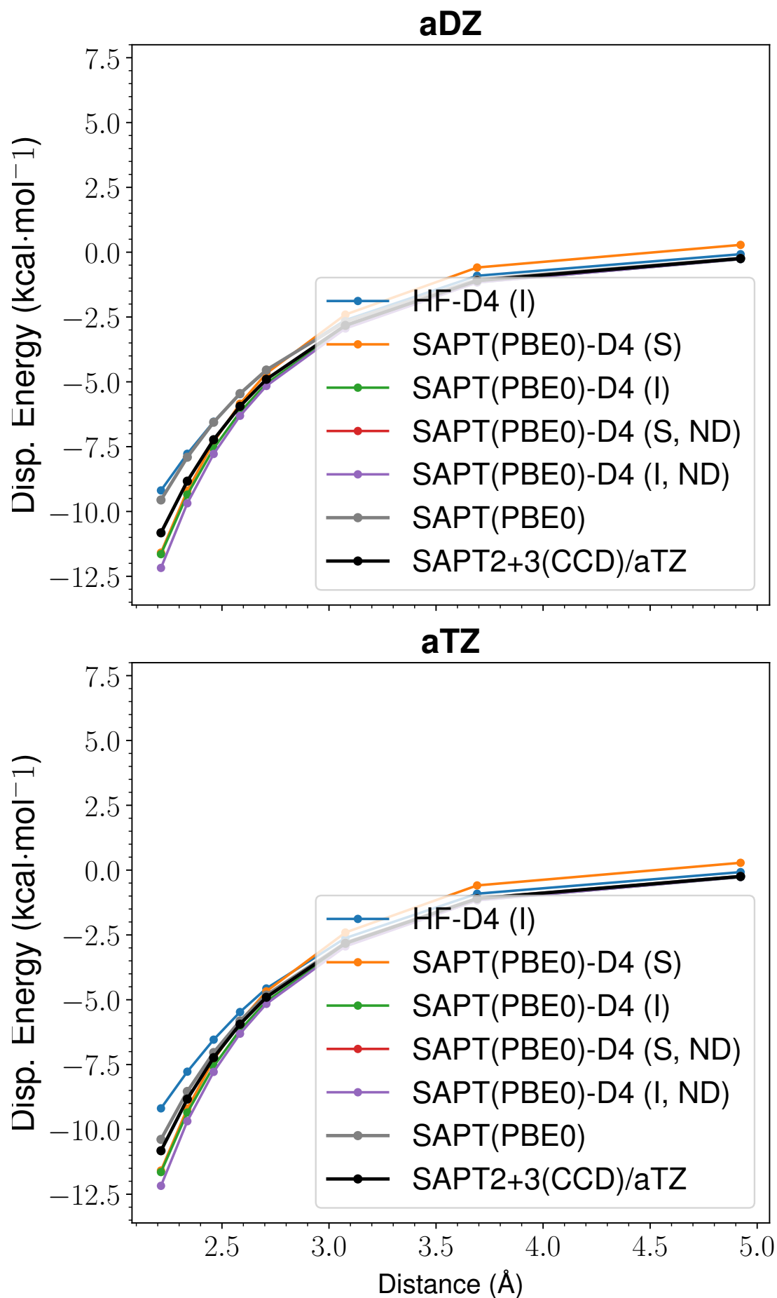
Figure 15: LoS Dispersion Curves for s66x8 46_Peptide-Pentane
