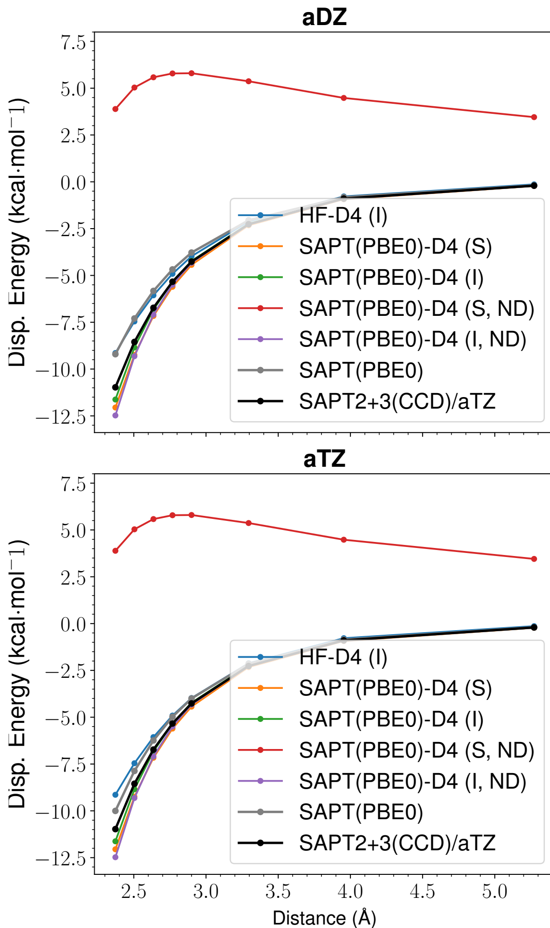
Figure 60: LoS Dispersion Curves for s66x8 57_Benzene-Peptide
