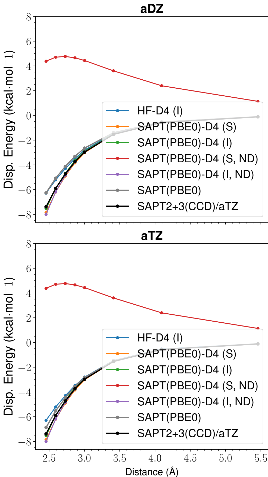
Figure 11: LoS Dispersion Curves for s66x8 56_Benzene-MeNH2
