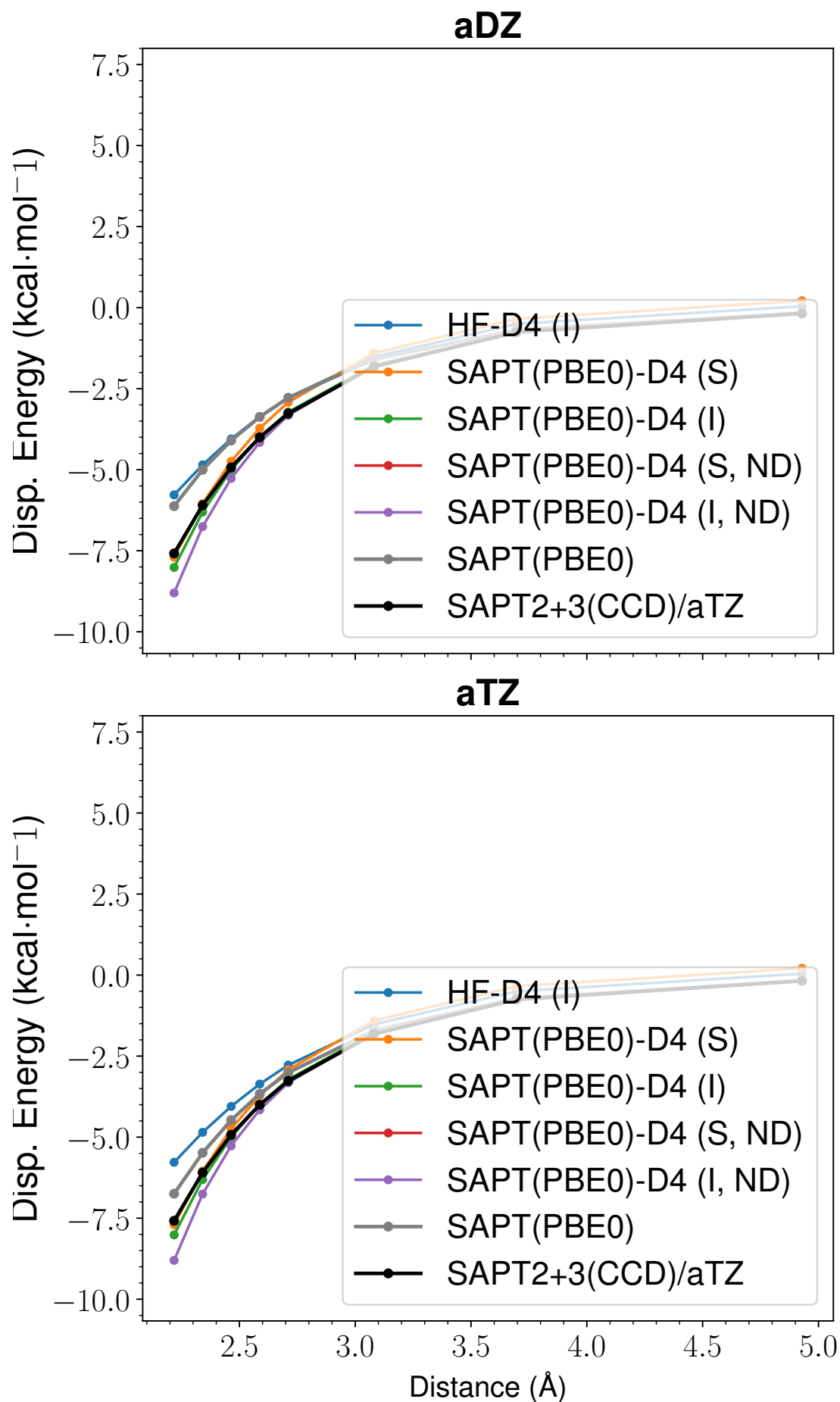
Figure 14: LoS Dispersion Curves for s66x8 52_Benzene-AcOH
