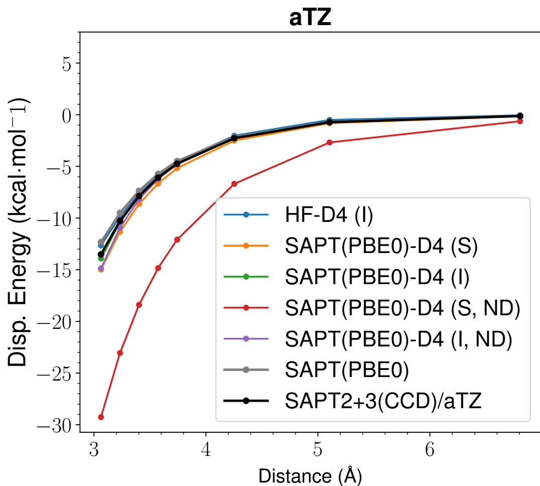
Figure 31: LoS Dispersion Curves for s66x8 24_Benzene-Benzene
