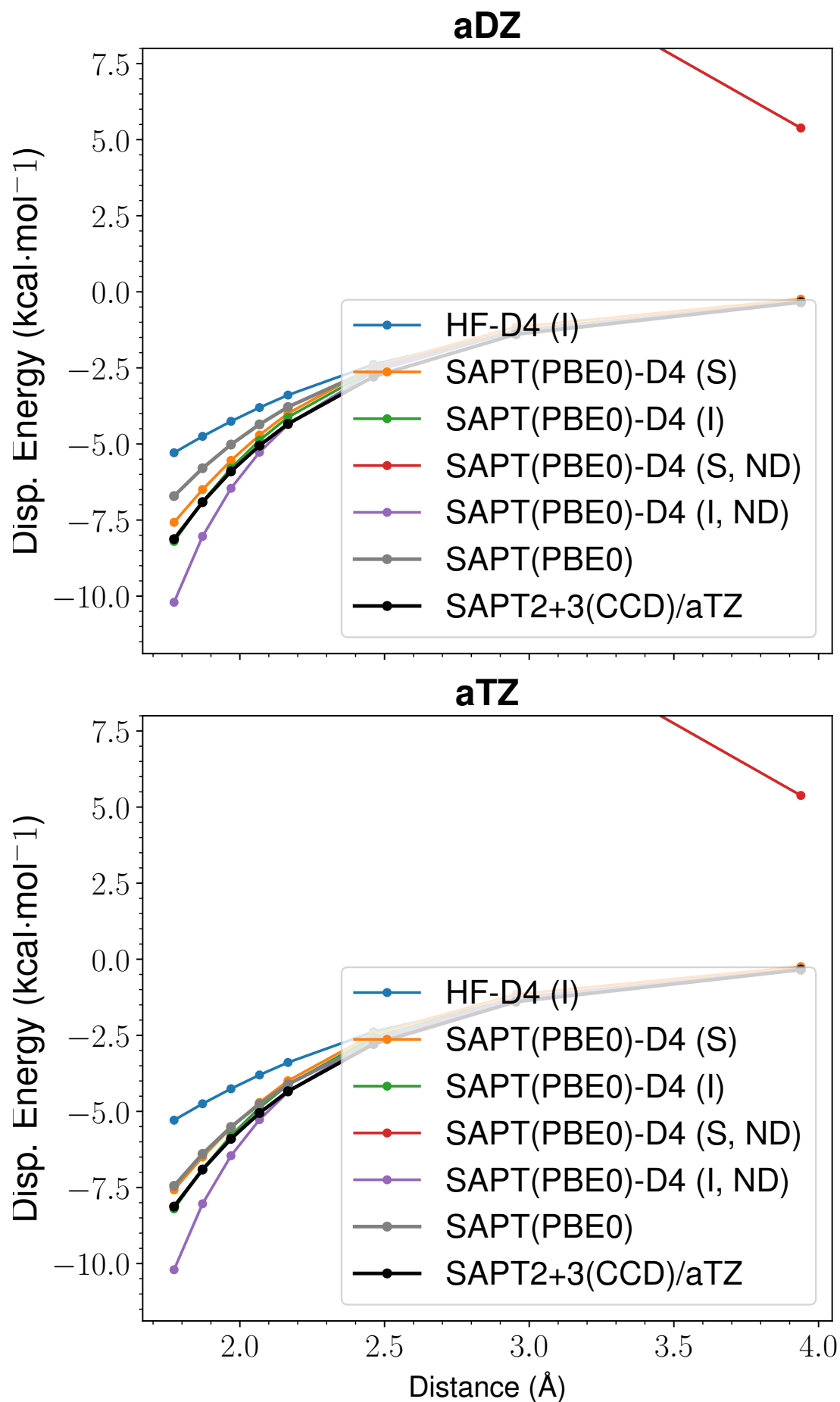
Figure 36: LoS Dispersion Curves for s66x8 15_Peptide-Peptide
