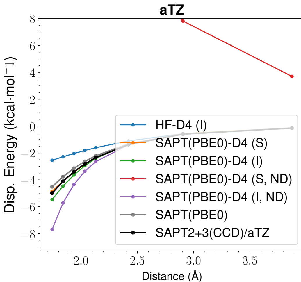
Figure 50: LoS Dispersion Curves for s66x8 05_MeOH-MeOH
