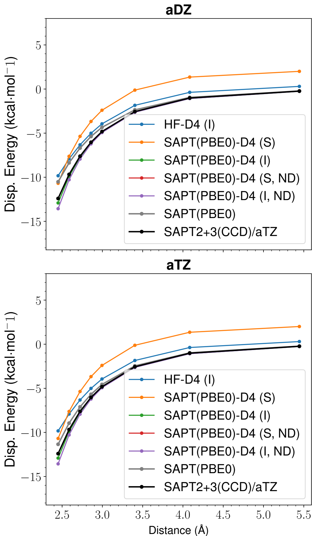
Figure 33: LoS Dispersion Curves for s66x8 42_Uracil-Cyclopentane
