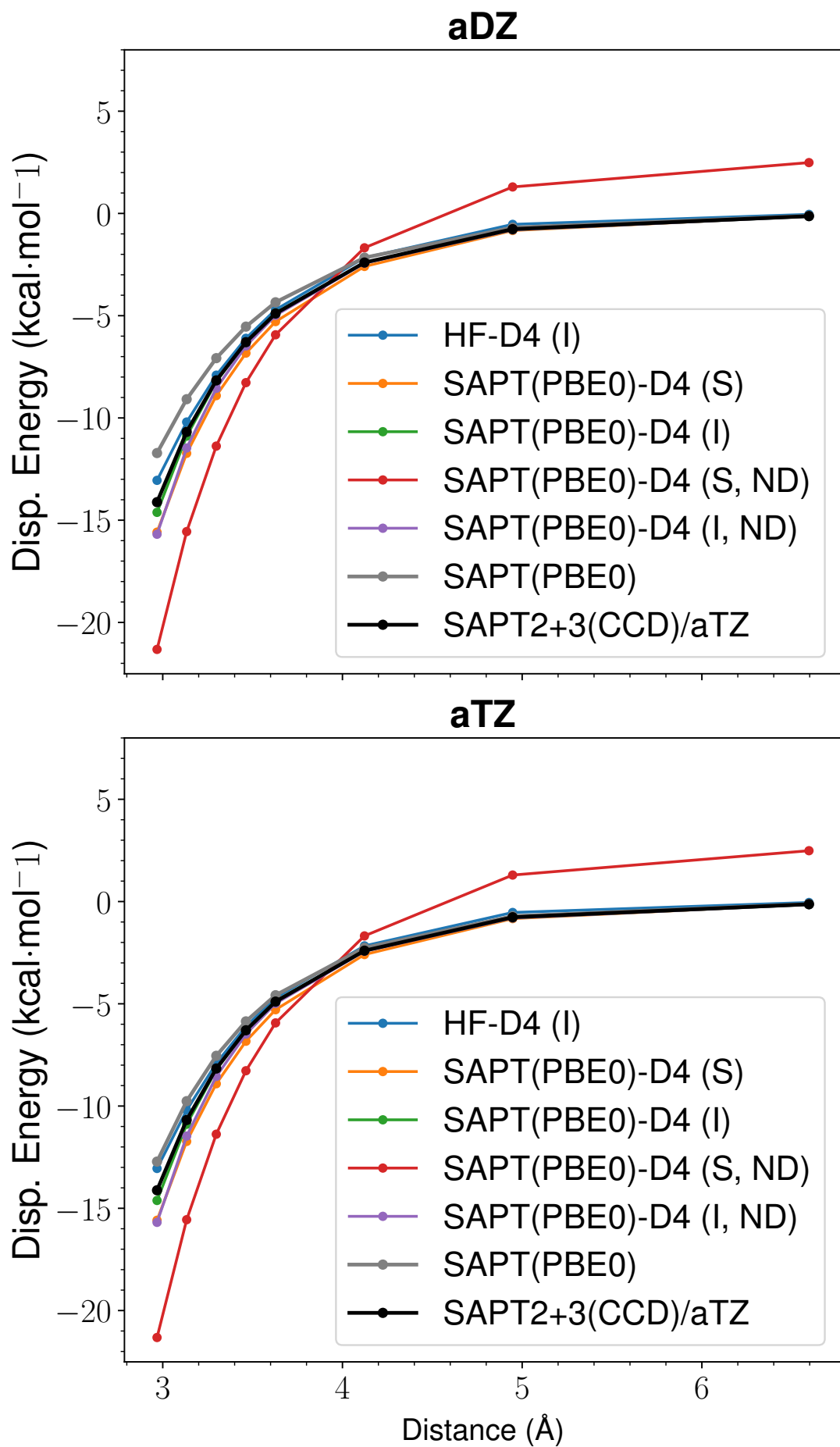
Figure 1: LoS Dispersion Curves for s66x8 27_Benzene-Pyridine
