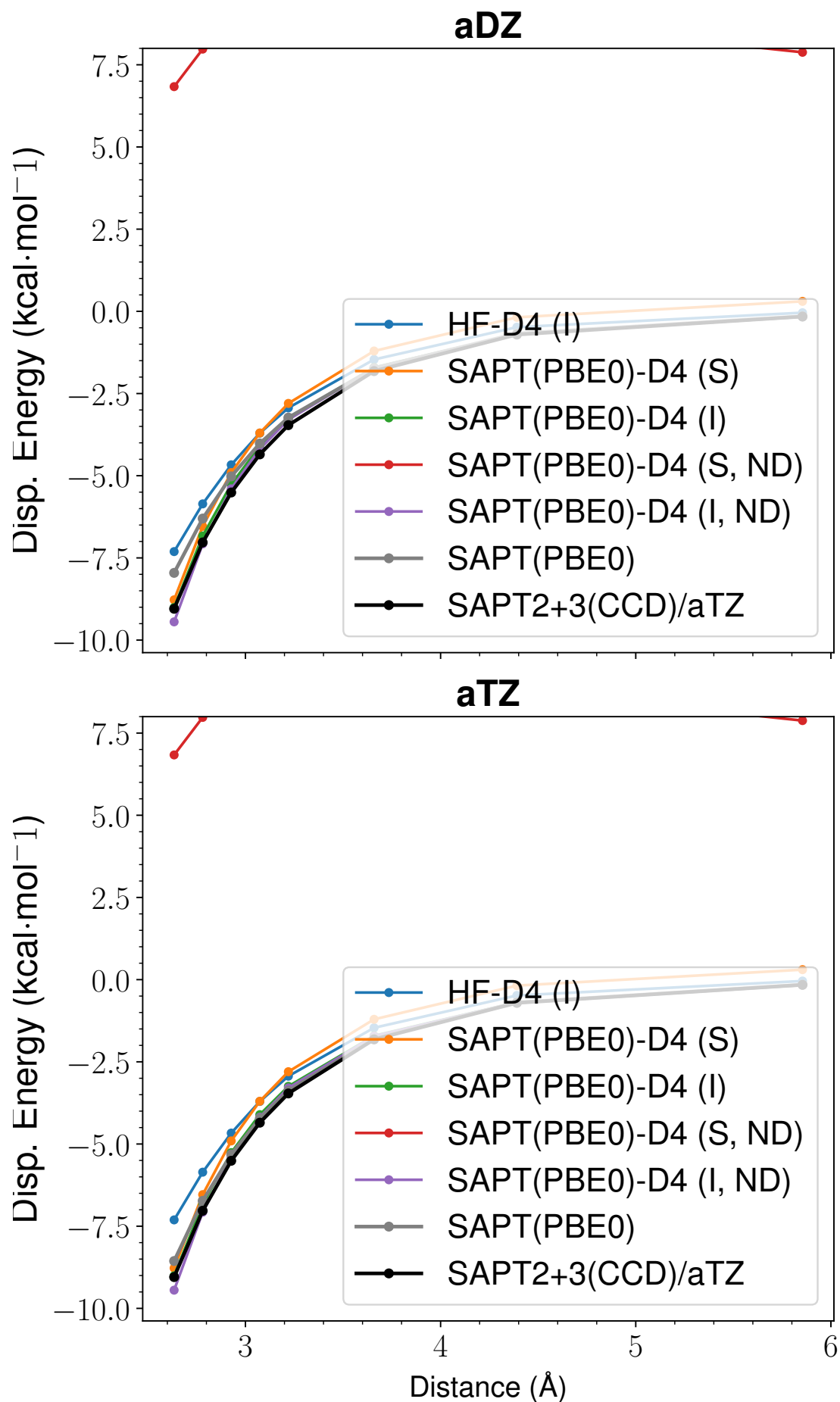
Figure 42: LoS Dispersion Curves for s66x8 40_Benzene-Neopentane
