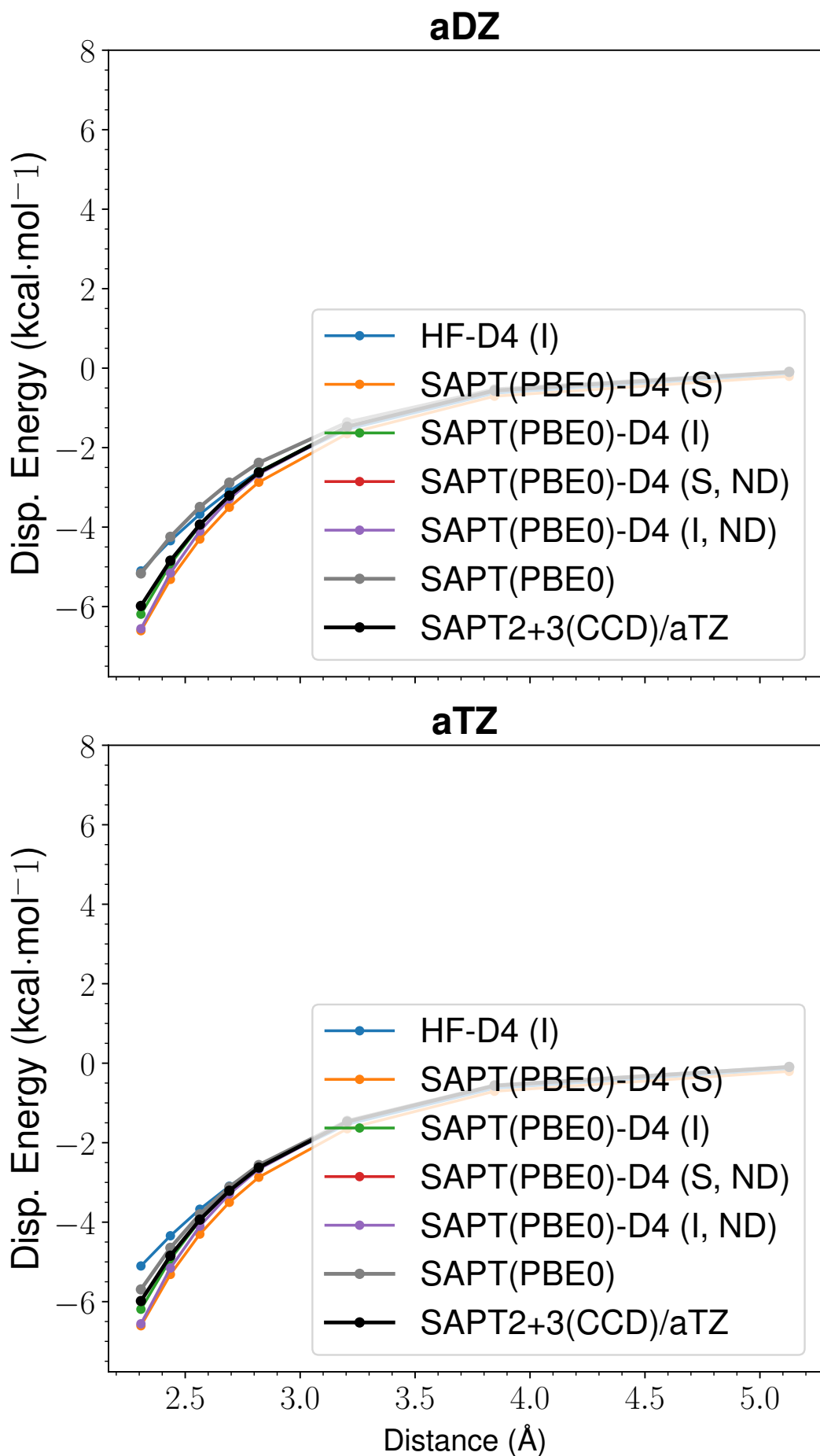
Figure 45: LoS Dispersion Curves for s66x8 64.Peptide-Ethene
