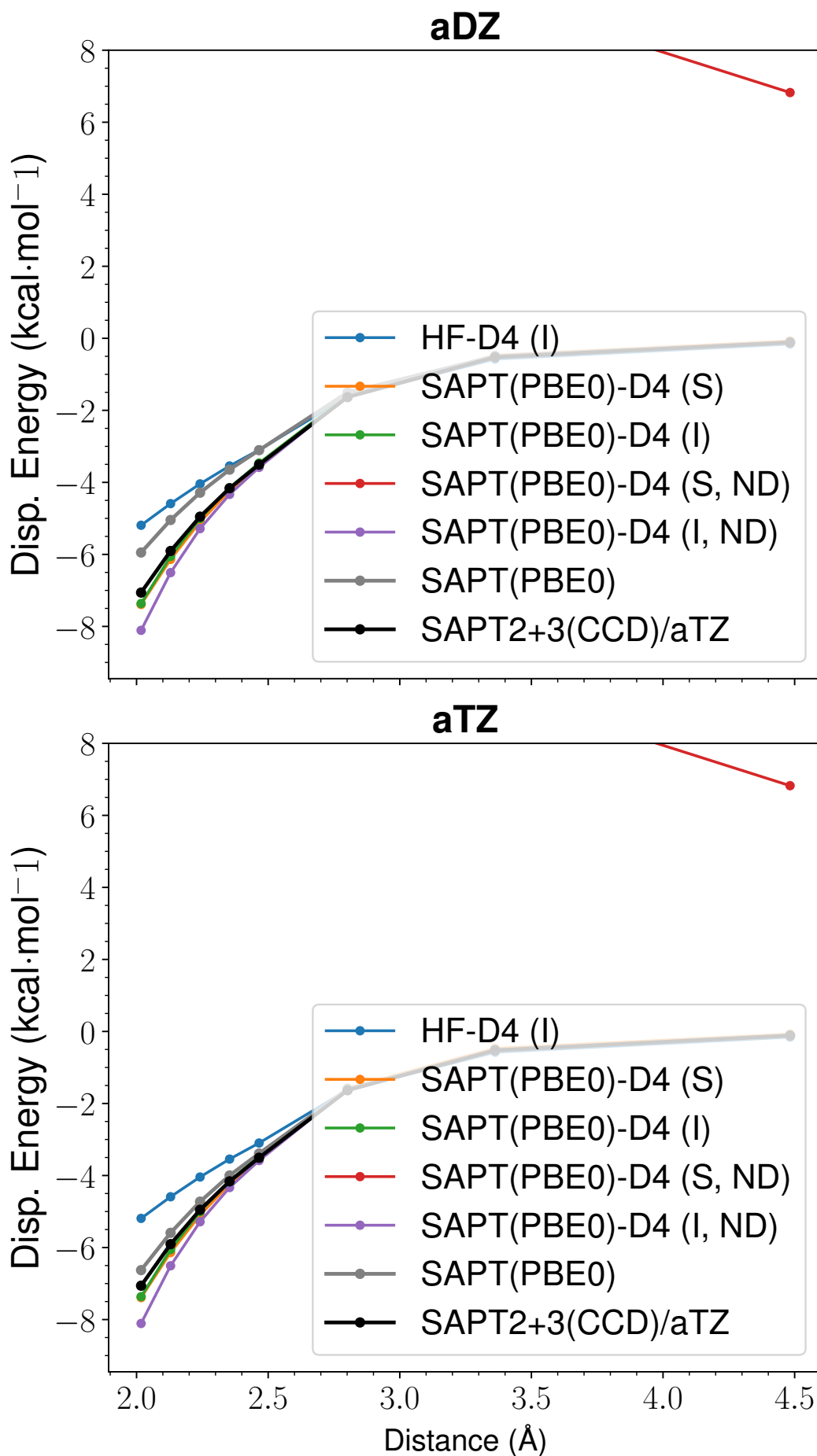
Figure 20: LoS Dispersion Curves for s66x8 11_MeNH2-Peptide
