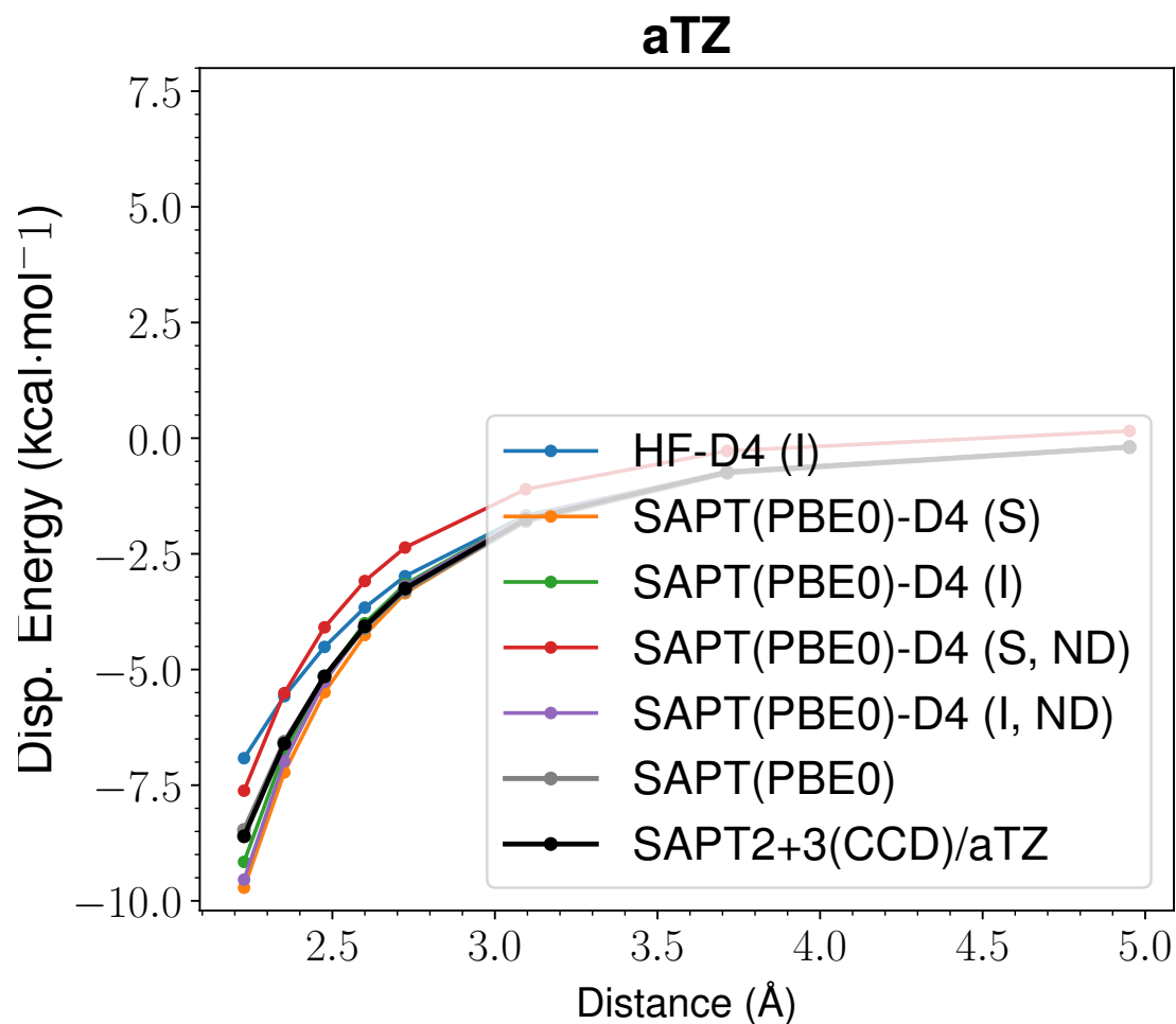
Figure 30: LoS Dispersion Curves for s66x8 35_Neopentane-Pentane
