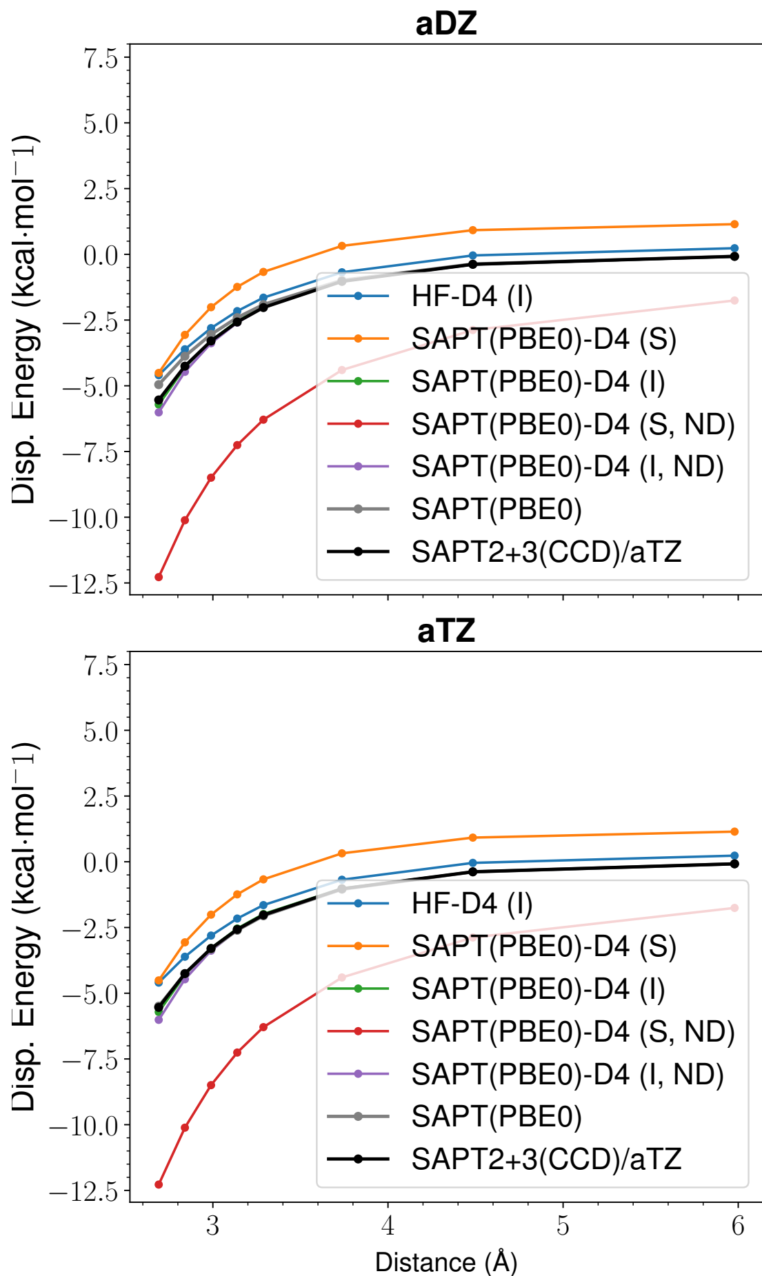
Figure 10: LoS Dispersion Curves for s66x8 45_Ethyne-Pentane
