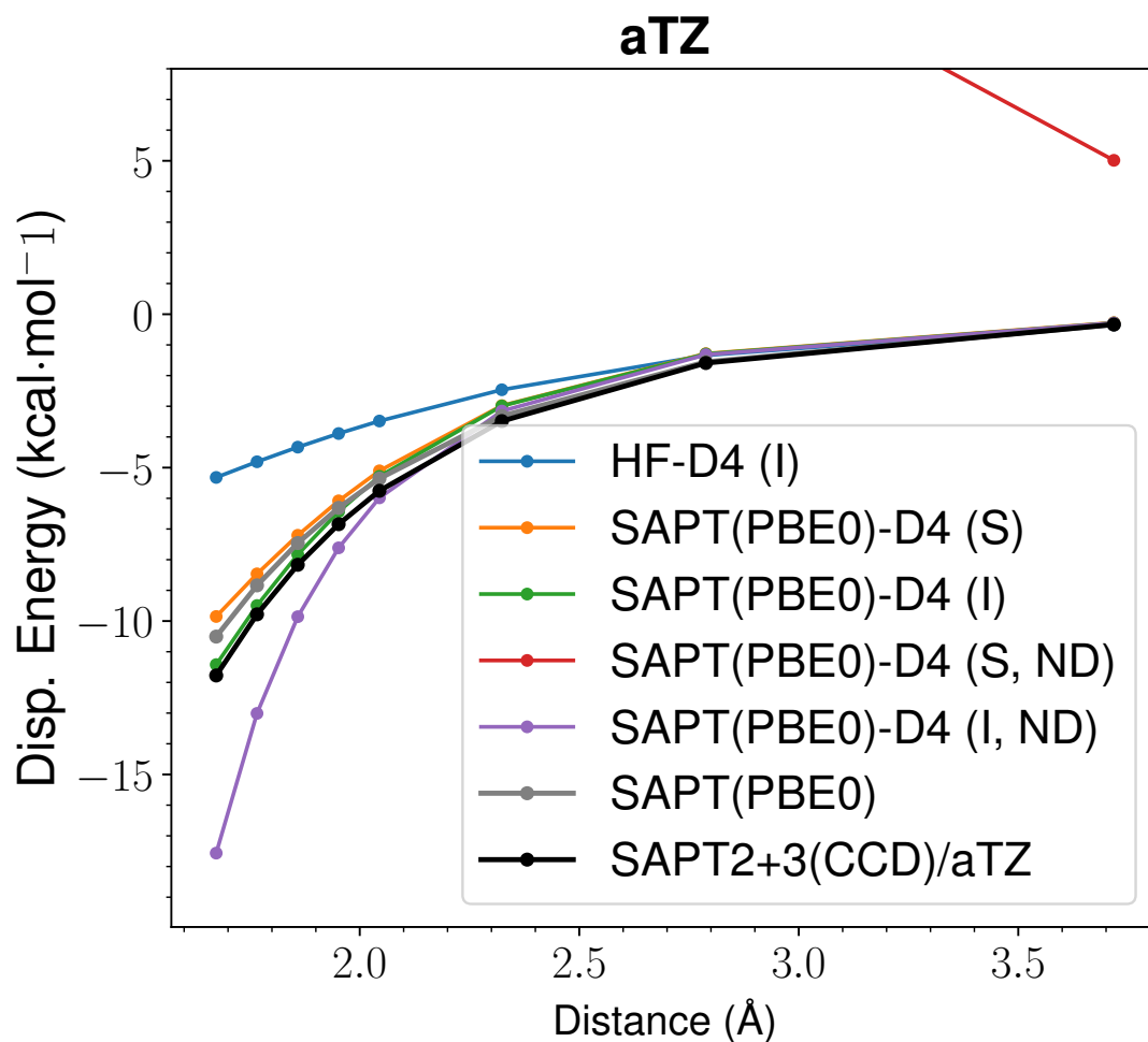
Figure 43: LoS Dispersion Curves for s66x8 21_AcNH2-AcNH2
