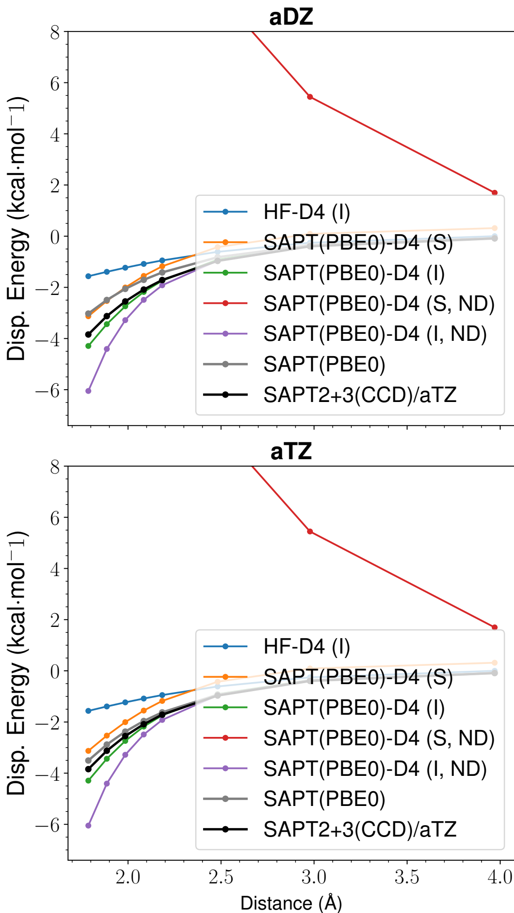
Figure 44: LoS Dispersion Curves for s66x8 08_MeOH-Water
