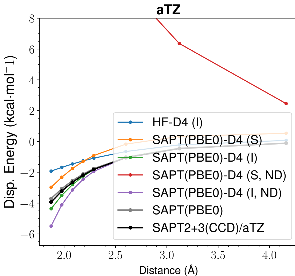
Figure 51: LoS Dispersion Curves for s66x8 16_Peptide-Water
