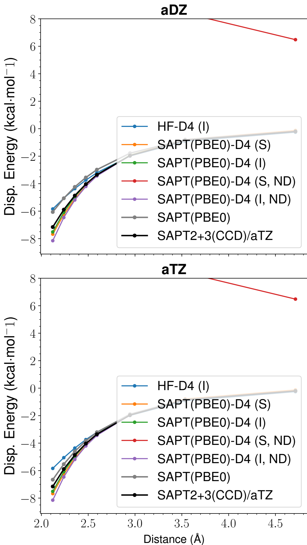
Figure 22: LoS Dispersion Curves for s66x8 66_MeNH2-Pyridine
