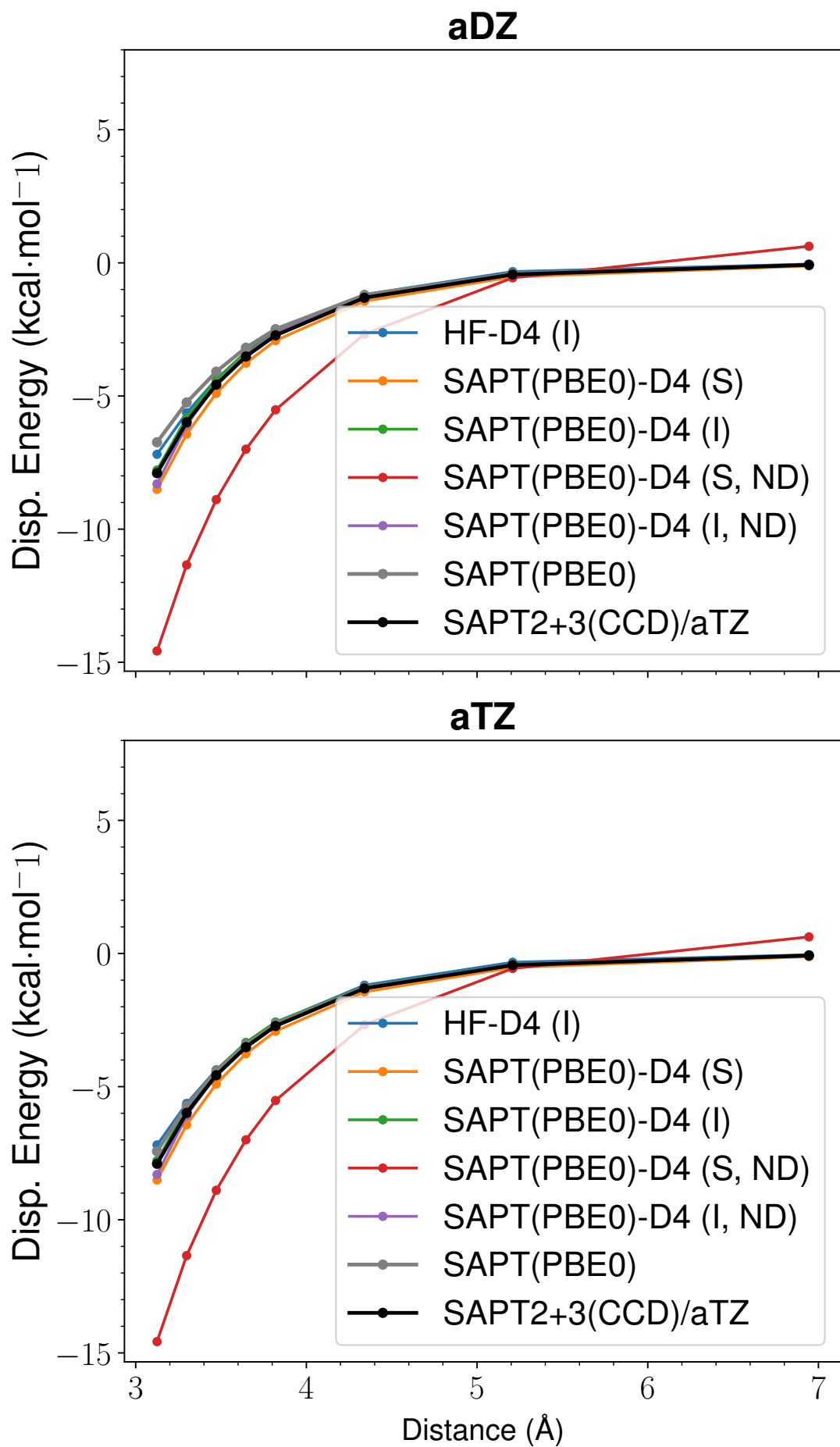
Figure 3: LoS Dispersion Curves for s66x8 30_Benzene-Ethene
