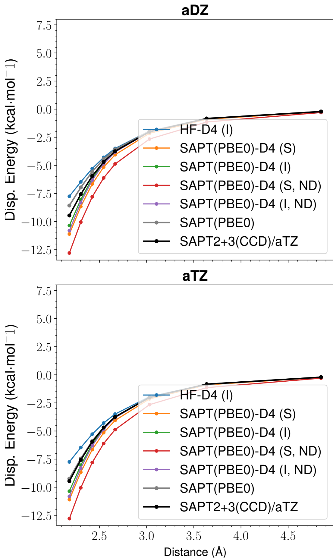
Figure 19: LoS Dispersion Curves for s66x8 38_Cyclopentane-Cyclopentane
