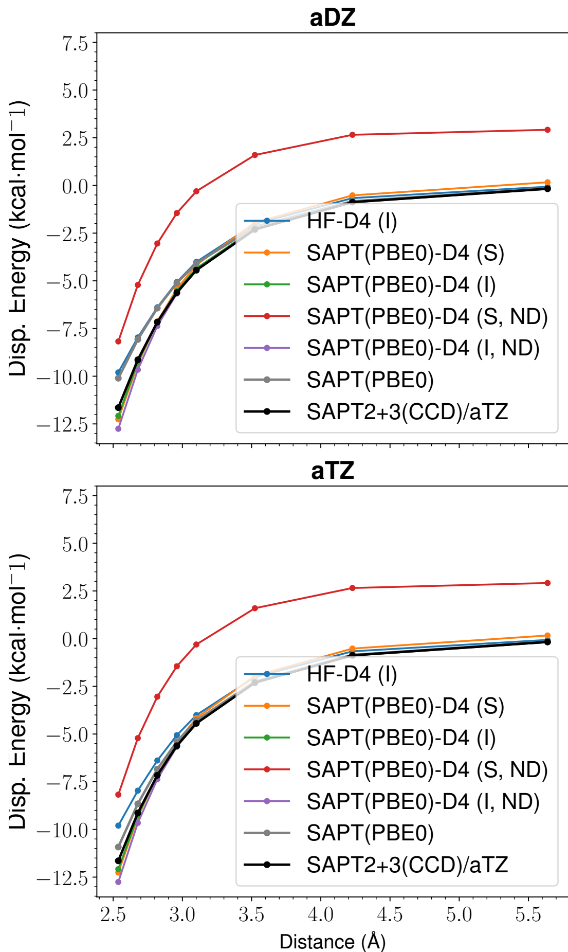
Figure 49: LoS Dispersion Curves for s66x8 39_Benzene-Cyclopentane
