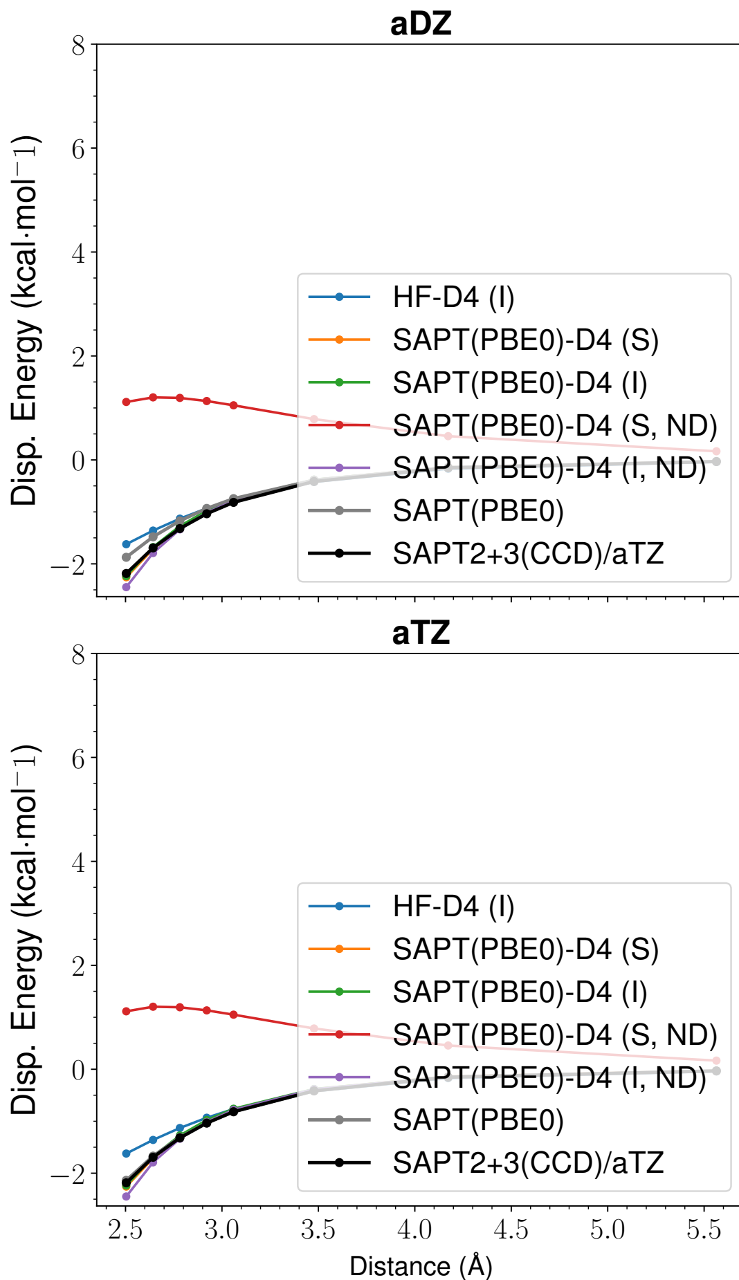
Figure 65: LoS Dispersion Curves for s66x8 51_Ethyne-Ethyne
