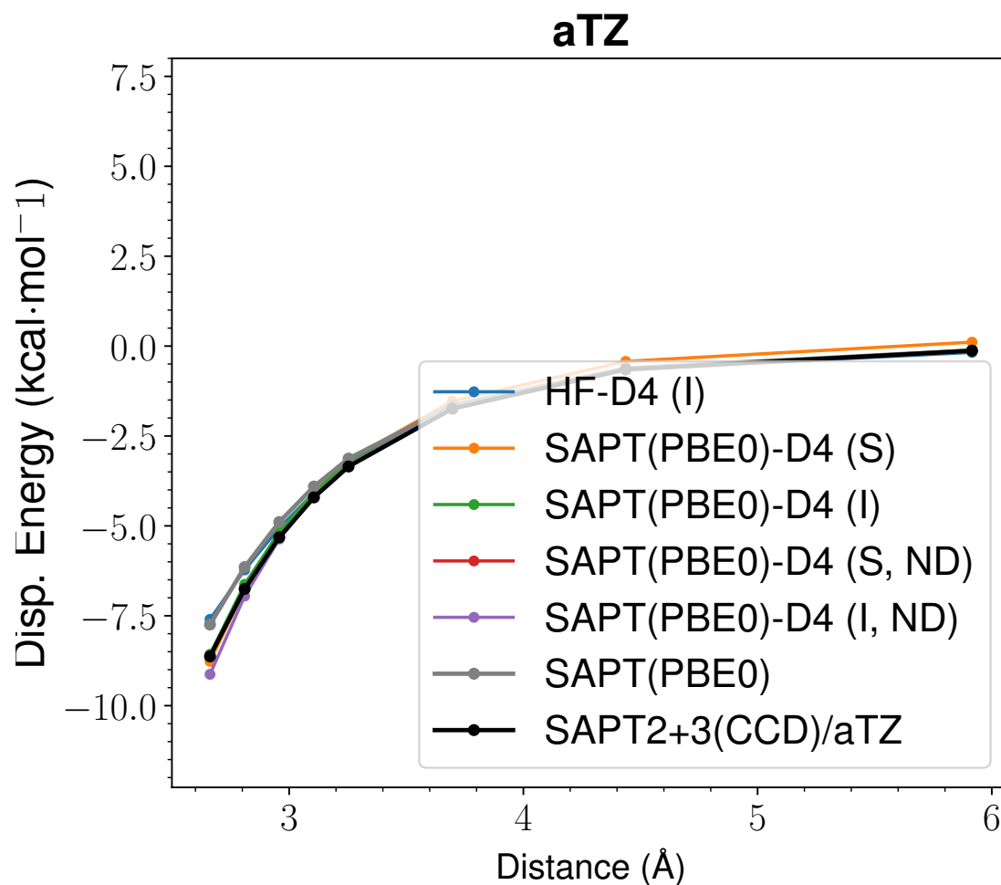
Figure 26: LoS Dispersion Curves for s66x8 31_Uracil-Ethene
