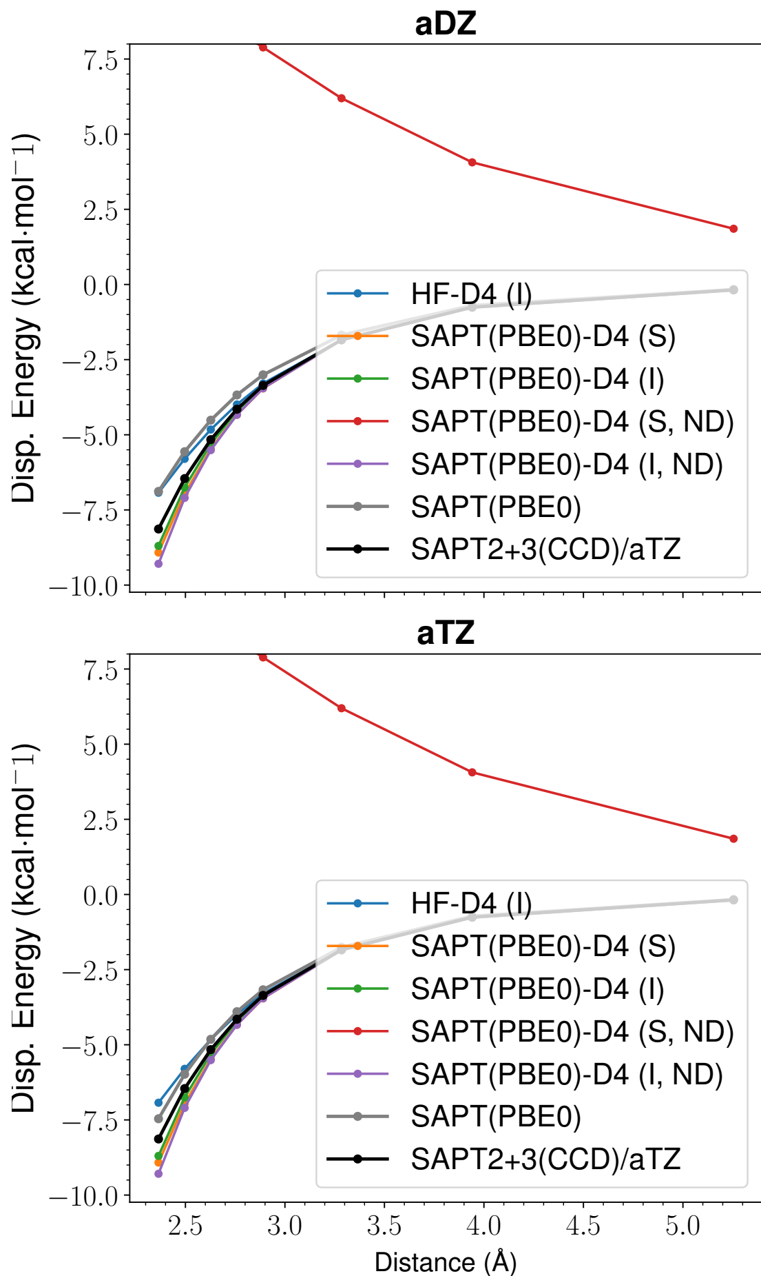
Figure 40: LoS Dispersion Curves for s66x8 48_Pyridine-Pyridine
