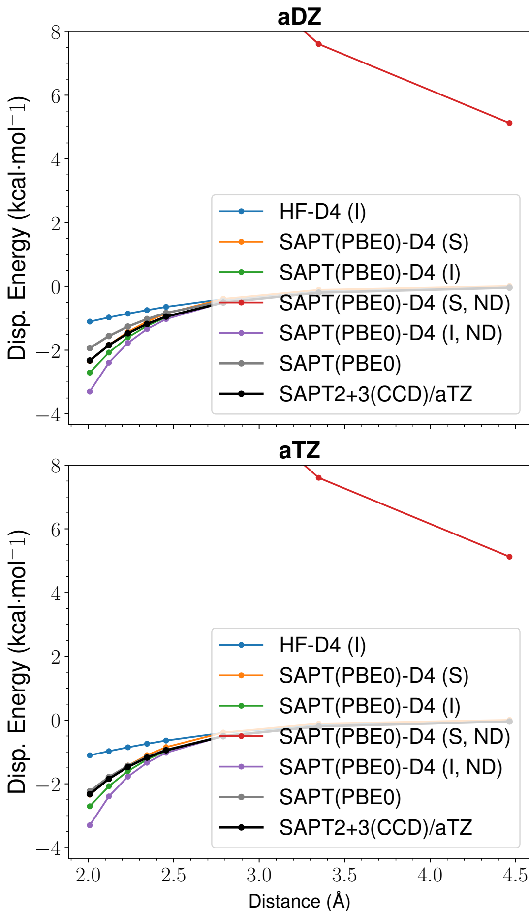
Figure 27: LoS Dispersion Curves for s66x8 59_Ethyne-Water
