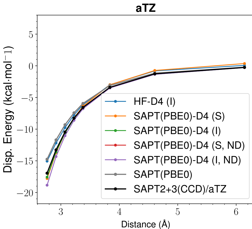
Figure 5: LoS Dispersion Curves for s66x8 28_Benzene-Uracil
