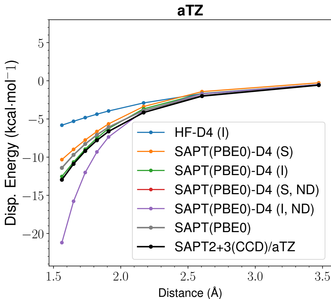
Figure 52: LoS Dispersion Curves for s66x8 23_AcNH2-Uracil
