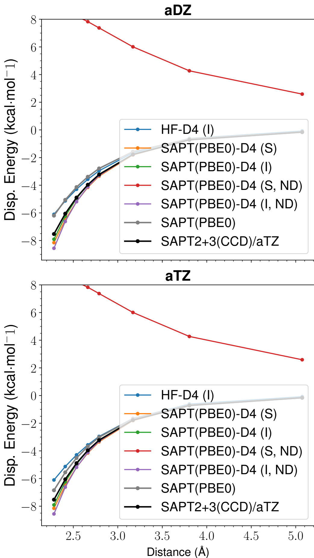
Figure 9: LoS Dispersion Curves for s66x8 55_Benzene-MeOH
