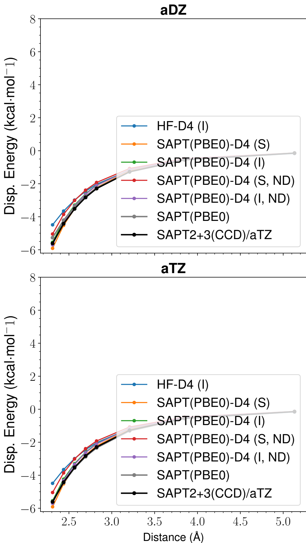
Figure 56: LoS Dispersion Curves for s66x8 36_Neopentane-Neopentane
