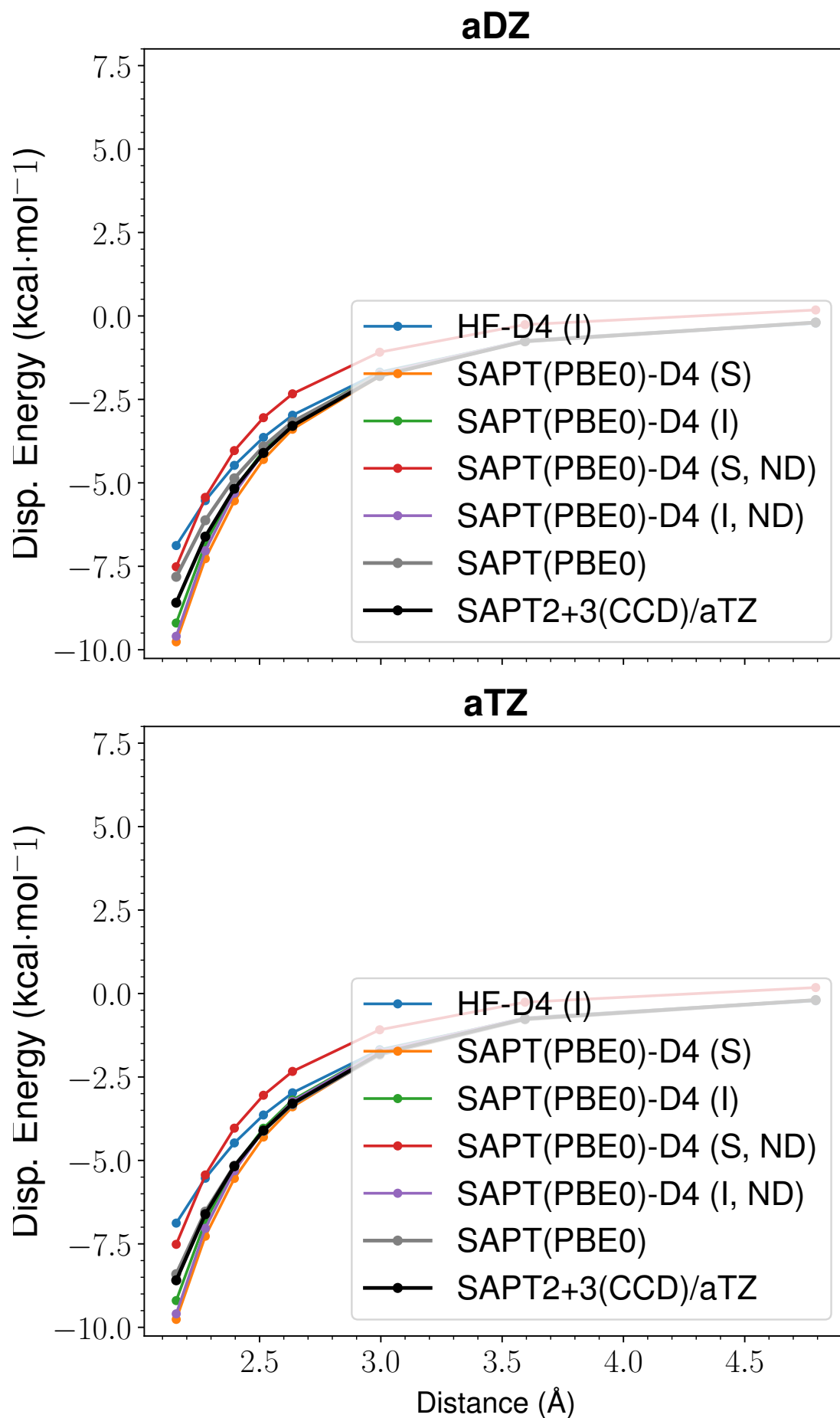
Figure 66: LoS Dispersion Curves for s66x8 37_Cyclopentane-Neopentane
