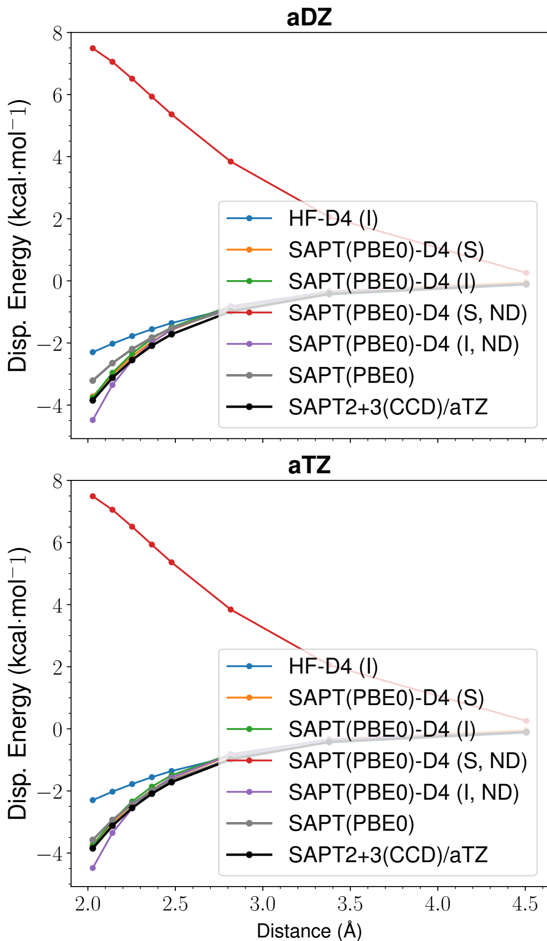
Figure 23: LoS Dispersion Curves for s66x8 65_Pyridine-Ethyne
