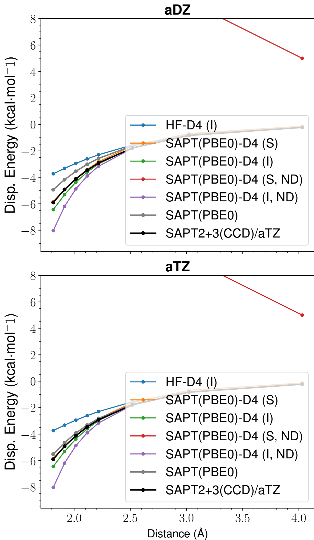
Figure 47: LoS Dispersion Curves for s66x8 13_Peptide-MeOH
