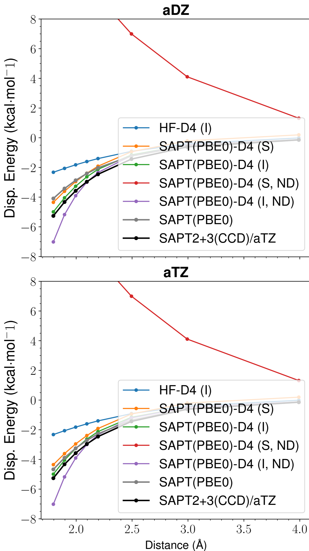
Figure 55: LoS Dispersion Curves for s66x8 18_Water-Pyridine
