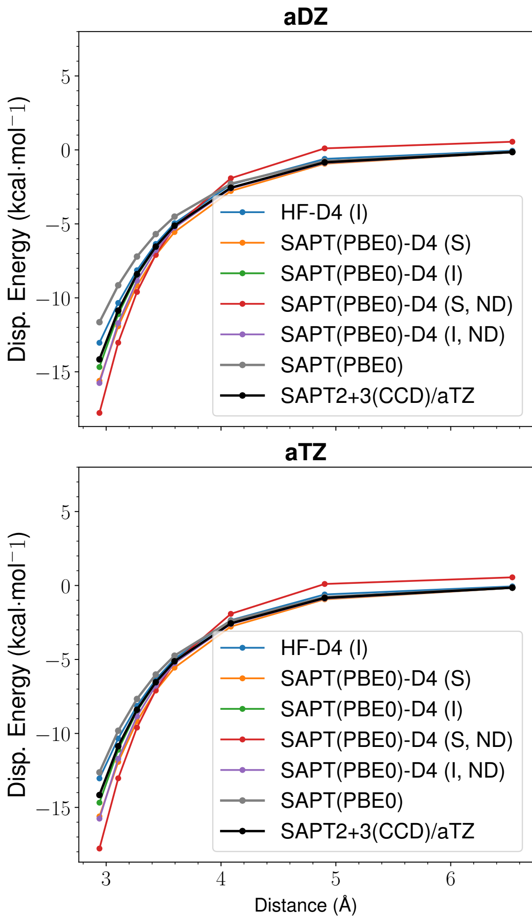
Figure 54: LoS Dispersion Curves for s66x8 25_Pyridine-Pyridine
