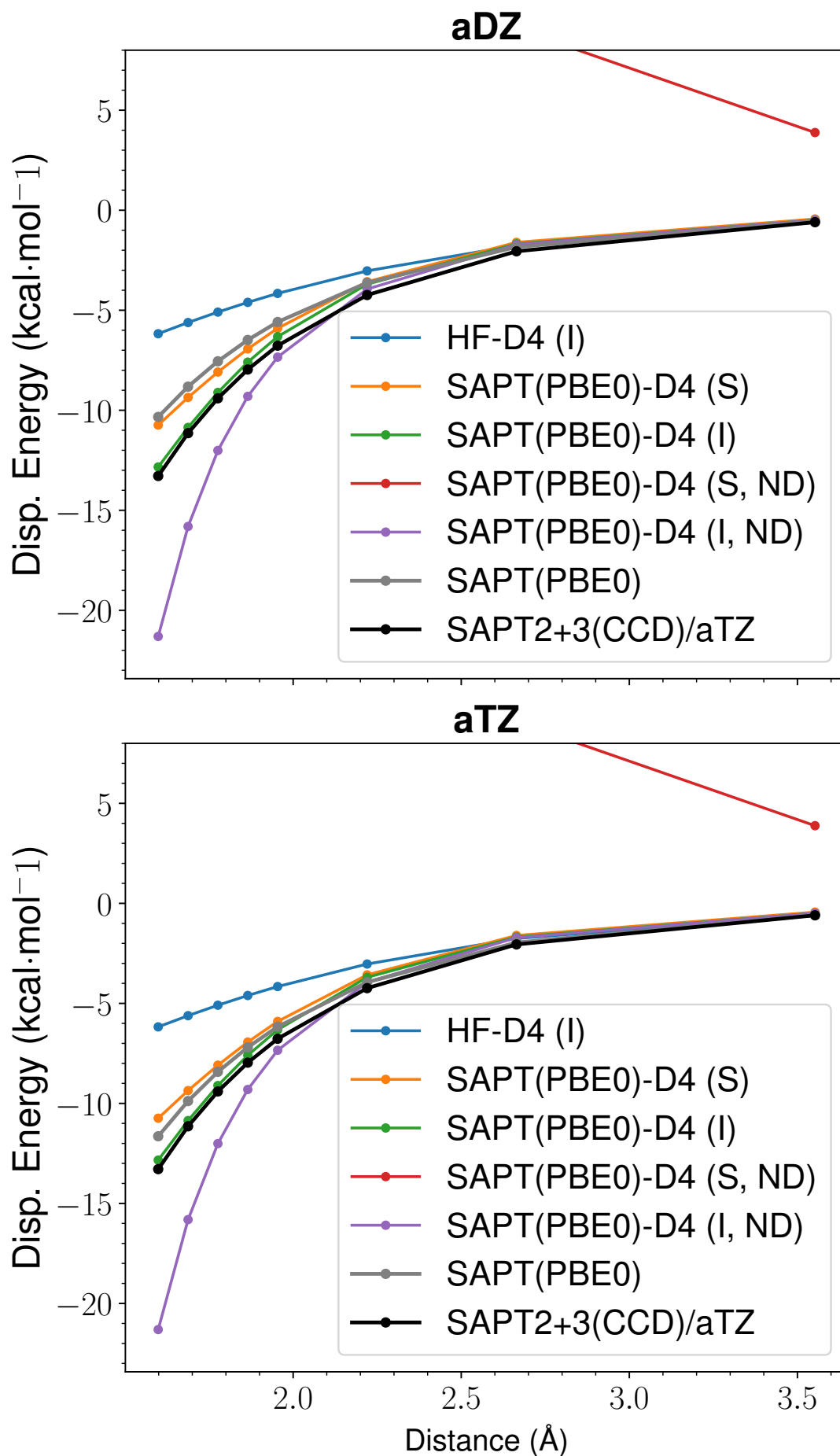
Figure 25: LoS Dispersion Curves for s66x8 17_Uracil-Uracil
