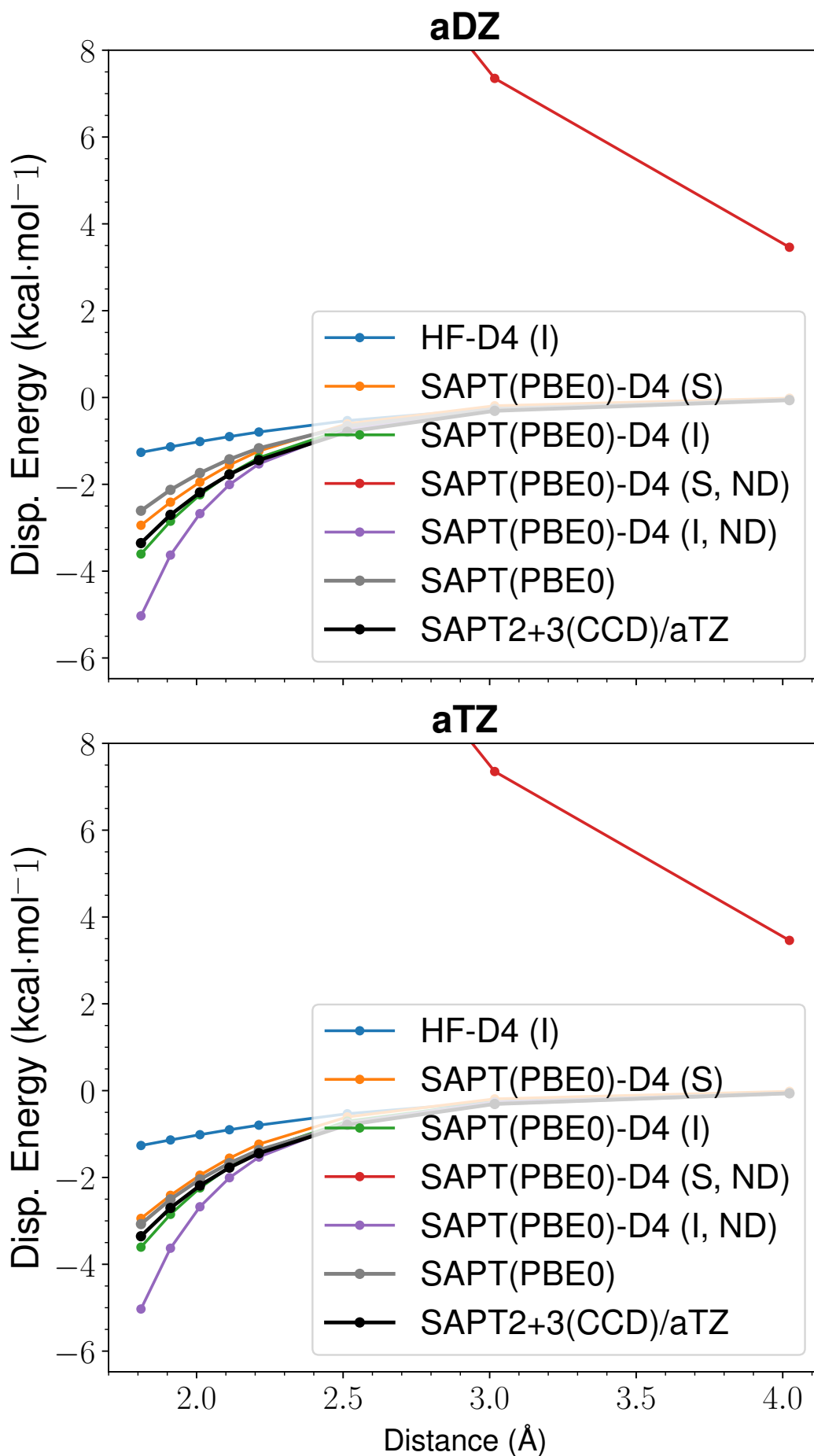
Figure 2: LoS Dispersion Curves for s66x8 01_Water-Water
