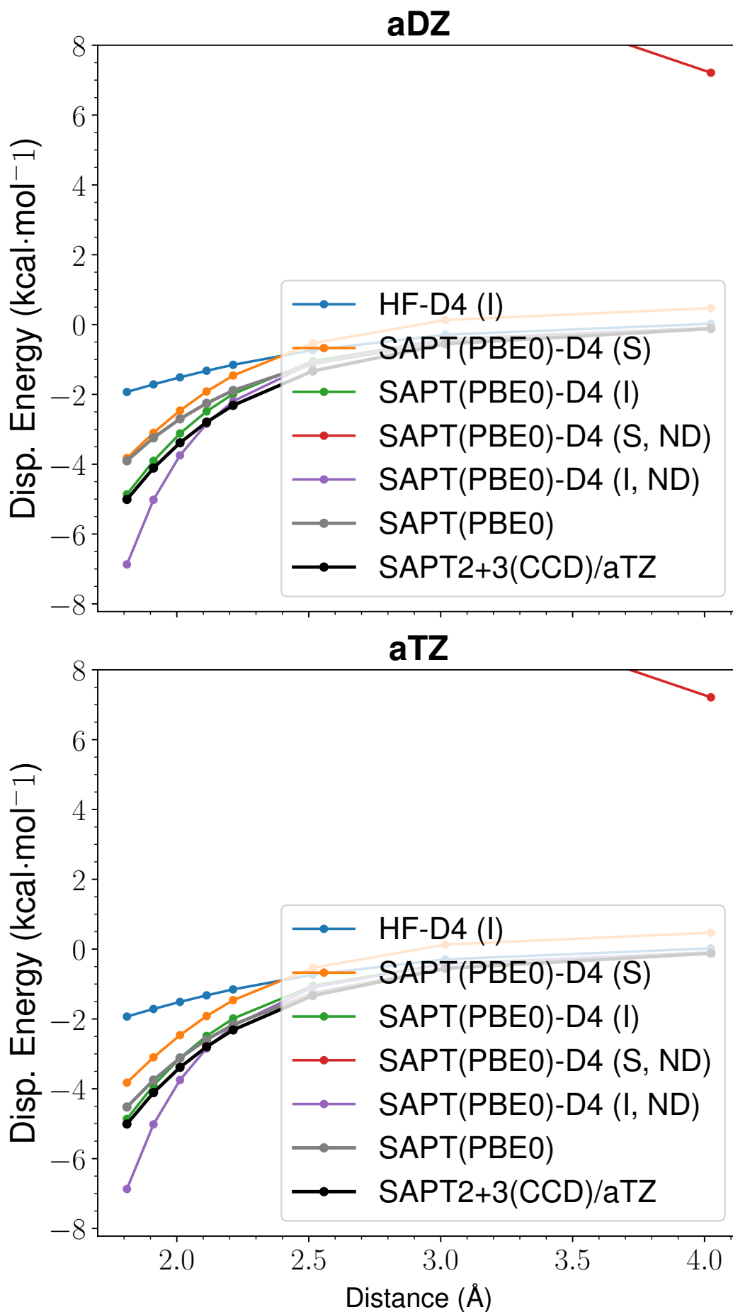
Figure 48: LoS Dispersion Curves for s66x8 03_Water-MeNH2
