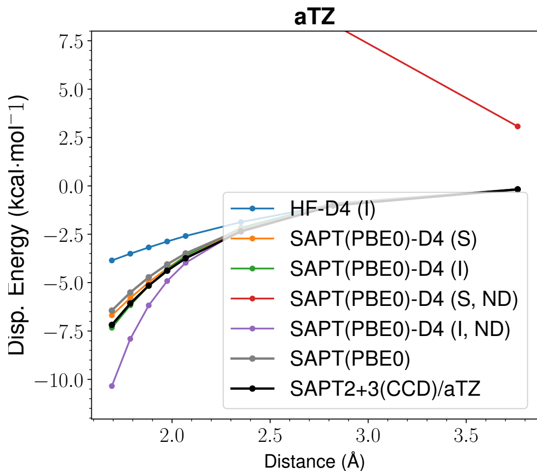
Figure 62: LoS Dispersion Curves for s66x8 07_MeOH-Peptide
