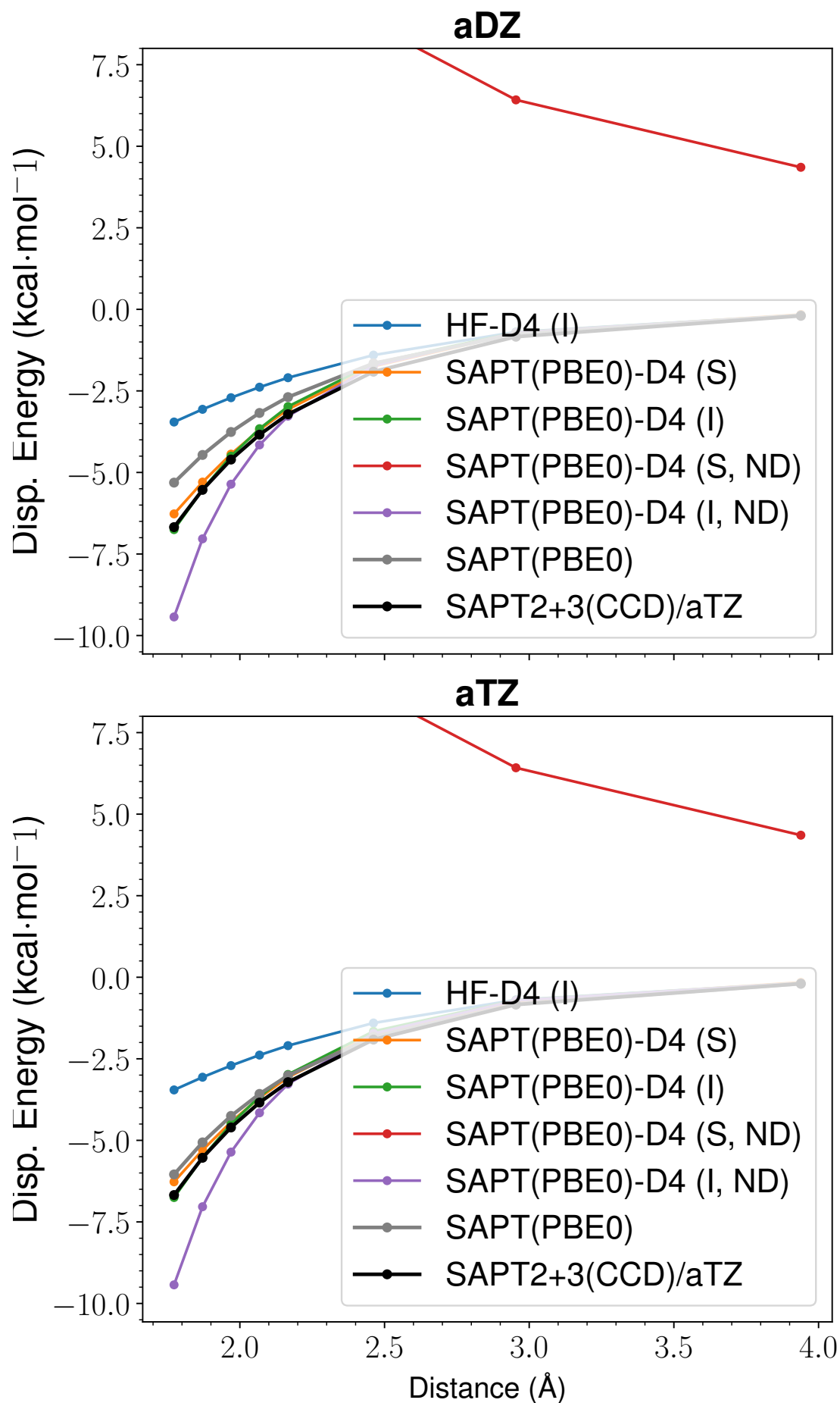
Figure 46: LoS Dispersion Curves for s66x8 06_MeOH-MeNH2
