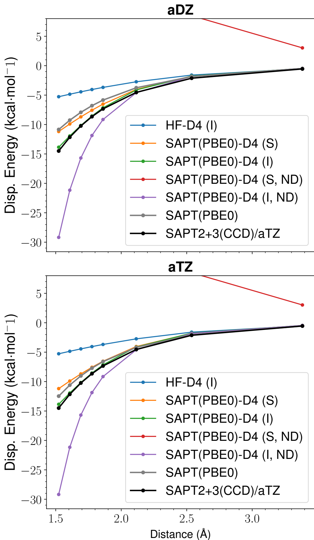
Figure 37: LoS Dispersion Curves for s66x8 20_AcOH-AcOH
