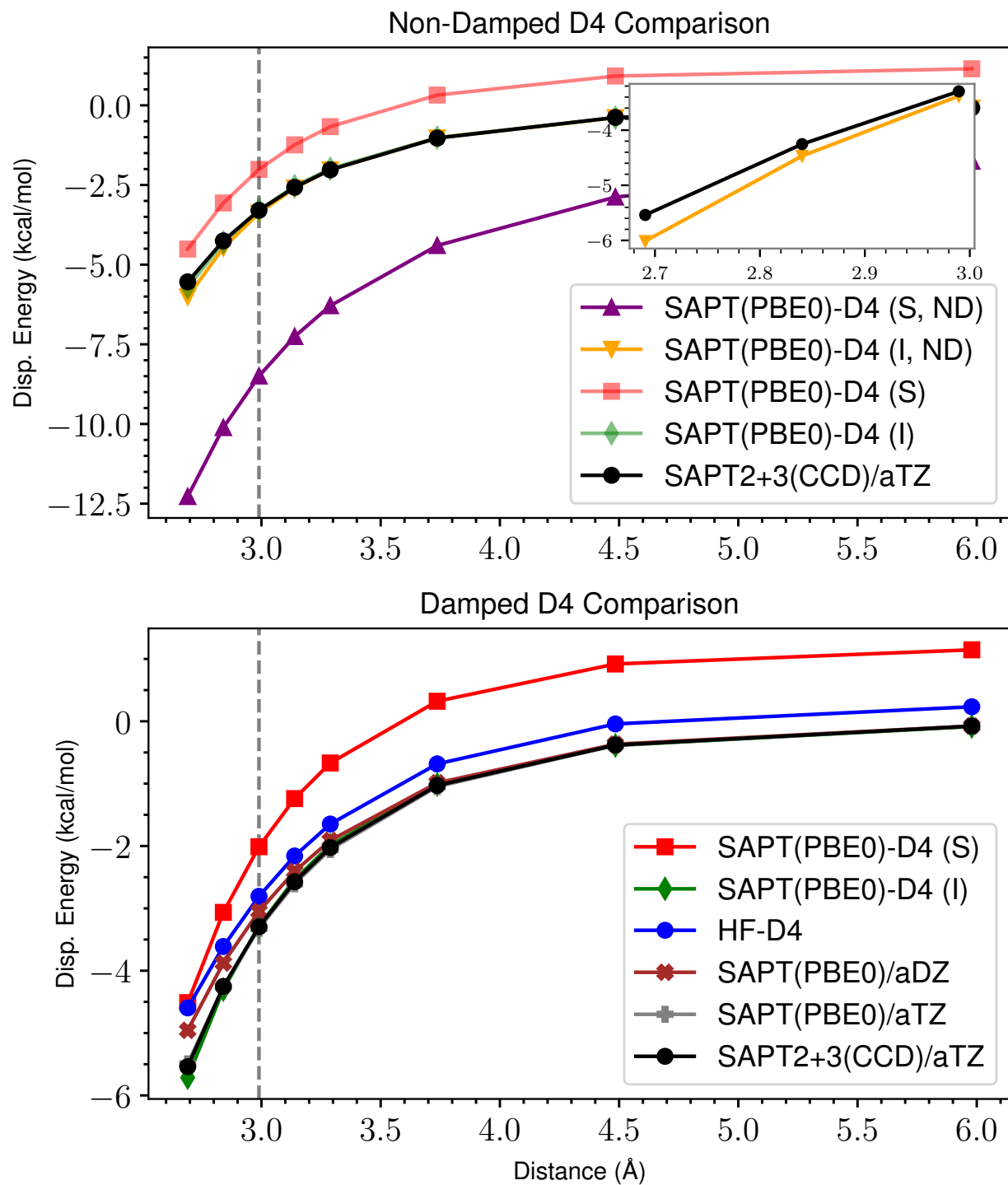
Figure 2: ND vs Damped D4 Dispersion for s66x8 45_Ethyne-Pentane
