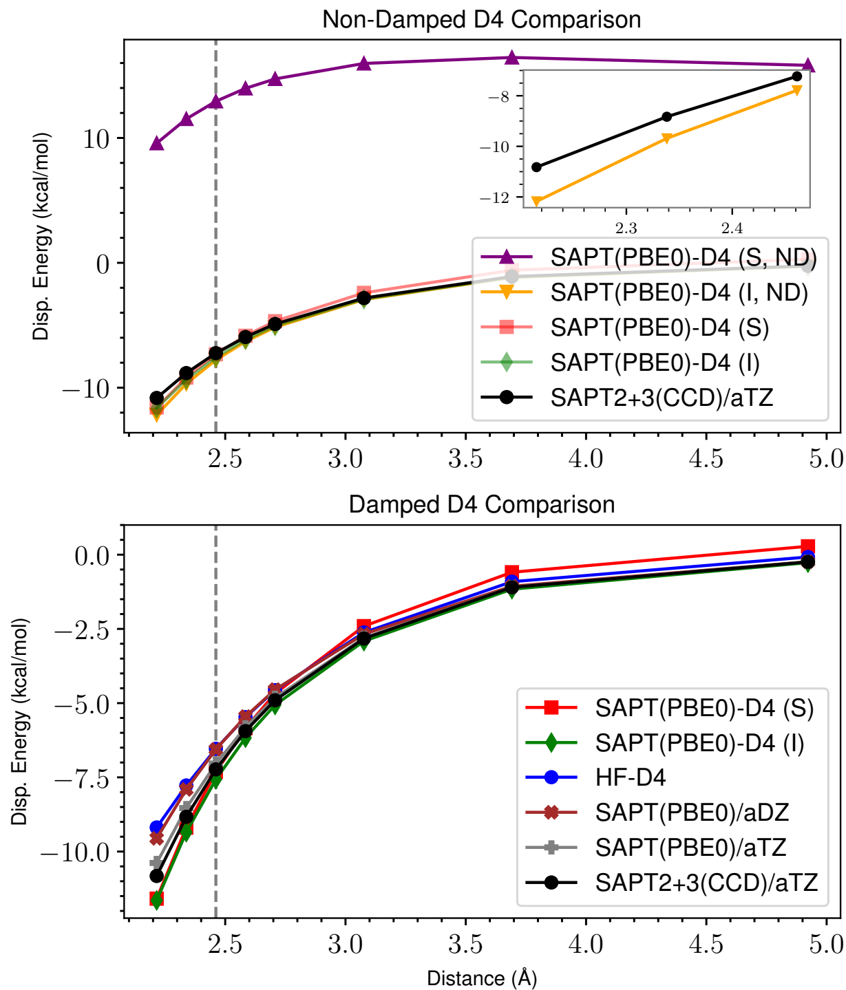
Figure 45: ND vs Damped D4 Dispersion for s66x8 46_Peptide-Pentane
