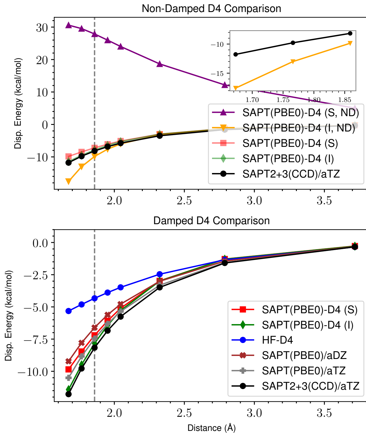
Figure 50: ND vs Damped D4 Dispersion for s66x8 21_AcNH2-AcNH2
