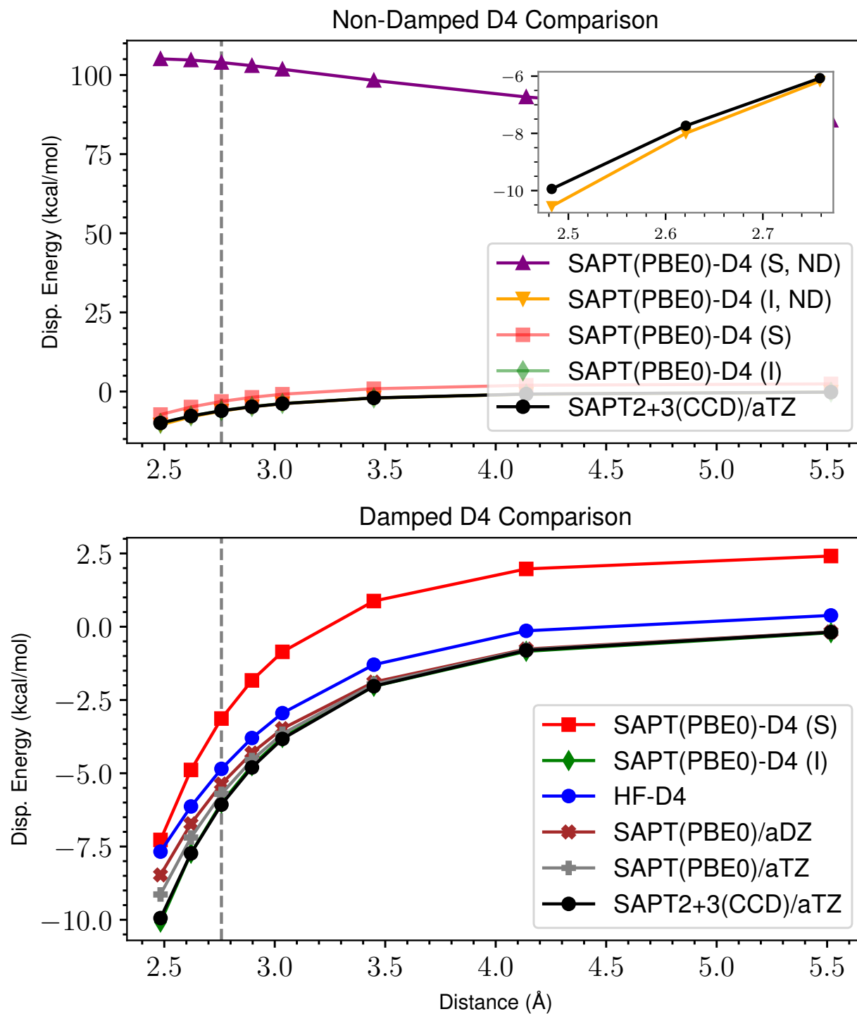
Figure 53: ND vs Damped D4 Dispersion for s66x8 43_Uracil-Neopentane
