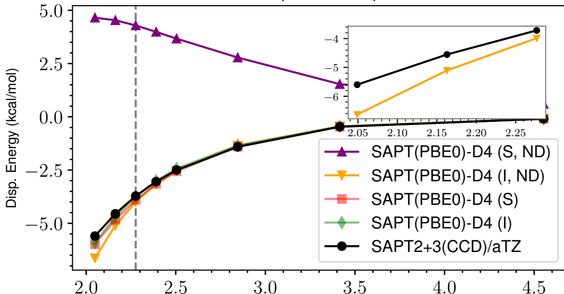
Non-Damped D4 Comparison
