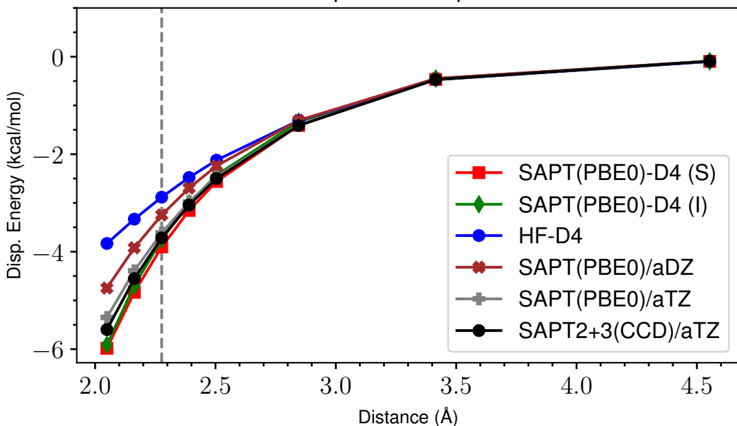
Damped D4 Comparison
