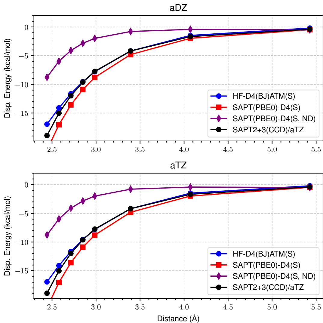
Figure 10: LoS Dispersion Curves for s66x8 26_Uracil-Uracil
