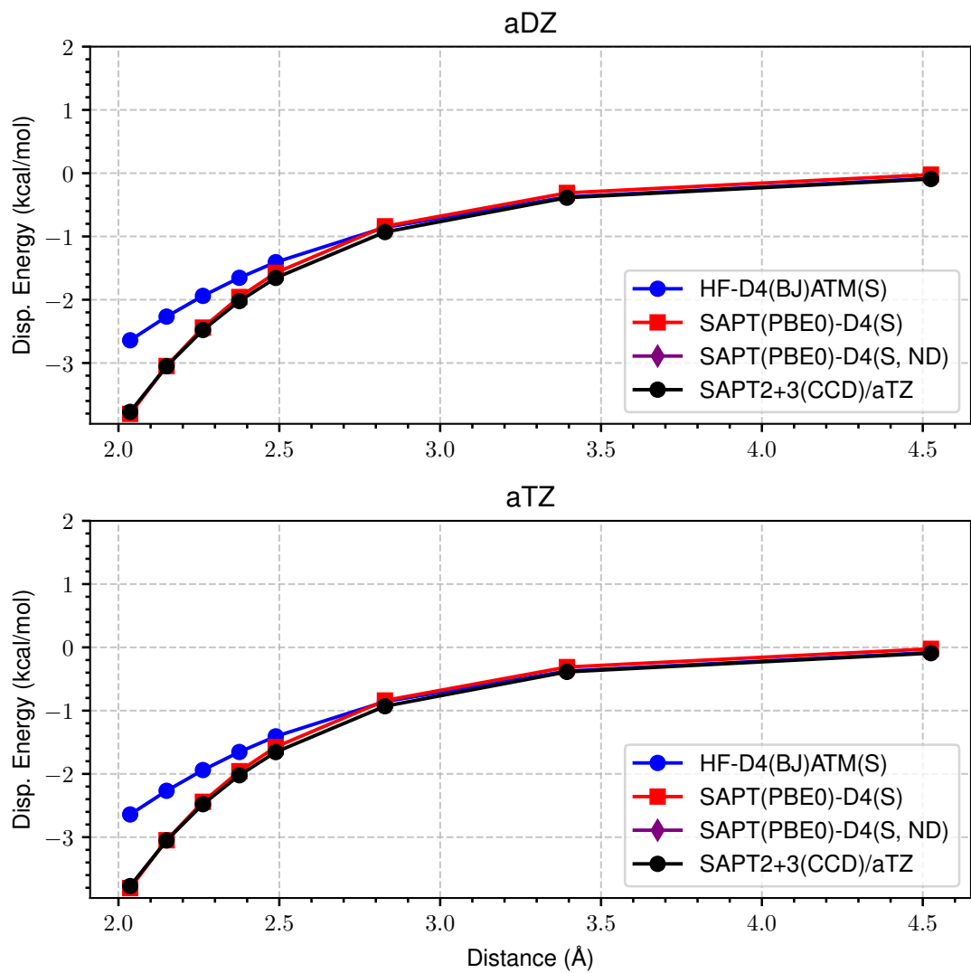
Figure 42: LoS Dispersion Curves for s66x8 09_MeNH2-MeOH
