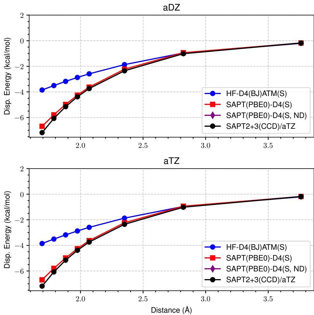
Figure 32: LoS Dispersion Curves for s66x8 07_MeOH-Peptide
