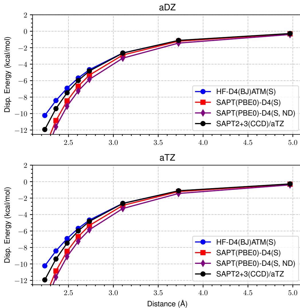
Figure 40: LoS Dispersion Curves for s66x8 34_Pentane-Pentane
