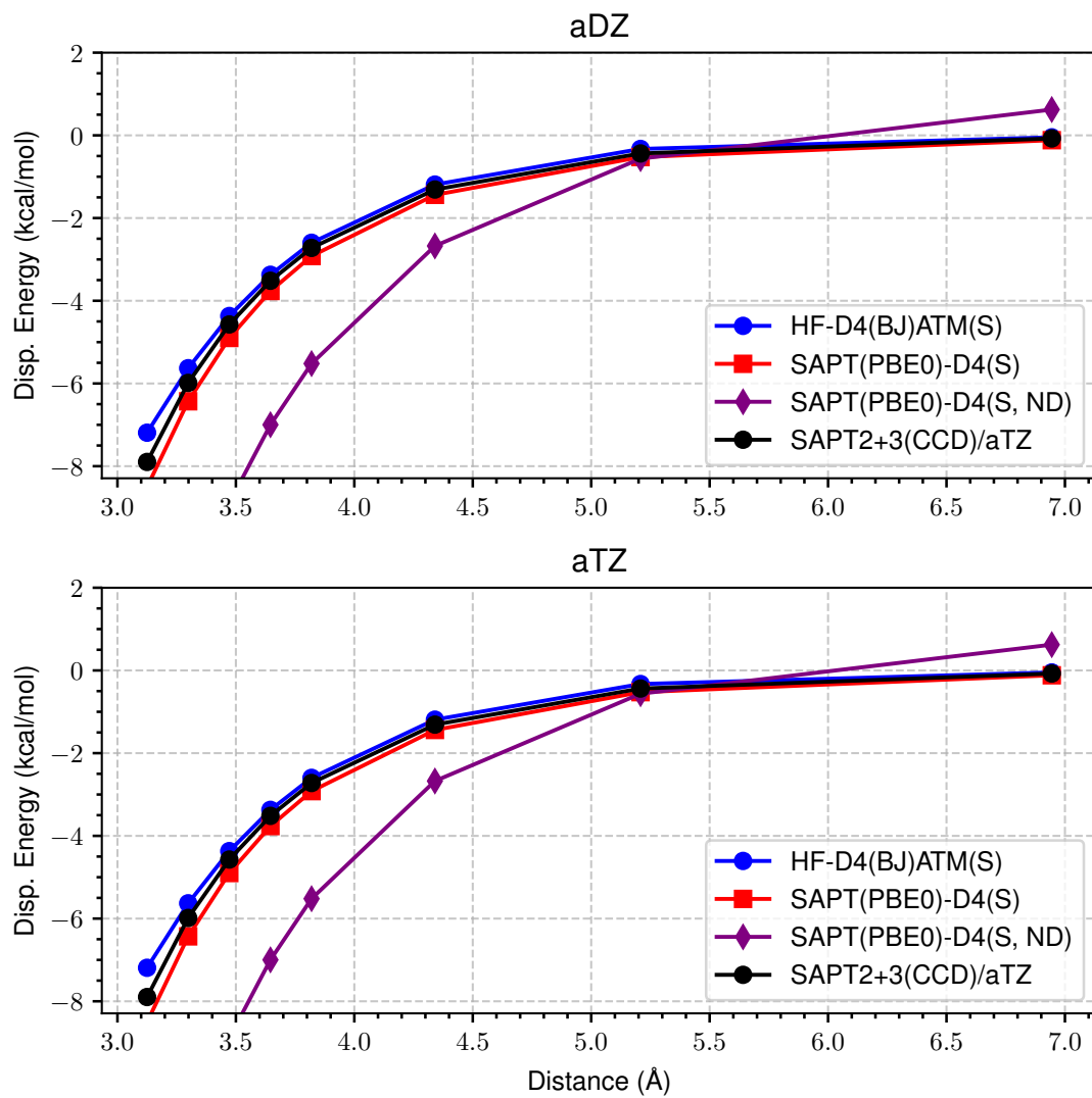
Figure 43: LoS Dispersion Curves for s66x8 30_Benzene-Ethene
