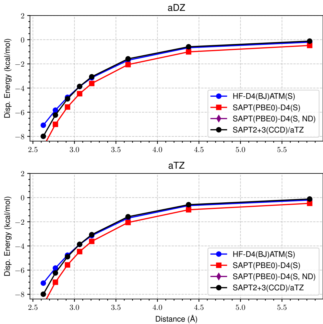
Figure 65: LoS Dispersion Curves for s66x8 32_Uracil-Ethyne
