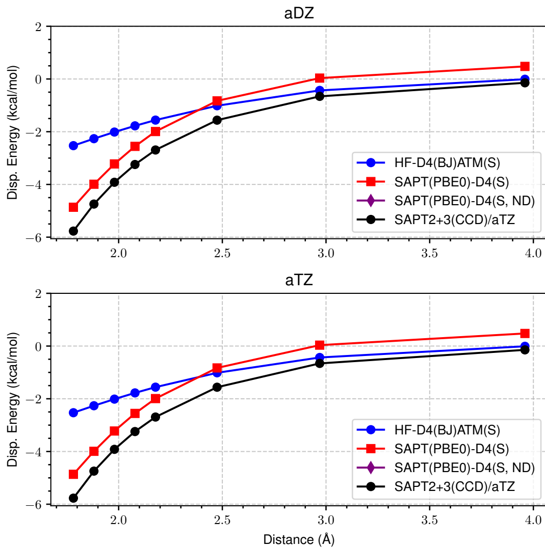
Figure 60: LoS Dispersion Curves for s66x8 12_MeNH2-Water
