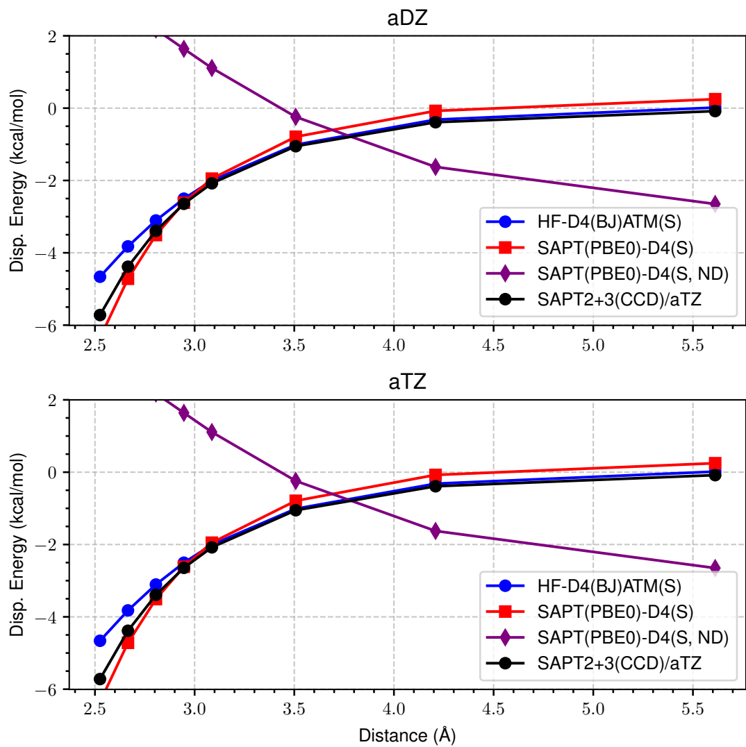
Figure 21: LoS Dispersion Curves for s66x8 50_Benzene-Ethyne
