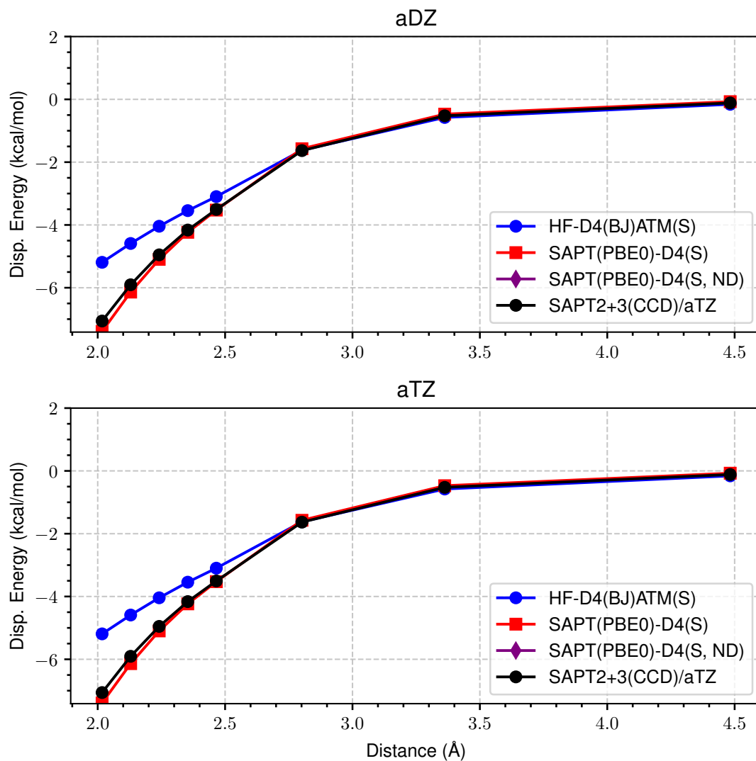
Figure 52: LoS Dispersion Curves for s66x8 11_MeNH2-Peptide
