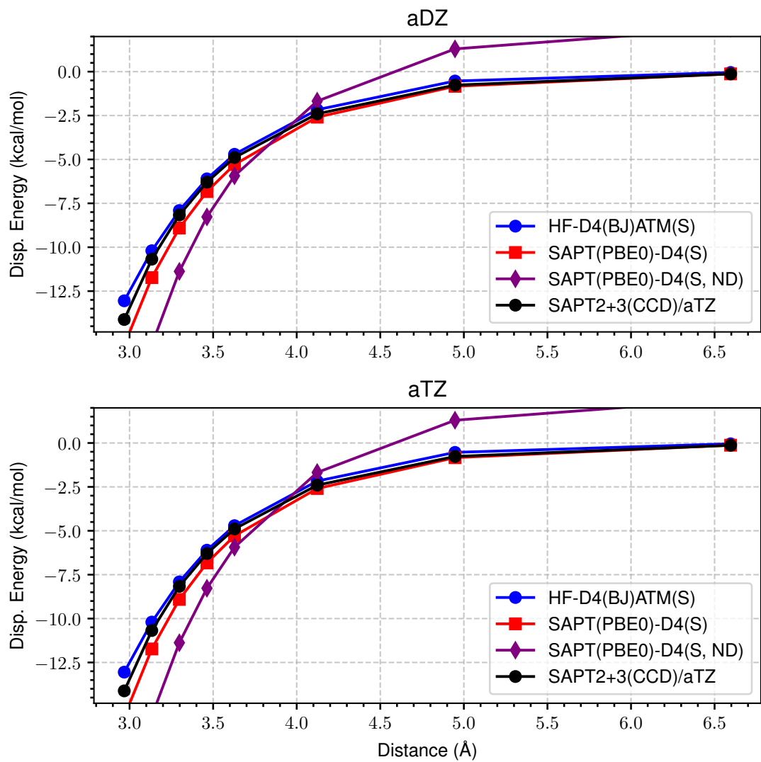
Figure 11: LoS Dispersion Curves for s66x8 27_Benzene-Pyridine
