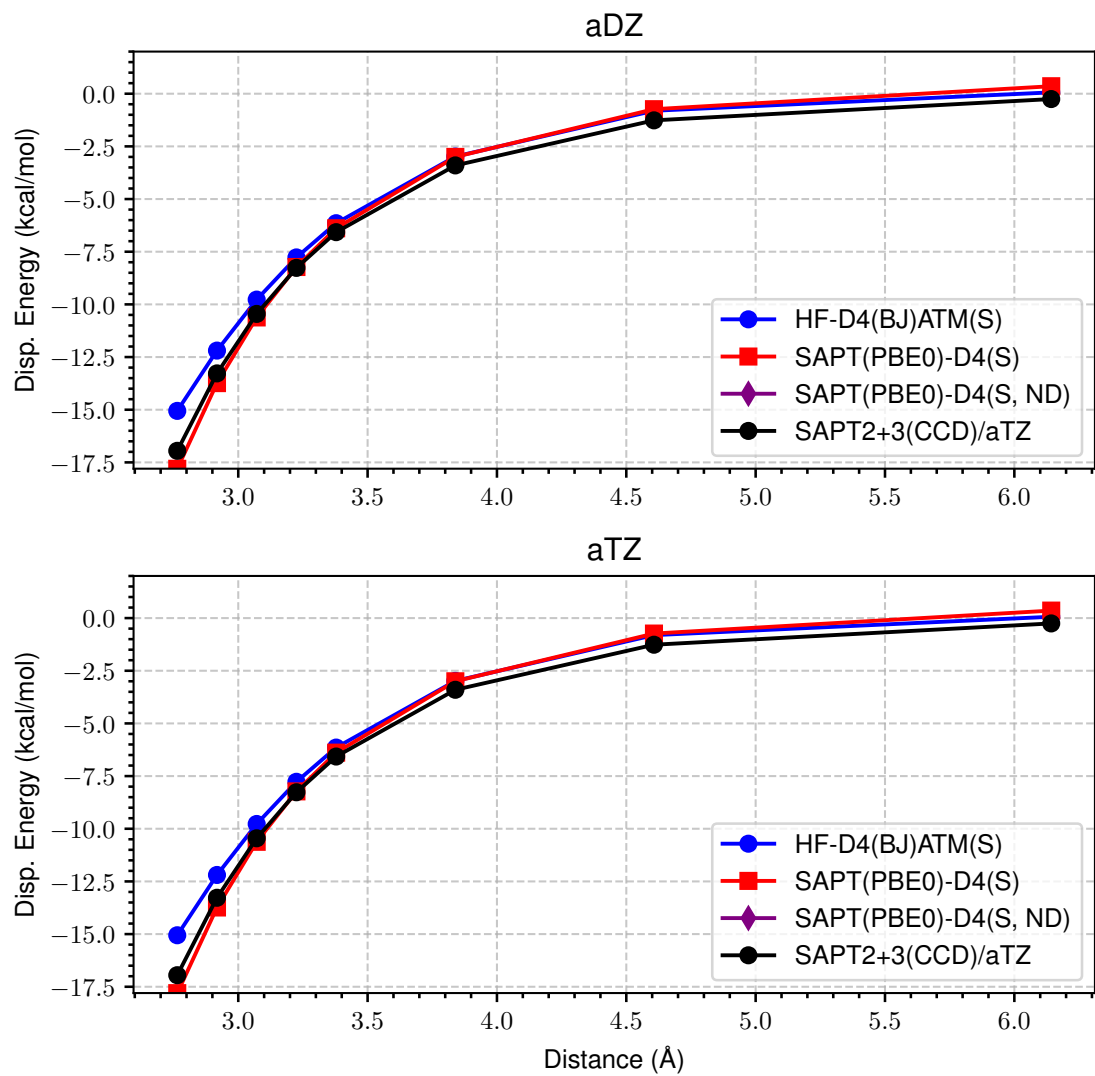
Figure 4: LoS Dispersion Curves for s66x8 28_Benzene-Uracil
