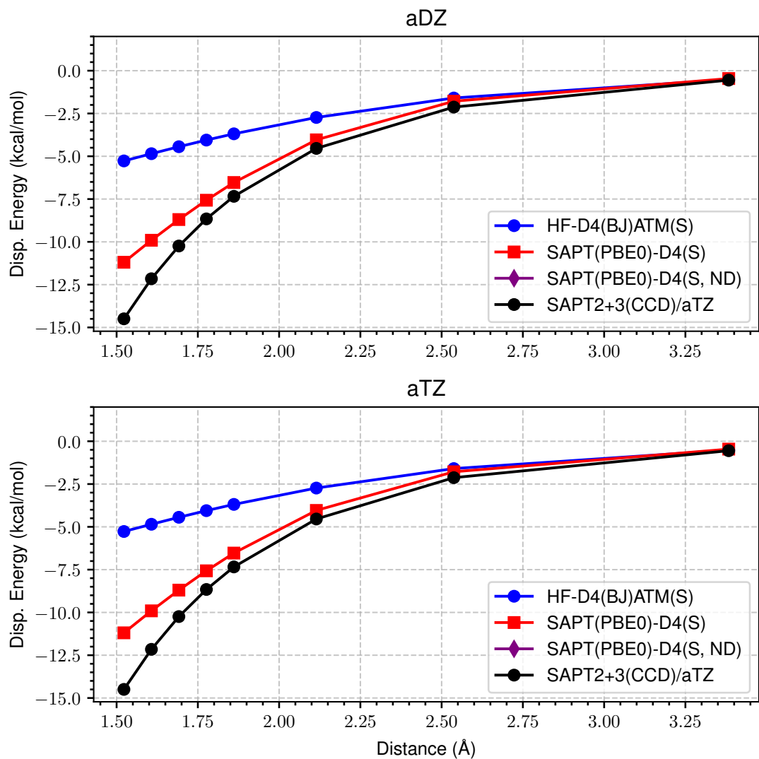
Figure 34: LoS Dispersion Curves for s66x8 20_AcOH-AcOH
