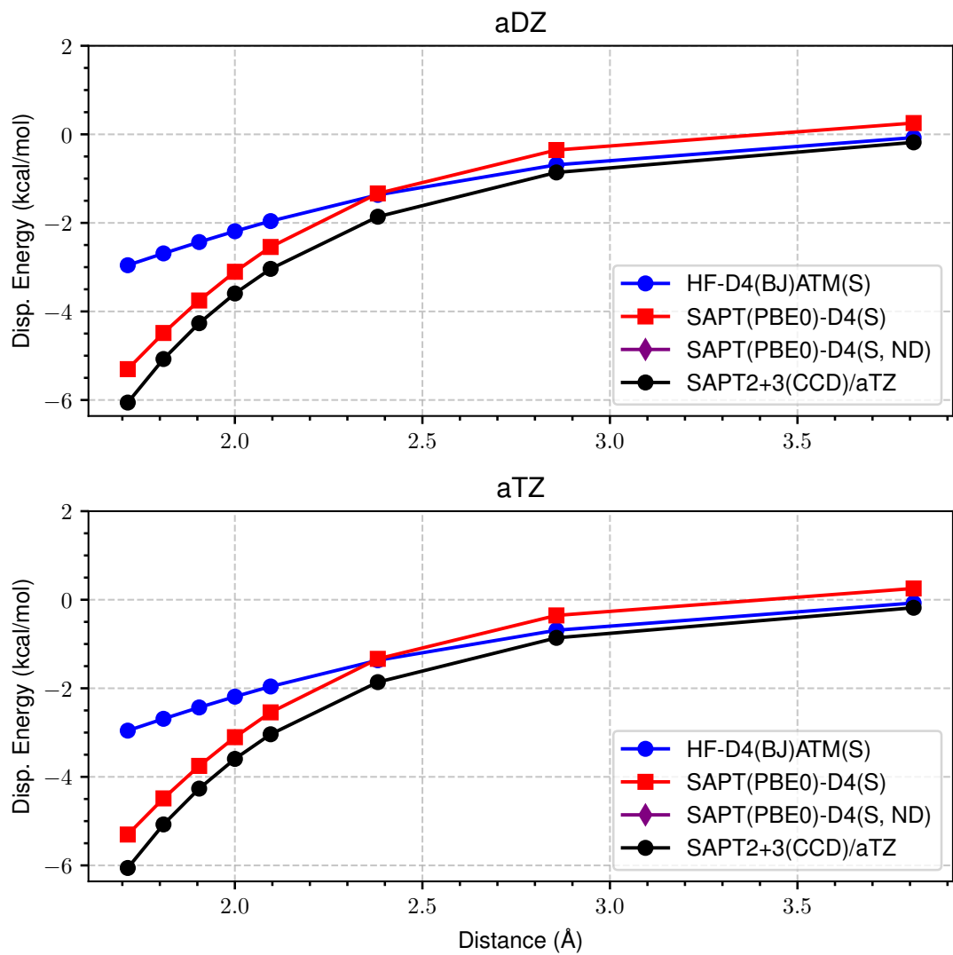
Figure 25: LoS Dispersion Curves for s66x8 04_Water-Peptide
