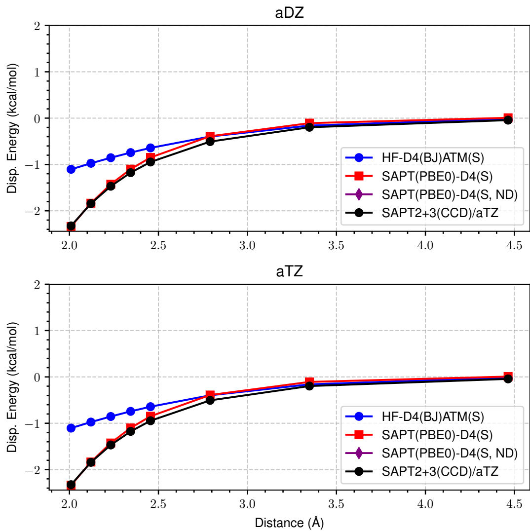
Figure 30: LoS Dispersion Curves for s66x8 59_Ethyne-Water
