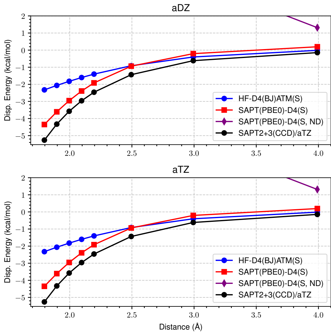
Figure 49: LoS Dispersion Curves for s66x8 18_Water-Pyridine
