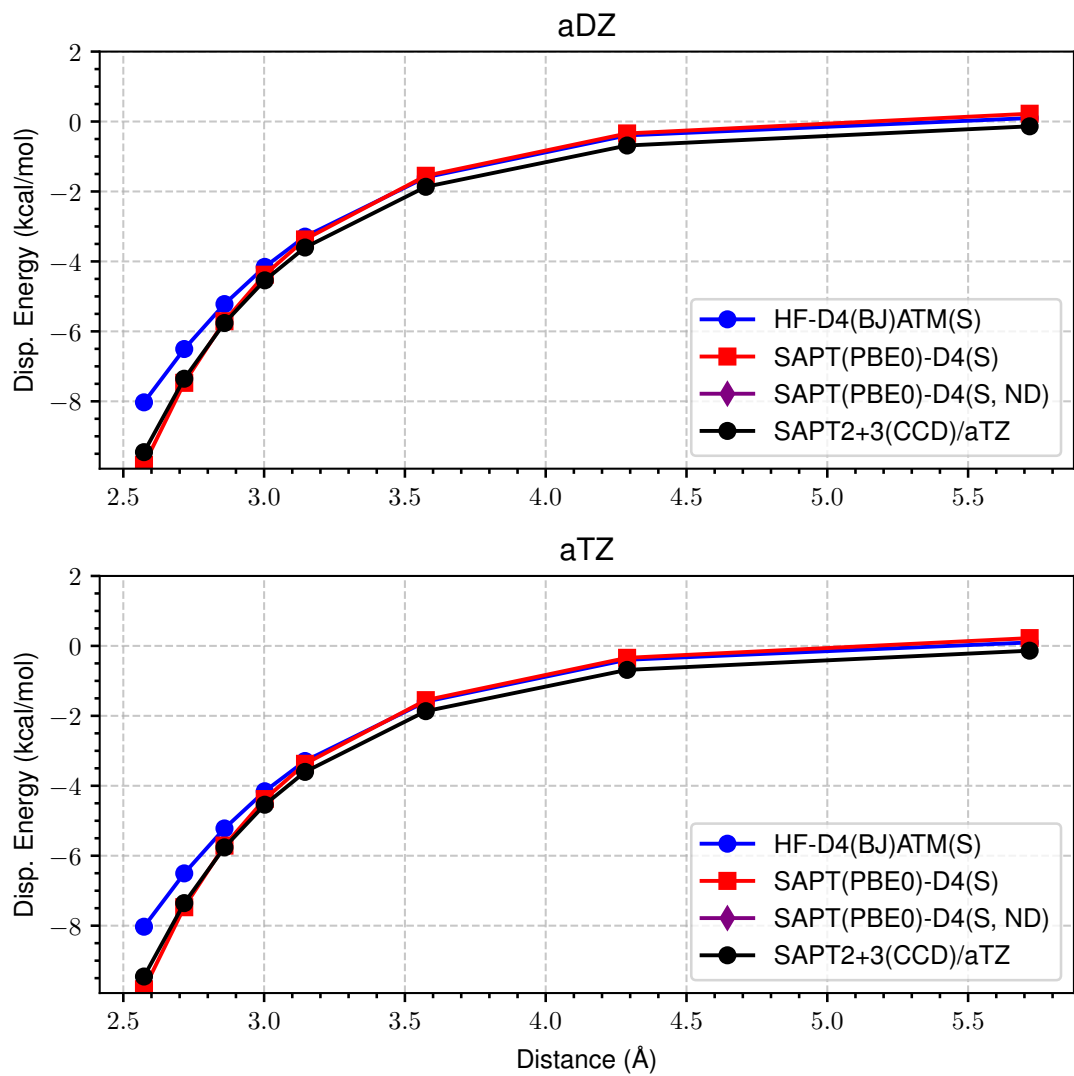
Figure 39: LoS Dispersion Curves for s66x8 63_Benzene-AcOH
