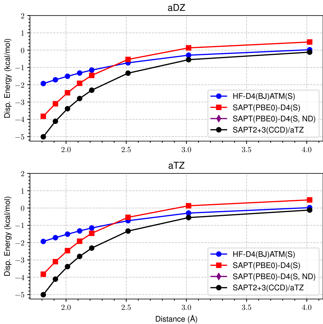
Figure 41: LoS Dispersion Curves for s66x8 03_Water-MeNH2
