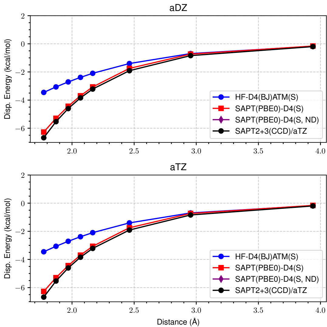
Figure 48: LoS Dispersion Curves for s66x8 06_MeOH-MeNH2
