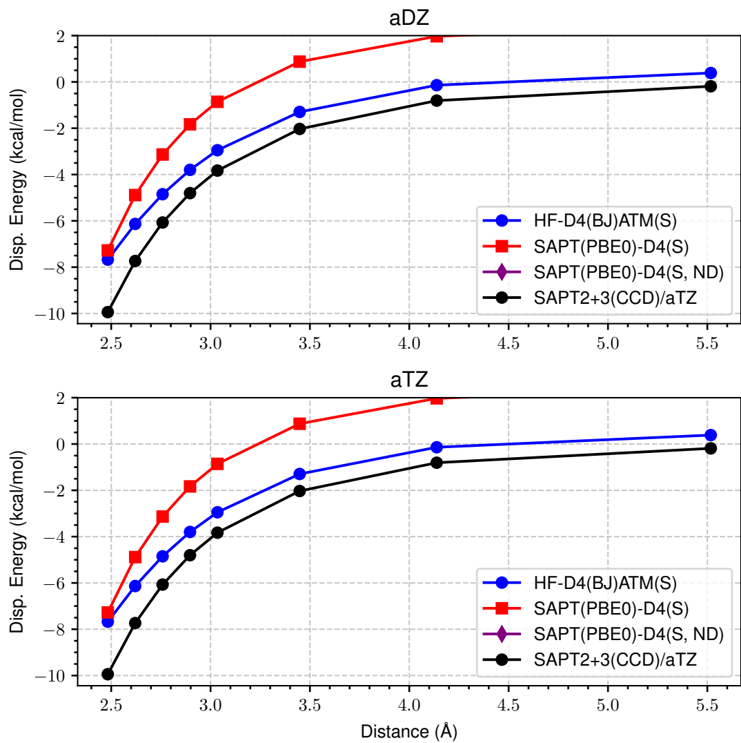
Figure 53: LoS Dispersion Curves for s66x8 43_Uracil-Neopentane
