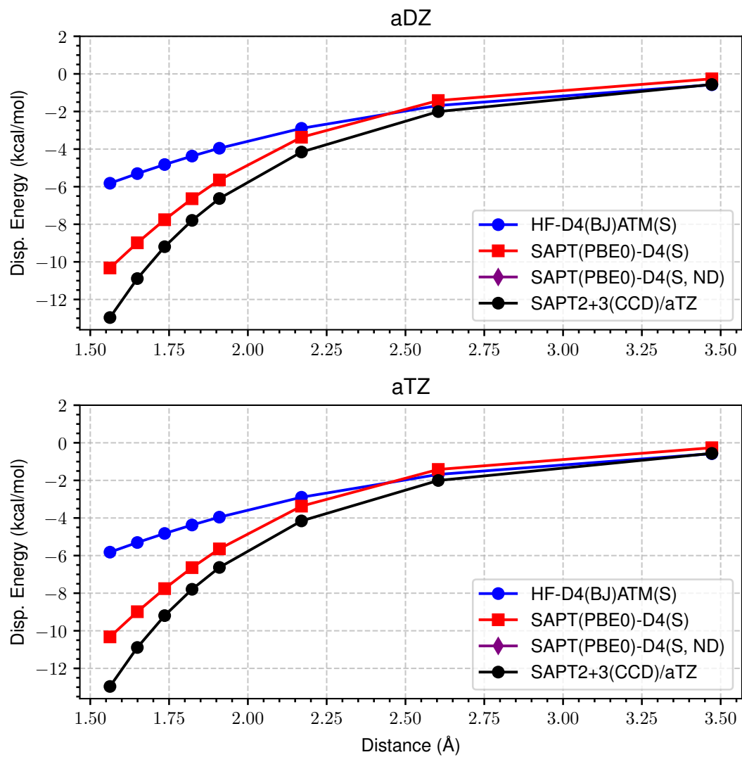
Figure 26: LoS Dispersion Curves for s66x8 23_AcNH2-Uracil
