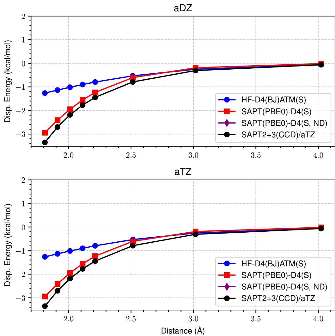
Figure 22: LoS Dispersion Curves for s66x8 01_Water-Water
