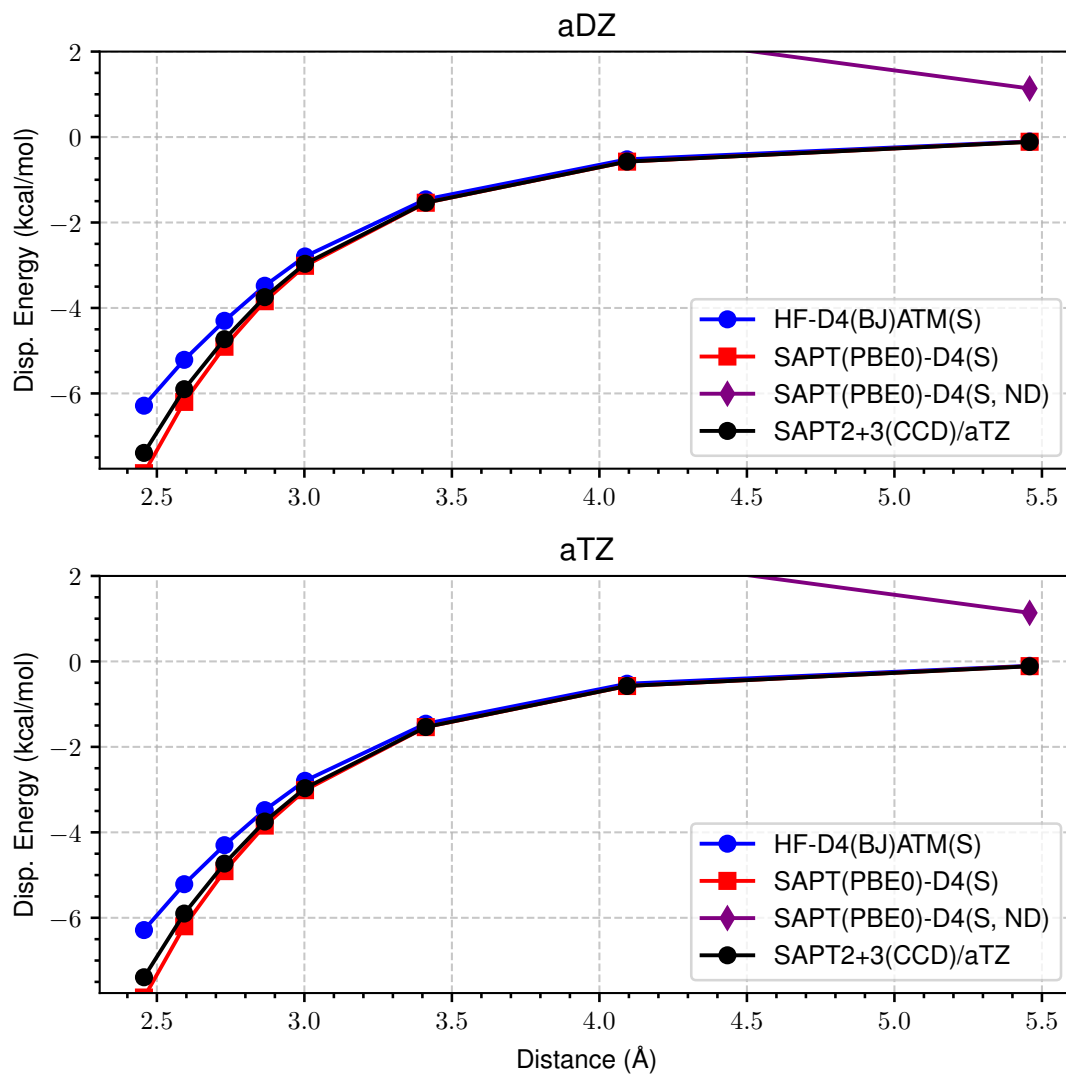
Figure 44: LoS Dispersion Curves for s66x8 56_Benzene-MeNH2
