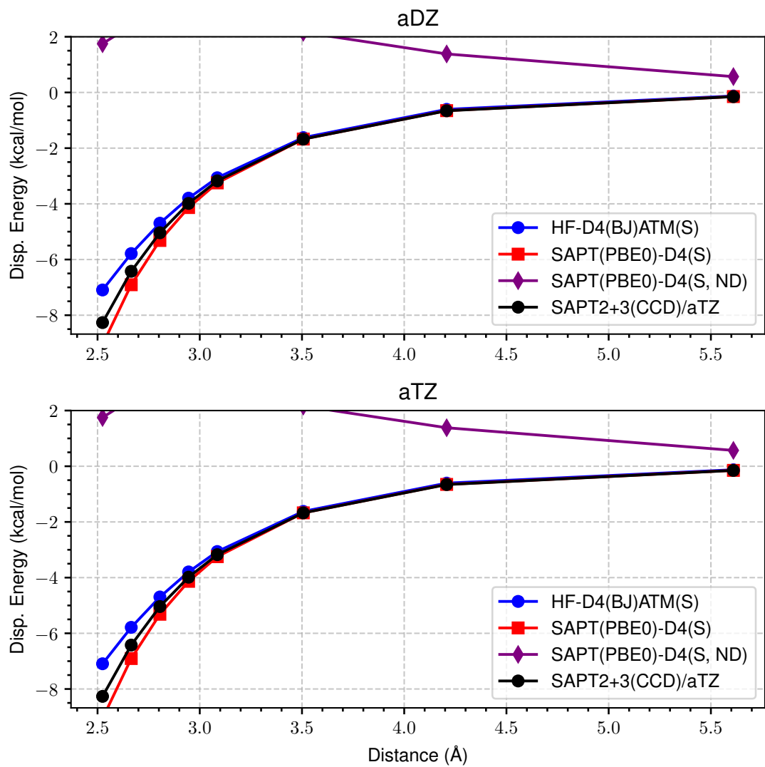
Figure 17: LoS Dispersion Curves for s66x8 47_Benzene-Benzene
