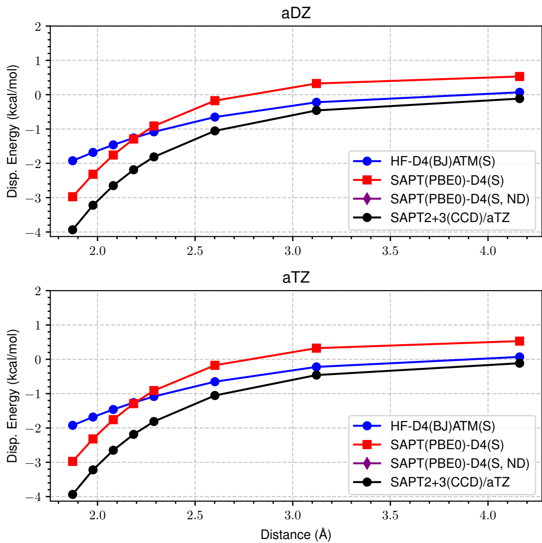
Figure 6: LoS Dispersion Curves for s66x8 16_Peptide-Water
