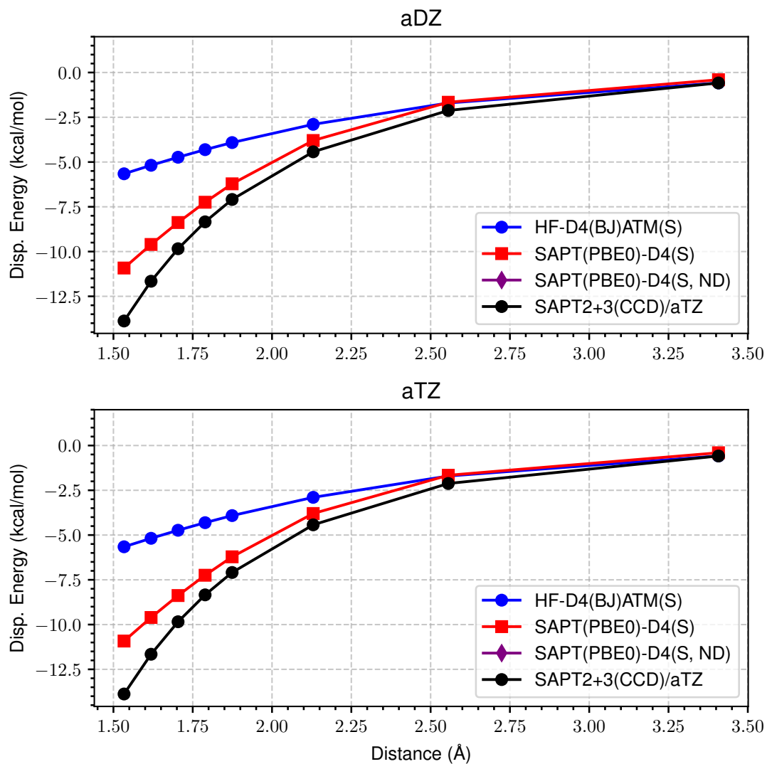
Figure 15: LoS Dispersion Curves for s66x8 22_AcOH-Uracil
