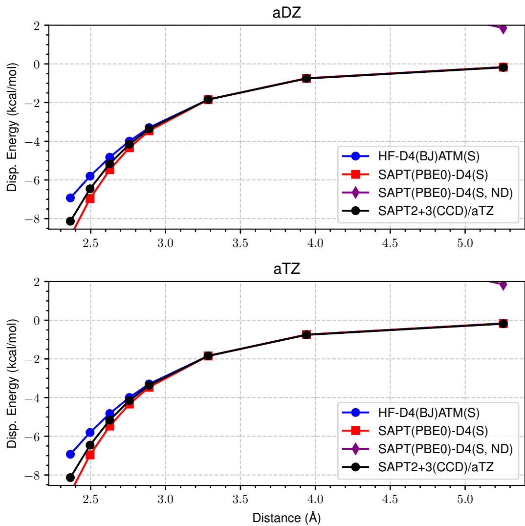
Figure 28: LoS Dispersion Curves for s66x8 48_Pyridine-Pyridine
