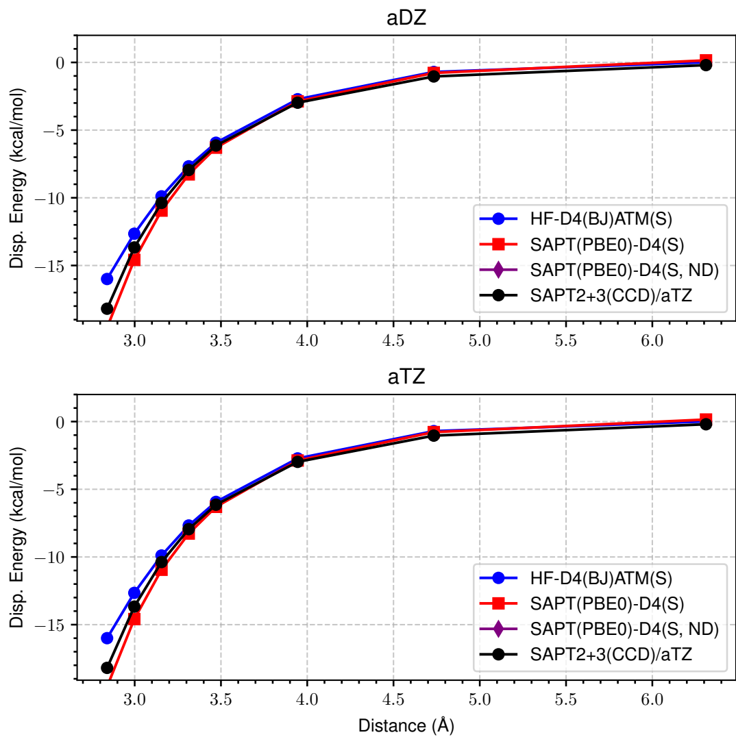
Figure 18: LoS Dispersion Curves for s66x8 29_Pyridine-Uracil
