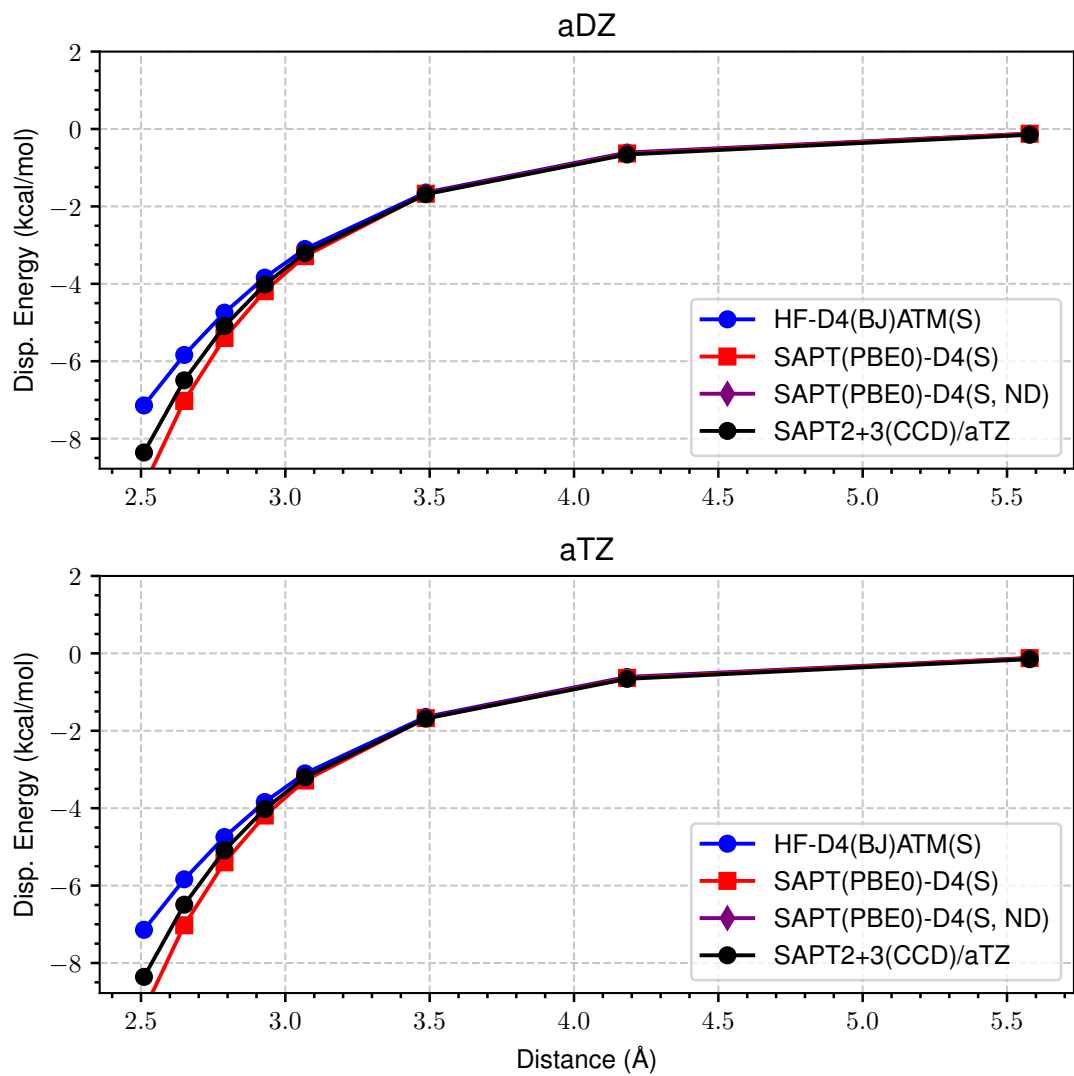
Figure 64: LoS Dispersion Curves for s66x8 49_Benzene-Pyridine
