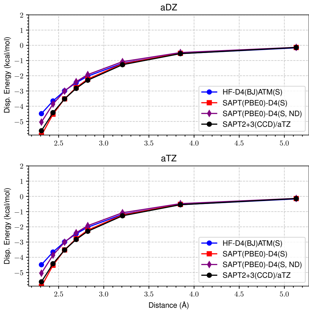
Figure 62: LoS Dispersion Curves for s66x8 36_Neopentane-Neopentane
