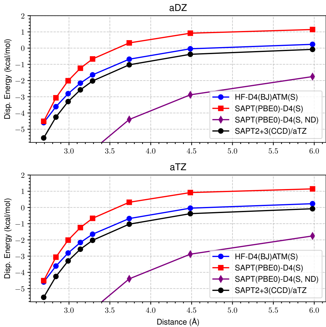
Figure 2: LoS Dispersion Curves for s66x8 45_Ethyne-Pentane
