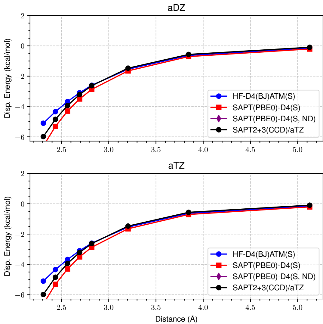
Figure 31: LoS Dispersion Curves for s66x8 64_Peptide-Ethene
