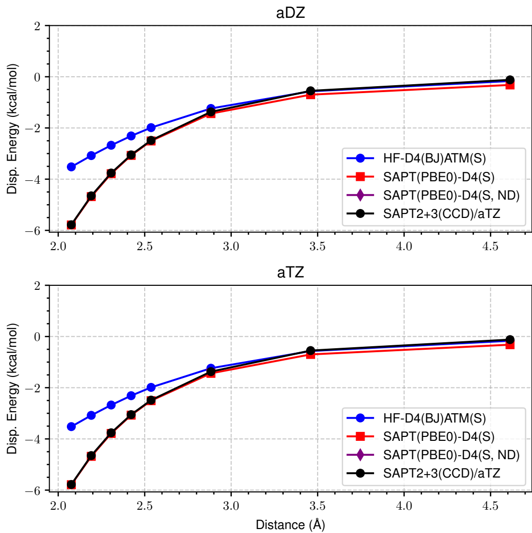
Figure 58: LoS Dispersion Curves for s66x8 60_Ethyne-AcOH
