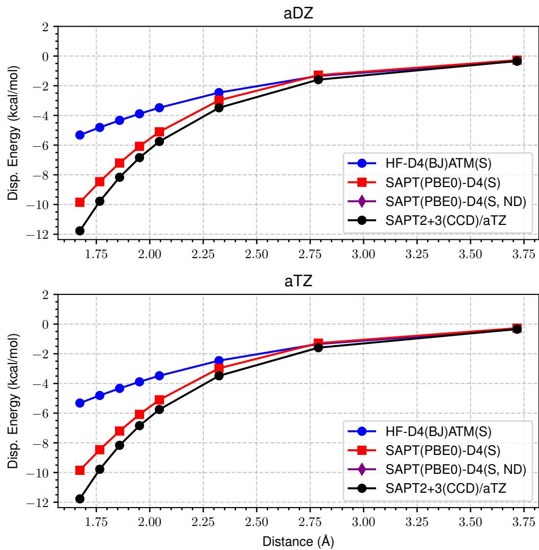
Figure 50: LoS Dispersion Curves for s66x8 21_AcNH2-AcNH2
