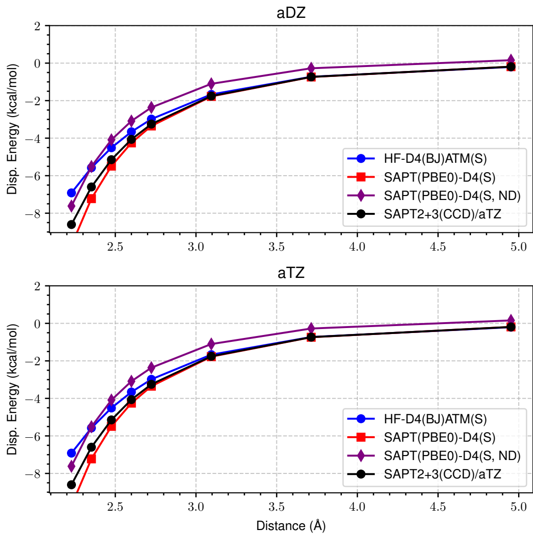
Figure 47: LoS Dispersion Curves for s66x8 35_Neopentane-Pentane
