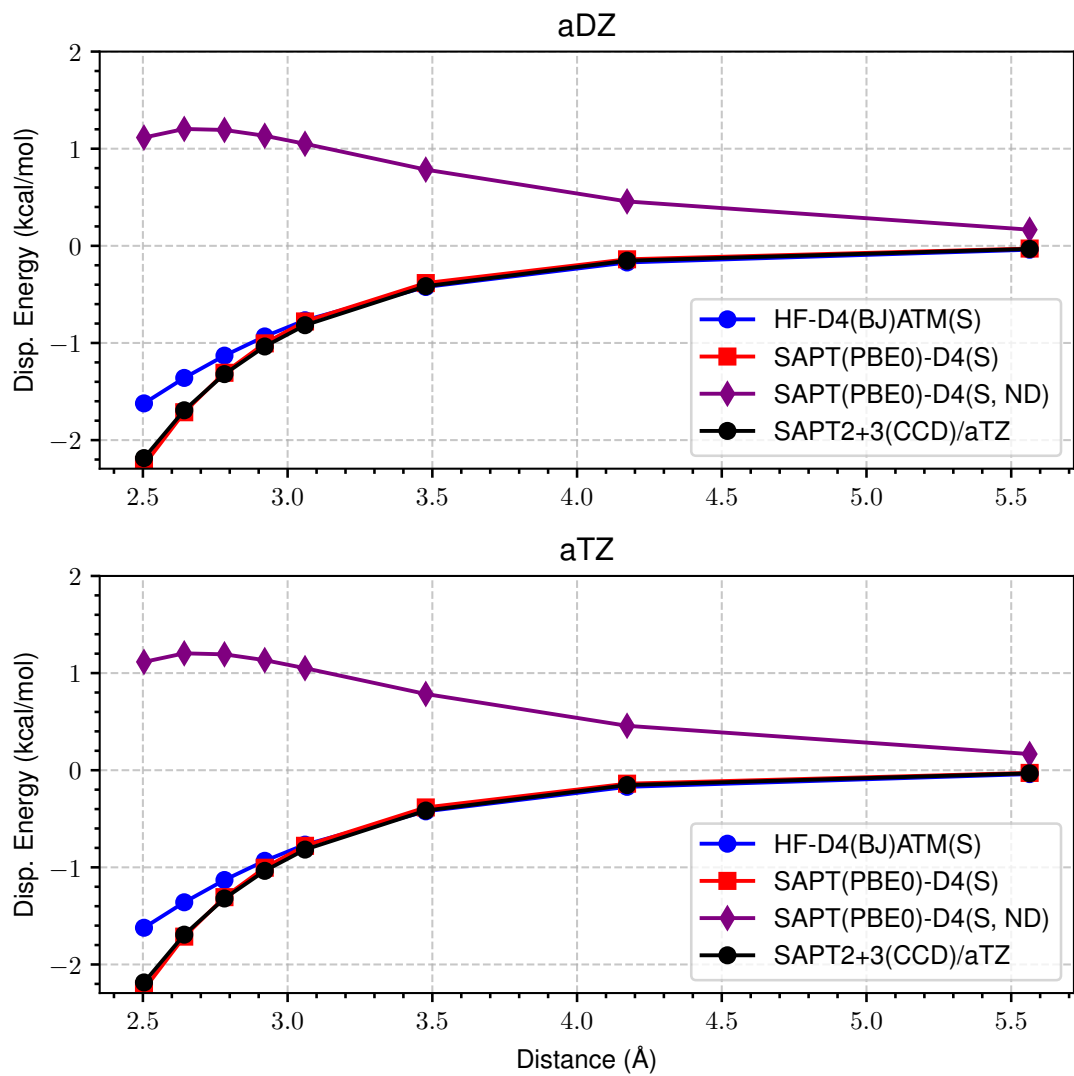
Figure 35: LoS Dispersion Curves for s66x8 51_Ethyne-Ethyne
