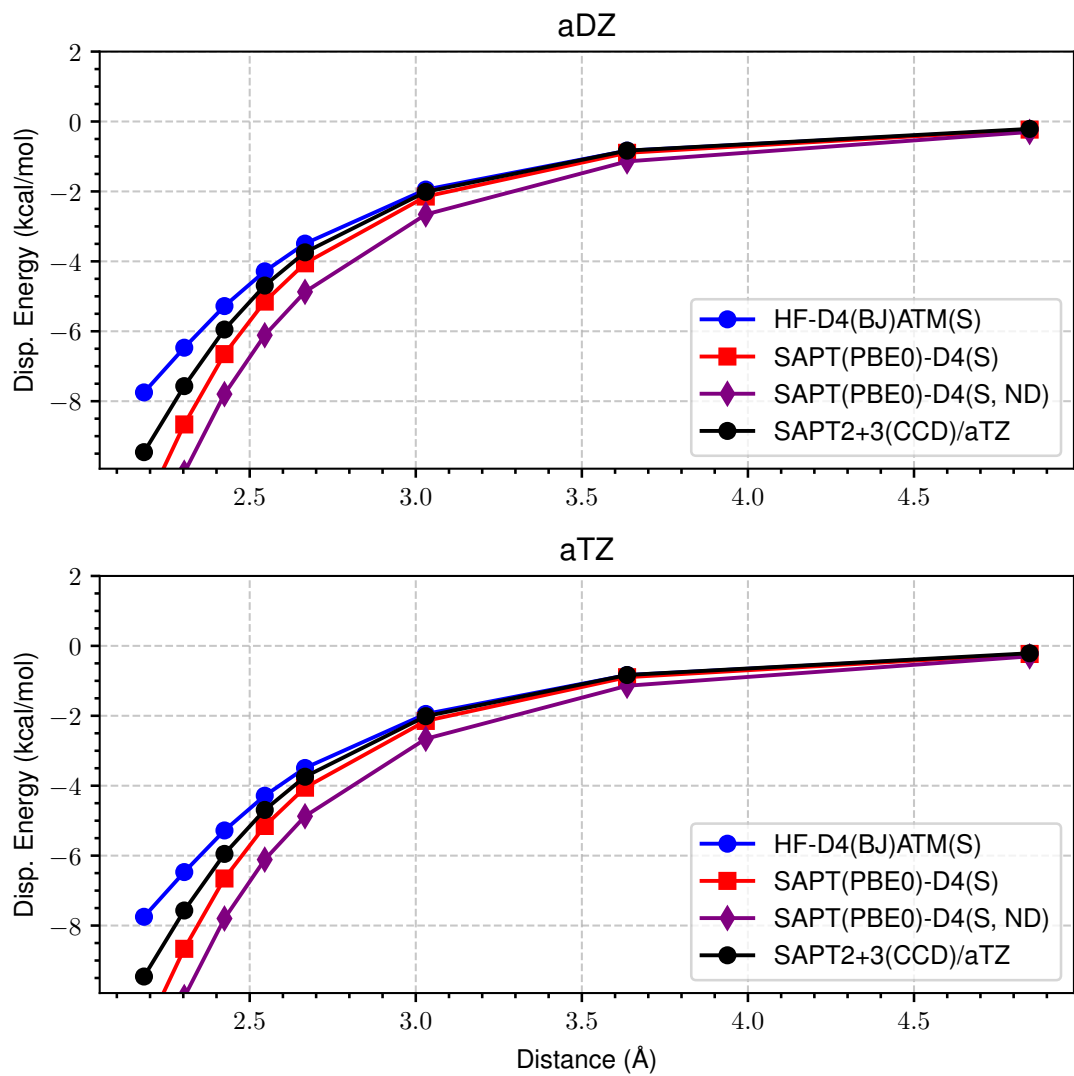
Figure 57: LoS Dispersion Curves for s66x8 38_Cyclopentane-Cyclopentane
