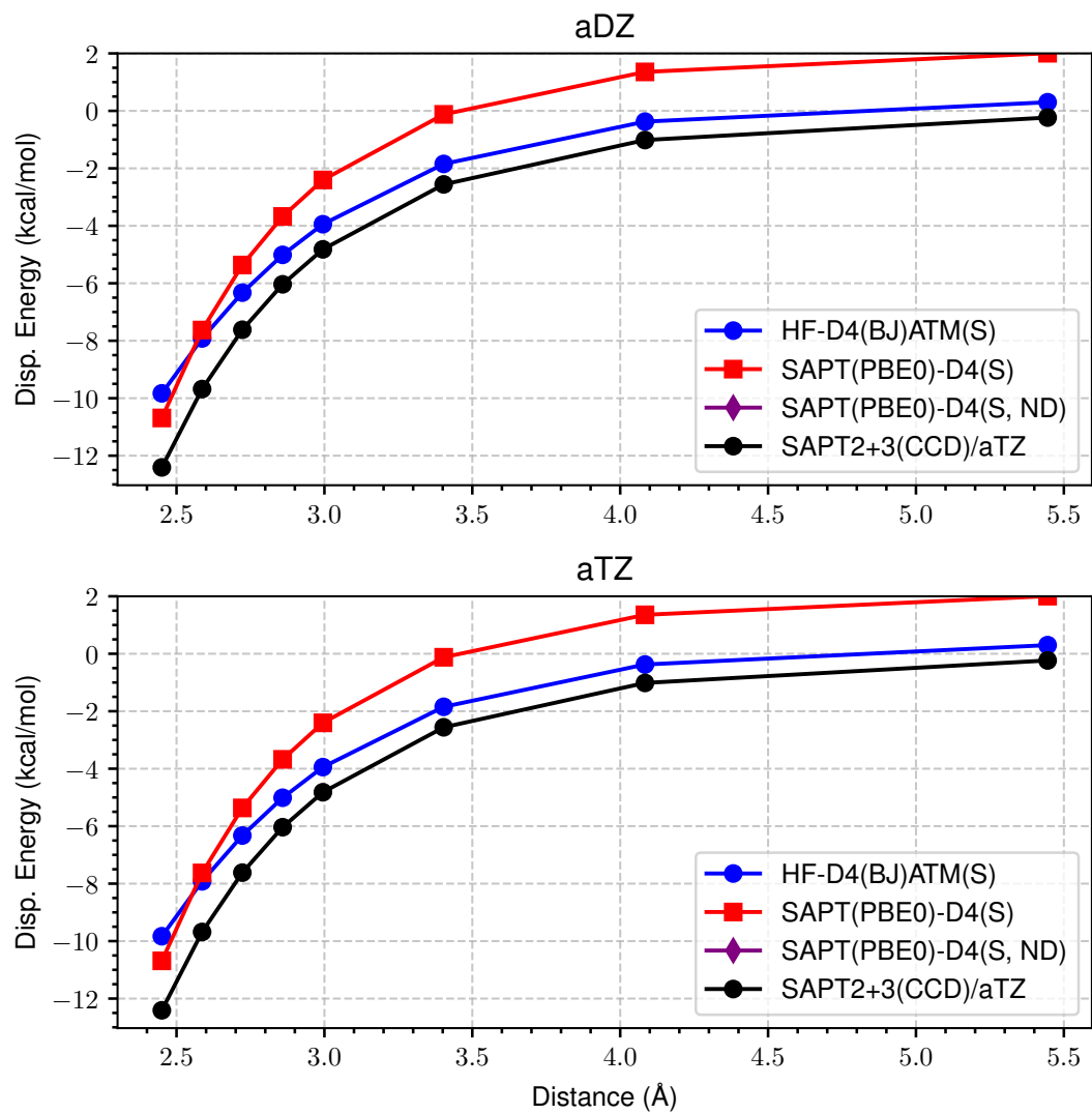
Figure 29: LoS Dispersion Curves for s66x8 42_Uracil-Cyclopentane
