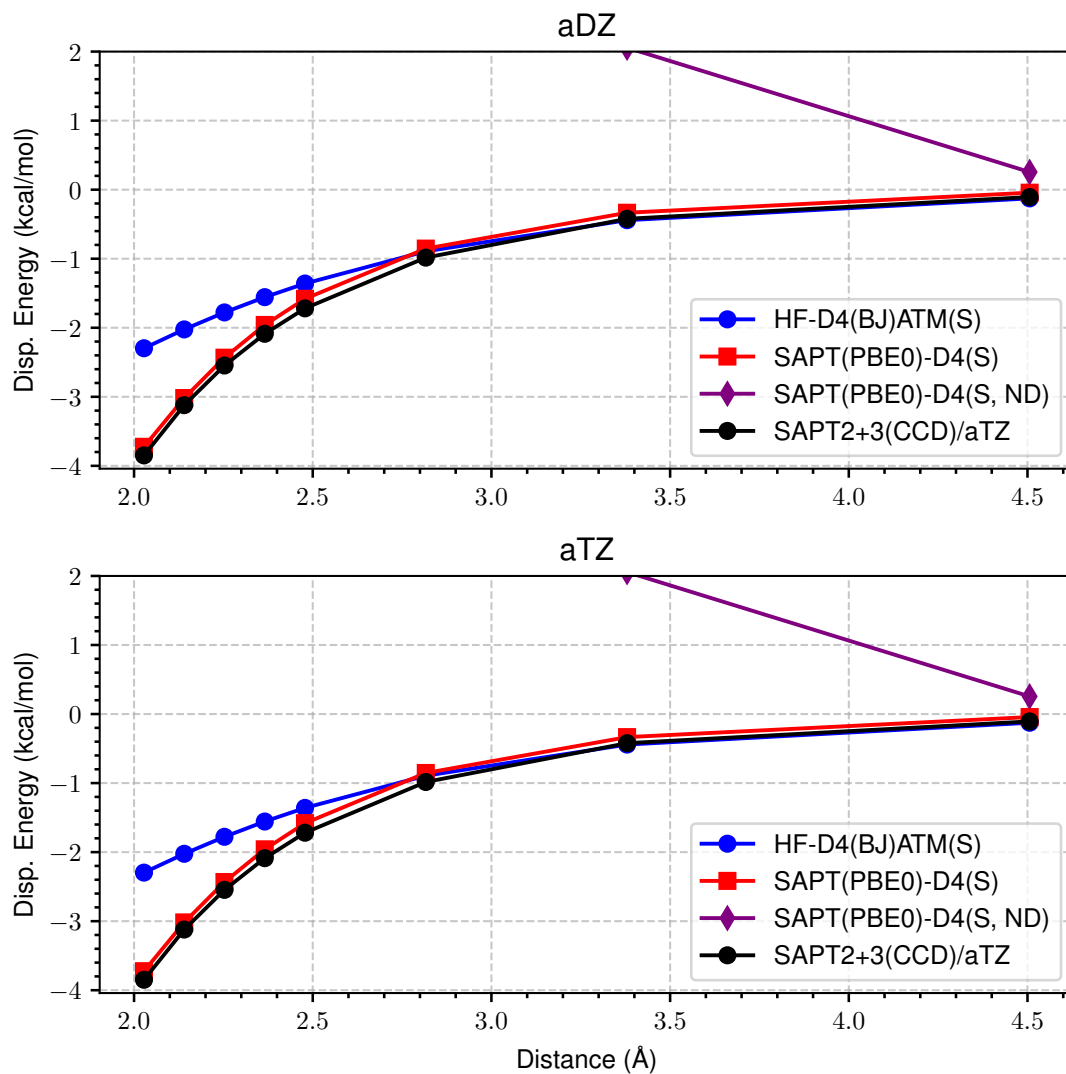
Figure 16: LoS Dispersion Curves for s66x8 65_Pyridine-Ethyne
