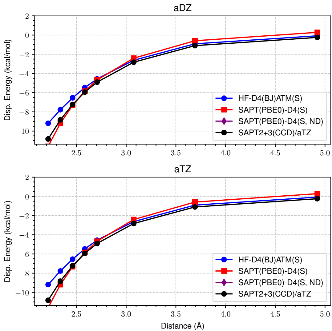
Figure 45: LoS Dispersion Curves for s66x8 46_Peptide-Pentane
