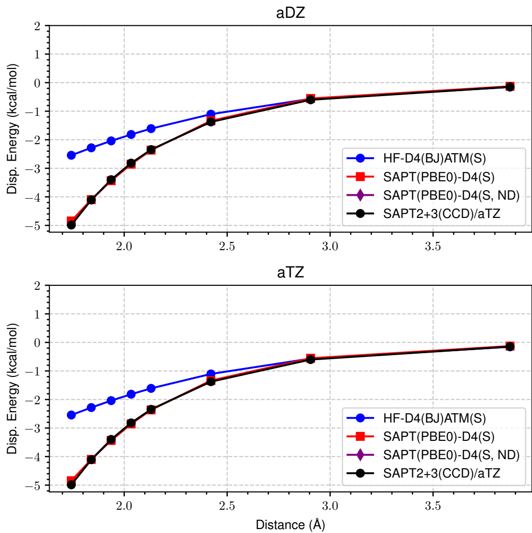
Figure 33: LoS Dispersion Curves for s66x8 05_MeOH-MeOH
