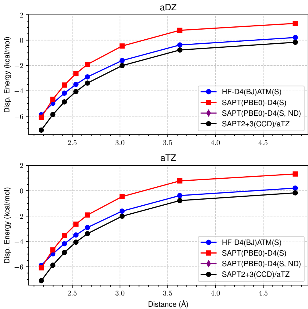
Figure 61: LoS Dispersion Curves for s66x8 61_Pentane-AcOH
