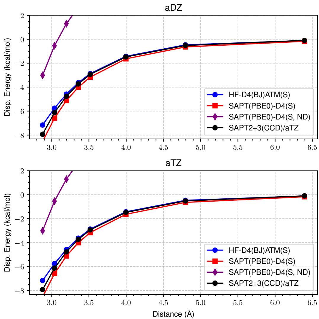
Figure 14: LoS Dispersion Curves for s66x8 33_Pyridine-Ethene
