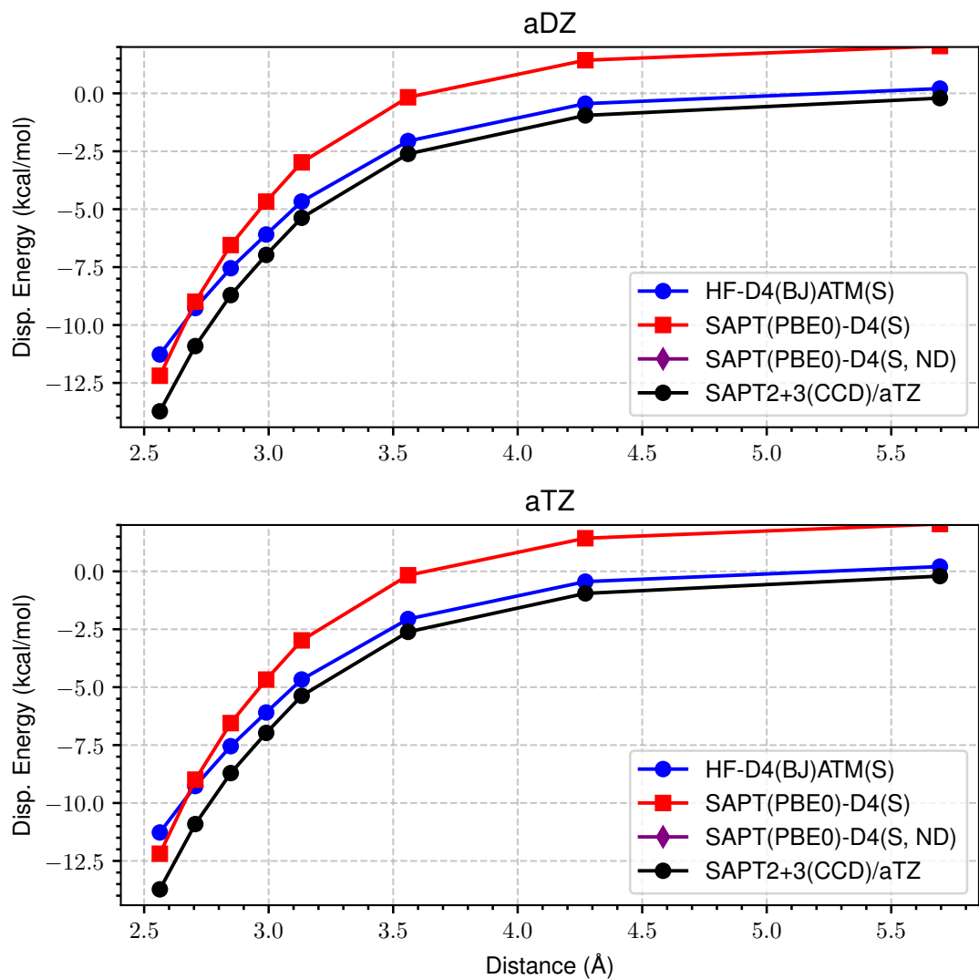
Figure 3: LoS Dispersion Curves for s66x8 41_Uracil-Pentane
