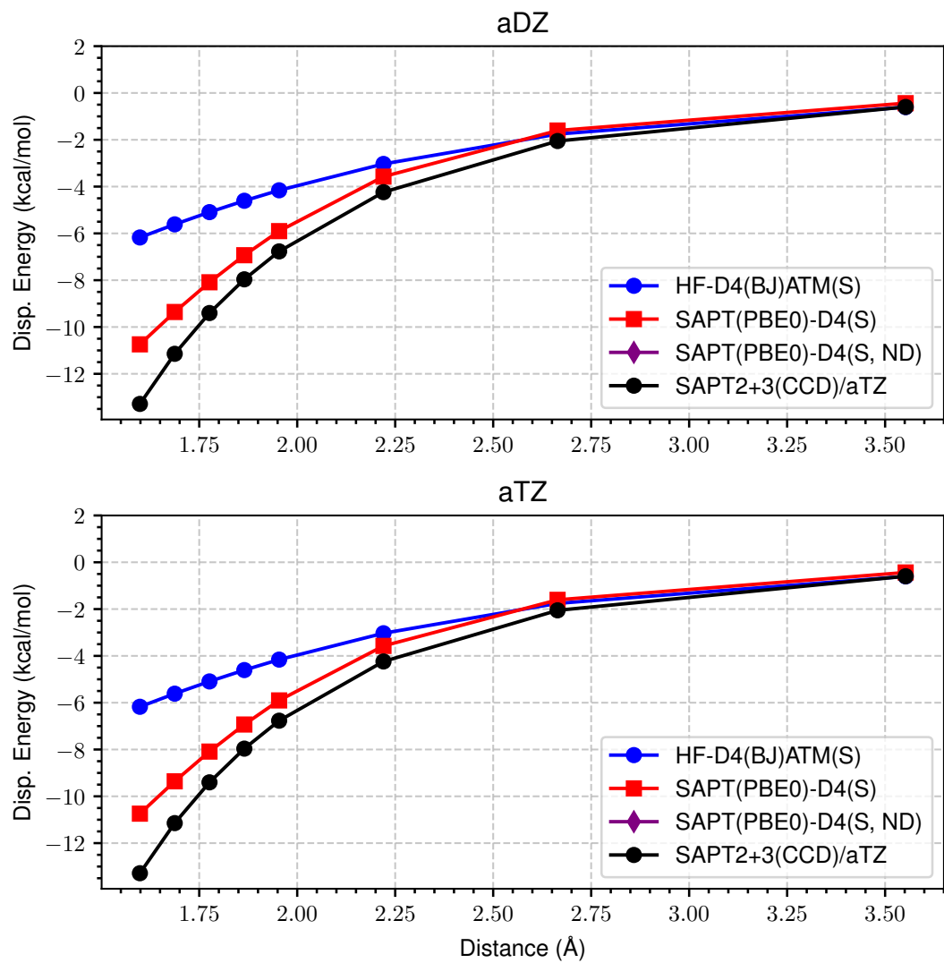
Figure 46: LoS Dispersion Curves for s66x8 17_Uracil-Uracil
