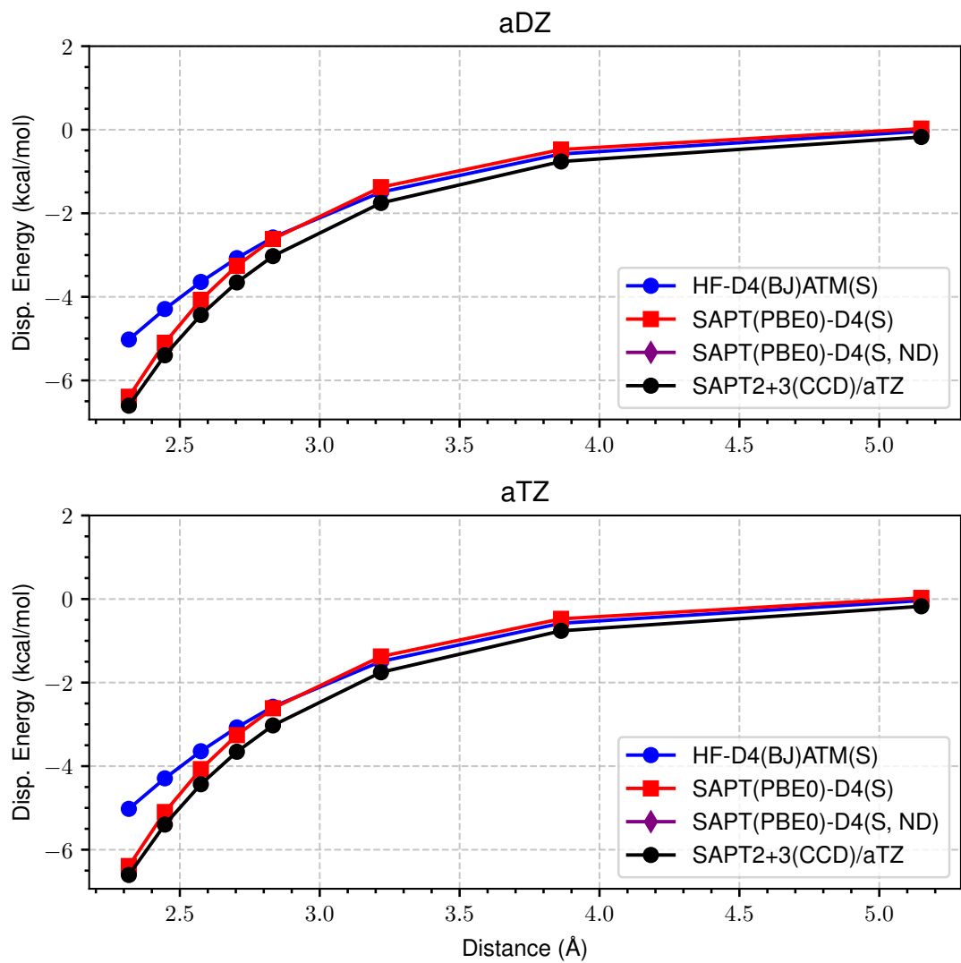
Figure 36: LoS Dispersion Curves for s66x8 53_Benzene-AcNH2
