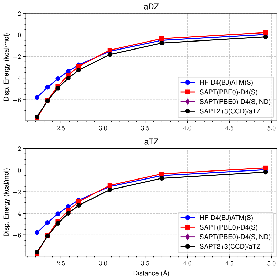
Figure 9: LoS Dispersion Curves for s66x8 52_Benzene-AcOH
