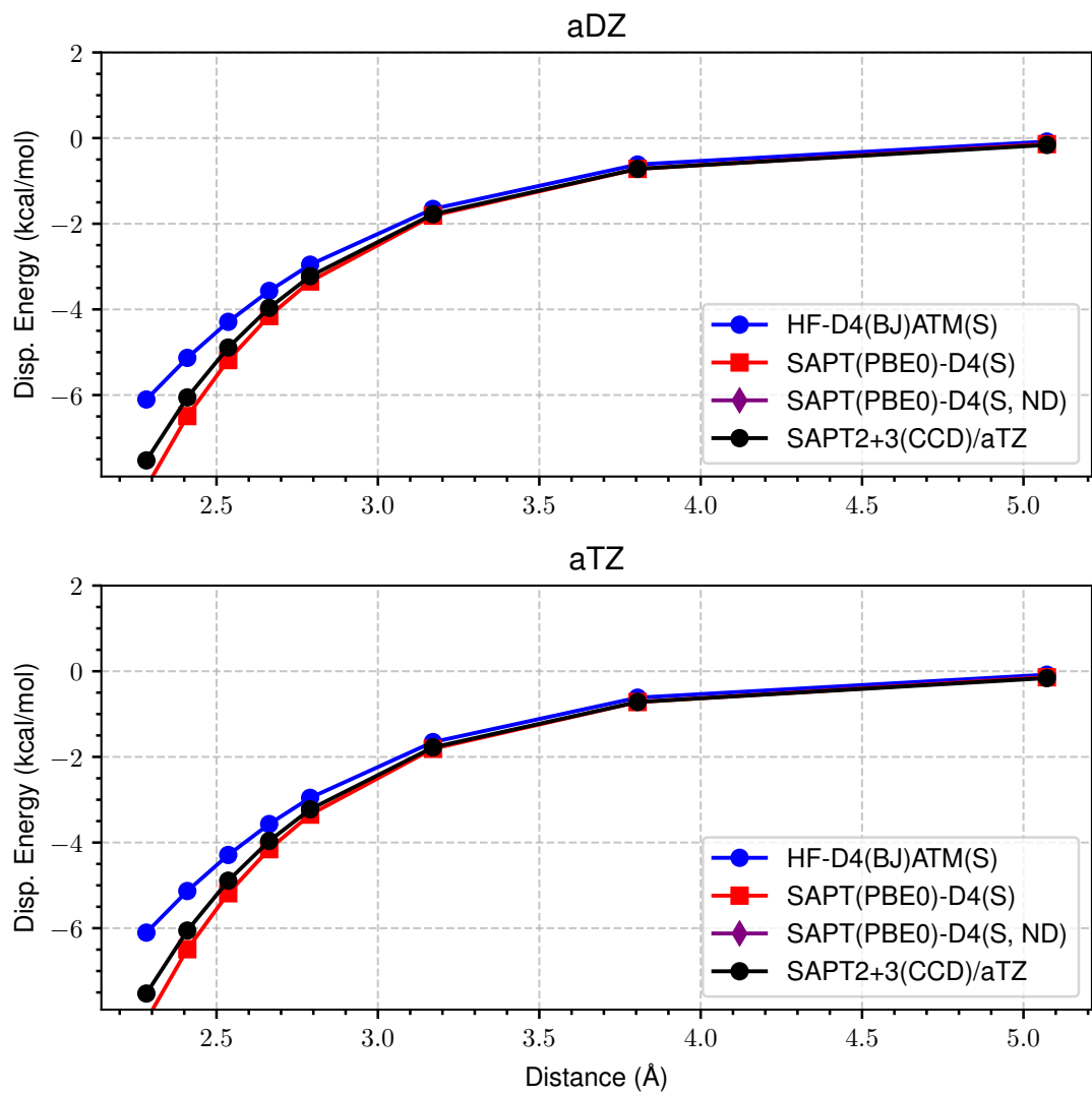
Figure 19: LoS Dispersion Curves for s66x8 55_Benzene-MeOH
