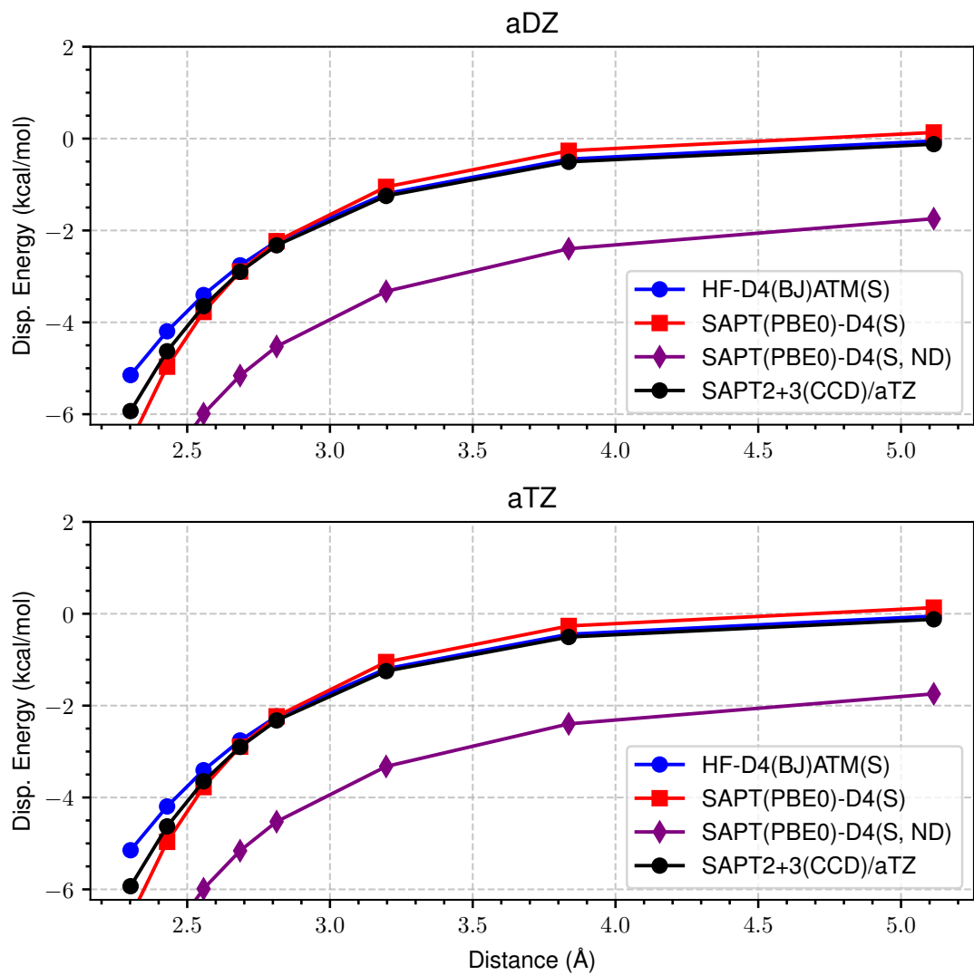
Figure 7: LoS Dispersion Curves for s66x8 44 Ethene-Pentane
