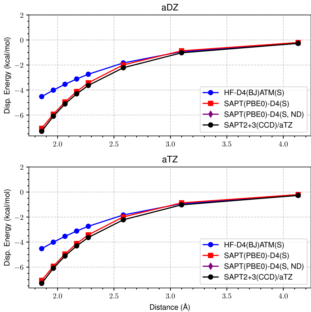
Figure 1: LoS Dispersion Curves for s66x8 14_Peptide-MeNH2
