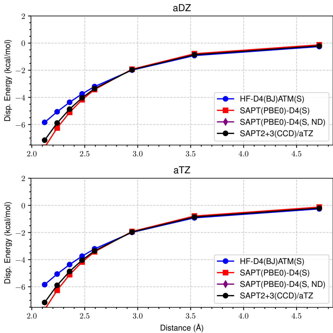
Figure 38: LoS Dispersion Curves for s66x8 66_MeNH2-Pyridine
