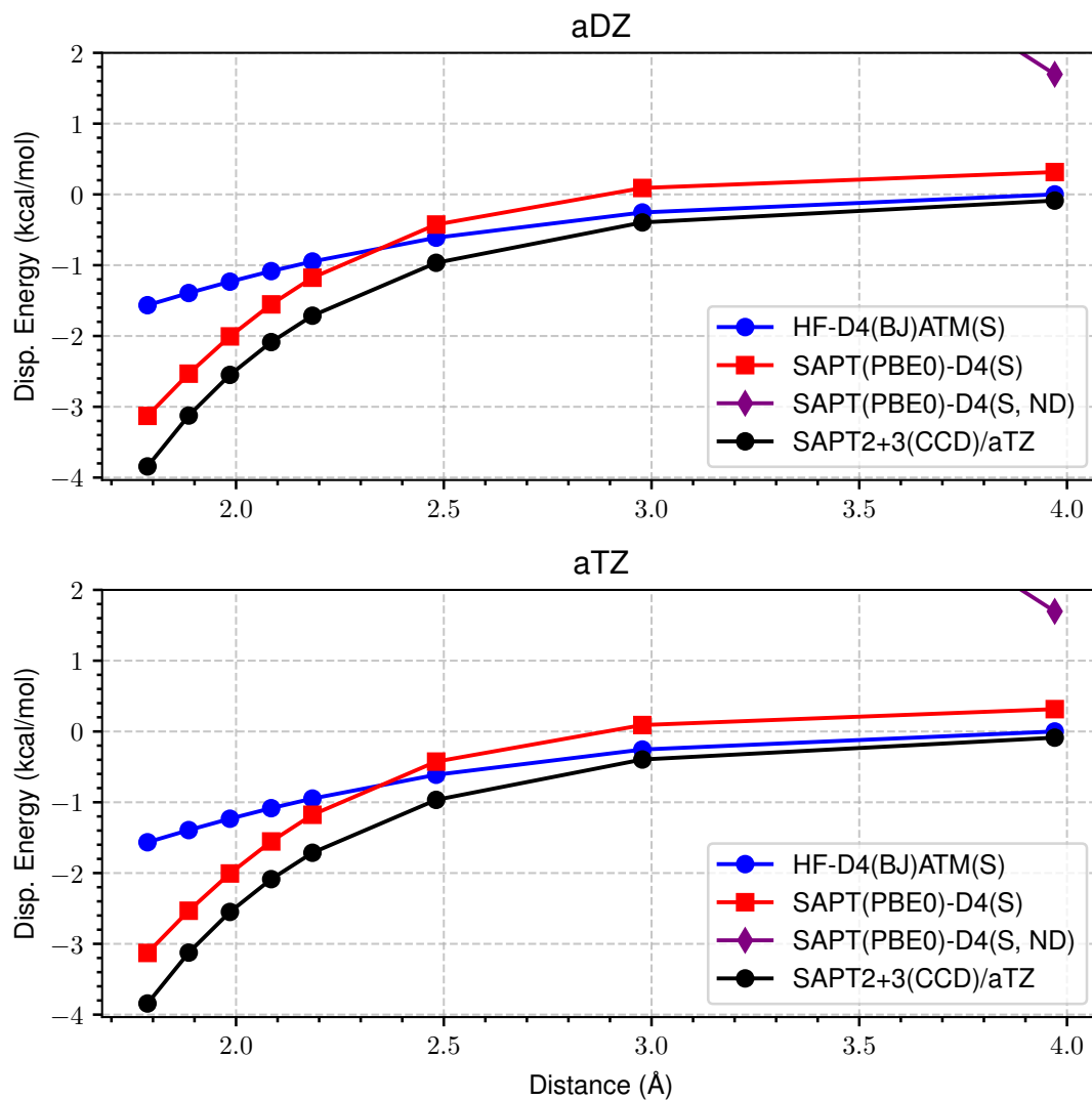
Figure 55: LoS Dispersion Curves for s66x8 08_MeOH-Water
