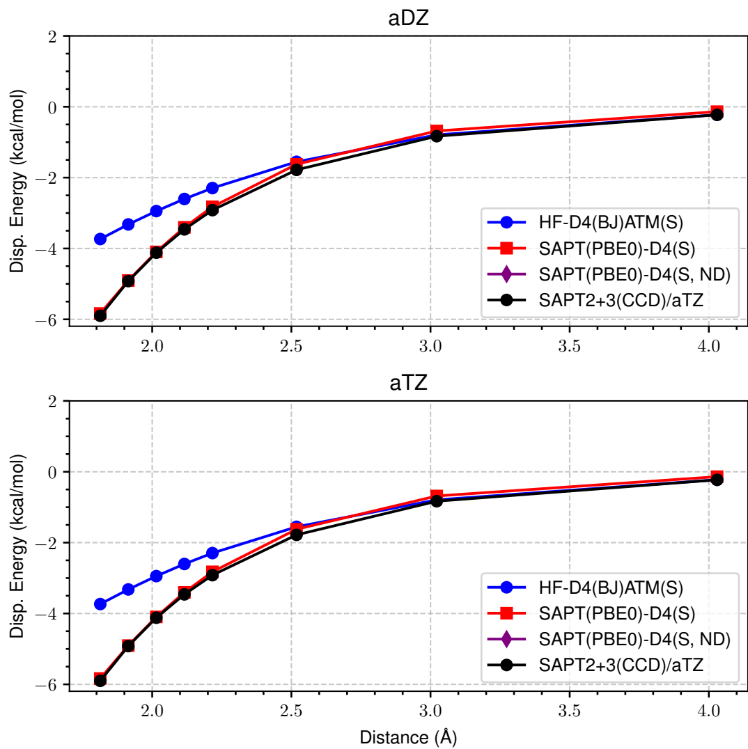
Figure 56: LoS Dispersion Curves for s66x8 13_Peptide-MeOH
