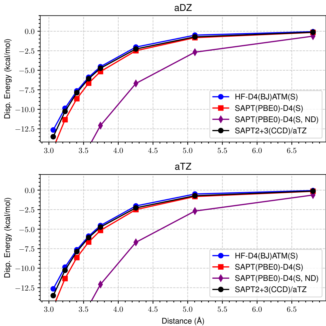
Figure 37: LoS Dispersion Curves for s66x8 24_Benzene-Benzene
