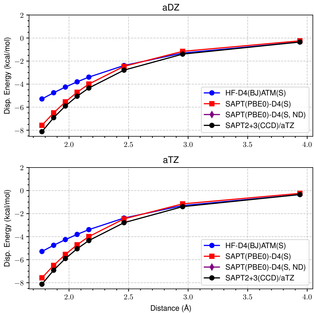
Figure 27: LoS Dispersion Curves for s66x8 15_Peptide-Peptide
