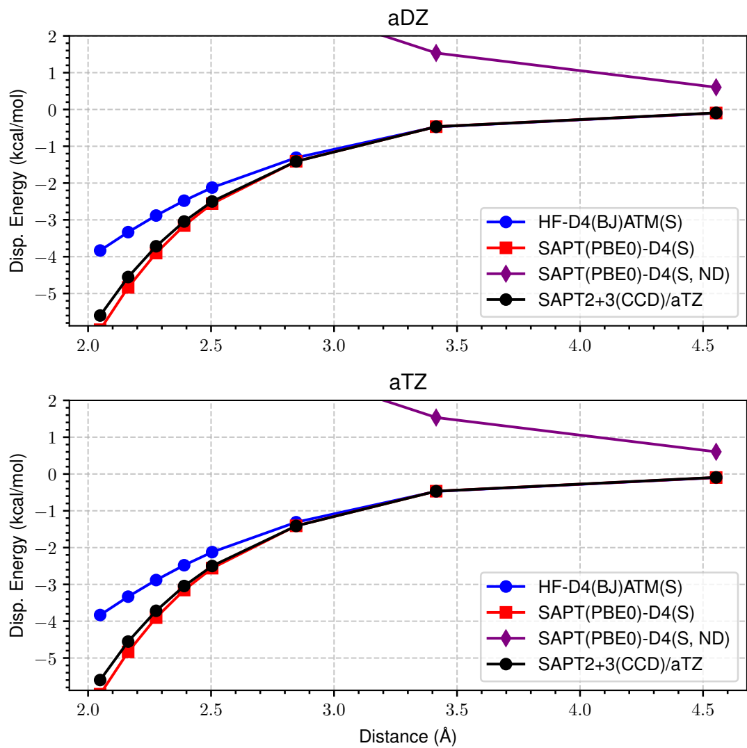
Figure 5: LoS Dispersion Curves for s66x8 10_MeNH2-MeNH2
