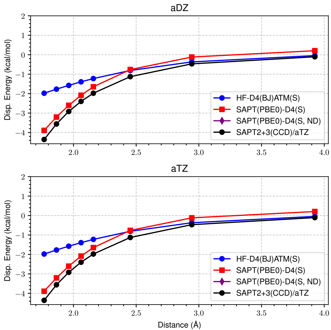
Figure 8: LoS Dispersion Curves for s66x8 02_Water-MeOH
