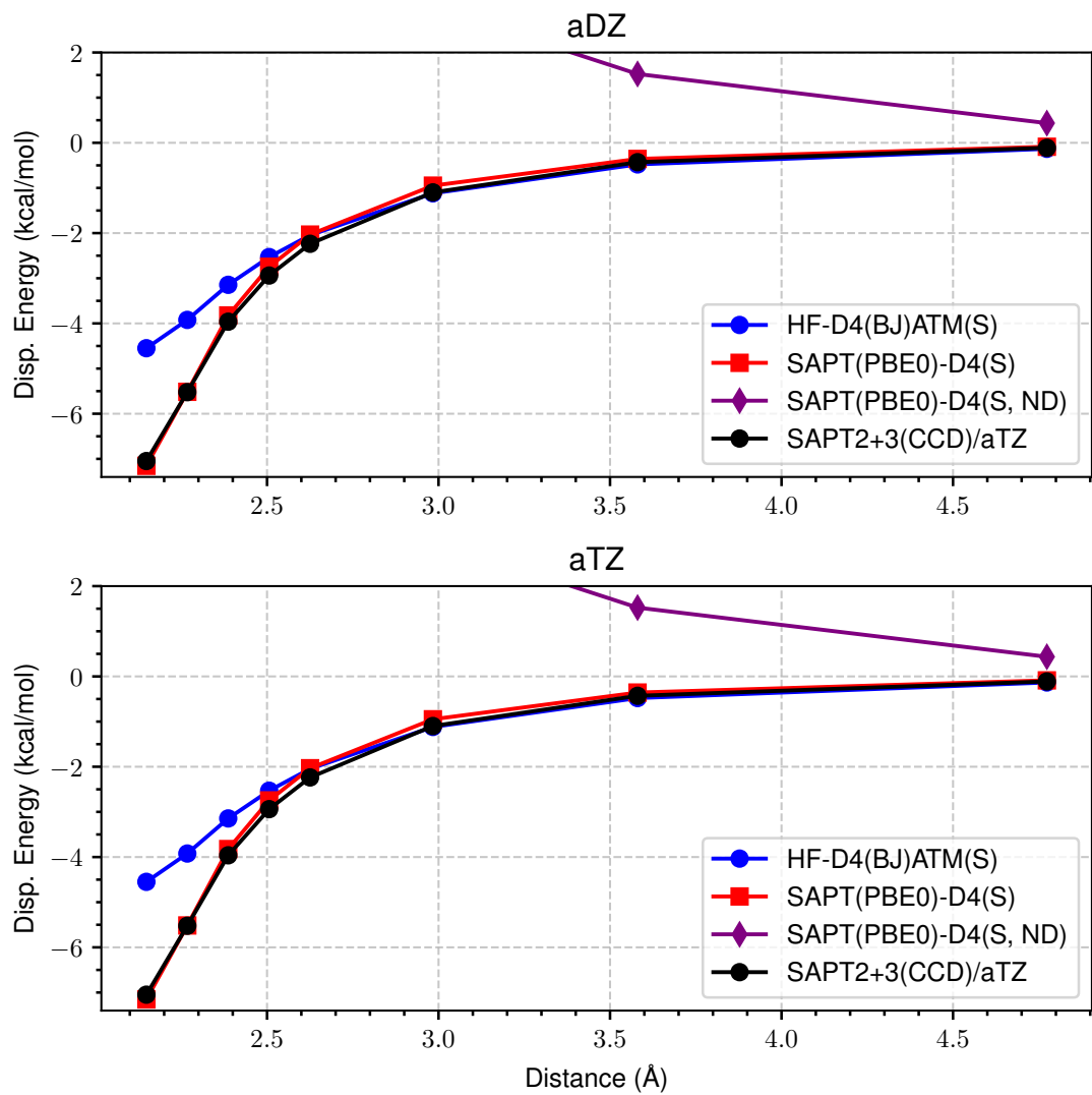
Figure 20: LoS Dispersion Curves for s66x8 58_Pyridine-Pyridine
