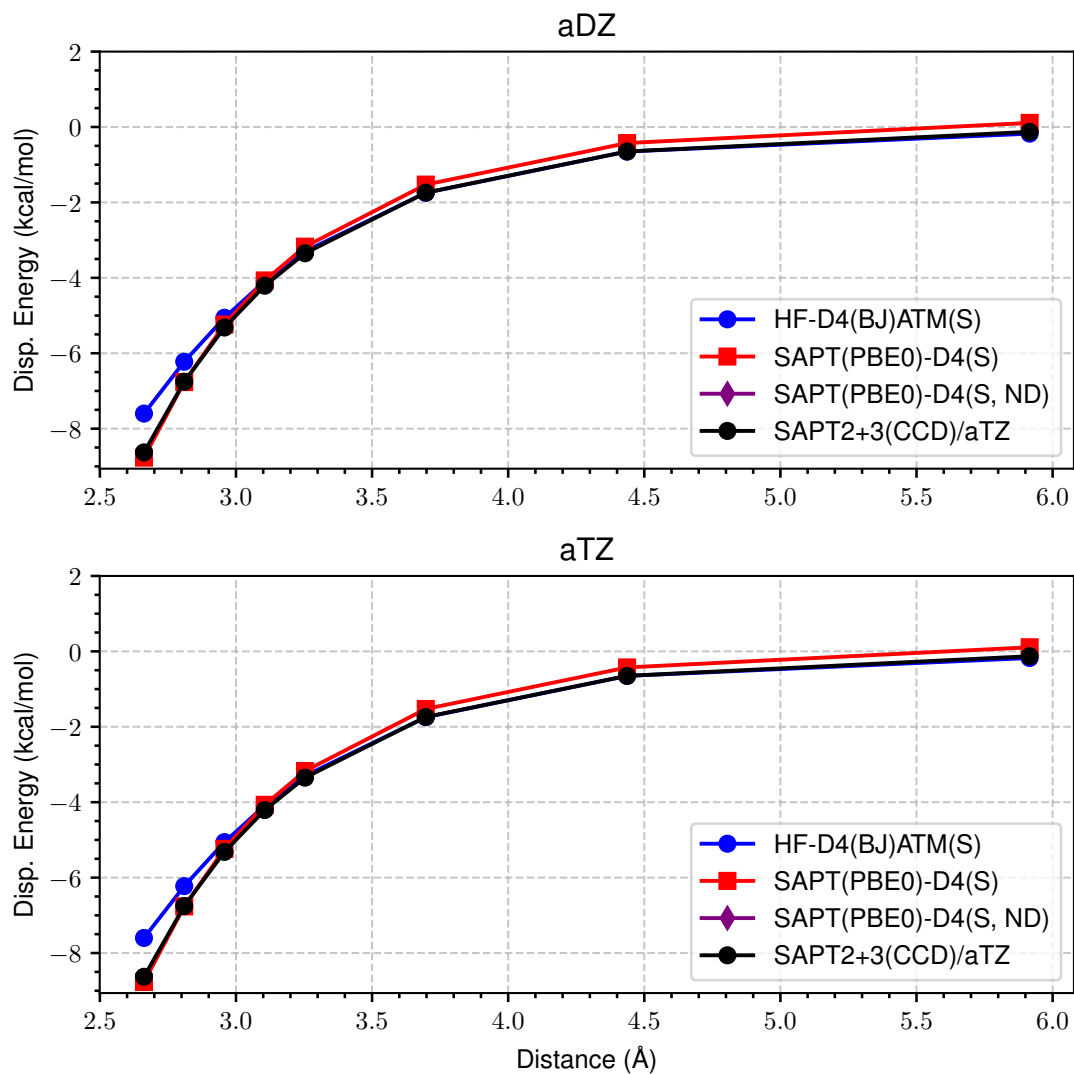
Figure 23: LoS Dispersion Curves for s66x8 31_Uracil-Ethene
