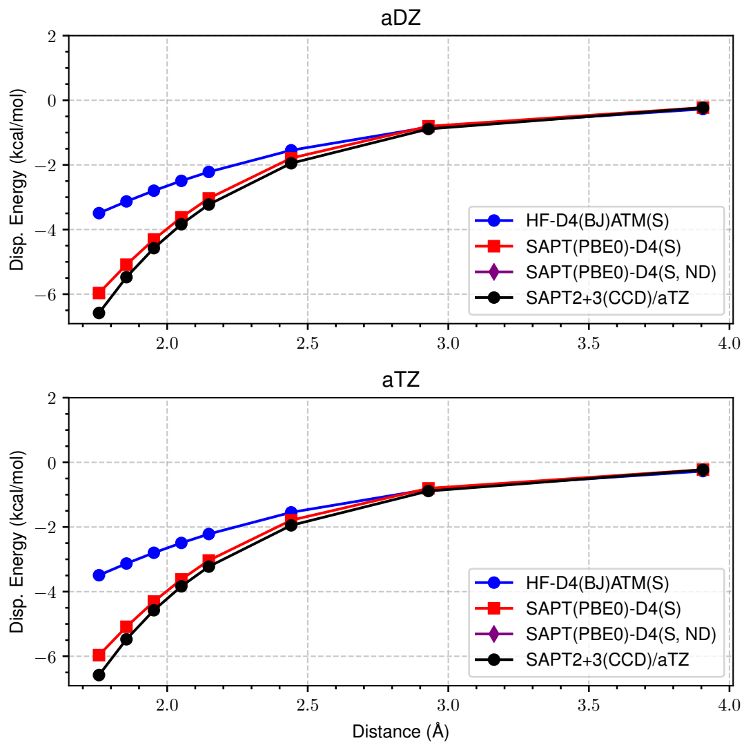
Figure 66: LoS Dispersion Curves for s66x8 19_MeOH-Pyridine
