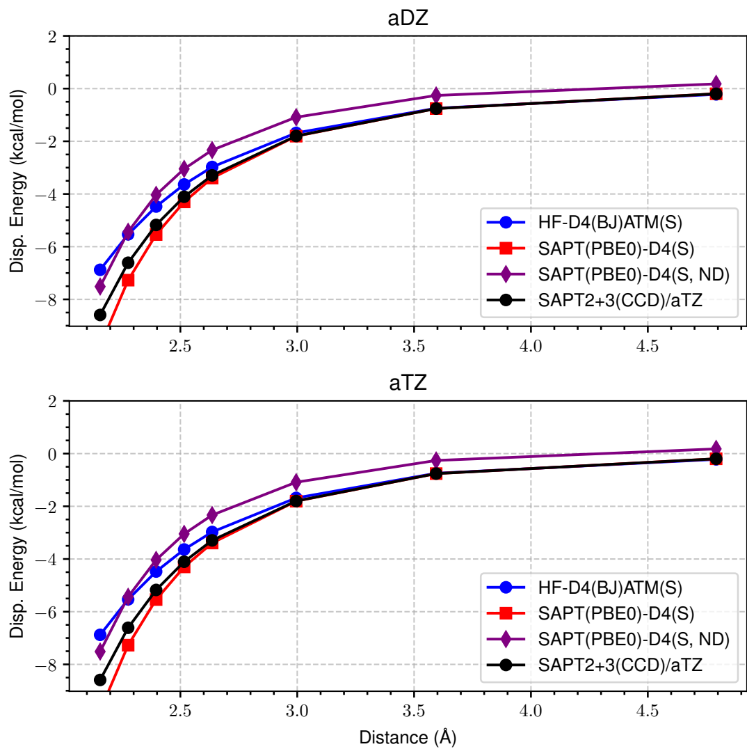
Figure 63: LoS Dispersion Curves for s66x8 37_Cyclopentane-Neopentane
