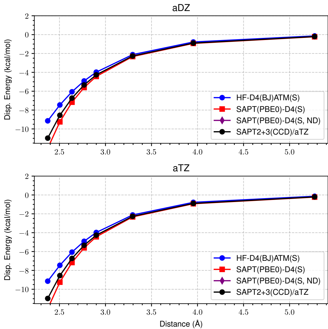
Figure 24: LoS Dispersion Curves for s66x8 57_Benzene-Peptide
