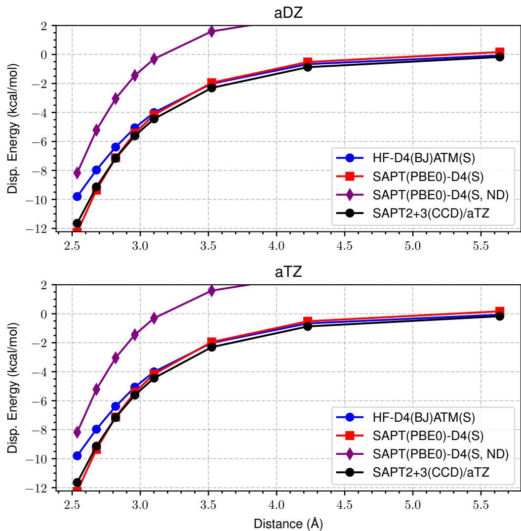
Figure 54: LoS Dispersion Curves for s66x8 39_Benzene-Cyclopentane
