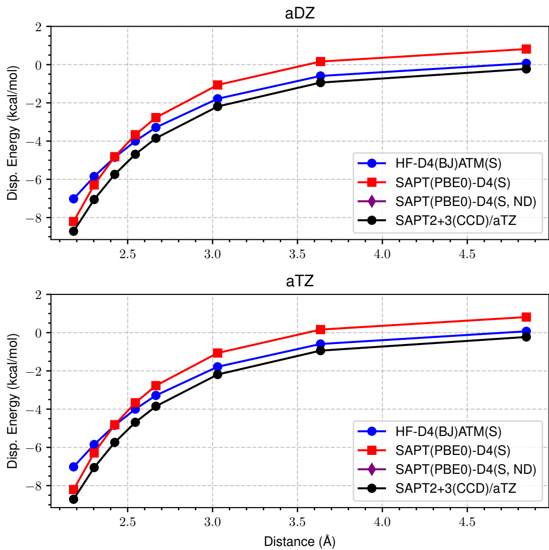
Figure 51: LoS Dispersion Curves for s66x8 62_Pentane-AcNH2
