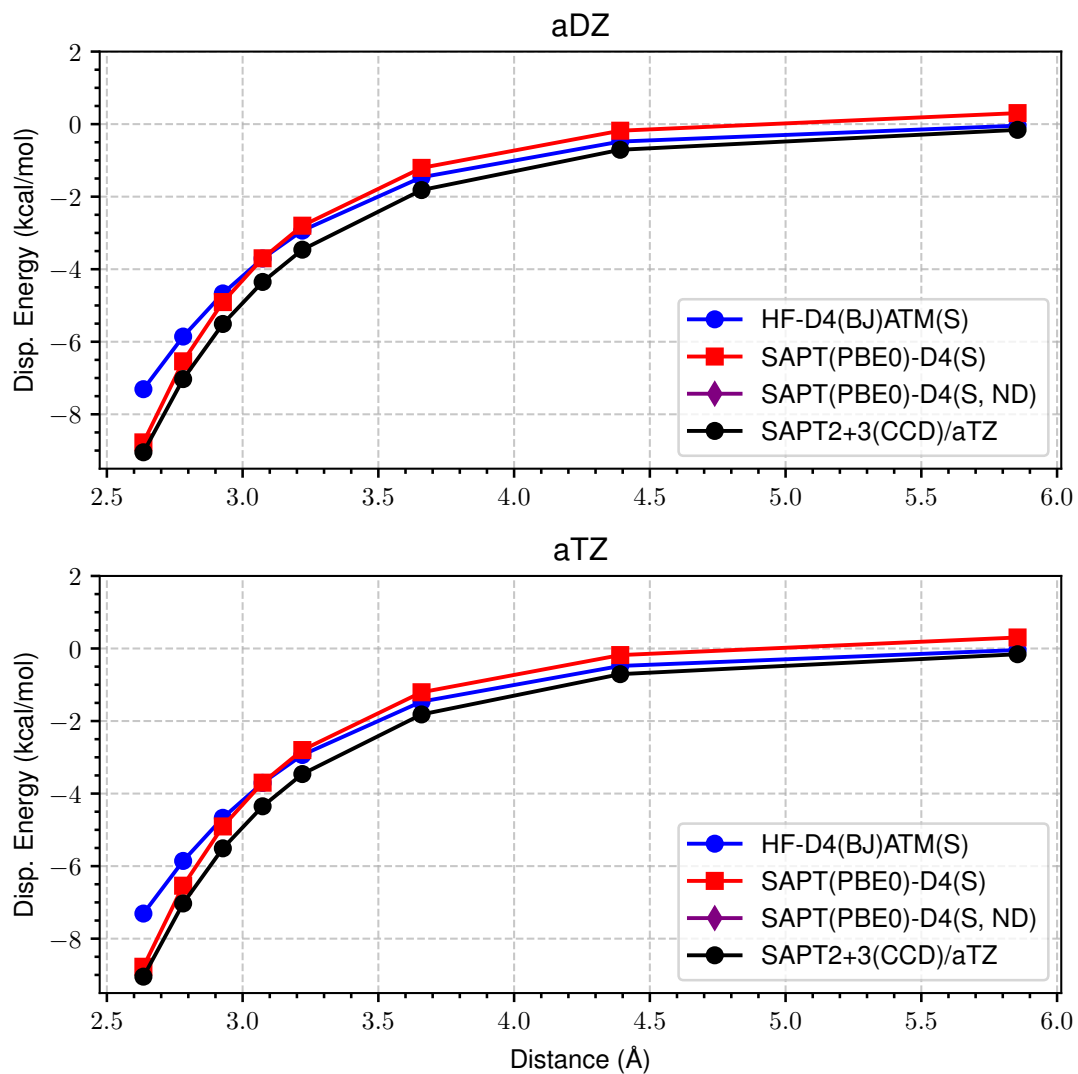
Figure 59: LoS Dispersion Curves for s66x8 40_Benzene-Neopentane
