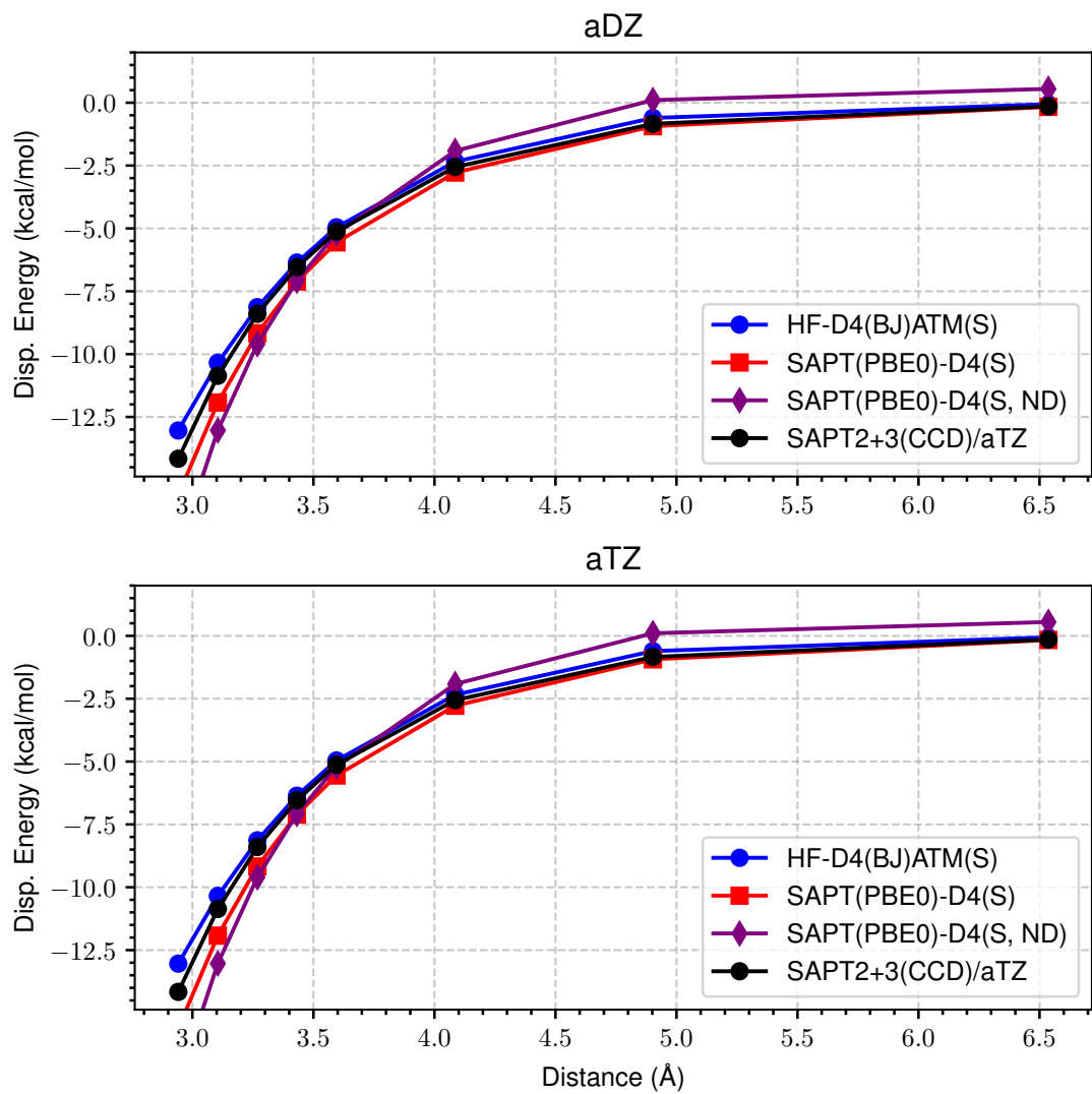
Figure 12: LoS Dispersion Curves for s66x8 25_Pyridine-Pyridine
