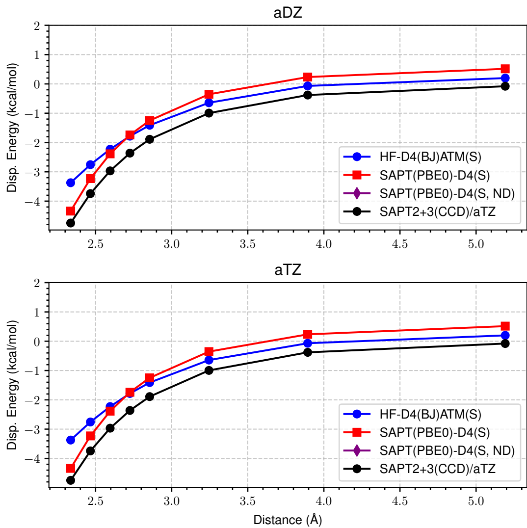
Figure 13: LoS Dispersion Curves for s66x8 54_Benzene-Water
