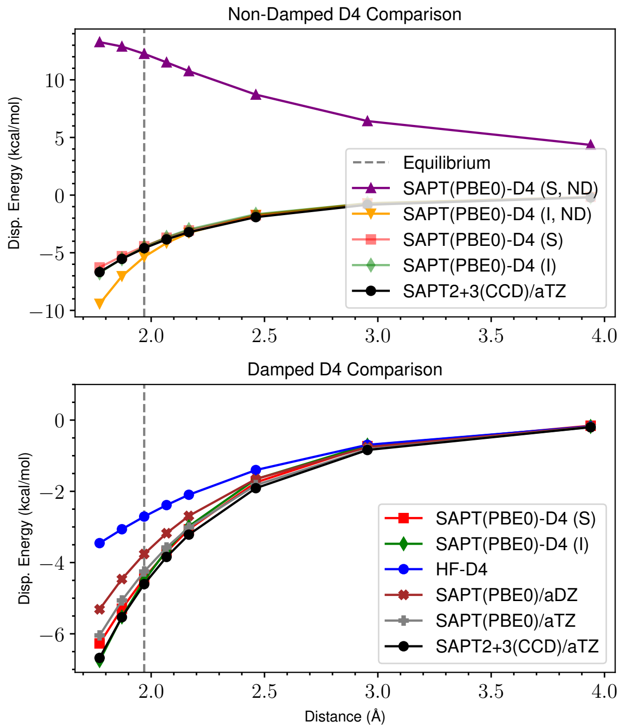
Figure 48: ND vs Damped D4 Dispersion for s66x8_06_MeOH-MeNH2
