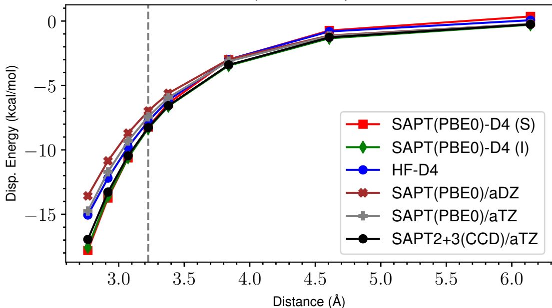
Damped D4 Comparison
