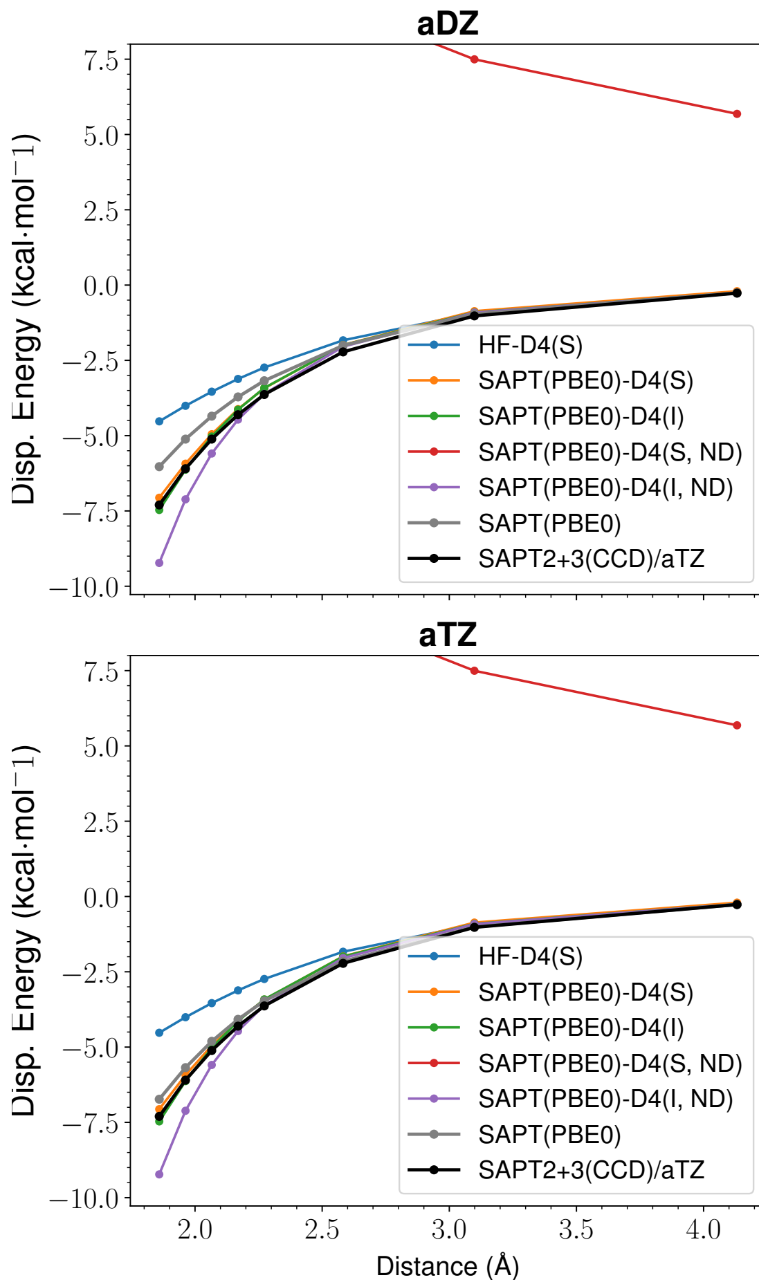
Figure 1: LoS Dispersion Curves for s66x8 14_Peptide-MeNH2
