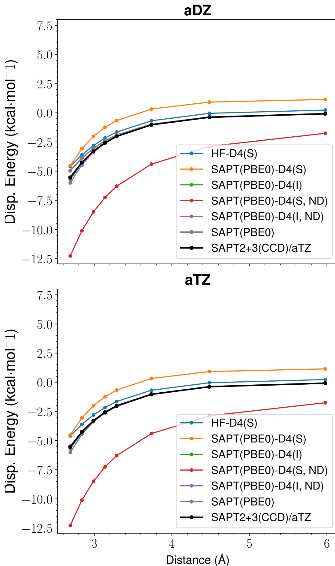
Figure 2: LoS Dispersion Curves for s66x8 45_Ethyne-Pentane
