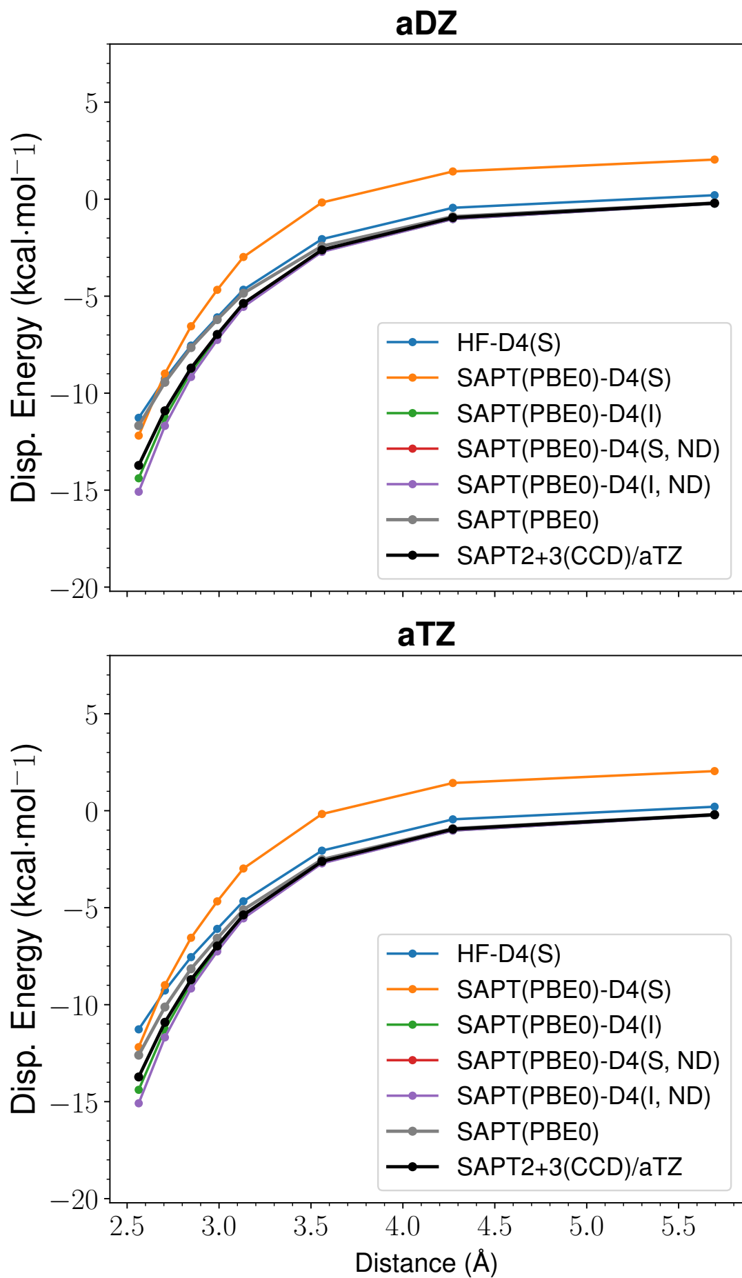
Figure 3: LoS Dispersion Curves for s66x8 41_Uracil-Pentane
